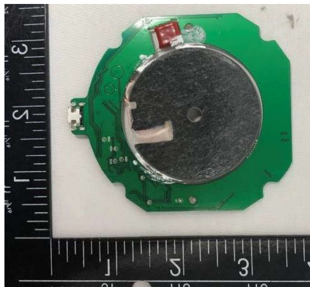
Fig 7. Internal View
