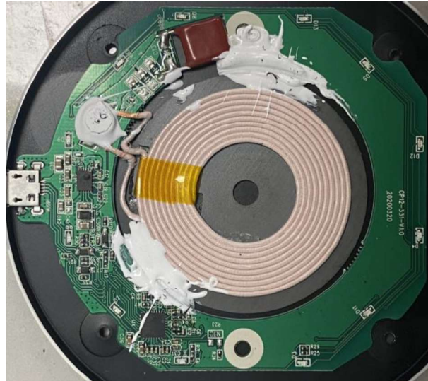
Fig 6. Internal View
