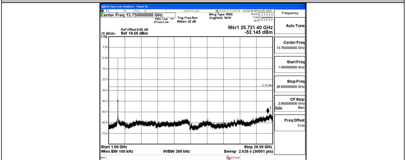
11N20SISO_Ant1_2412_0~Reference
