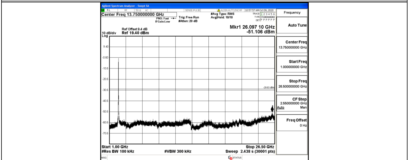
11N40SISO_Ant1_2437_0~Reference
