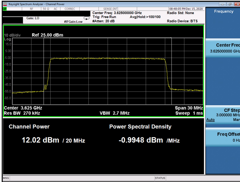
Plot 36. Conducted PSD, Mid-Channel SAS Granted maxEIRP 10 – Antenna 1
