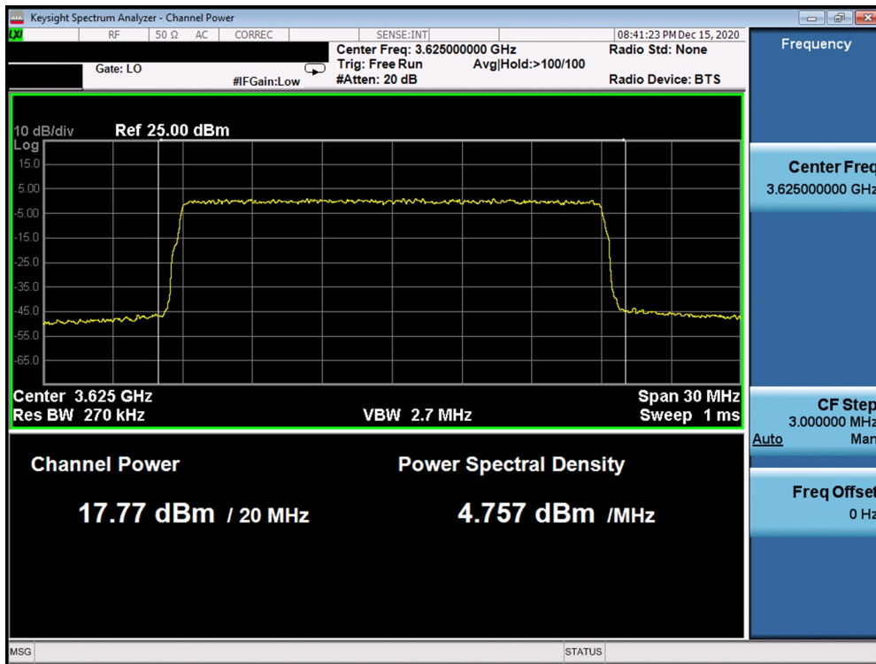
Plot 35. Conducted PSD, Mid-Channel SAS Granted maxEIRP 15 – Antenna 2
