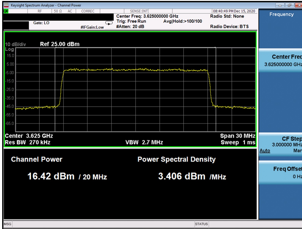
Plot 34. Conducted PSD, Mid-Channel SAS Granted maxEIRP 15 – Antenna 1
