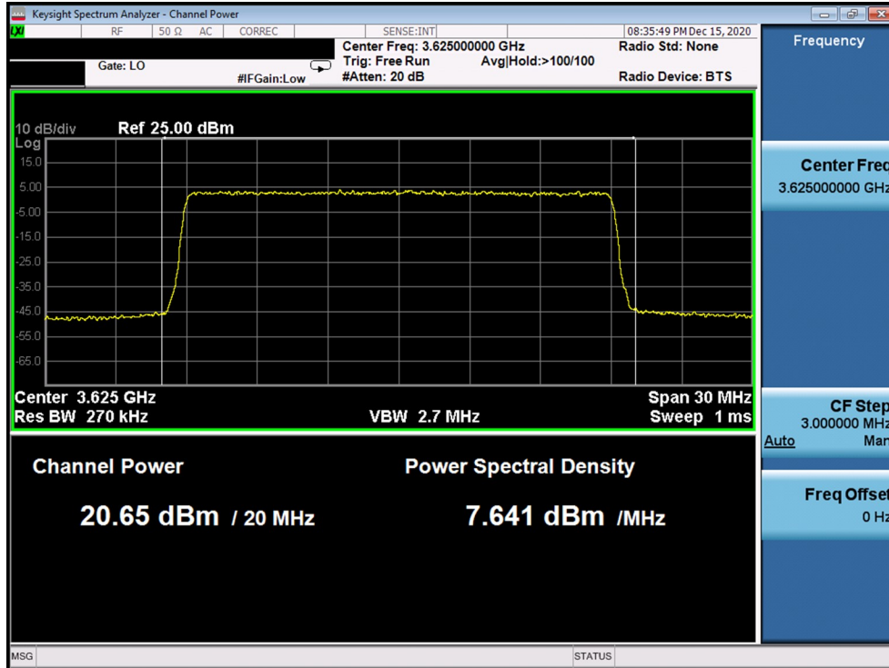
Plot 33. Conducted PSD, Mid-Channel SAS Granted maxEIRP 19 – Antenna 2
