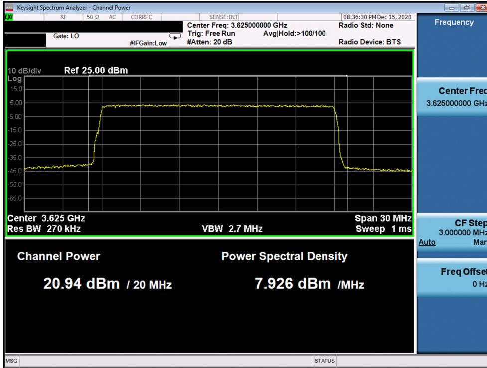
Plot 32. Conducted PSD, Mid-Channel SAS Granted maxEIRP 19 – Antenna 1
