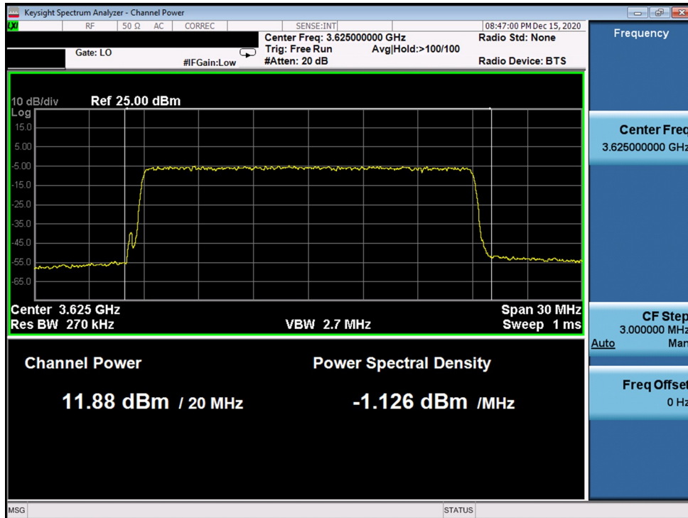
Plot 37. Conducted PSD, Mid-Channel SAS Granted maxEIRP 10 – Antenna 2
