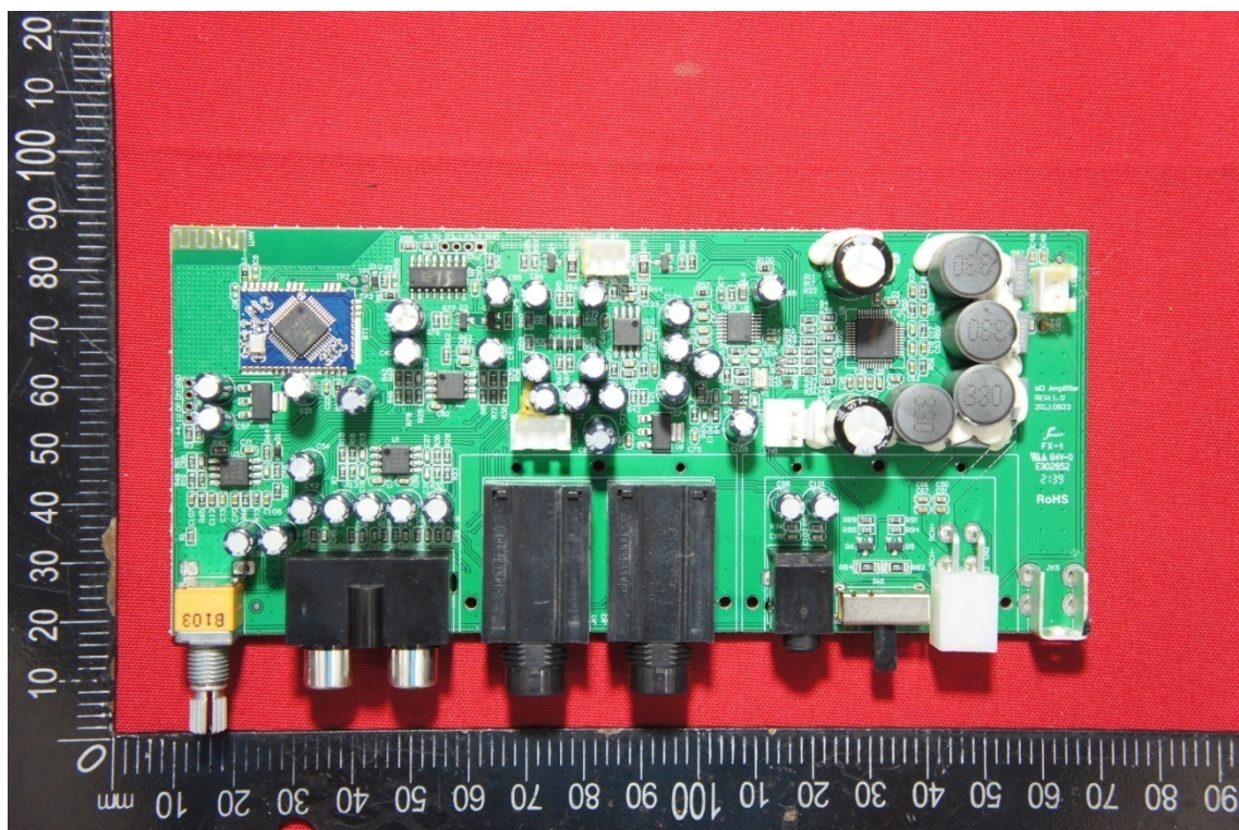
Main PCB
