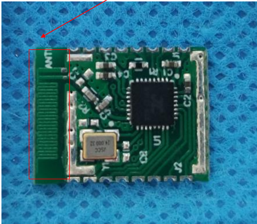
BT antenna
