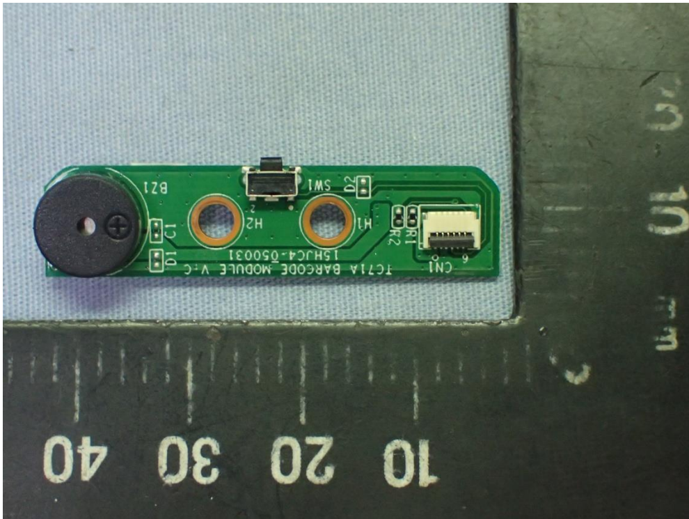
Figure 50 Barcode Scanner mPAD, Internal View (Switch Board, Front View)
