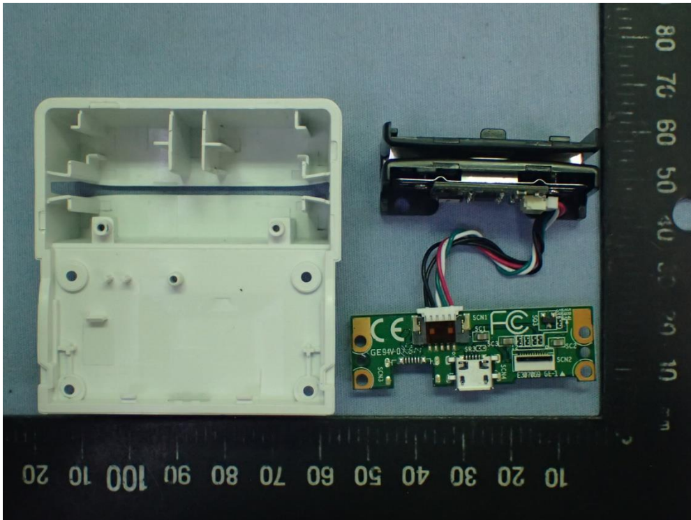
Figure 60 MSR Module, Internal View
