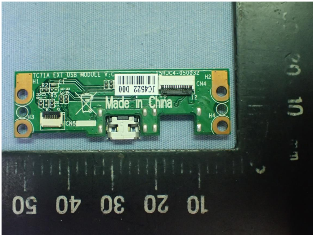
Figure 67 USB Ethernet mPAD, Internal View (USB Board, Back View)
