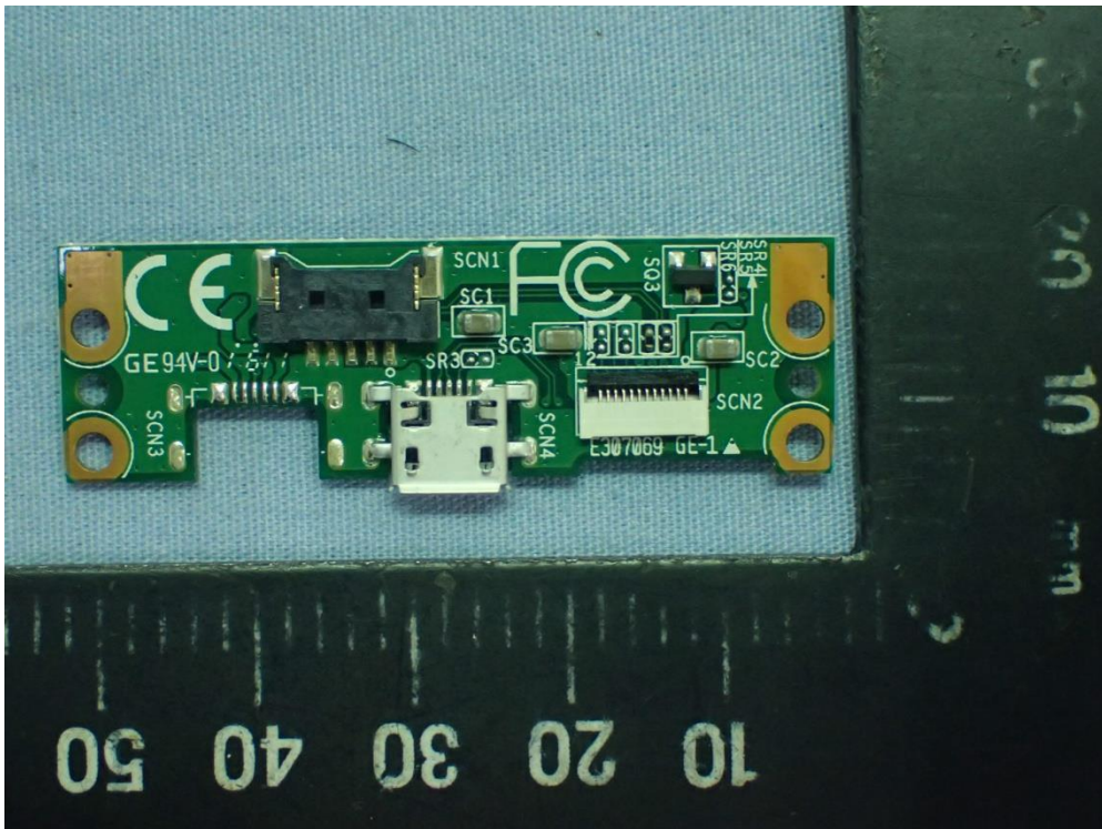
Figure 55 SCR mPAD, Internal View (USB Board, Front View)
