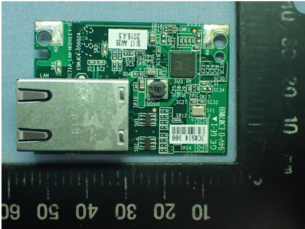
Figure 68 USB Ethernet mPAD, Internal View (LAN Board, Front View)
