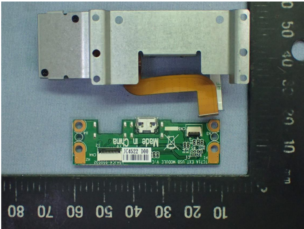
Figure 47 Barcode Scanner mPAD, Internal View (USB Board, Front View)
