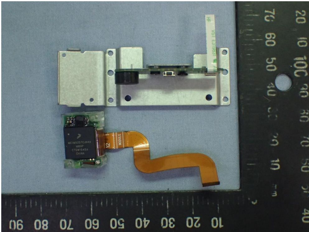
Figure 52 Barcode Scanner mPAD, Internal View
