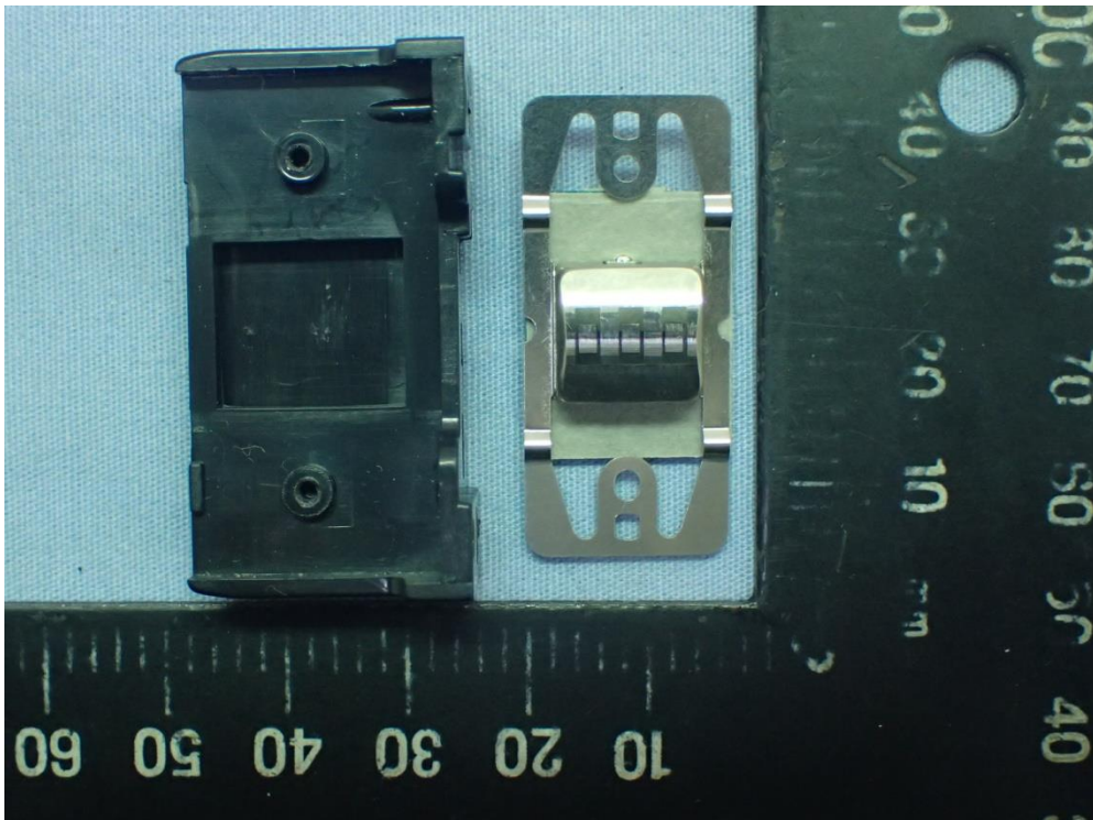
Figure 63 MSR Module, Internal View
