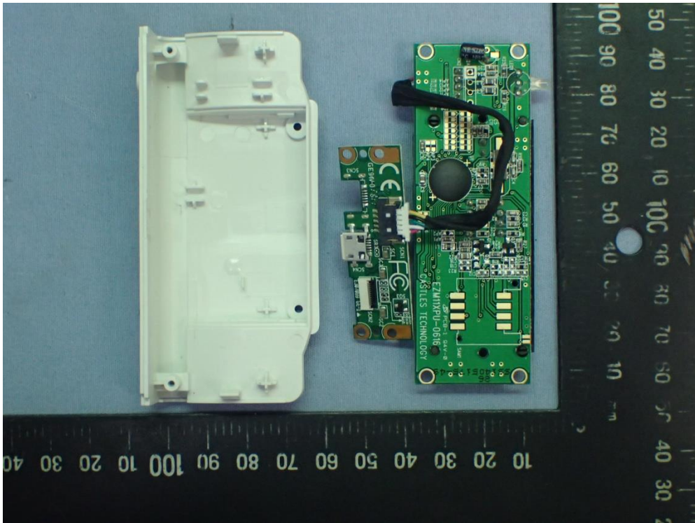
Figure 54 SCR mPAD, Internal View (Removed Cover)
