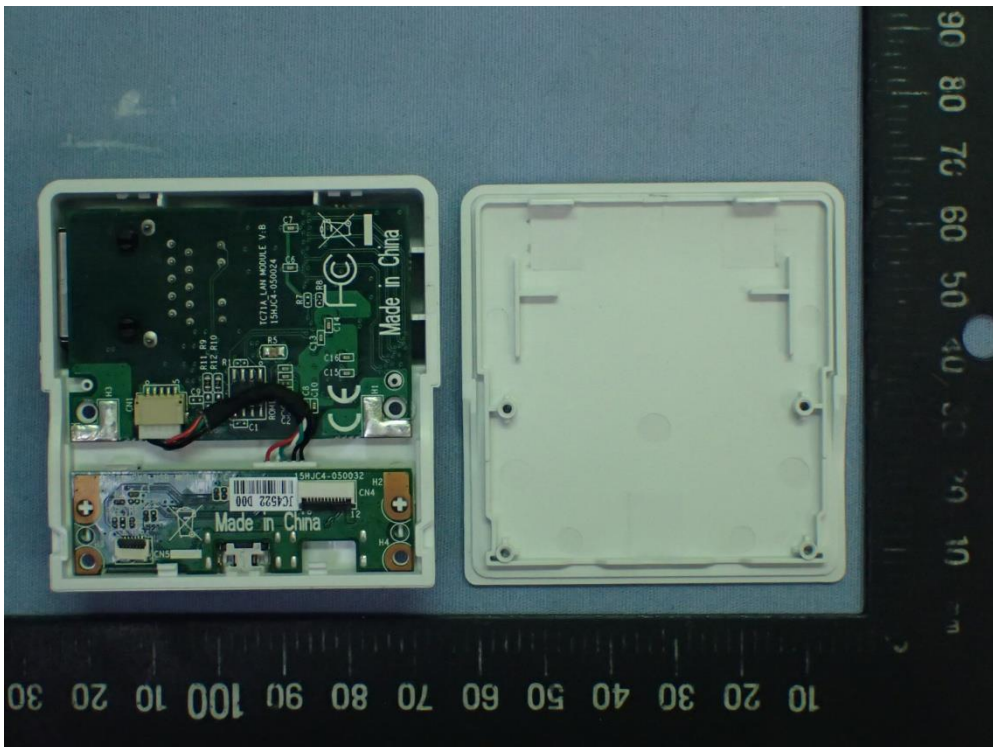
Figure 65 USB Ethernet mPAD, Internal View
