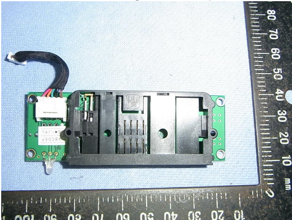
Figure 71 7" Pad Docking, Internal View (Control Board, Front View)
