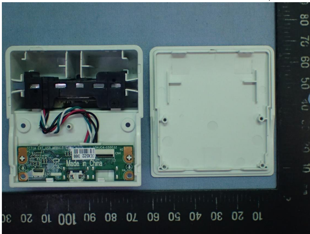
Figure 59 MSR Module, Internal View (Removed Cover)
