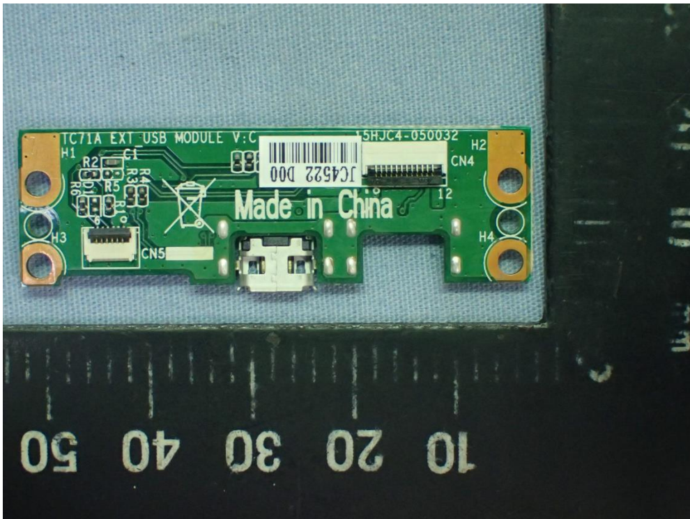
Figure 56 SCR mPAD, Internal View (USB Board, Back View)
