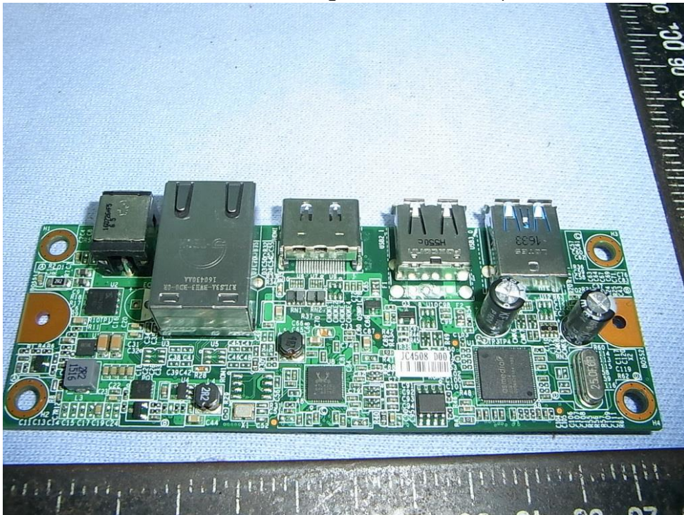
Figure 74 7" Pad Docking, Internal View (Control Board, Front View)
