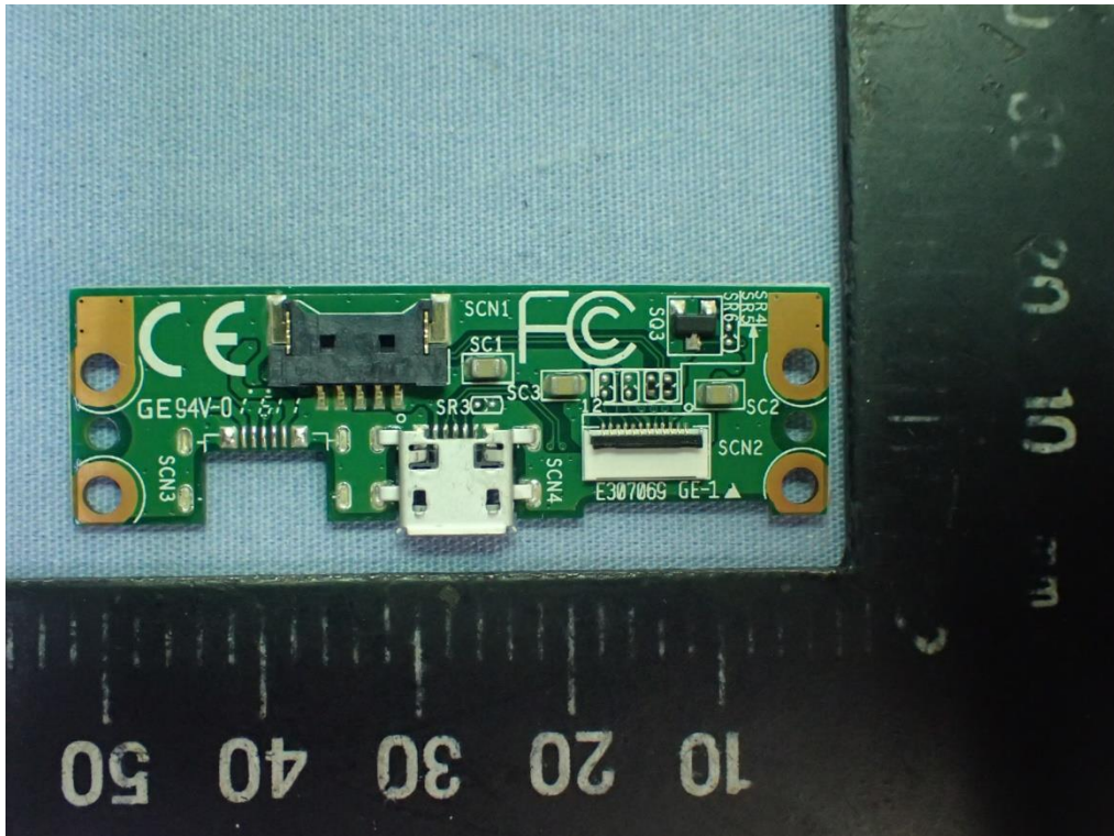
Figure 66 USB Ethernet mPAD, Internal View (USB Board, Front View)
