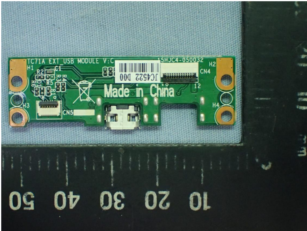
Figure 48 Barcode Scanner mPAD, Internal View (USB Board, Back View)
