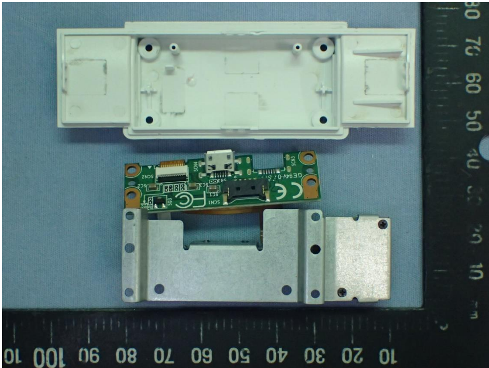
Figure 46 Barcode Scanner mPAD, Internal View (Removed USB Board)
