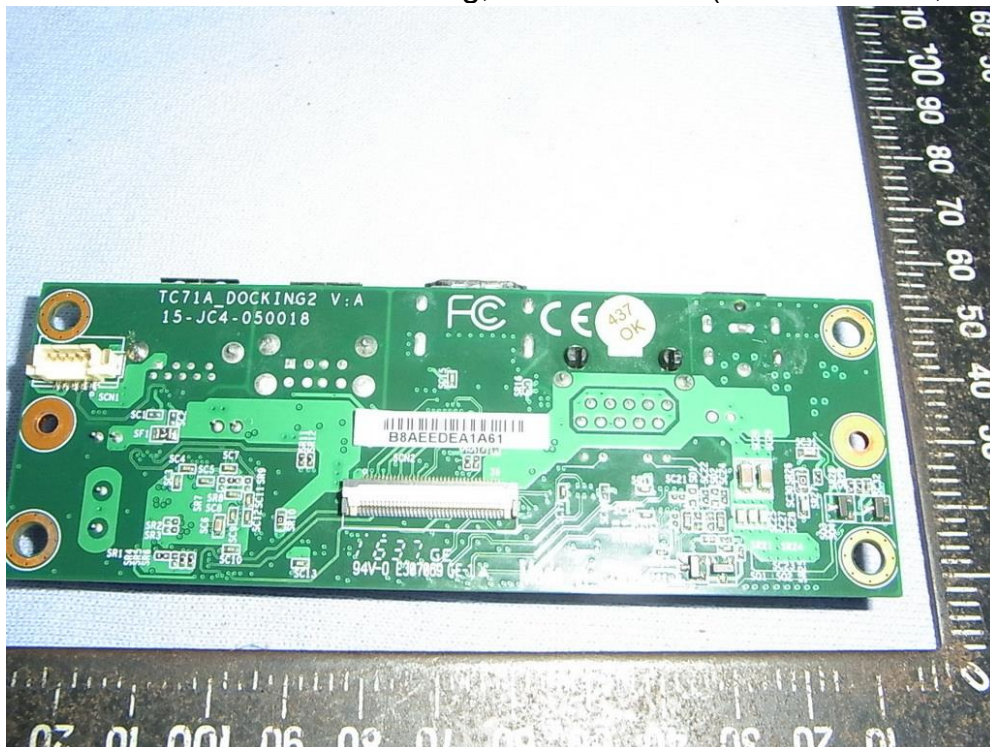
Figure 75 7" Pad Docking, Internal View (Control Board, Back View)
