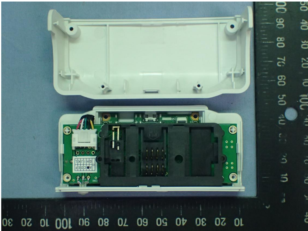
Figure 53 SCR mPAD, Internal View (Removed Cover)
