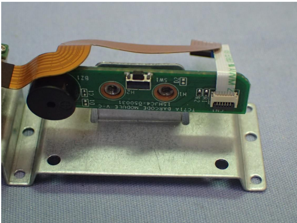
Figure 49 Barcode Scanner mPAD, Internal View
