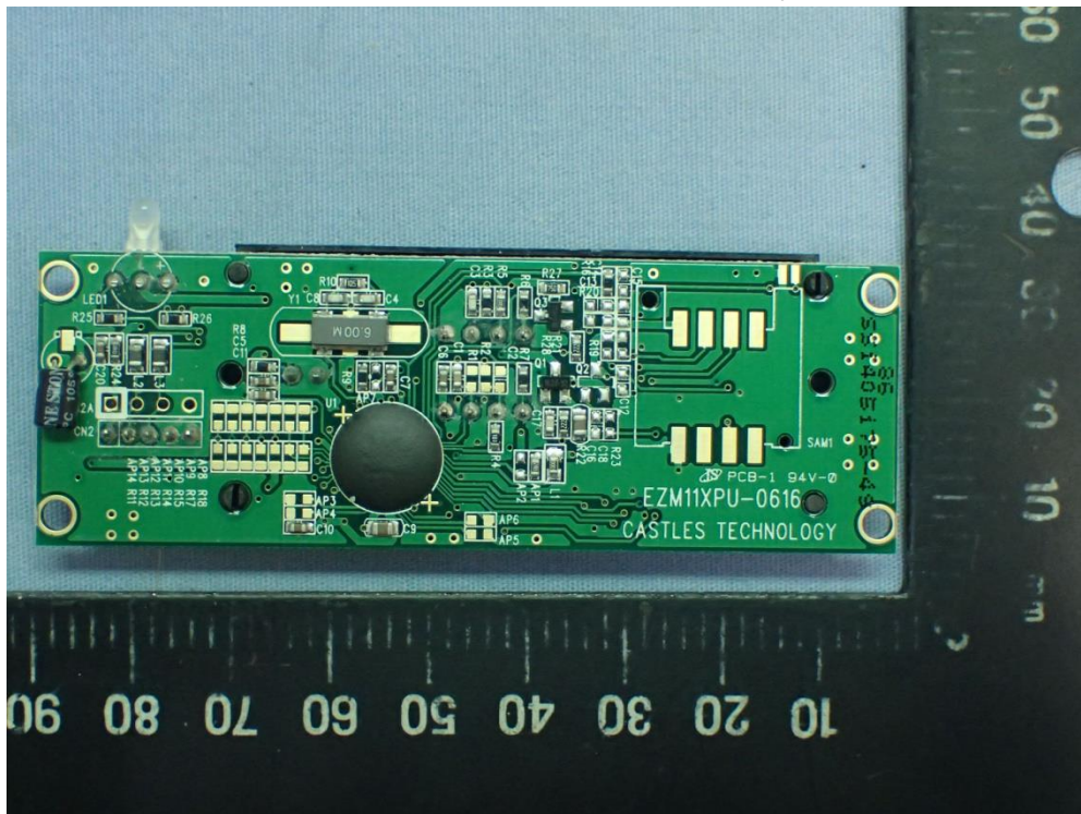
Figure 58 SCR mPAD, Internal View (Control Board, Back View)
