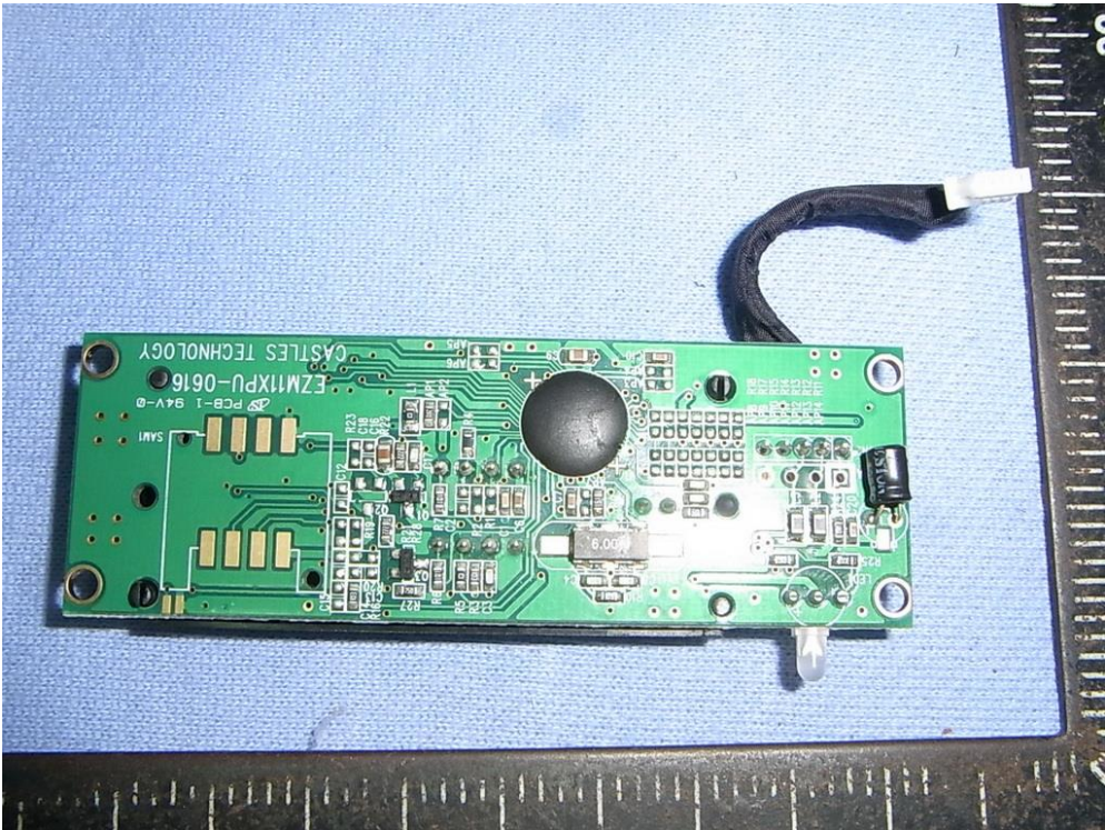
Figure 72 7" Pad Docking, Internal View (Control Board, Back View)
