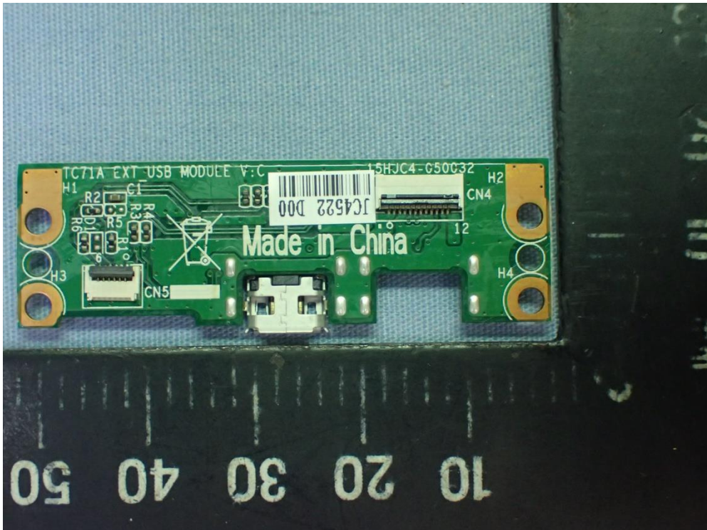
Figure 62 MSR Module, Internal View (USB Board, Back View)
