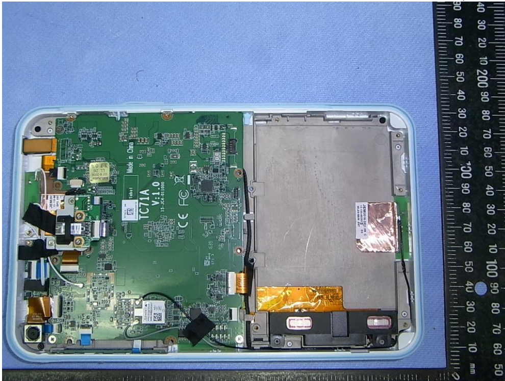
Figure 24 Medical Grade Mobile Tablet PC, Internal View
