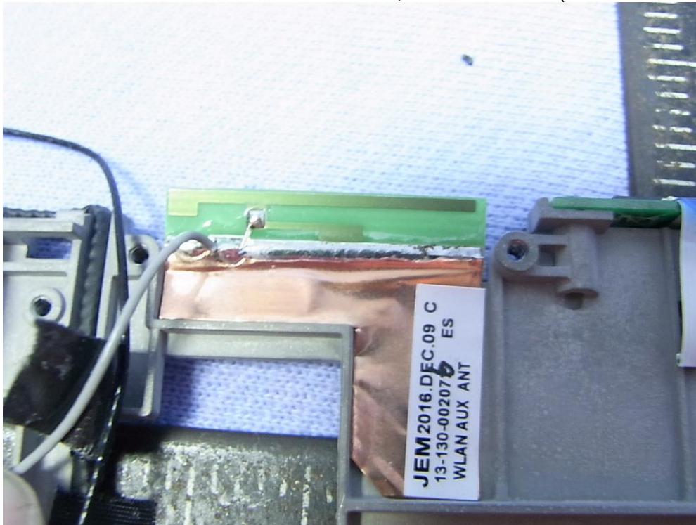
Figure 36 Medical Grade Mobile Tablet PC, Internal View (WLAN Aux Antenna)
