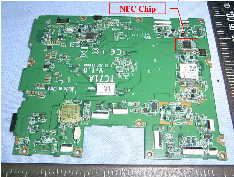
Figure 30 Medical Grade Mobile Tablet PC, Internal View (Main Board, Back View)
