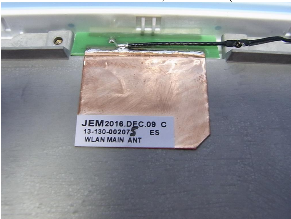
Figure 35 Medical Grade Mobile Tablet PC, Internal View (WLAN Main Antenna)
