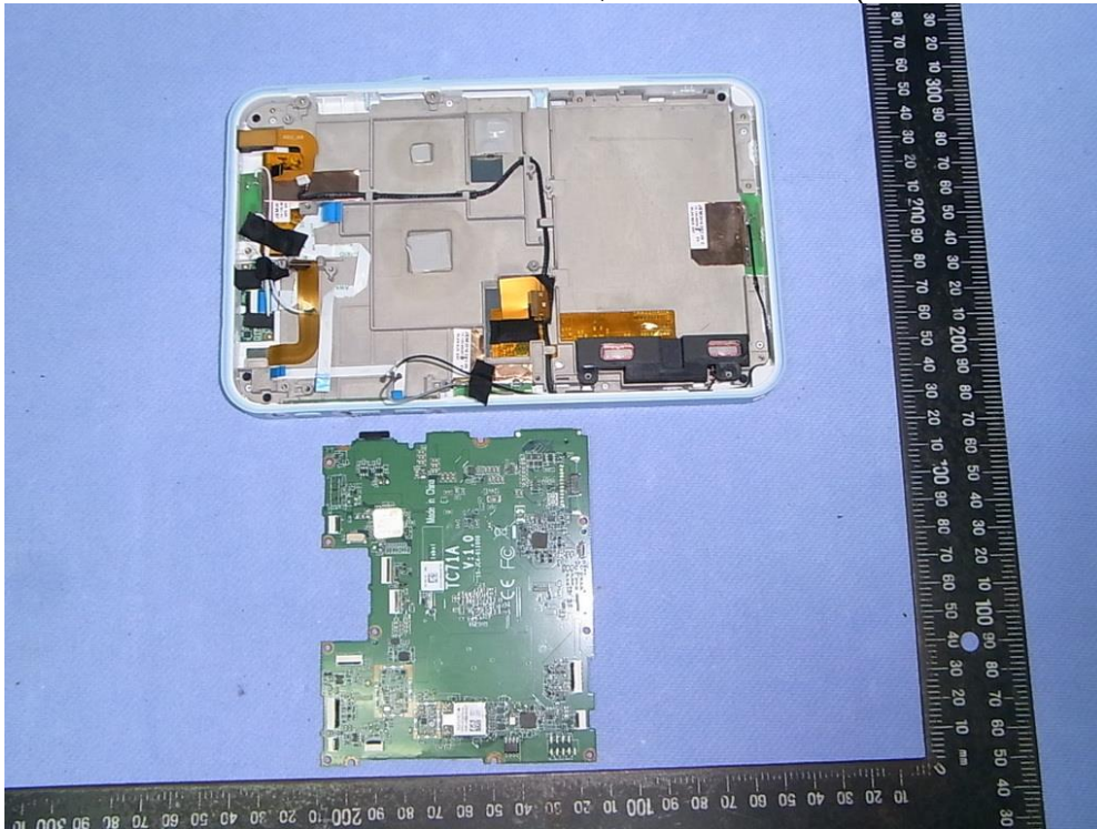
Figure 28 Medical Grade Mobile Tablet PC, Internal View (Removed Main Board)
