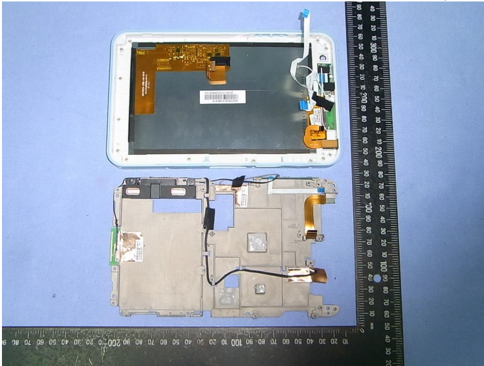
Figure 34 Medical Grade Mobile Tablet PC, Internal View
