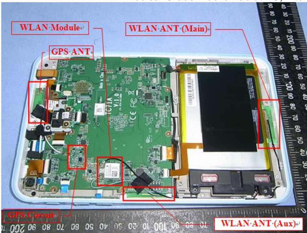
Figure 23 Medical Grade Mobile Tablet PC, Internal View
