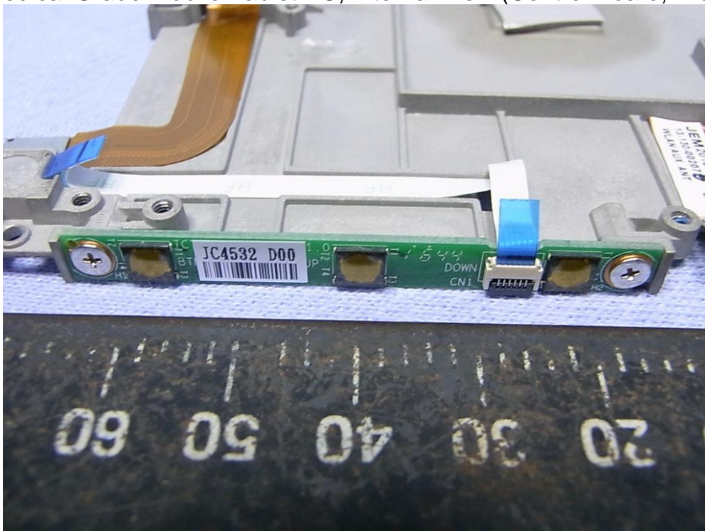
Figure 37 Medical Grade Mobile Tablet PC, Internal View (Control Board, Front View)
