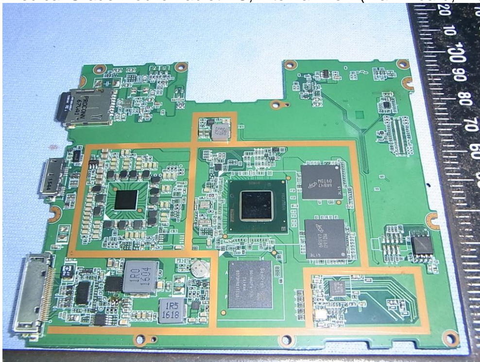
Figure 29 Medical Grade Mobile Tablet PC, Internal View (Main Board, Front View)
