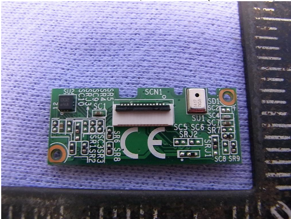
Figure 39 Medical Grade Mobile Tablet PC, Internal View (Control Board, Front View)
