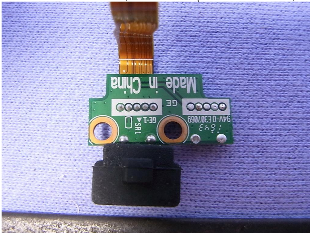
Figure 27 Medical Grade Mobile Tablet PC, Internal View (USB Control Board, Back View)
