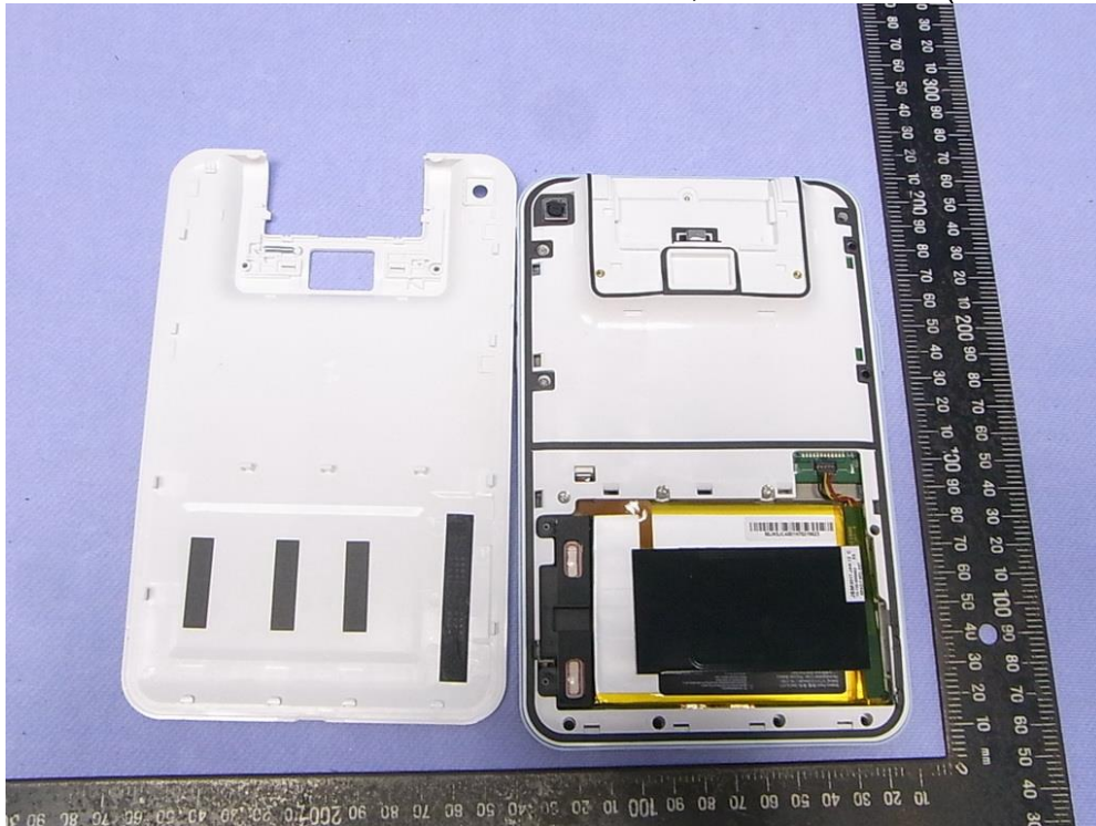
Medical Grade Mobile Tablet PC, Internal View (Removed Cover)
