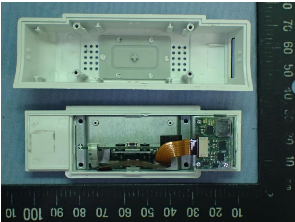
Figure 45 Barcode Scanner mPAD, Internal View (Removed Cover)
