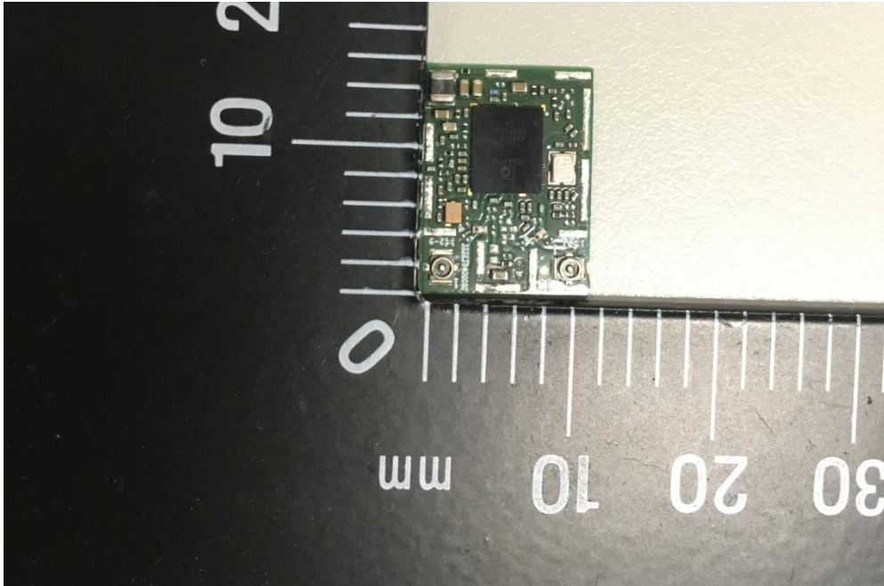
Figure 32 Medical Grade Mobile Tablet PC, Internal View (Wireless Module/Front View, Removed Cover)
