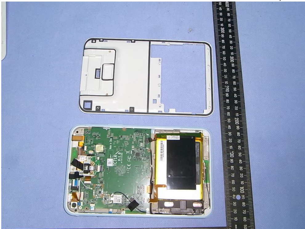
Medical Grade Mobile Tablet PC, Internal View
