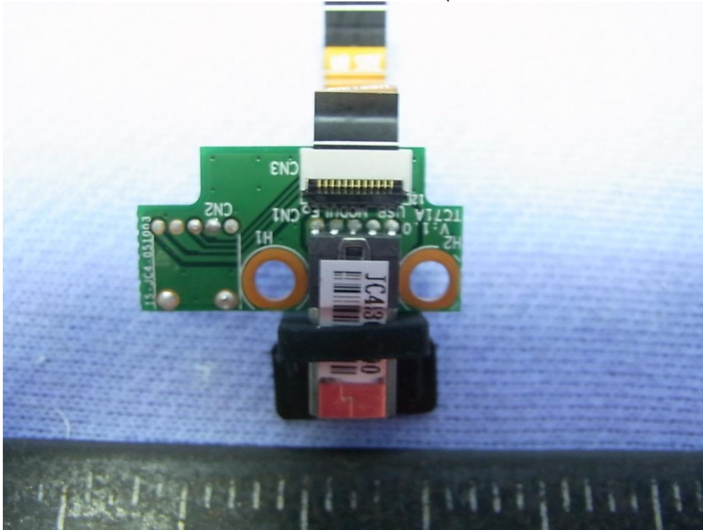
Figure 26 Medical Grade Mobile Tablet PC, Internal View (USB Control Board, Front View)
