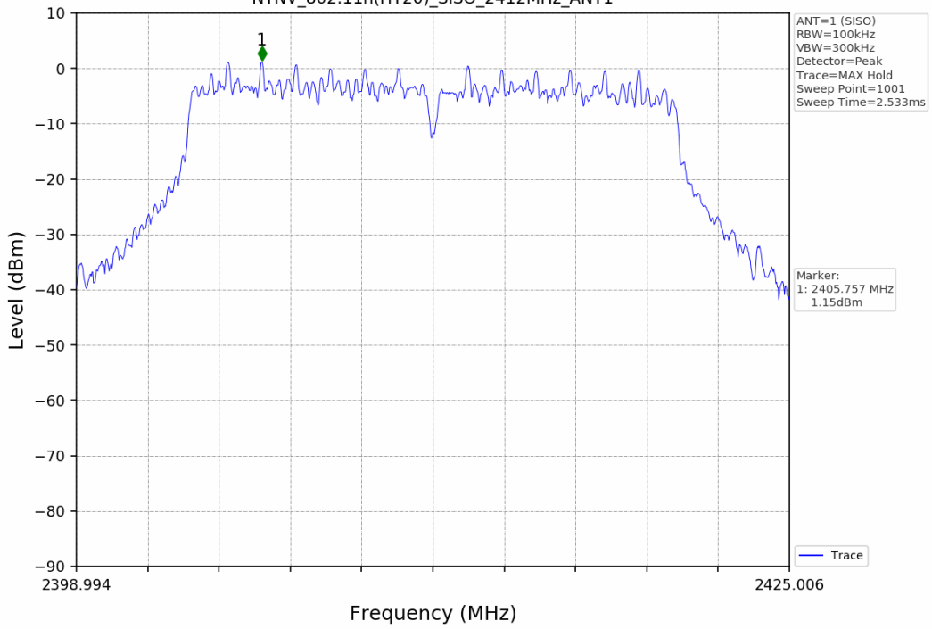
Unwanted Emissions in Non-restricted Frequency Bands NTNV_802.11n(HT20)_SISO_2412MHz_ANT1
