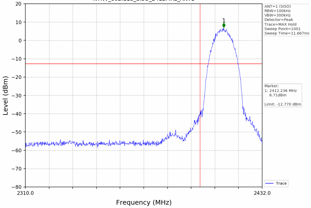
Unwanted Emissions in Non-restricted Frequency Bands NTNV_802.11b_SISO_2412MHz_ANT1
