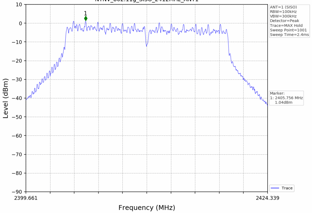
Unwanted Emissions in Non-restricted Frequency Bands NTNV_802.11g_SISO_2412MHz_ANT1
