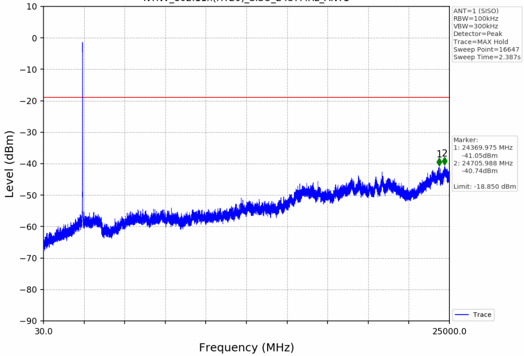
Unwanted Emissions in Non-restricted Frequency Bands NTNV_802.11n(HT20)_SISO_2437MHz_ANT1
