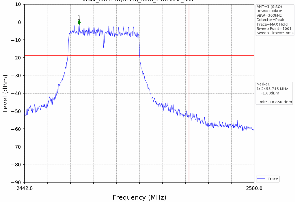
Unwanted Emissions in Non-restricted Frequency Bands NTNV_802.11n(HT20)_SISO_2462MHz_ANT1
