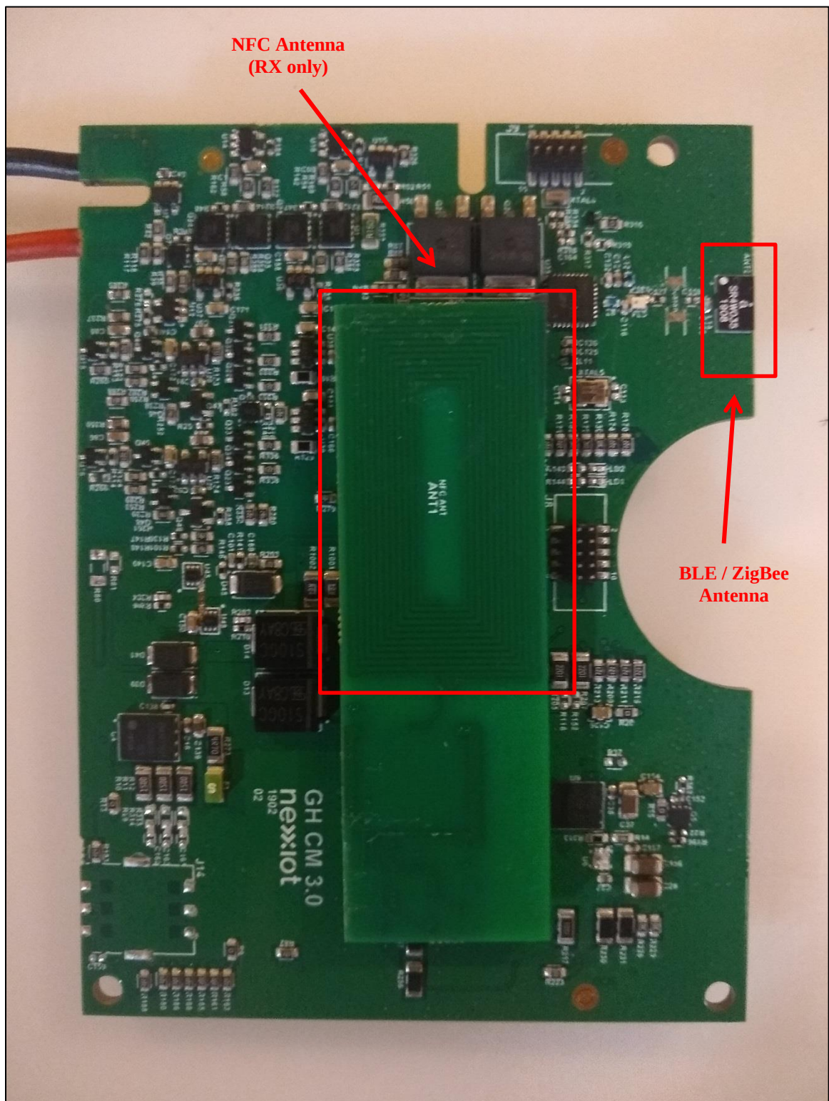
Photograph 4: PCB Back
