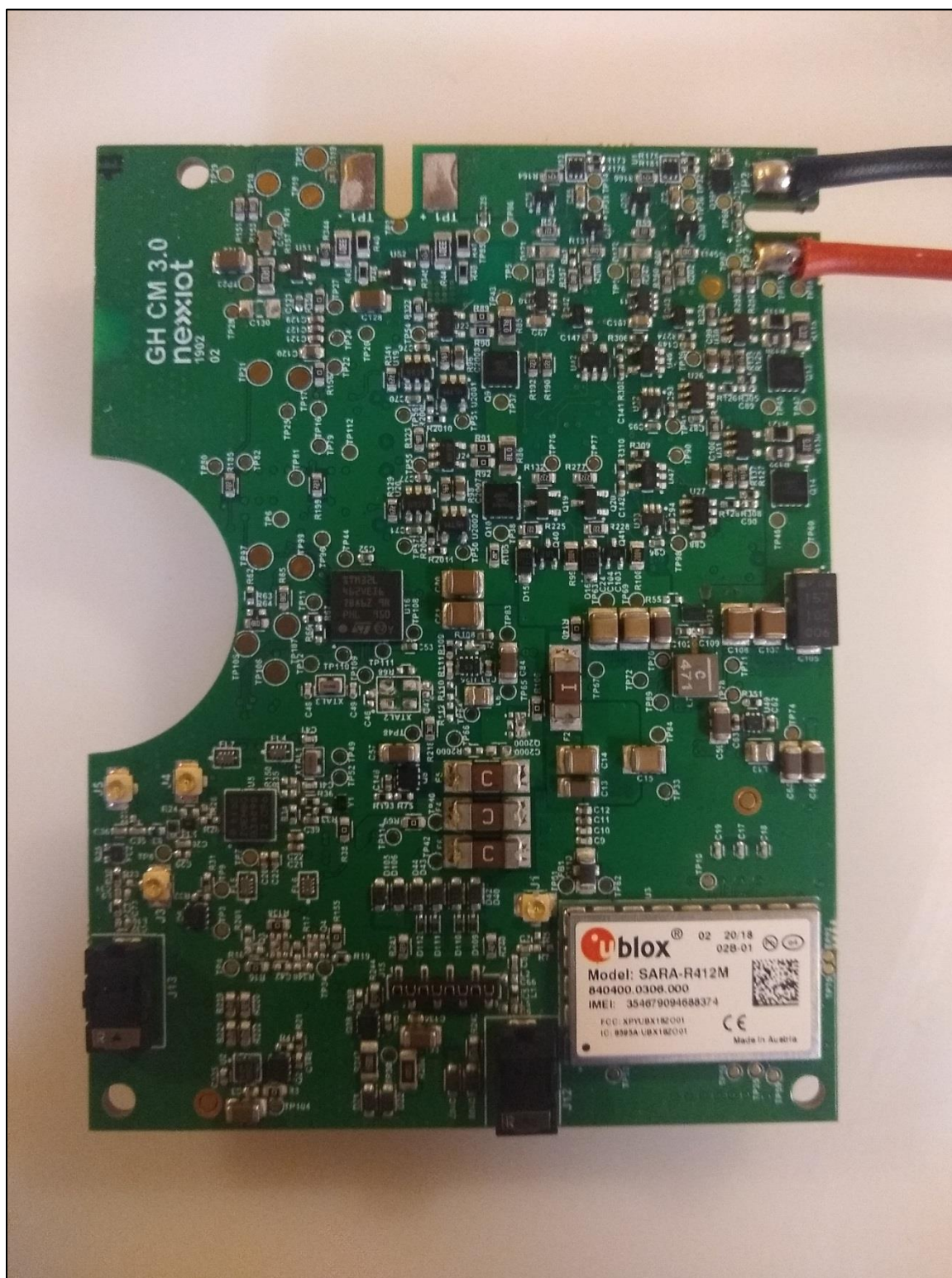
Photograph 3: PCB Front
