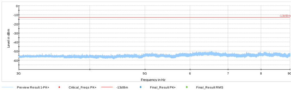
Plot #10 Radiated Emissions: 3-9 GHz
