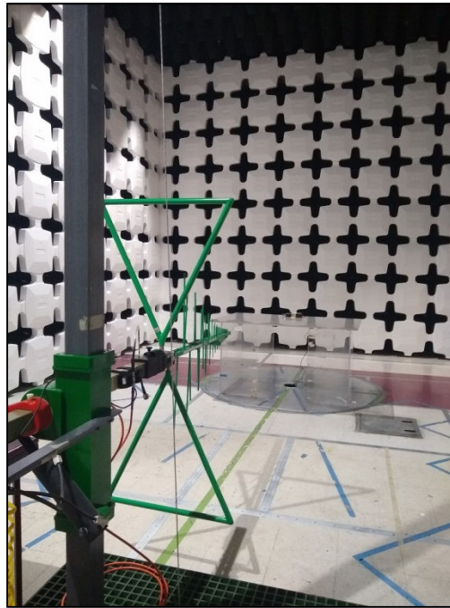
Radiated Spurious Emissions, Below 1GHz, Test Setup
