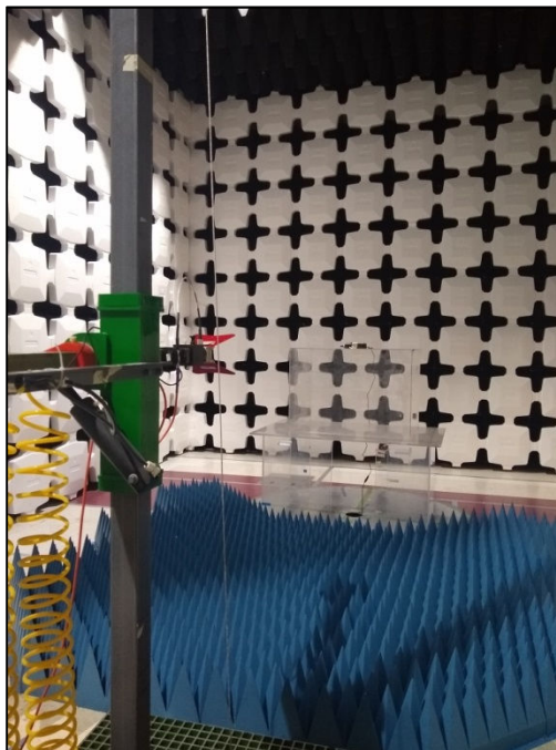
Radiated Spurious Emissions, Above 1GHz, Test Setup
