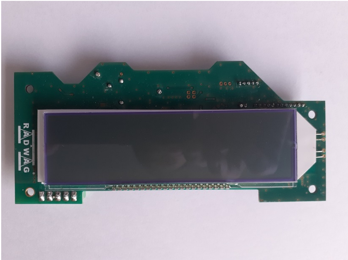
PCB 240R2003 Top view
