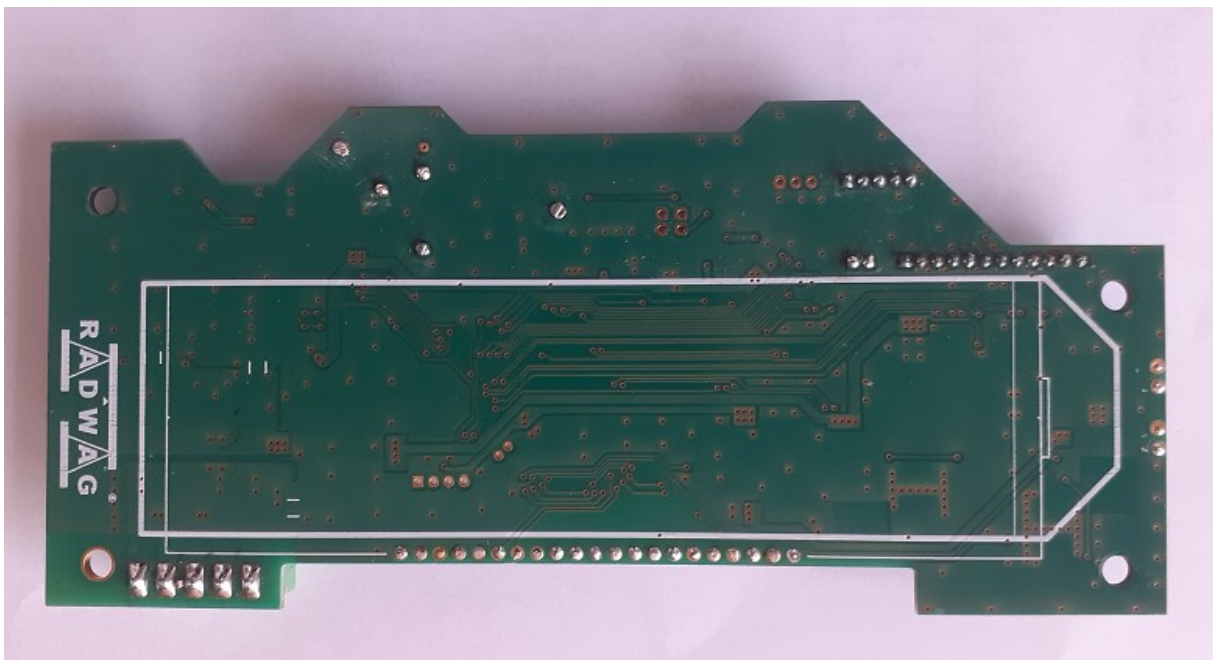
PCB 240R2003 Top view with unsoldered display
