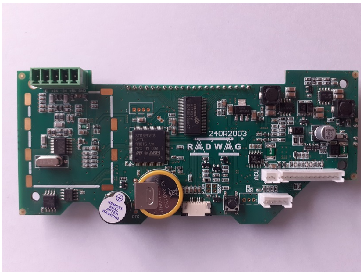
PCB 240R2003 Bottom view
