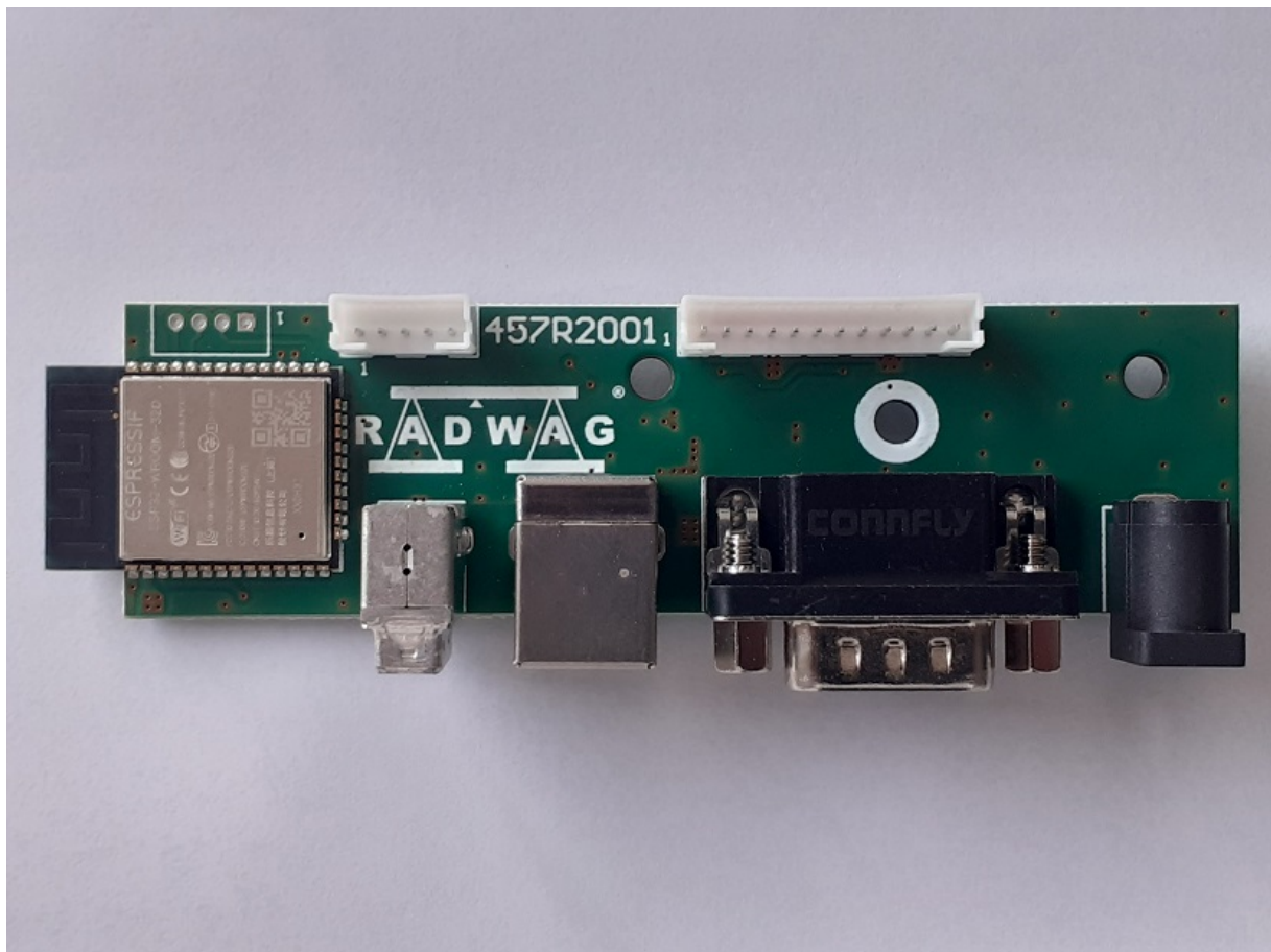
PCB 457R2001 Top view
