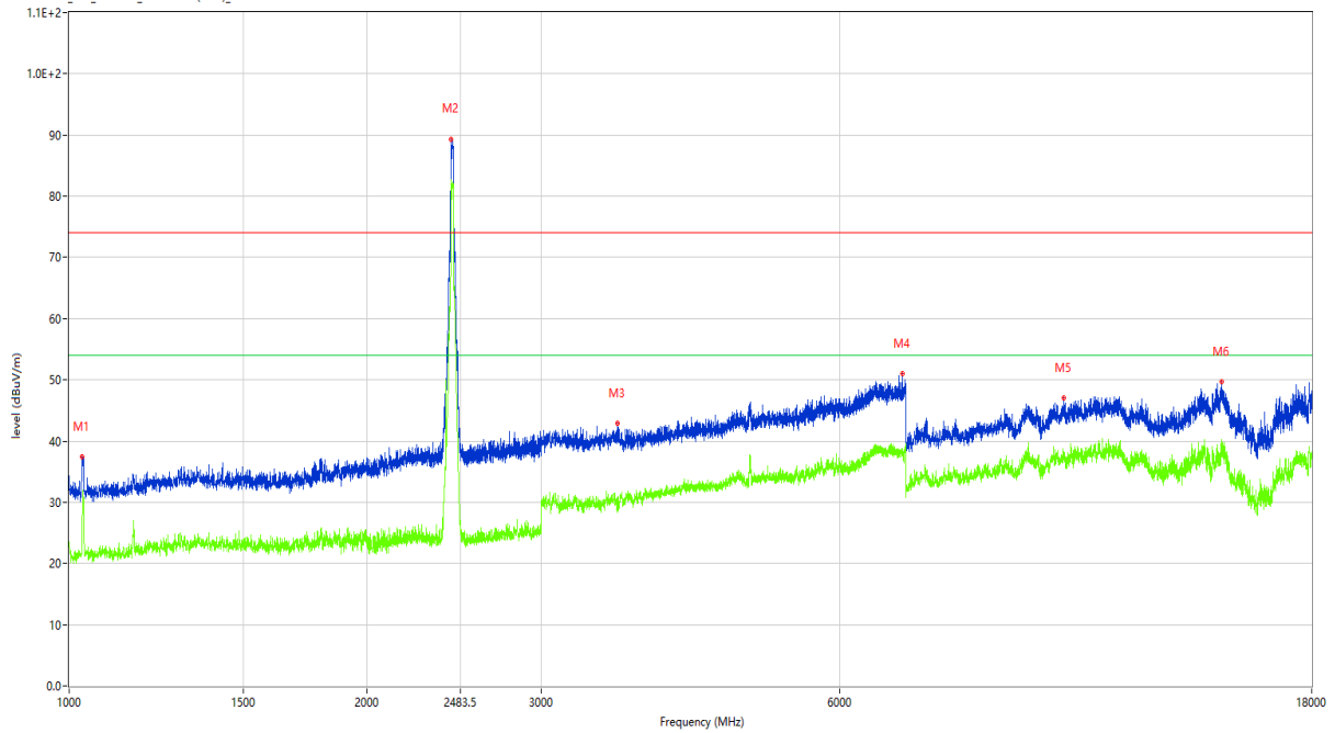
RE Test case FCC_Part 15C_FCC 15.247(2.45)_1GHz-18GHz
