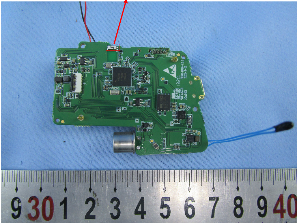
Bluetooth Antenna
