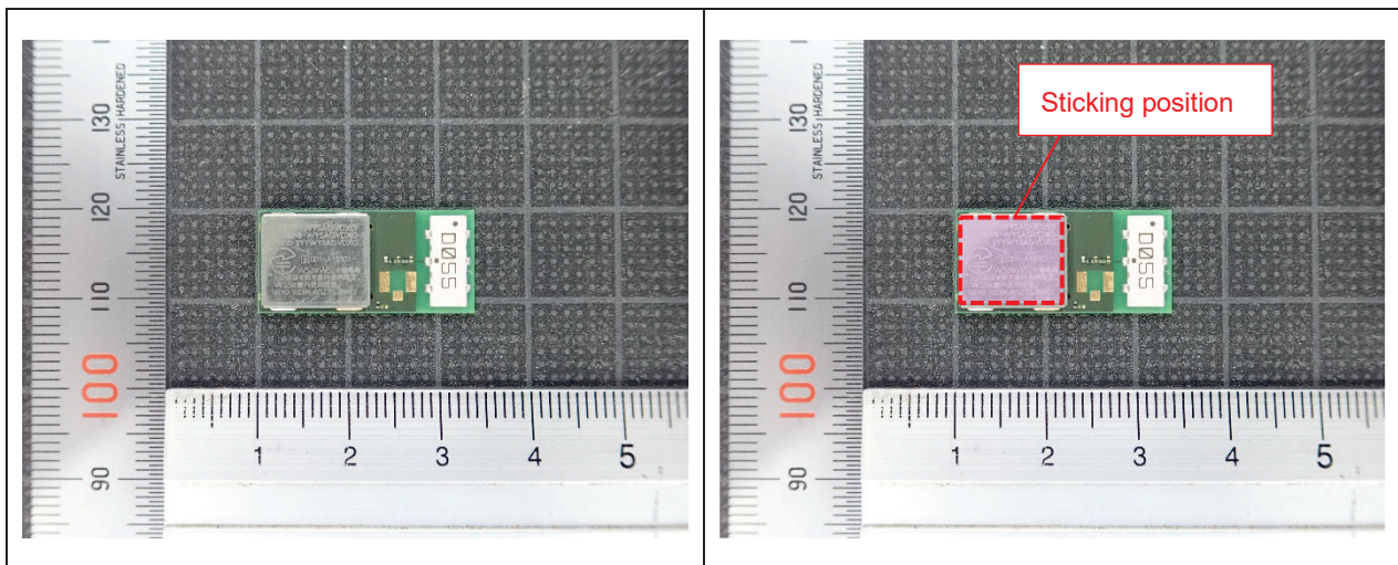
Figure 2 Sticking position
