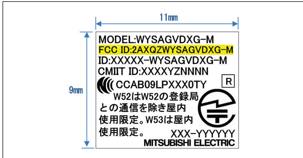
Figure 1 Label specification
