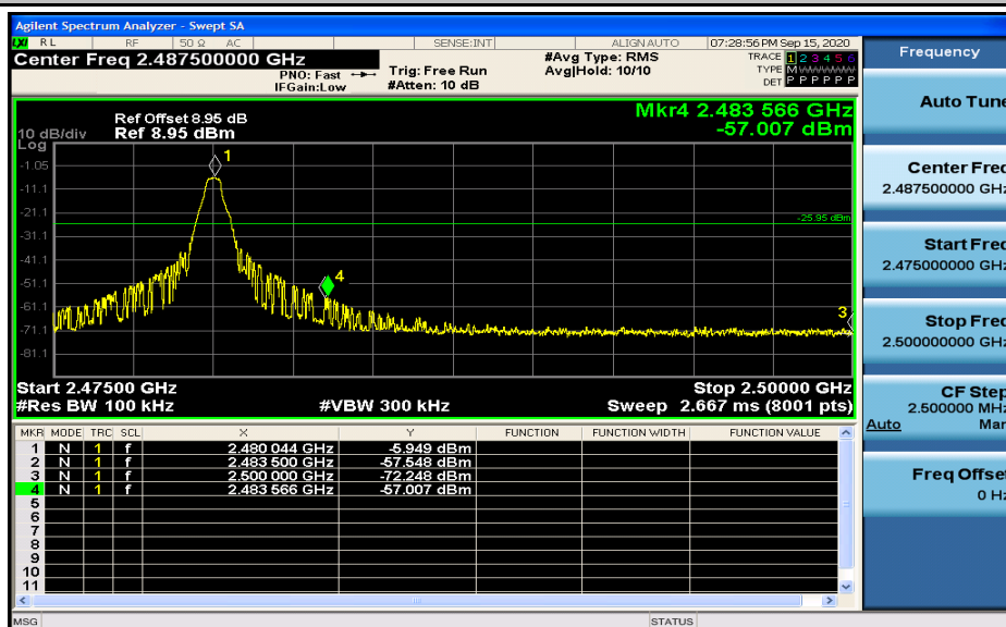
Band-edge for RF Conducted Emissions_BLE_2480_Ant1
