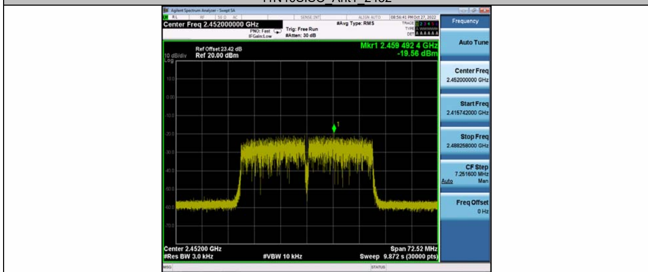
11N40SISO Ant1_2452
