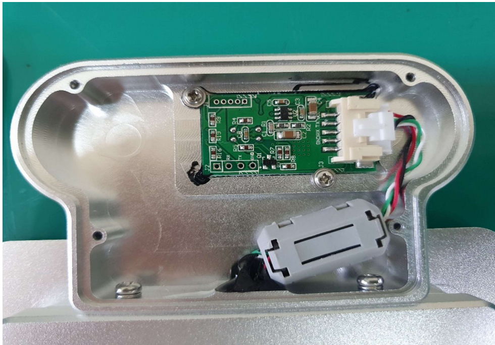
Inside of Camera board
