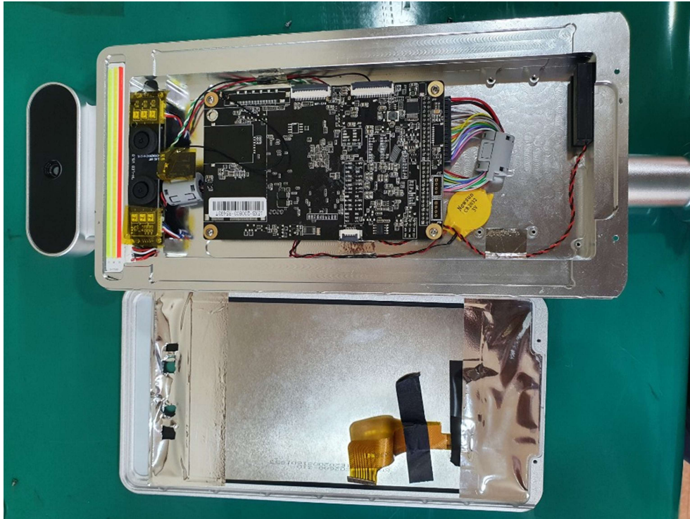
Inside of Camera board
