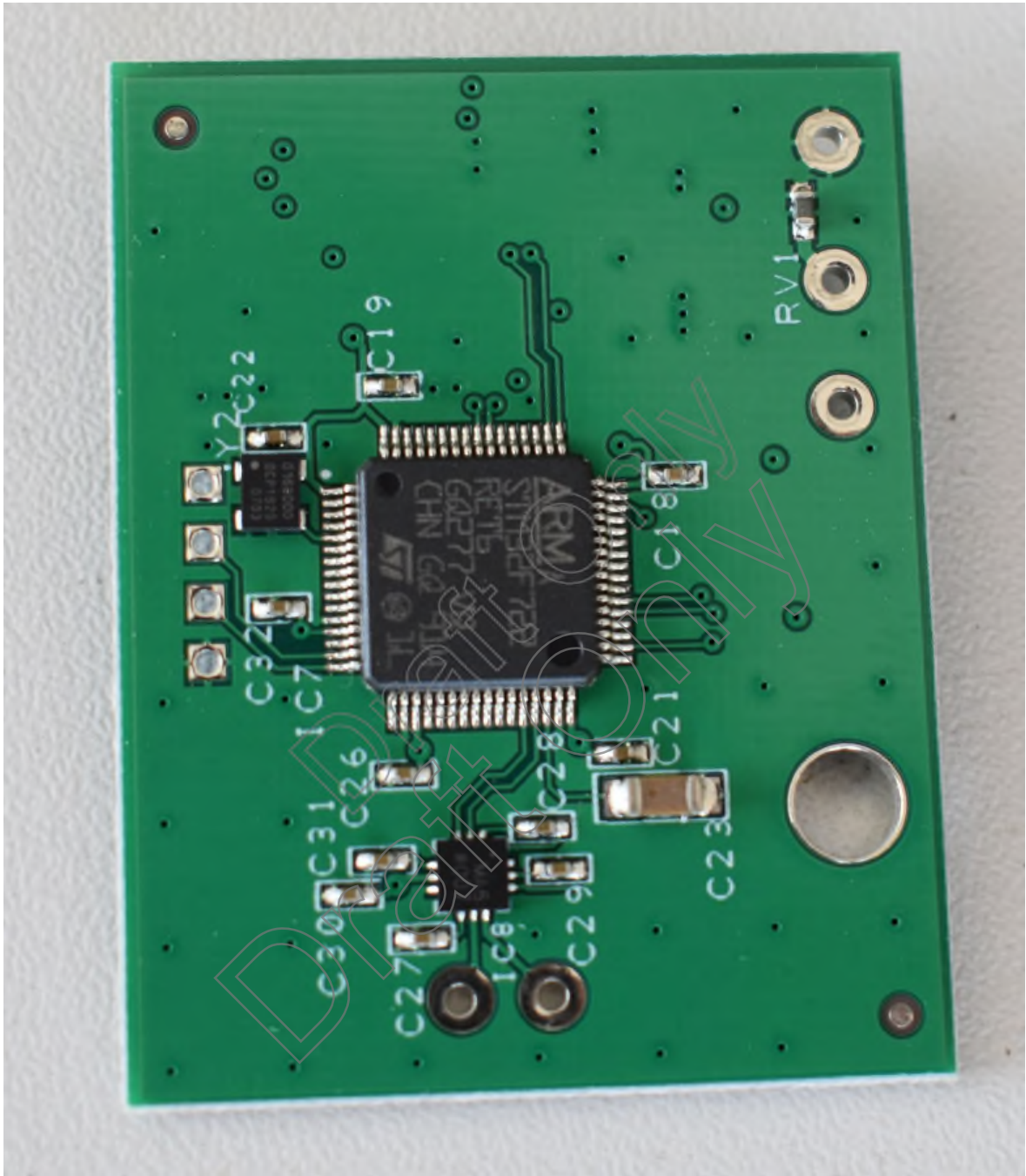
Main PCB (front) with MCU
