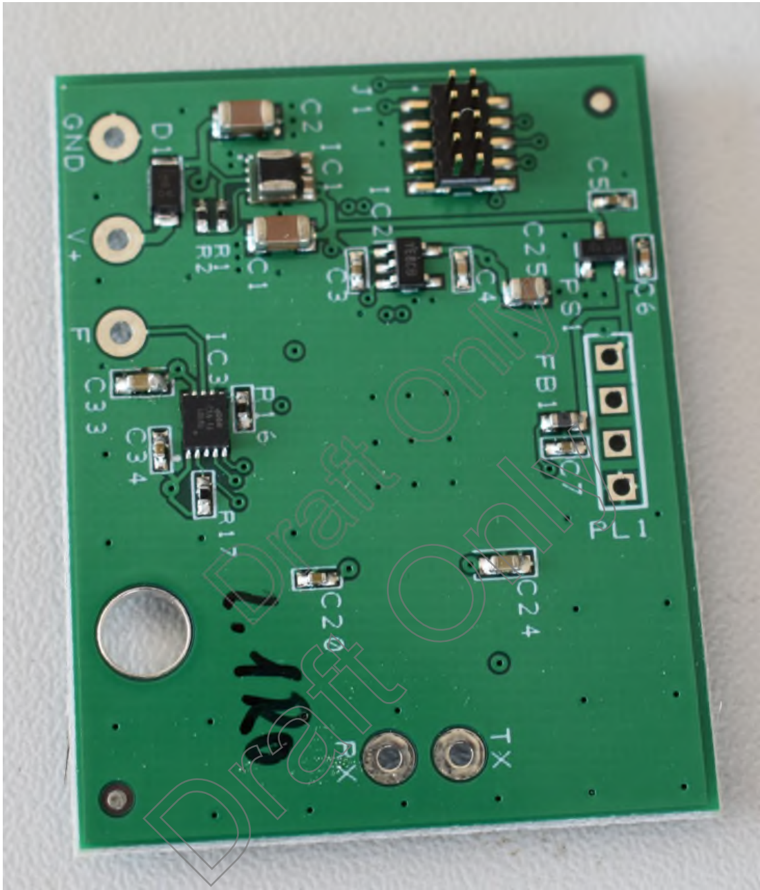
Main PCB (back)
