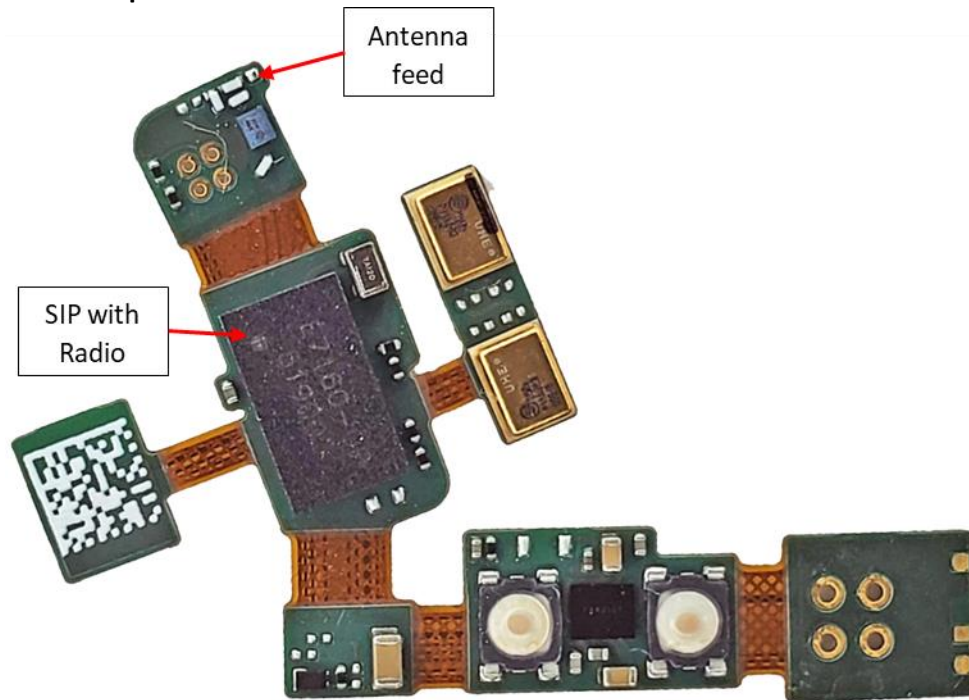
Uncoated PCBA – Top View
