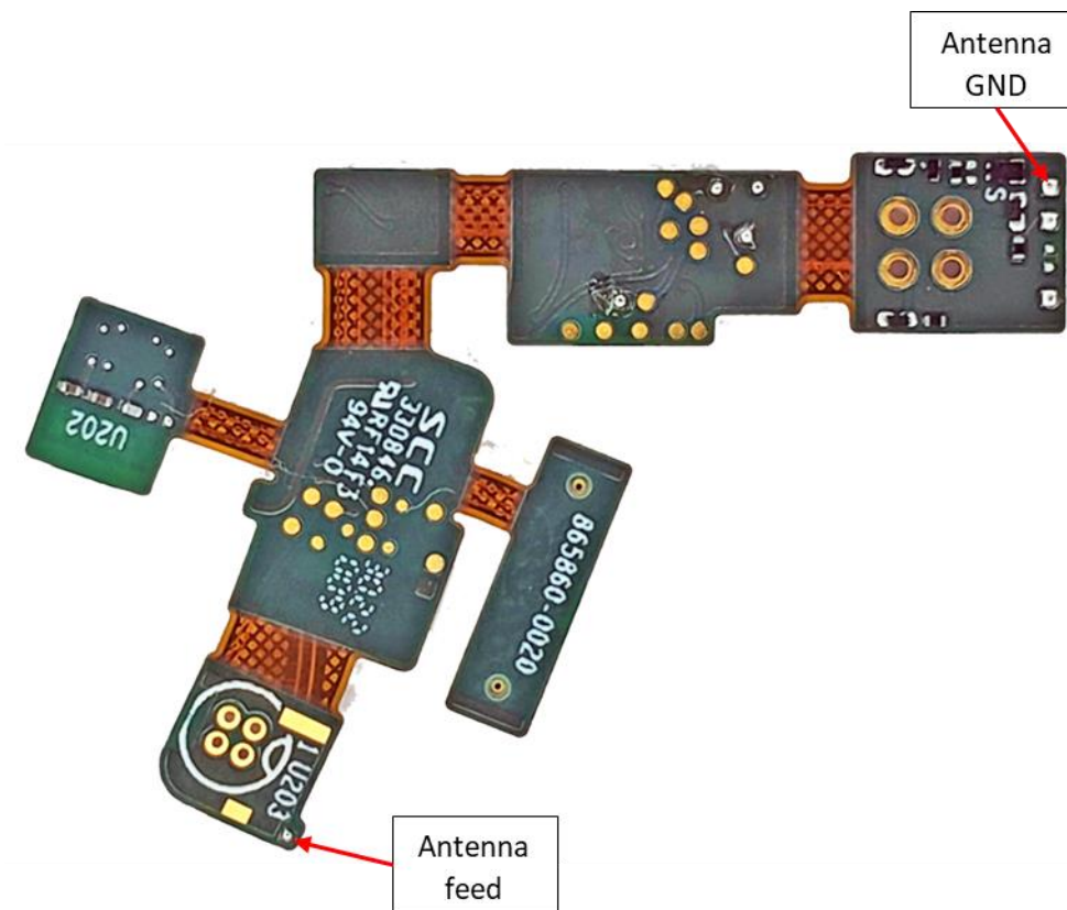
Uncoated PCBA – Bottom View
