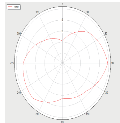
BLUETOOTH_Trp_V78 Total
