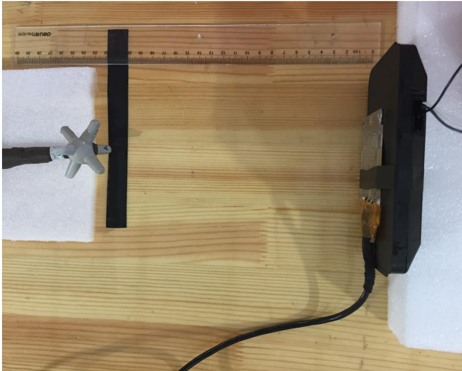
E-field Test Setup Photo Positon E Load (20cm)
