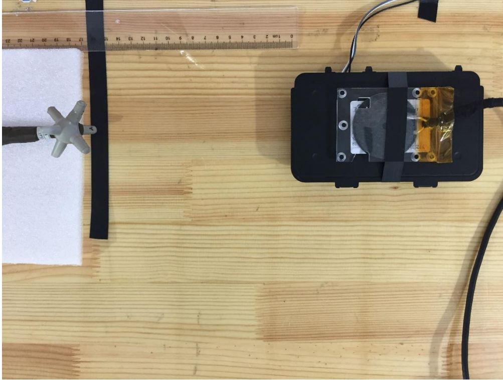
E-field Test Setup Photo Positon A Load (15cm)
