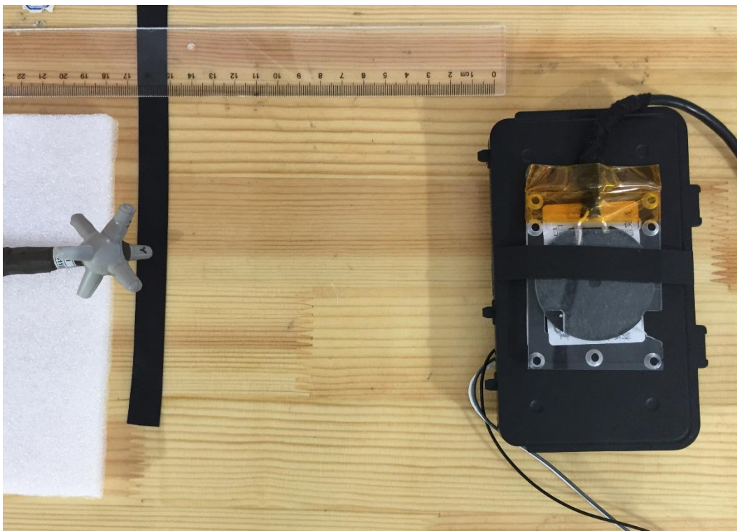
E-field Test Setup Photo Positon B Load (15cm)
