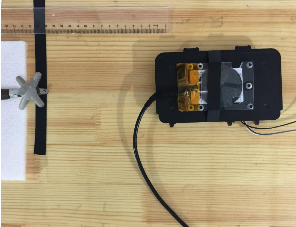
E-field Test Setup Photo Positon C Load (15cm)
