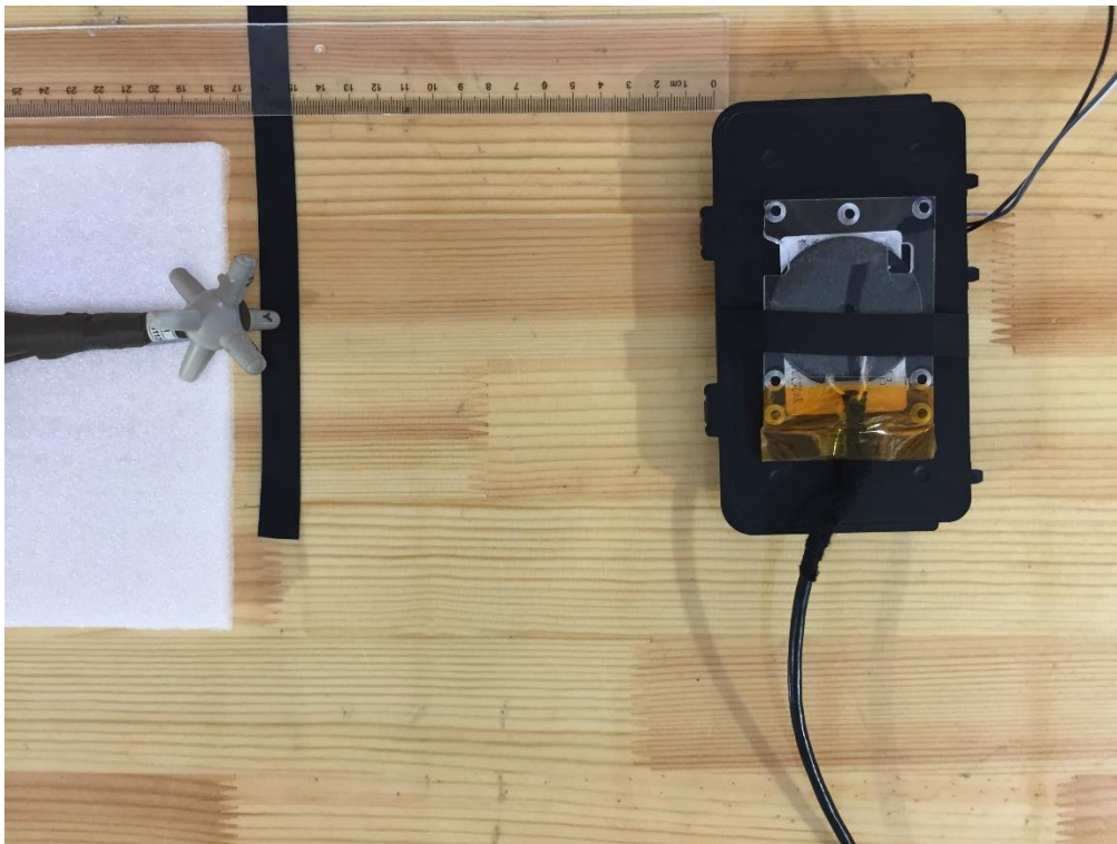
E-field Test Setup Photo Positon D Load (15cm)
