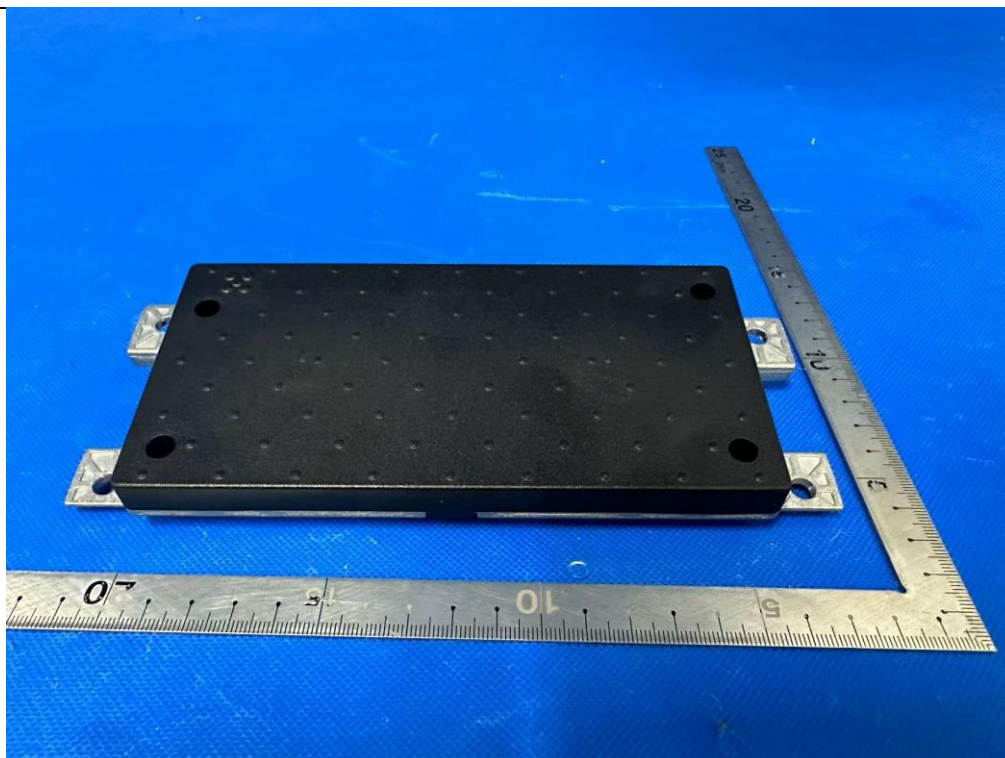
(2) EUT Photo(WPC013)
