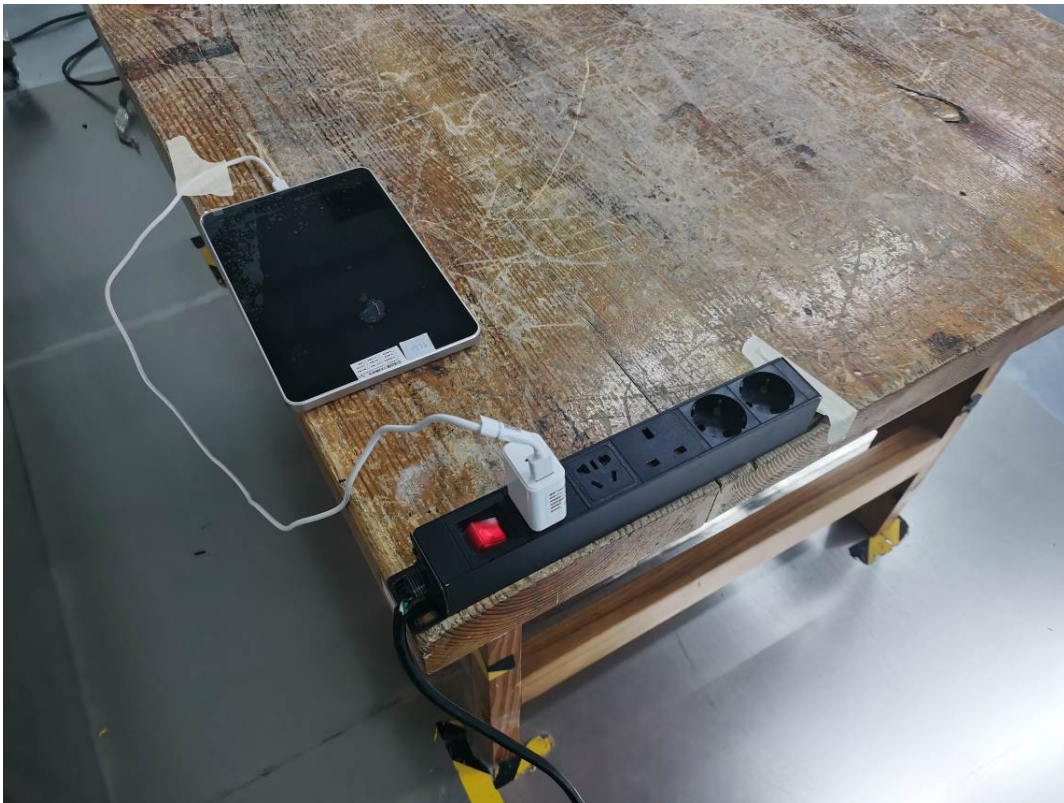
Conducted Emissions Side View #1
