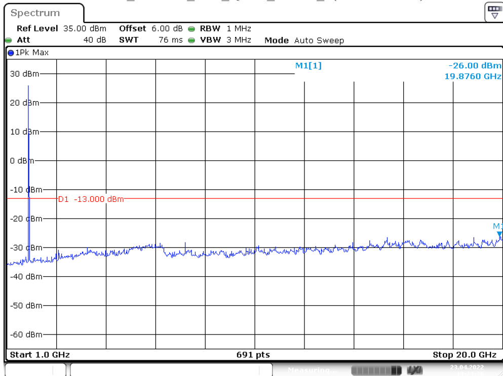
Band 2 1.4 MHz Low QPSK RB6#0 2(1GHz-20GHz)
