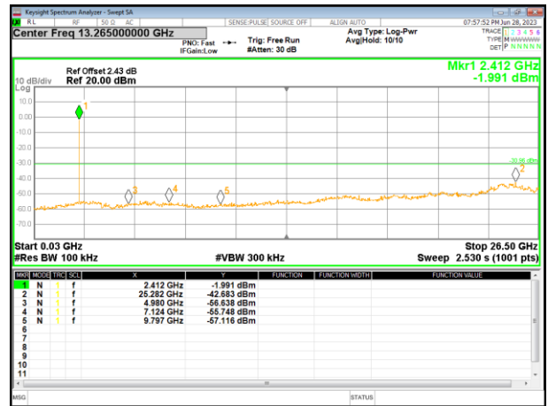
30MHz~26.5GHz
