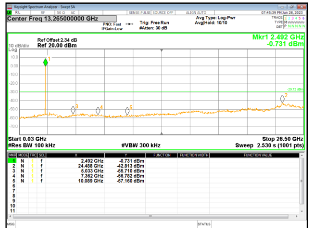
30MHz~26.5GHz
