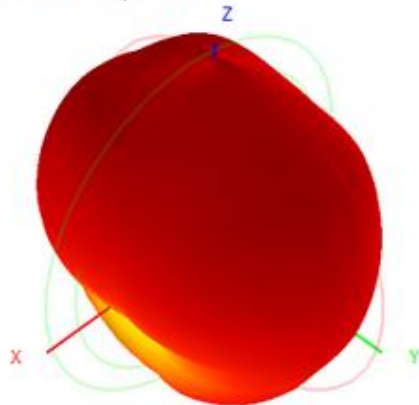
2450.0MHz H+V, Eff: 65.7%
