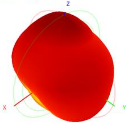
2400.0MHz H+V, Eff: 67.2%
