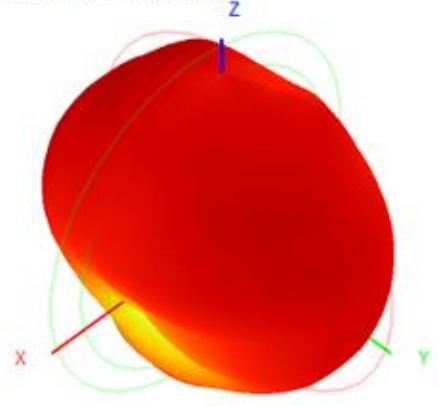
2500.0MHz H+V, Eff: 70.7%
