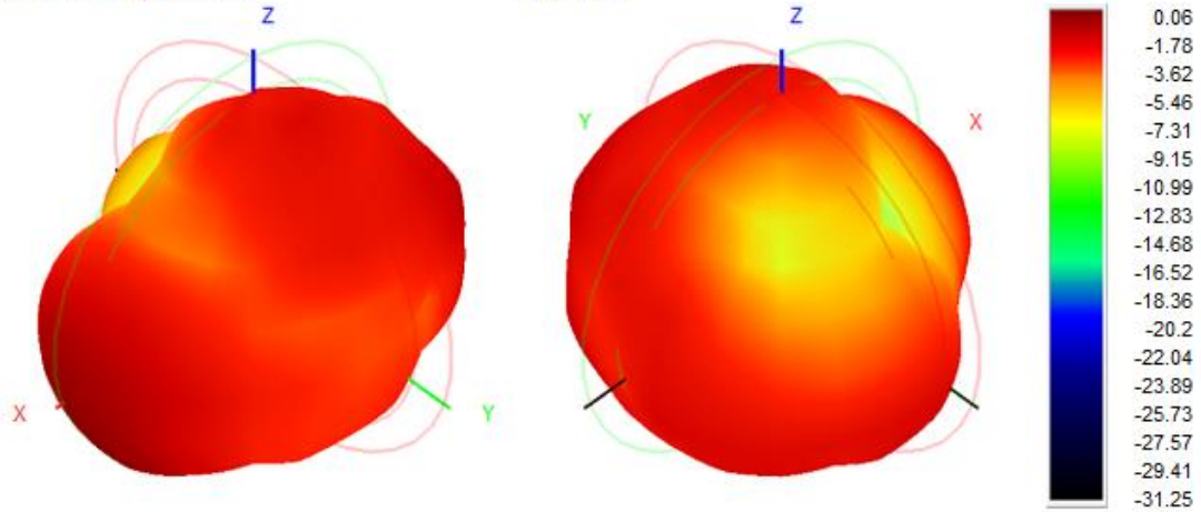
2500.0MHz H+V, Eff: 32.3%
