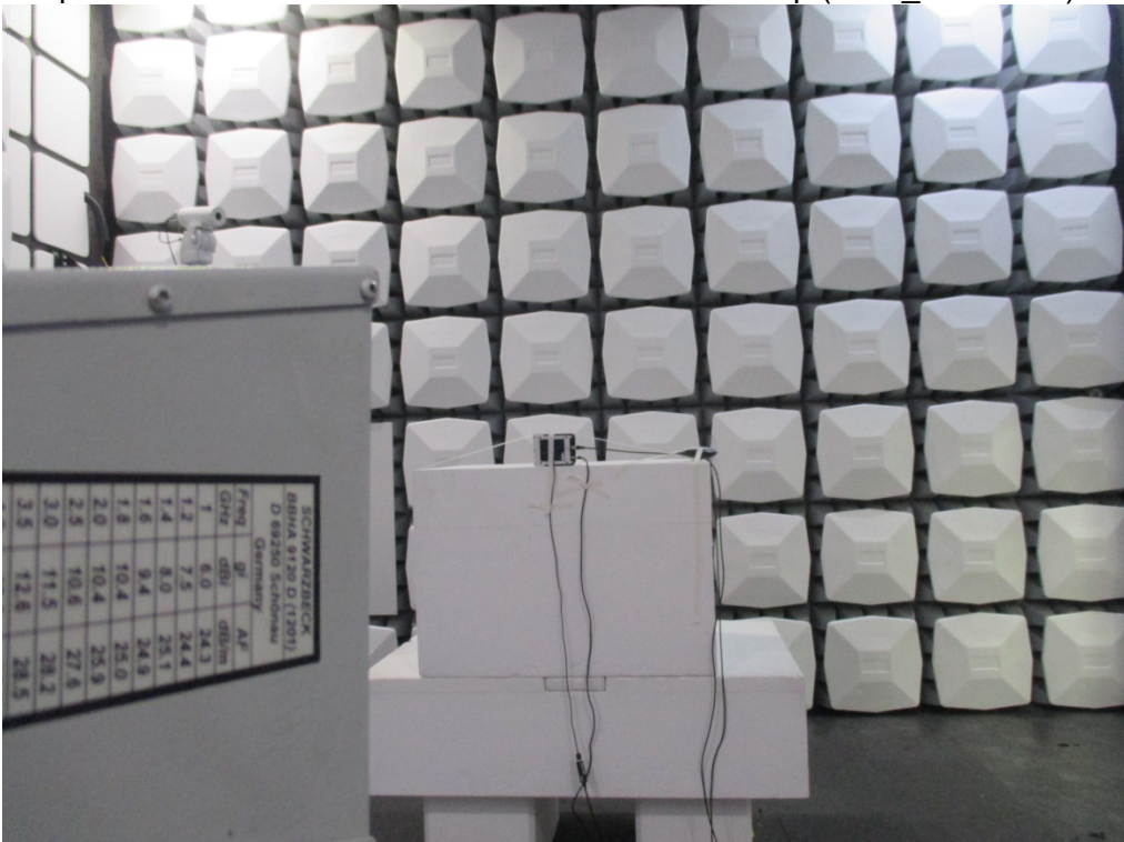
Description: Back View of Radiated Emission Test Setup (Horn_Above 1G)
