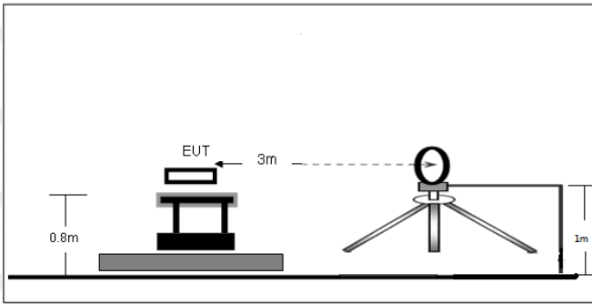
Figure 1. Below 30MHz
