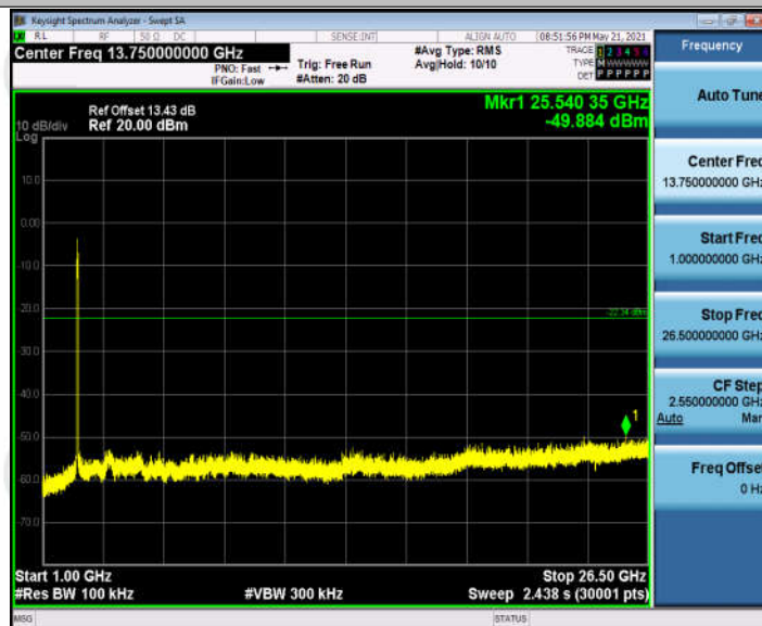
11N40SISO_Ant1_2462_1000~26500
