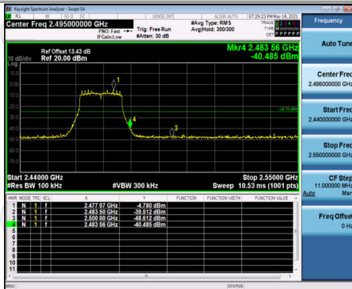
11G_Ant1_High_2472
