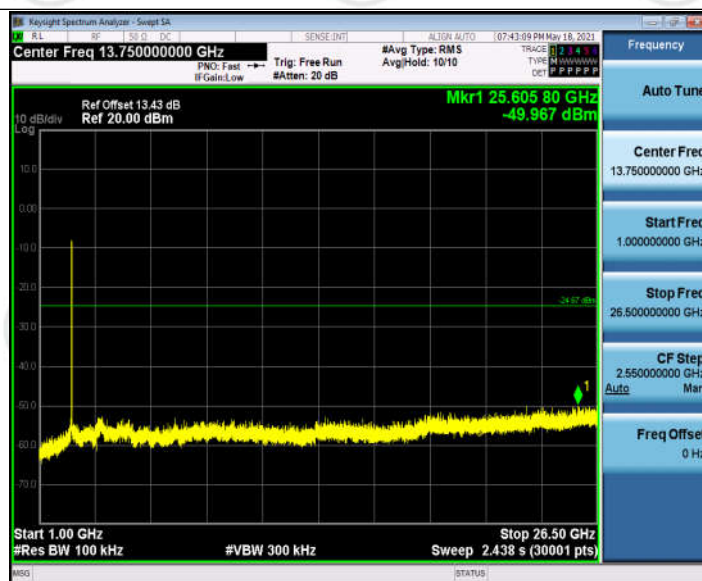
11N20SISO_Ant1_2472_1000~26500
