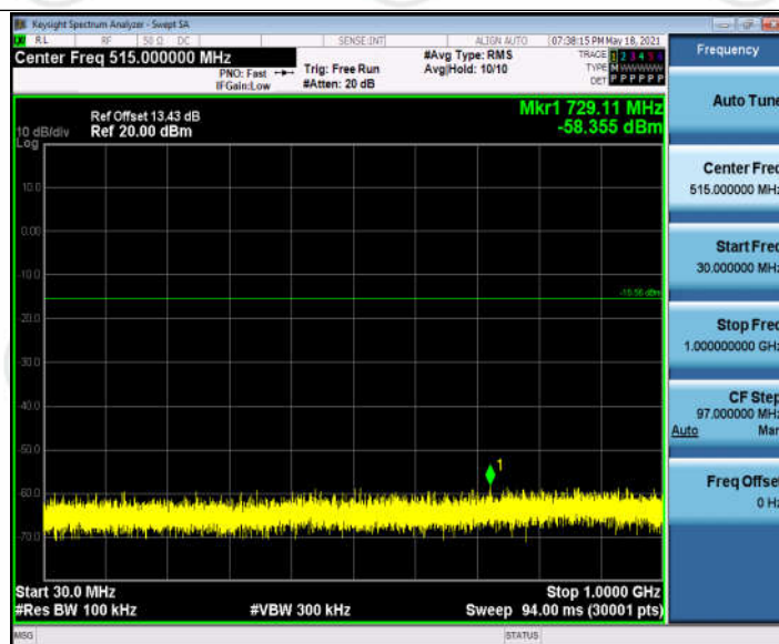
11N20SISO_Ant1_2442_30~1000
