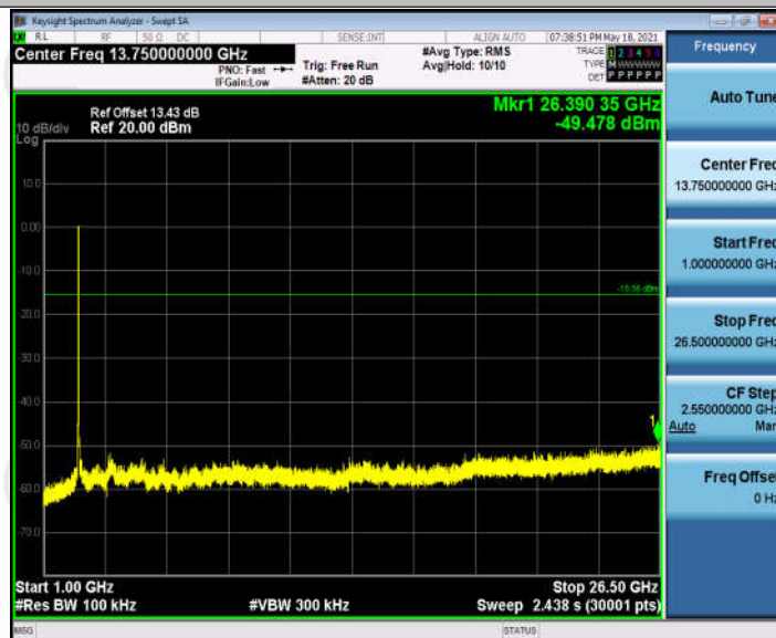
11N20SISO_Ant1_2442_1000~26500
