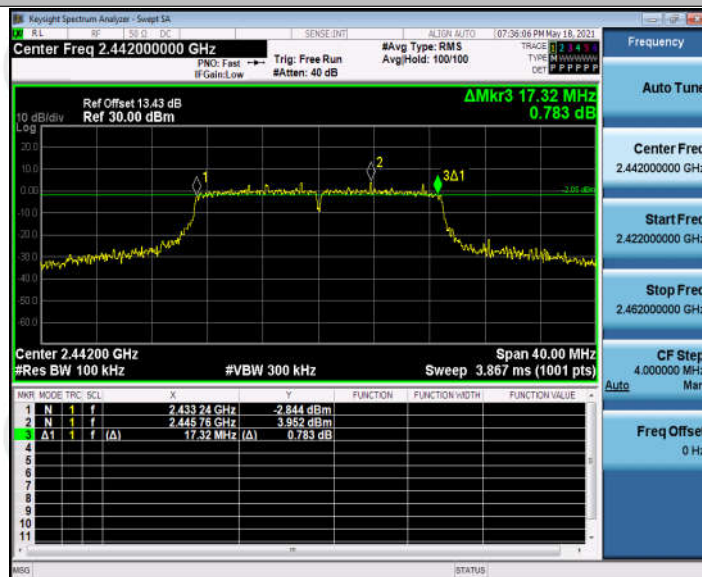
11N20SISO_Ant1_2442
