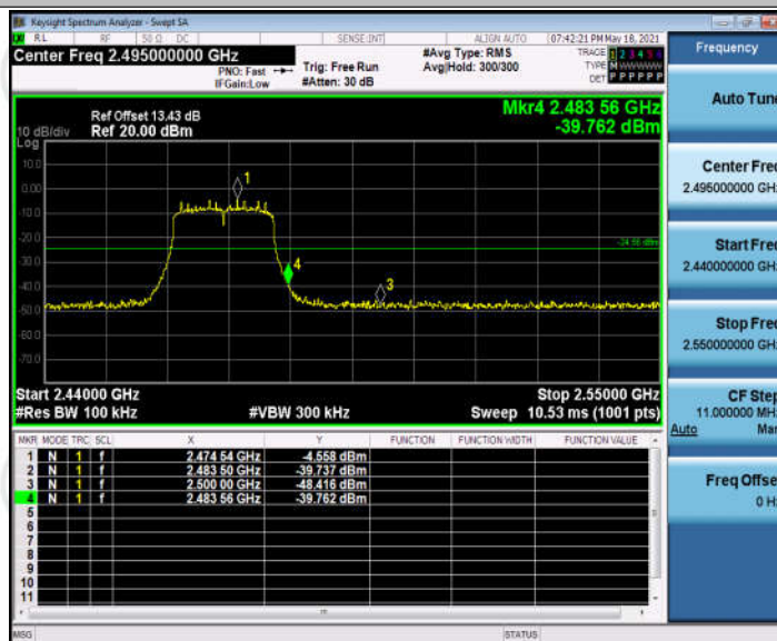
11N20SISO_Ant1_High_2472
