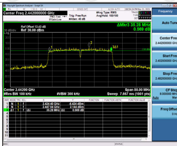
11N40SISO_Ant1_2442
