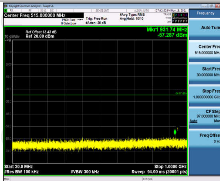
11N20SISO_Ant1_2472_30~1000
