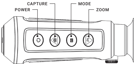
FIGURE 2-2. CONTROL BUTTONS
