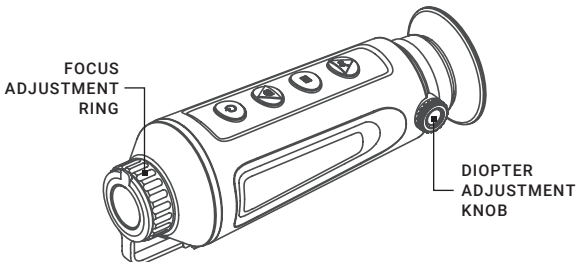
FIGURE 2-4. DIOPTER AND FOCUS ADJUSTMENT
