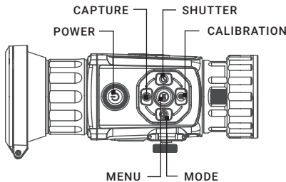
FIGURE 2-3. CONTROL BUTTONS
