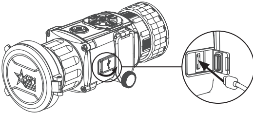
FIGURE 2-2. CABLE INTERFACE
