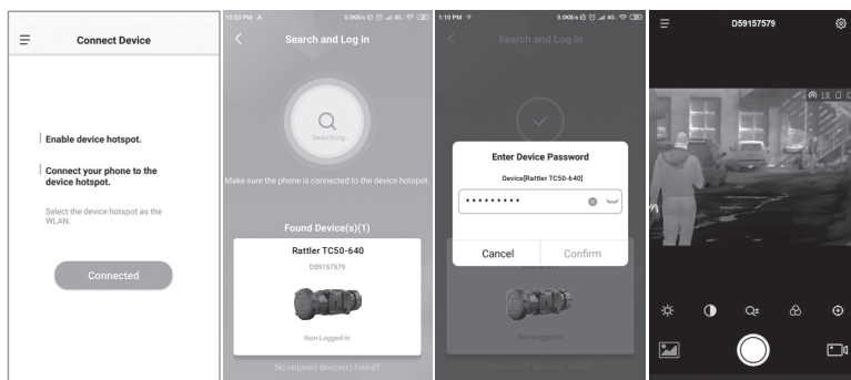
FIGURE 2-14. CLIENT SOFTWARE
