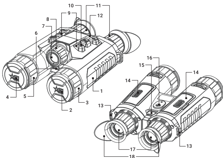
FIGURE 1-1. MAIN PARTS
