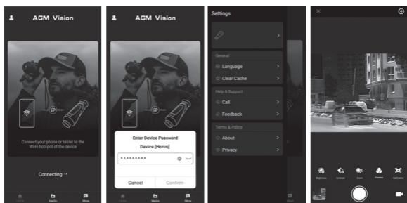
FIGURE 2-11. CLIENT SOFTWARE
