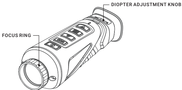
FIGURE 2-4. DIOPTRER ADJUSTMENT KNOB AND FOCUS RING
