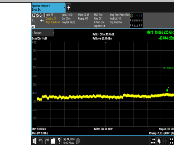
Band66_20MHz_16QAM_132572_1RB#0_3000-20000_3000-20000
