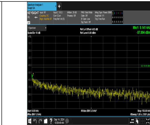
Band66_20MHz_16QAM_132322_100RB#0_0.009~0.15_0.009~0.15
