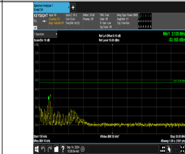
Band66_20MHz_QPSK_132322_100RB#0_0.15~30_0.15~30
