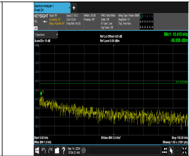
Band66_20MHz_16QAM_132072_100RB#0_0.009~0.15_0.009~0.15
