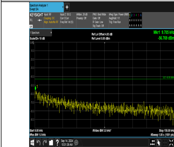
Band66_20MHz_QPSK_132072_1RB#99_0.009~0.15_0.009~0.15
