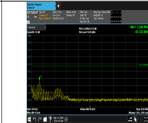
Band66_20MHz_QPSK_132072_1RB#99_0.15~30_0.15~30
