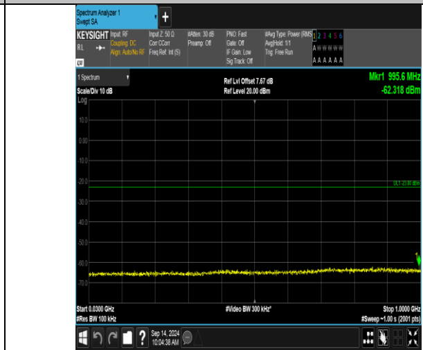
Band66_20MHz_16QAM_132072_100RB#0_30~1000_30~1000
