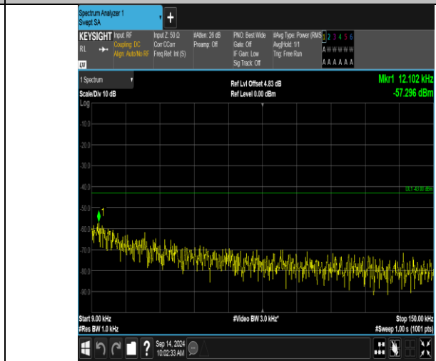
Band66_20MHz_16QAM_132072_1RB#99_0.009~0.15_0.009~0.15
