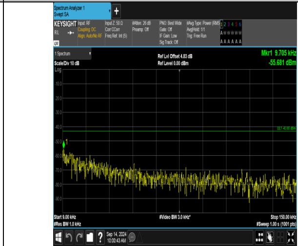
Band66_20MHz_16QAM_132072_1RB#0_0.009~0.15_0.009~0.15
