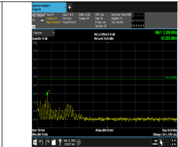
Band66_20MHz_QPSK_132072_1RB#0_0.15~30_0.15~30
