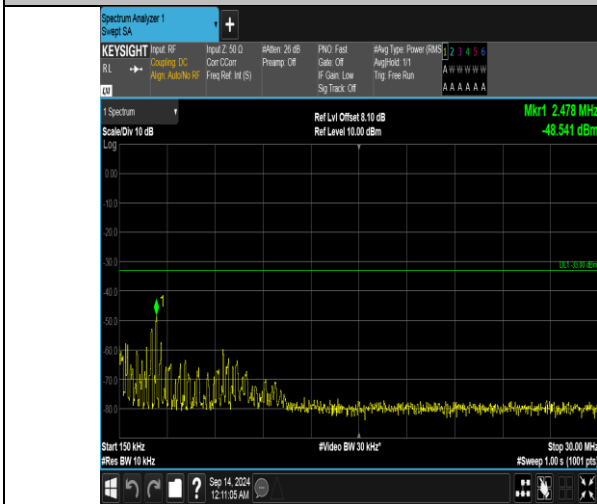
Band66_15MHz_16QAM_132597_75RB#0_0.15~30_0.15~30
