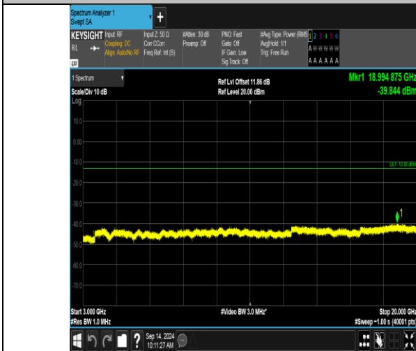
Band66_20MHz_QPSK_132572_1RB#0_3000~20000_3000~20000
