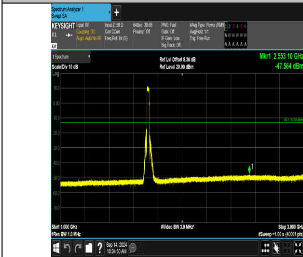
Band66_20MHz_16QAM_132072_100RB#0_1000~3000_1000~3000
