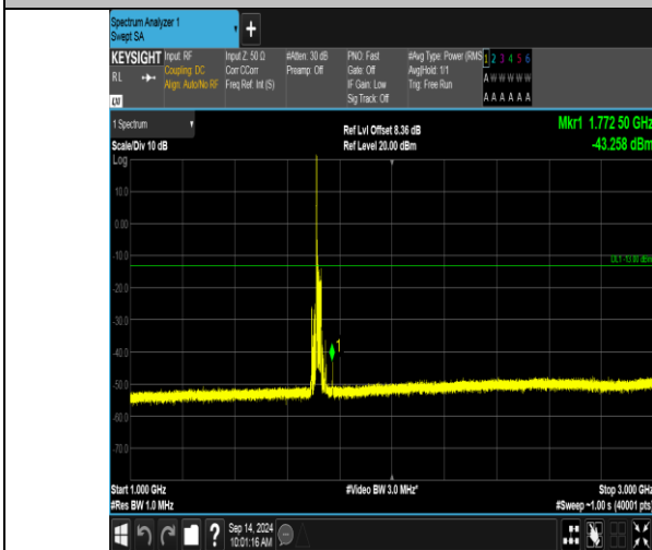
Band66_20MHz_16QAM_132072_1RB#0_1000~3000_1000~3000
