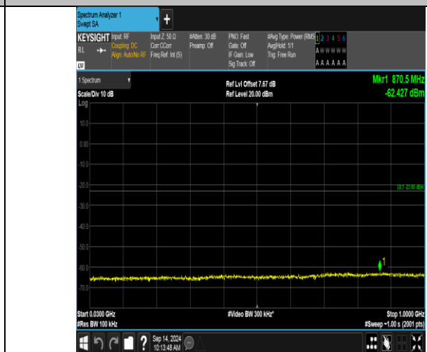
Band66_20MHz_16QAM_132572_1RB#99_30~1000_30~1000
