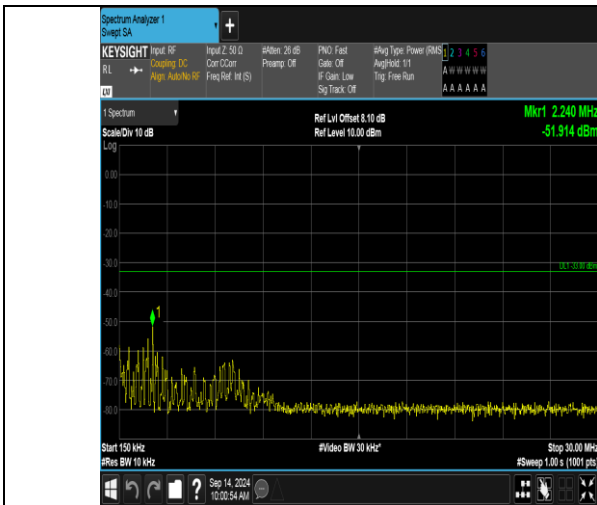
Band66_20MHz_16QAM_132072_1RB#0_0.15~30_0.15~30
