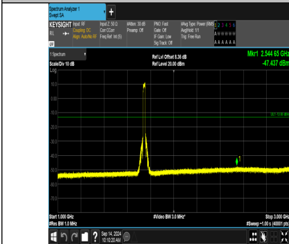
Band66_20MHz_16QAM_132322_100RB#0_1000~3000_1000~3000
