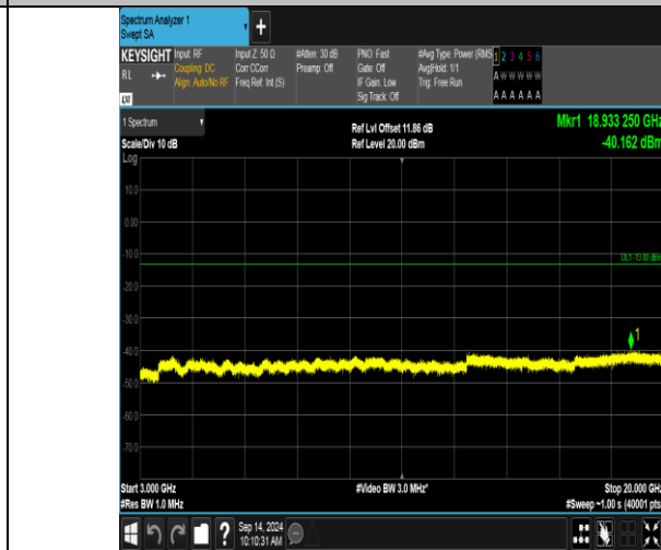
Band66_20MHz_16QAM_132322_100RB#0_3000~20000_3000~20000
