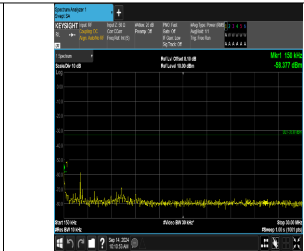
Band66_20MHz_QPSK_132572_1RB#0_0.15~30_0.15~30
