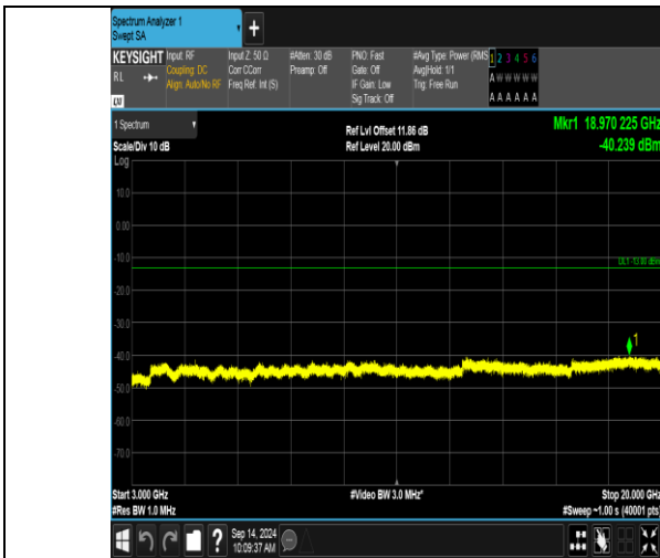
Band66_20MHz_QPSK_132322_100RB#0_3000~20000_3000~20000
