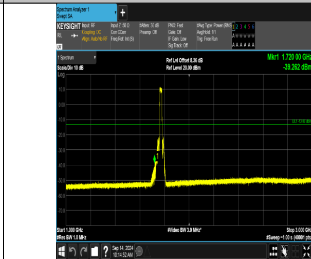
Band66_20MHz_QPSK_132572_100RB#0_1000~3000_1000~3000
