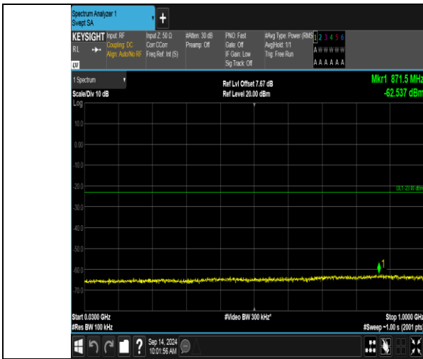
Band66_20MHz_QPSK_132072_1RB#99_30~1000_30~1000
