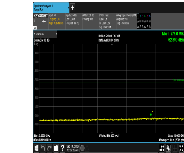
Band66_20MHz_16QAM_132322_1RB#0_30~1000_30~1000
