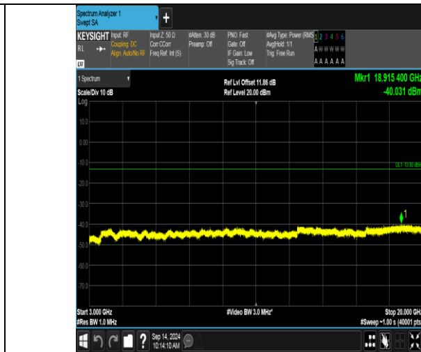
Band66_20MHz_16QAM_132572_1RB#99_3000~20000_3000~20000
