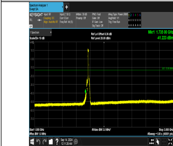
Band66_15MHz_16QAM_132597_75RB#0_1000~3000_1000~3000
