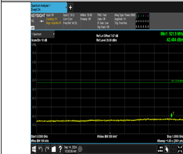
Band66_20MHz_QPSK_132072_1RB#0_30~1000_30~1000
