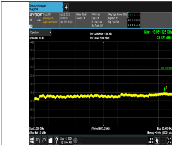
Band66_15MHz_QPSK_132597_75RB#0_3000~20000_3000~20000
