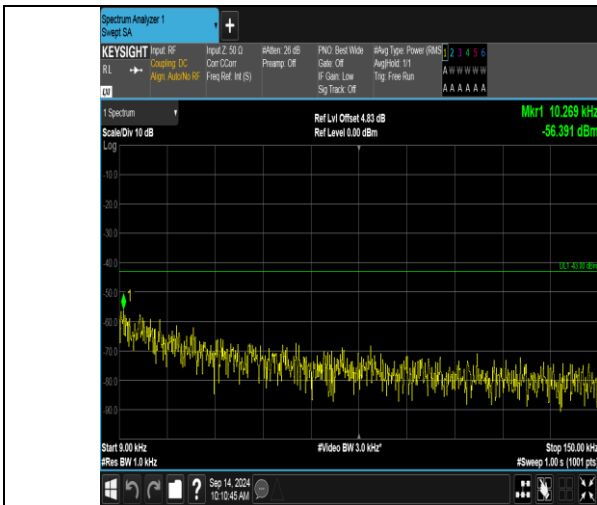
Band66_20MHz_QPSK_132572_1RB#0_0.009~0.15_0.009~0.15
