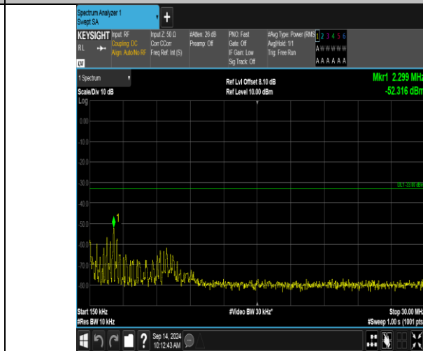
Band66_20MHz_QPSK_132572_1RB#99_0.15-30_0.15-30
