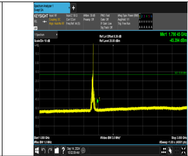
Band66_20MHz_QPSK_132072_1RB#99_1000~3000_1000~3000
