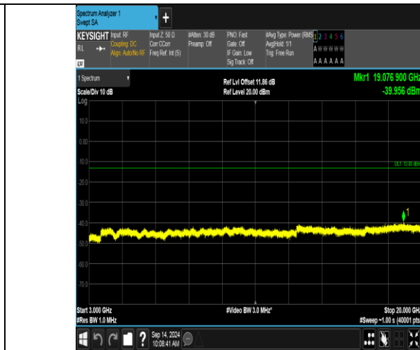
Band66_20MHz_16QAM_132322_1RB#99_3000~20000_3000~20000
