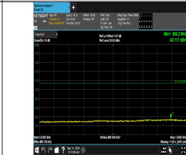
Band66_20MHz_16QAM_132322_100RB#0_30~1000_30~1000
