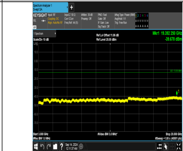
Band66_15MHz_16QAM_132597_75RB#0_3000~20000_3000~20000
