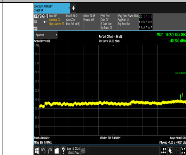
Band66_20MHz_16QAM_132072_1RB#0_3000~20000_3000~20000
