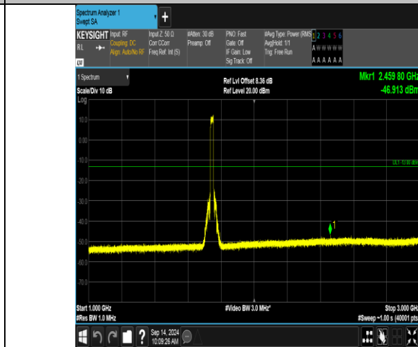
Band66_20MHz_QPSK_132322_100RB#0_1000~3000_1000~3000
