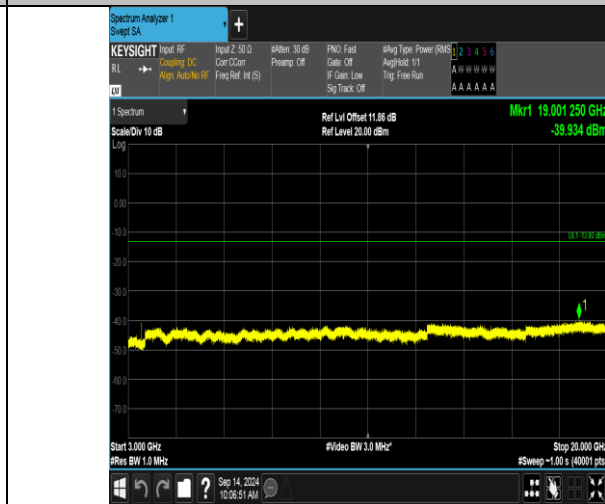
Band66_20MHz_16QAM_132322_1RB#0_3000~20000_3000~20000
