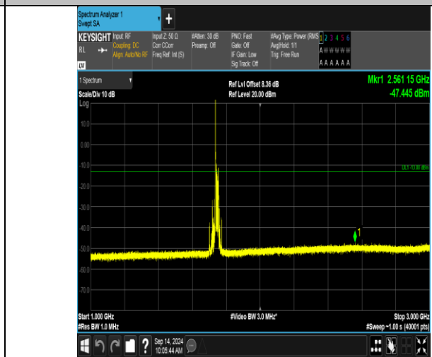
Band66_20MHz_QPSK_132322_1RB#0_1000~3000_1000~3000
