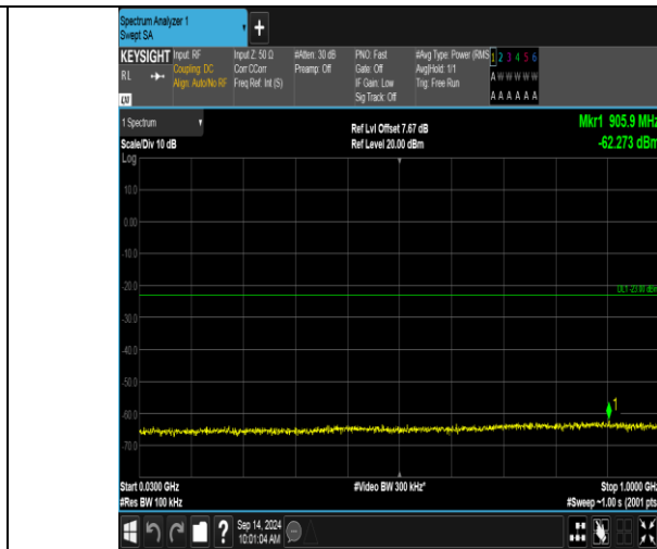
Band66_20MHz_16QAM_132072_1RB#0_30~1000_30~1000
