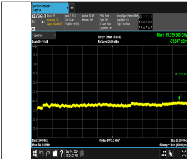
Band66_20MHz_QPSK_132072_100RB#0_3000~20000_3000~20000
