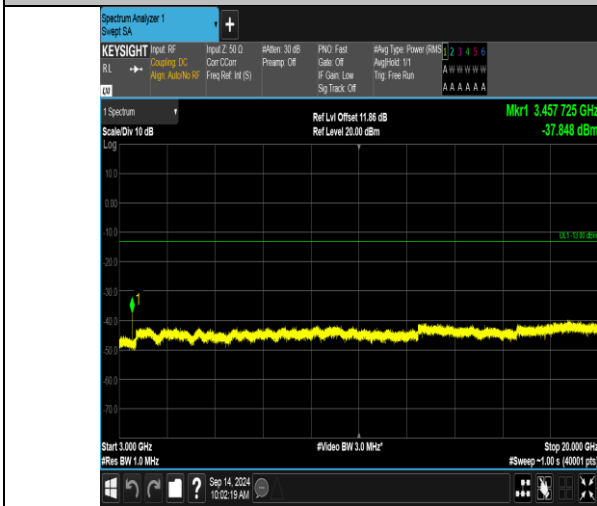
Band66_20MHz_QPSK_132072_1RB#99_3000~20000_3000~20000
