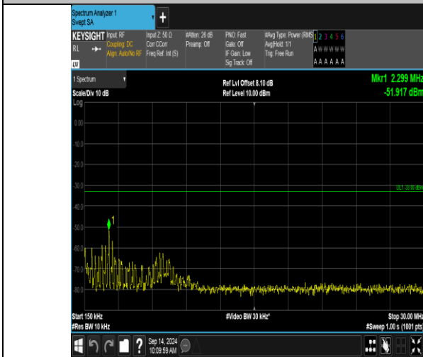
Band66_20MHz_16QAM_132322_100RB#0_0.15~30_0.15~30
