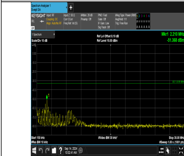
Band66_20MHz_16QAM_132072_1RB#99_0.15~30_0.15~30
