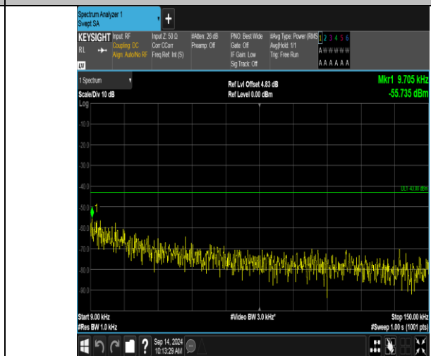
Band66_20MHz_16QAM_132572_1RB#99_0.009~0.15_0.009~0.15
