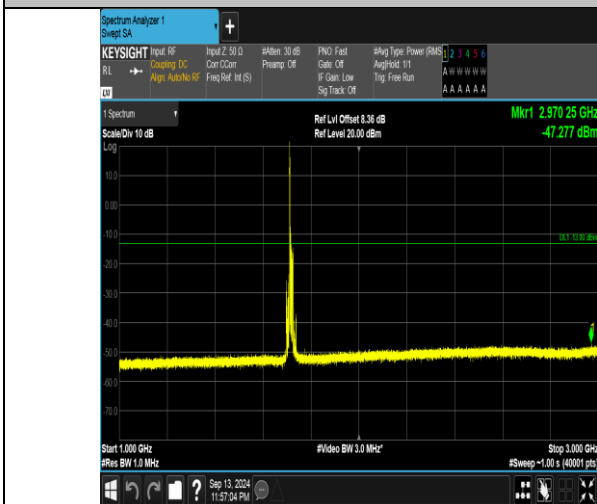
Band66_15MHz_16QAM_132047_1RB#0_1000~3000_1000~3000
