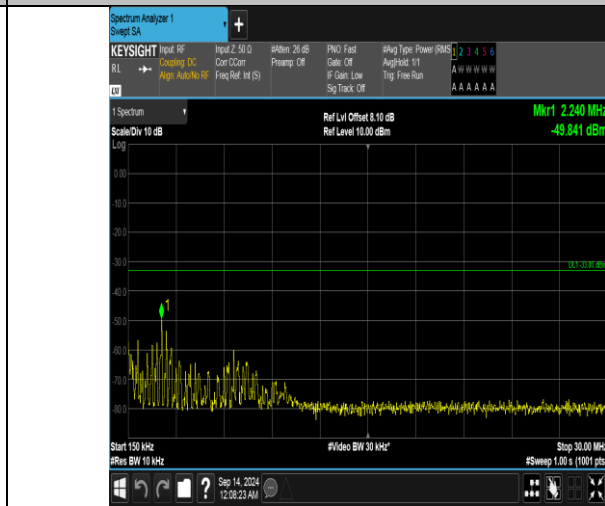
Band66_15MHz_QPSK_132597_1RB#74_0.15-30_0.15-30
