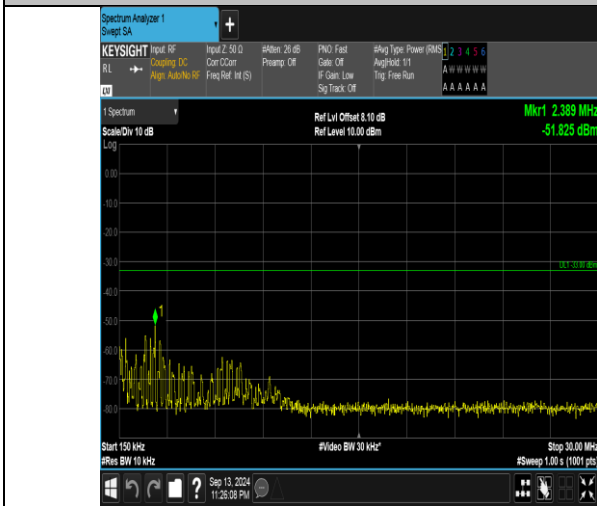
Band66_10MHz_16QAM_132622_50RB#0_0.15~30_0.15~30
