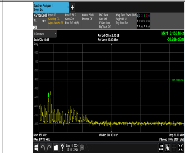
Band66_15MHz_QPSK_132597_75RB#0_0.15~30_0.15~30
