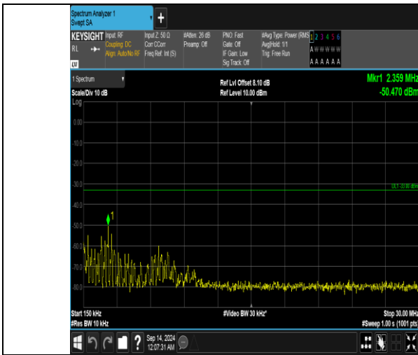
Band66_15MHz_16QAM_132597_1RB#0_0.15-30_0.15-30
