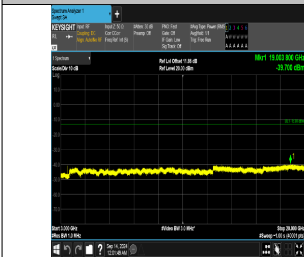
Band66_15MHz_QPSK_132322_1RB#0_3000~20000_3000~20000
