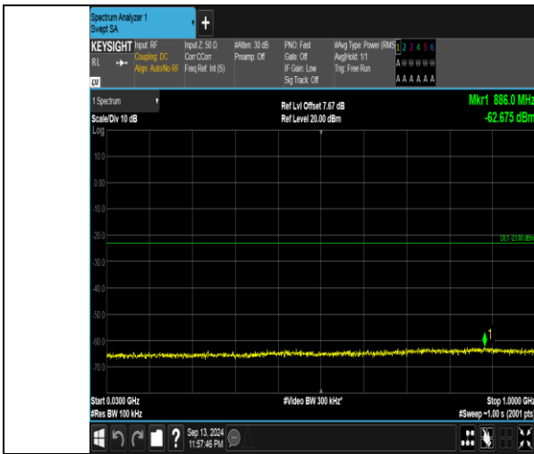
Band66_15MHz_QPSK_132047_1RB#74_30~1000_30~1000
