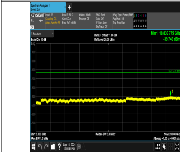
Band66_15MHz_QPSK_132597_1RB#74_3000~20000_3000~20000
