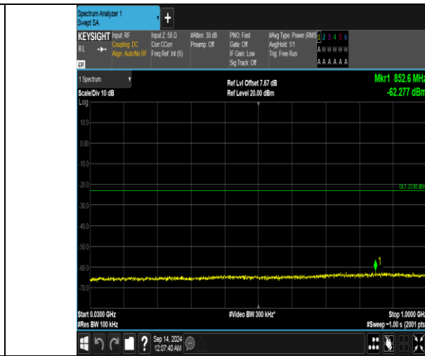
Band66_15MHz_16QAM_132597_1RB#0_30-1000_30-1000
