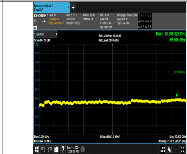
Band66_15MHz_16QAM_132322_75RB#0_3000~20000_3000~20000
