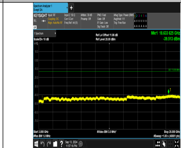
Band66_15MHz_16QAM_132047_1RB#0_3000~20000_3000~20000
