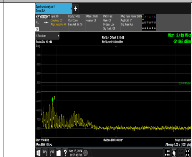
Band66_15MHz_QPSK_132047_1RB#74_0.15~30_0.15~30
