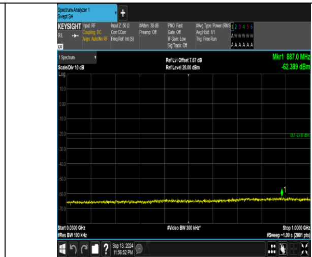
Band66_15MHz_16QAM_132047_1RB#0_30~1000_30~1000
