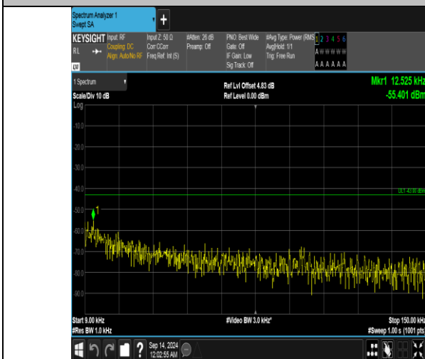
Band66_15MHz_QPSK_132322_1RB#74_0.009~0.15_0.009~0.15
