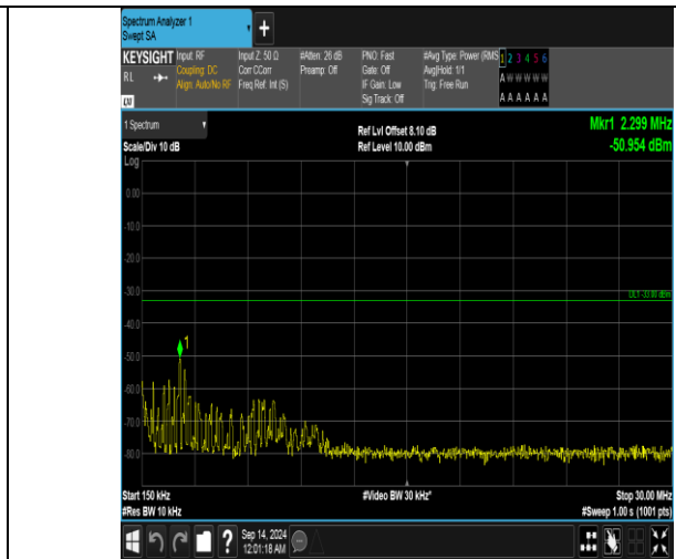
Band66_15MHz_QPSK_132322_1RB#0_0.15~30_0.15~30
