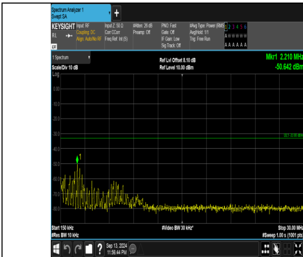
Band66_15MHz_16QAM_132047_1RB#0_0.15~30_0.15~30
