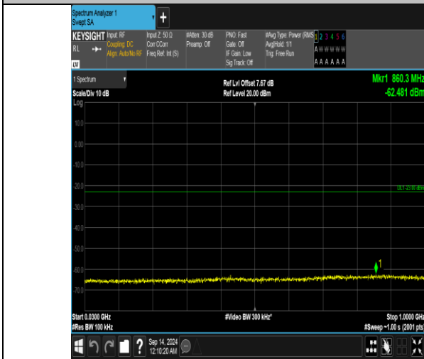
Band66_15MHz_QPSK_132597_75RB#0_30~1000_30~1000
