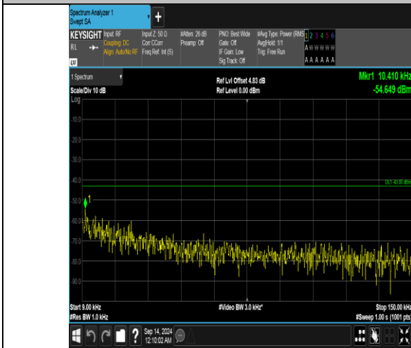
Band66_15MHz_QPSK_132597_75RB#0_0.009~0.15_0.009~0.15
