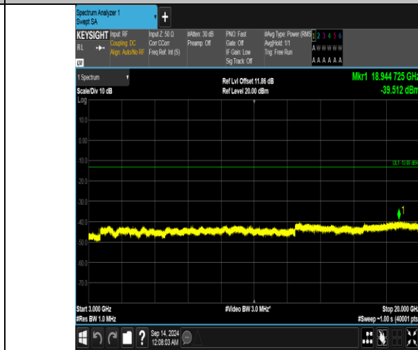
Band66_15MHz_16QAM_132597_1RB#0_3000-20000_3000-20000
