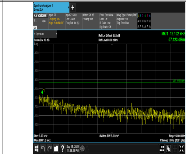
Band66_15MHz_16QAM_132047_1RB#74_0.009~0.15_0.009~0.15
