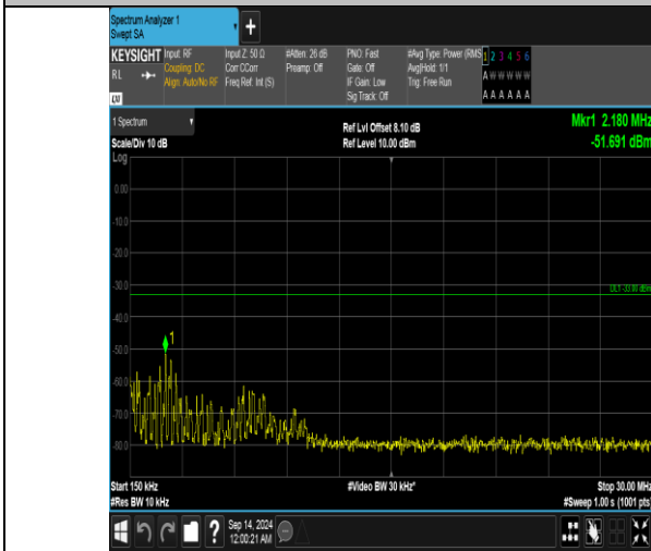
Band66_15MHz_16QAM_132047_75RB#0_0.15~30_0.15~30
