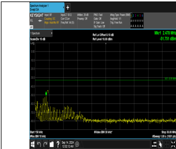
Band66_15MHz_16QAM_132322_1RB#0_0.15~30_0.15~30
