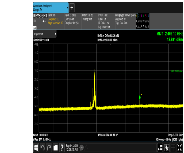
Band66_15MHz_QPSK_132597_1RB#74_1000~3000_1000~3000
