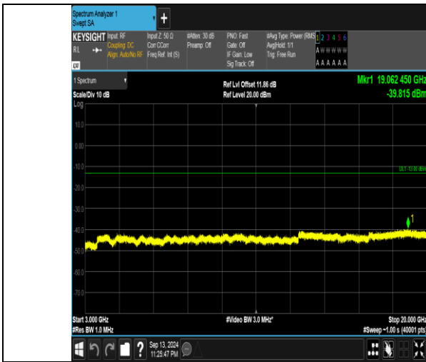
Band66_10MHz_QPSK_132622_50RB#0_3000~20000_3000~20000
