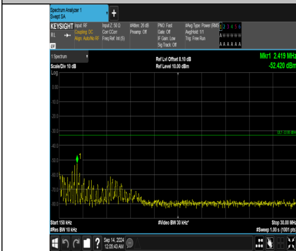
Band66_15MHz_16QAM_132322_75RB#0_0.15~30_0.15~30
