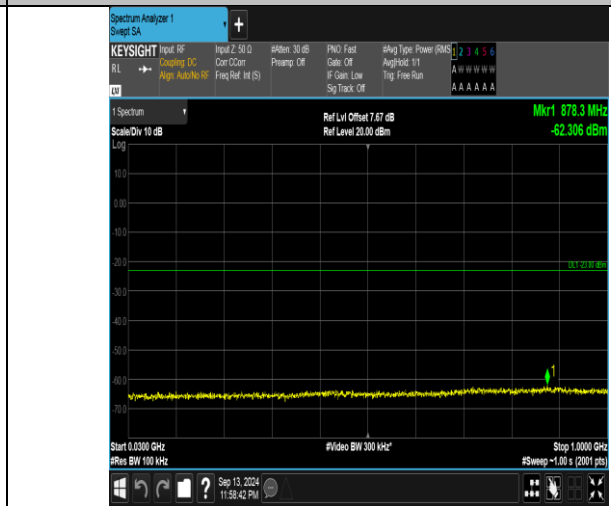
Band66_15MHz_16QAM_132047_1RB#74_30~1000_30~1000
