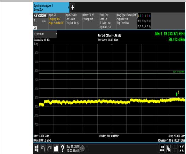
Band66_15MHz_16QAM_132047_75RB#0_3000~20000_3000~20000
