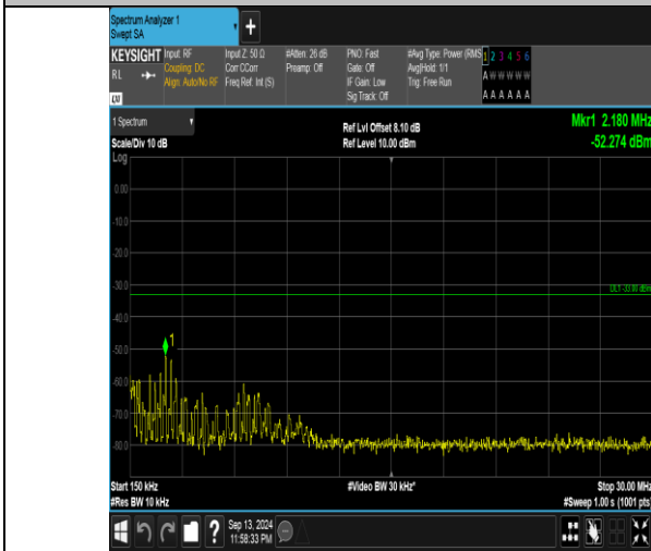
Band66_15MHz_16QAM_132047_1RB#74_0.15~30_0.15~30
