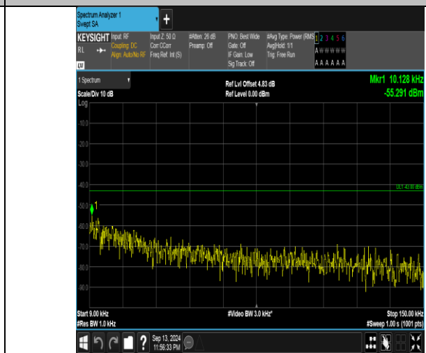
Band66_15MHz_16QAM_132047_1RB#0_0.009~0.15_0.009~0.15
