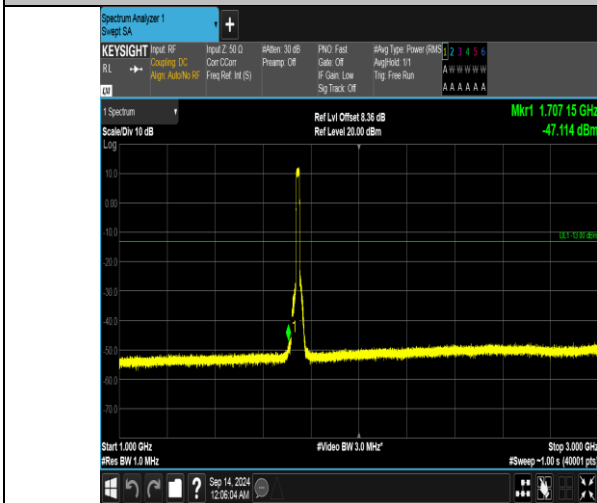
Band66_15MHz_16QAM_132322_75RB#0_1000~3000_1000~3000
