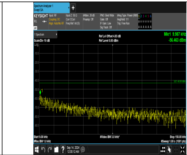
Band66_15MHz_16QAM_132047_75RB#0_0.009~0.15_0.009~0.15
