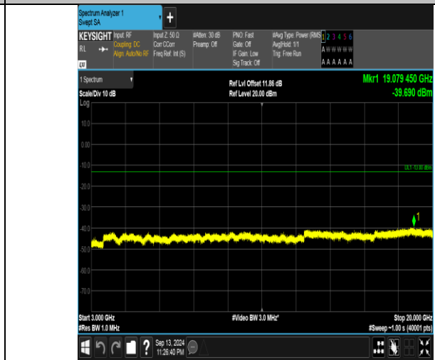
Band66_10MHz_16QAM_132622_50RB#0_3000~20000_3000~20000
