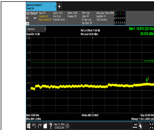
Band66_15MHz_QPSK_132322_75RB#0_3000~20000_3000~20000
