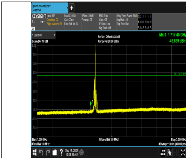
Band66_15MHz_16QAM_132597_1RB#74_1000~3000_1000~3000
