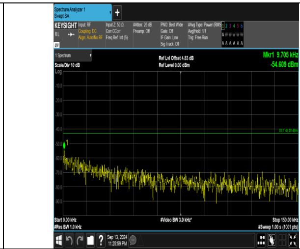
Band66_10MHz_16QAM_132622_50RB#0_0.009~0.15_0.009~0.15
