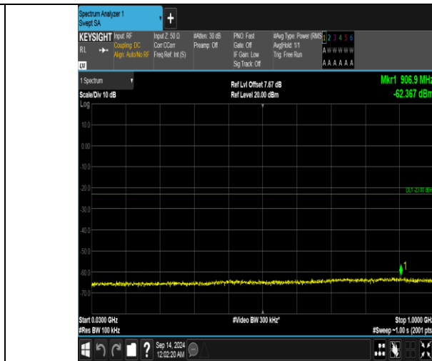
Band66_15MHz_16QAM_132322_1RB#0_30~1000_30~1000
