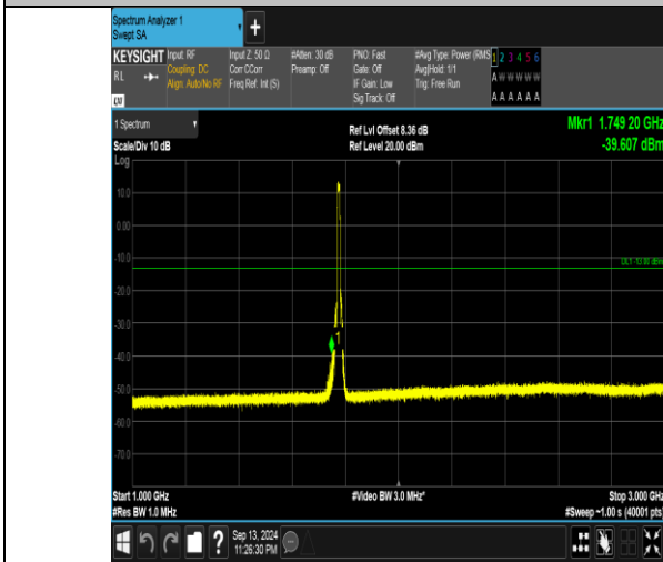
Band66_10MHz_16QAM_132622_50RB#0_1000~3000_1000~3000
