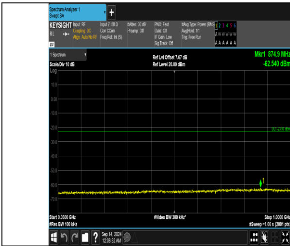
Band66_15MHz_QPSK_132597_1RB#74_30~1000_30~1000
