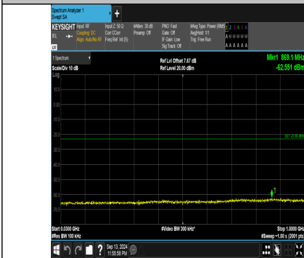
Band66_15MHz_QPSK_132047_1RB#0_30~1000_30~1000
