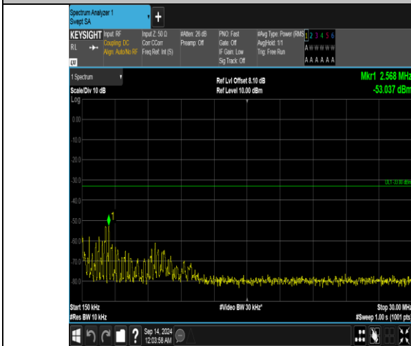
Band66_15MHz_16QAM_132322_1RB#74_0.15~30_0.15~30
