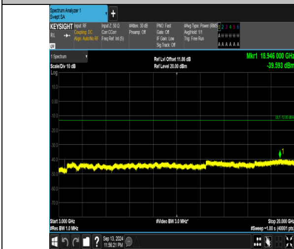
Band66_15MHz_QPSK_132047_1RB#0_3000~20000_3000~20000
