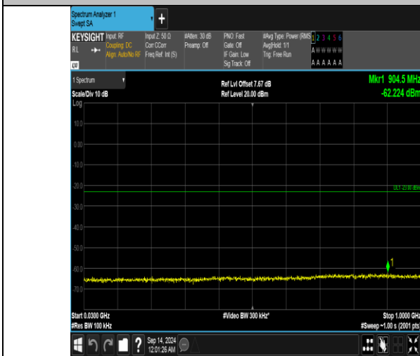
Band66_15MHz_QPSK_132322_1RB#0_30~1000_30~1000
