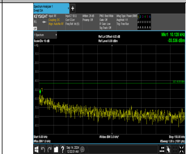
Band66_15MHz_16QAM_132322_1RB#0_0.009~0.15_0.009~0.15
