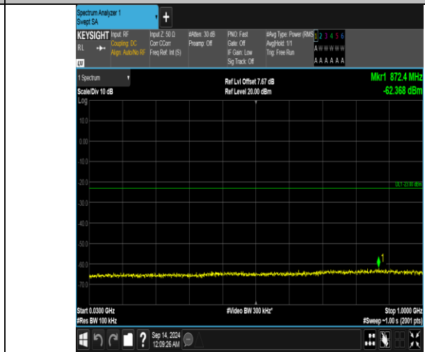
Band66_15MHz_16QAM_132597_1RB#74_30~1000_30~1000
