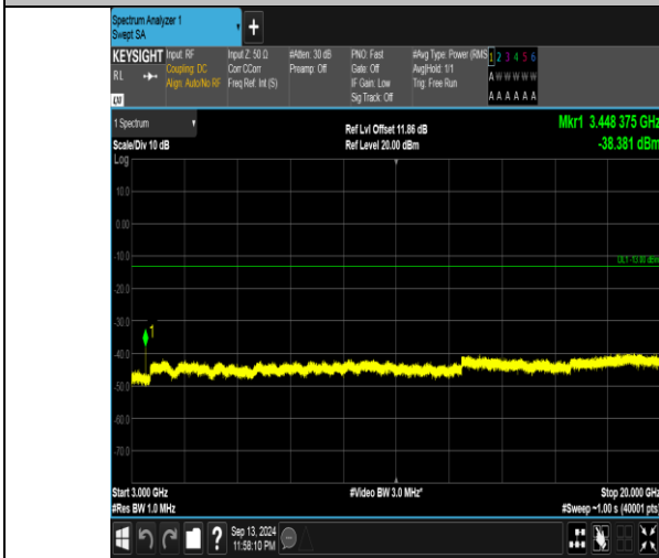
Band66_15MHz_QPSK_132047_1RB#74_3000~20000_3000~20000
