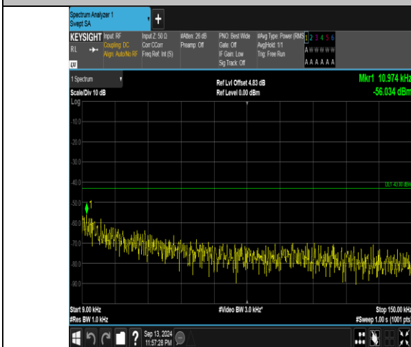
Band66_15MHz_QPSK_132047_1RB#74_0.009~0.15_0.009~0.15
