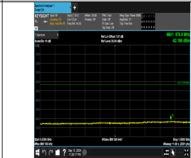
Band66_10MHz_16QAM_132622_50RB#0_30~1000_30~1000
