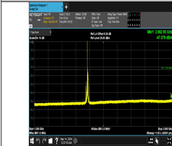
Band66_15MHz_16QAM_132597_1RB#0_1000-3000_1000-3000
