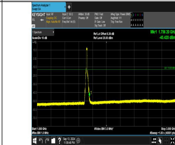
Band66_15MHz_QPSK_132047_75RB#0_1000~3000_1000~3000
