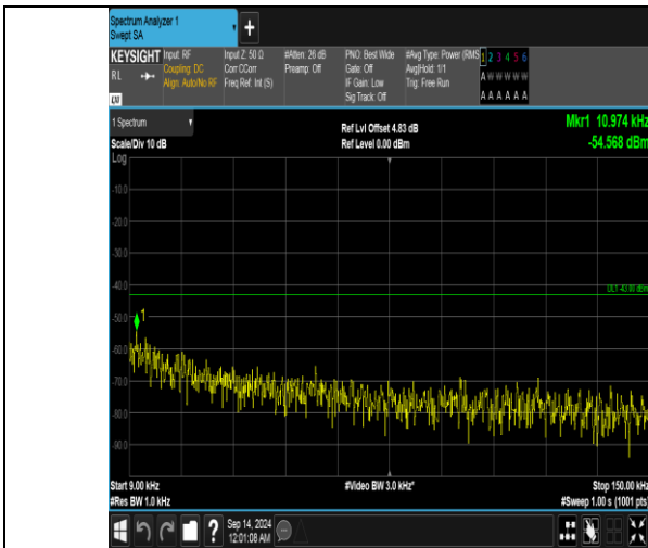
Band66_15MHz_QPSK_132322_1RB#0_0.009~0.15_0.009~0.15
