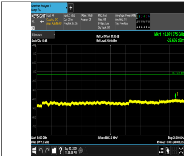
Band66_15MHz_QPSK_132047_75RB#0_3000~20000_3000~20000
