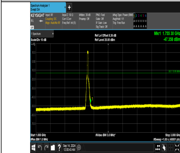
Band66_15MHz_16QAM_132047_75RB#0_1000~3000_1000~3000
