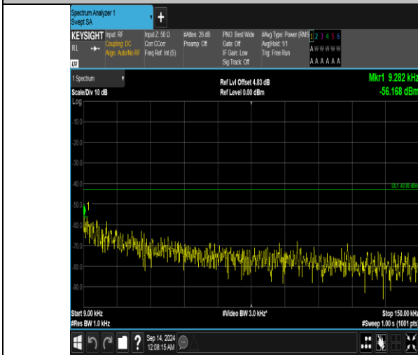
Band66_15MHz_QPSK_132597_1RB#74_0.009-0.15_0.009-0.15
