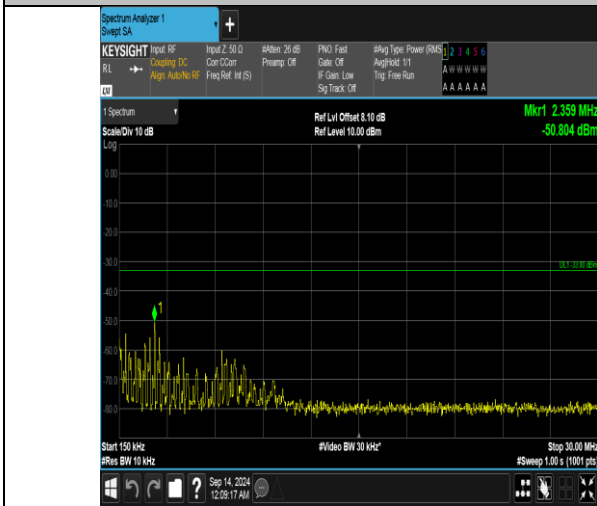
Band66_15MHz_16QAM_132597_1RB#74_0.15~30_0.15~30
