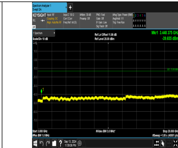
Band66_15MHz_16QAM_132047_1RB#74_3000~20000_3000~20000
