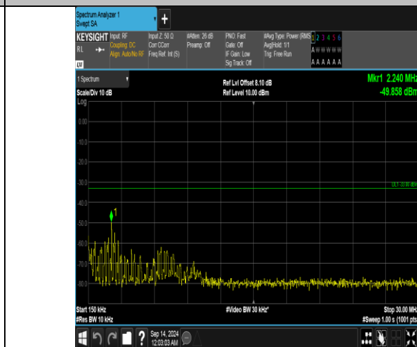
Band66_15MHz_QPSK_132322_1RB#74_0.15~30_0.15~30
