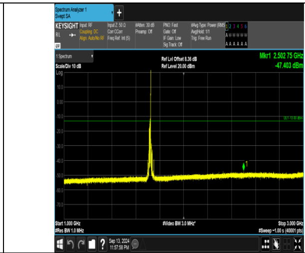
Band66_15MHz_QPSK_132047_1RB#74_1000~3000_1000~3000
