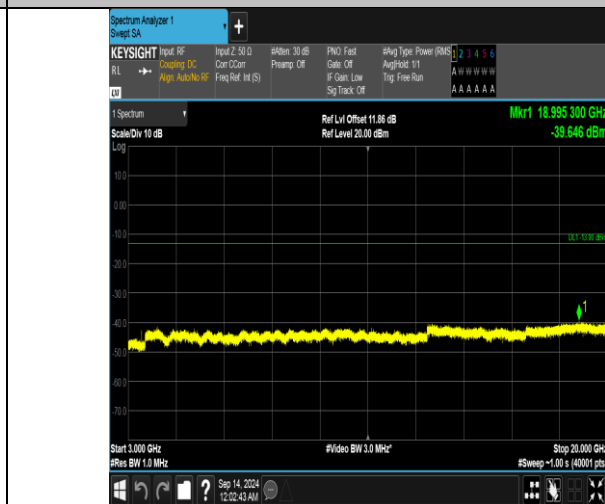
Band66_15MHz_16QAM_132322_1RB#0_3000~20000_3000~20000
