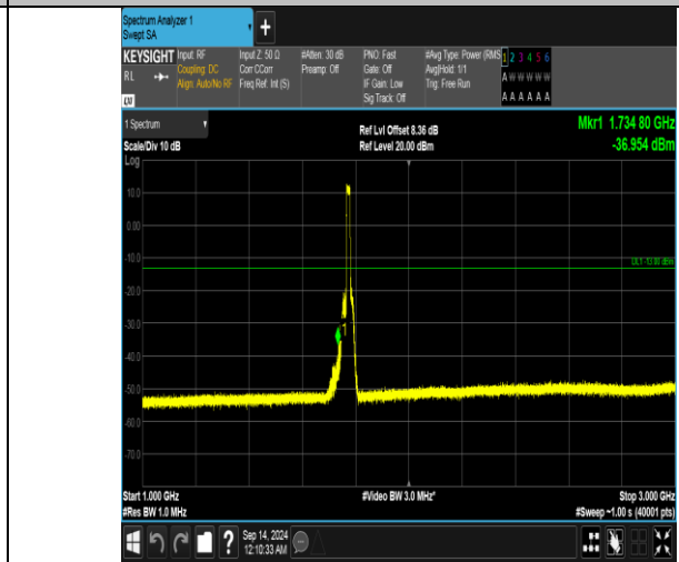
Band66_15MHz_QPSK_132597_75RB#0_1000~3000_1000~3000
