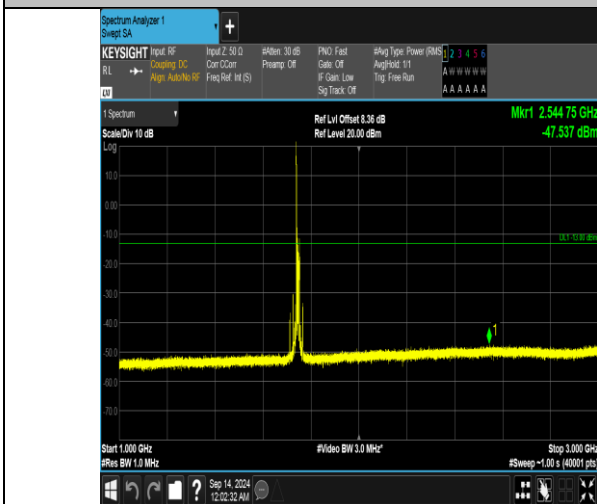
Band66_15MHz_16QAM_132322_1RB#0_1000~3000_1000~3000
