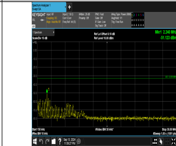
Band66_15MHz_QPSK_132047_75RB#0_0.15~30_0.15~30
