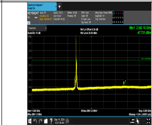
Band66_15MHz_QPSK_132322_1RB#0_1000~3000_1000~3000
