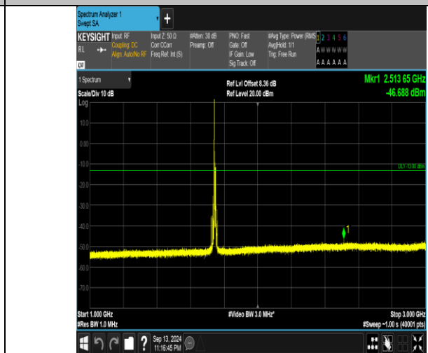
Band66_10MHz_QPSK_132322_1RB#0_1000~3000_1000~3000
