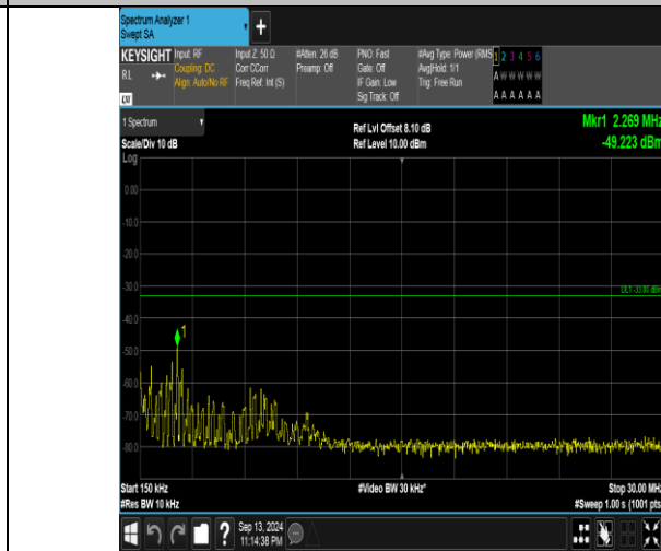
Band66_10MHz_QPSK_132022_50RB#0_0.15~30_0.15~30
