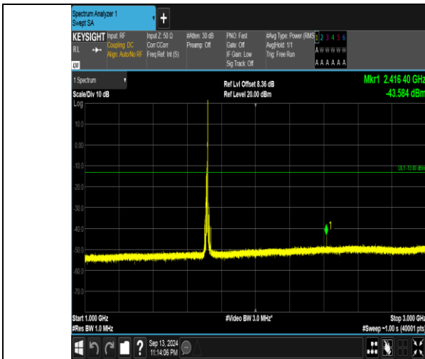
Band66_10MHz_16QAM_132022_1RB#49_1000~3000_1000~3000
