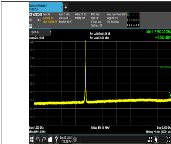
Band66_10MHz_16QAM_132322_1RB#49_1000~3000_1000~3000
