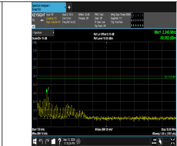
Band66_10MHz_QPSK_132322_1RB#0_0.15~30_0.15~30
