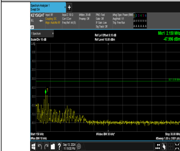
Band66_10MHz_16QAM_132322_1RB#49_0.15~30_0.15~30
