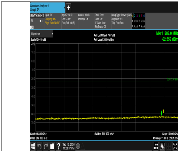
Band66_10MHz_QPSK_132622_1RB#49_30~1000_30~1000
