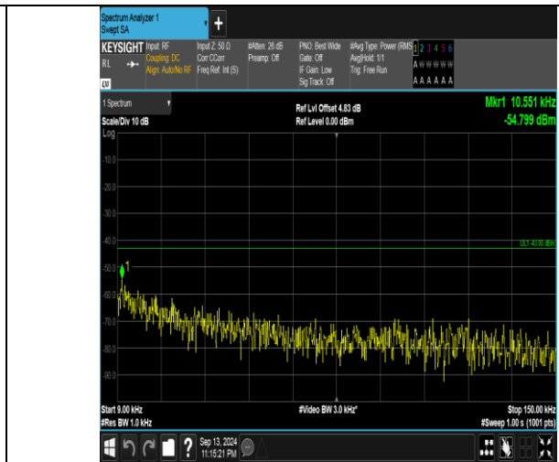
Band66_10MHz_16QAM_132022_50RB#0_0.009~0.15_0.009~0.15
