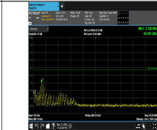
Band66_10MHz_QPSK_132622_1RB#49_0.15~30_0.15~30
