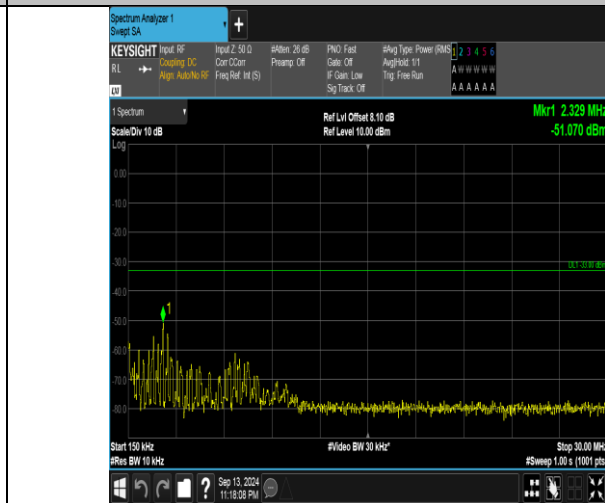
Band66_10MHz_QPSK_132322_1RB#49_0.15-30_0.15-30
