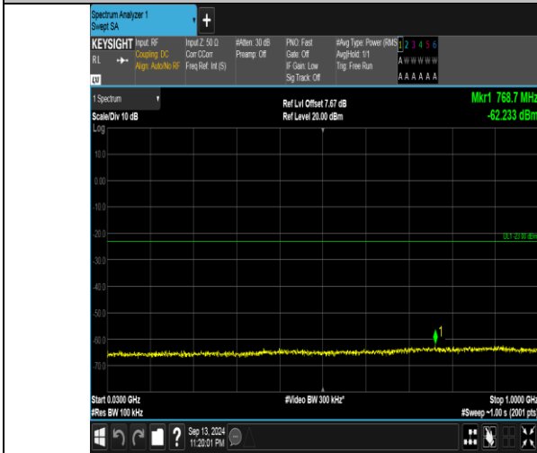
Band66_10MHz_QPSK_132322_50RB#0_30~1000_30~1000
