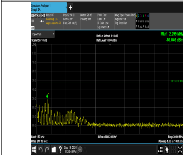
Band66_10MHz_16QAM_132322_50RB#0_0.15~30_0.15~30
