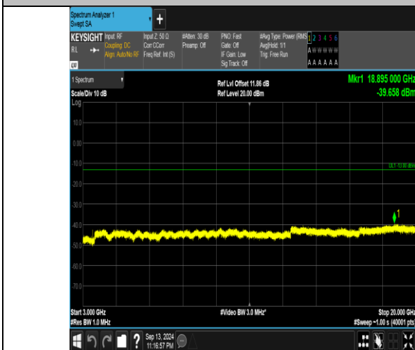
Band66_10MHz_QPSK_132322_1RB#0_3000~20000_3000~20000
