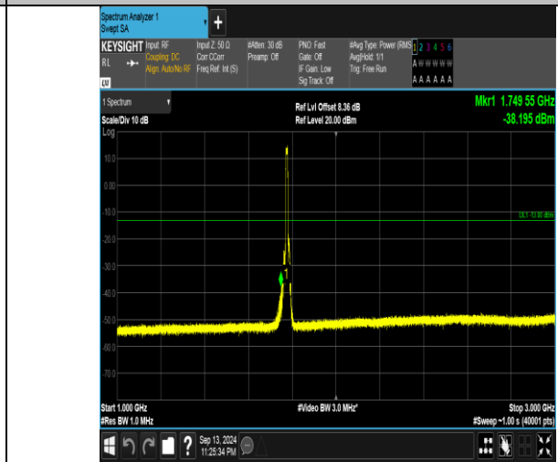
Band66_10MHz_QPSK_132622_50RB#0_1000~3000_1000~3000
