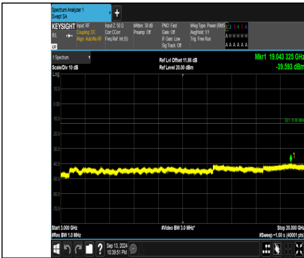
Band66_5MHz_QPSK_132647_25RB#0_3000~20000_3000~20000
