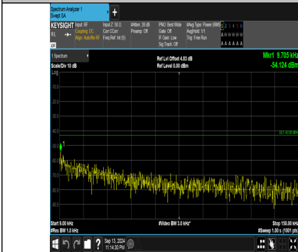
Band66_10MHz_QPSK_132022_50RB#0_0.009~0.15_0.009~0.15
