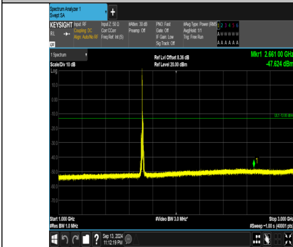
Band66_10MHz_16QAM_132022_1RB#0_1000-3000_1000-3000
