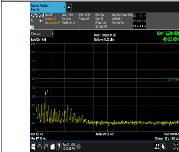
Band66_5MHz_16QAM_132647_25RB#0_0.15~30_0.15~30
