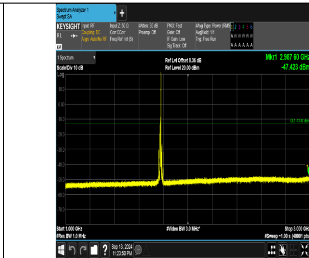
Band66_10MHz_QPSK_132622_1RB#49_1000~3000_1000~3000
