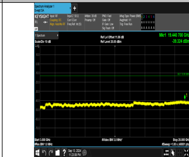
Band66_10MHz_16QAM_132622_1RB#0_3000~20000_3000~20000
