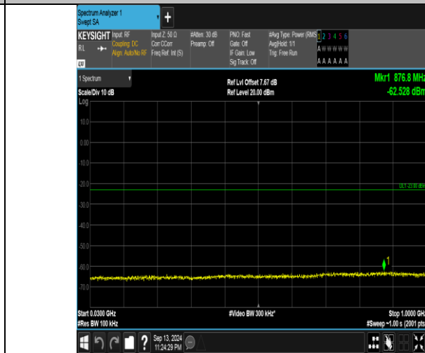
Band66_10MHz_16QAM_132622_1RB#49_30~1000_30~1000
