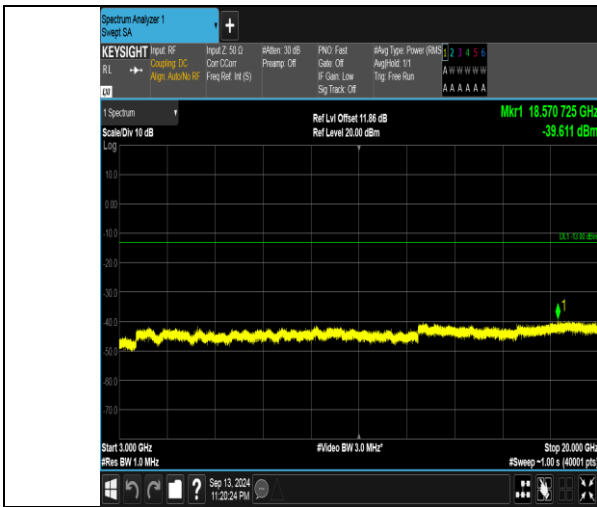
Band66_10MHz_QPSK_132322_50RB#0_3000~20000_3000~20000
