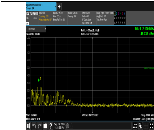
Band66_10MHz_16QAM_132022_1RB#0_0.15-30_0.15-30
