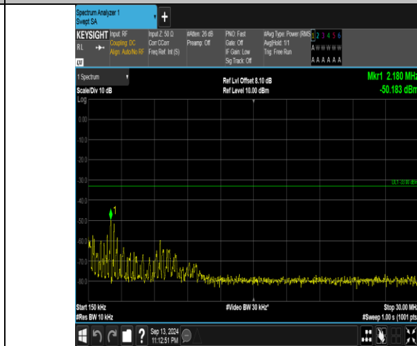
Band66_10MHz_QPSK_132022_1RB#49_0.15-30_0.15-30
