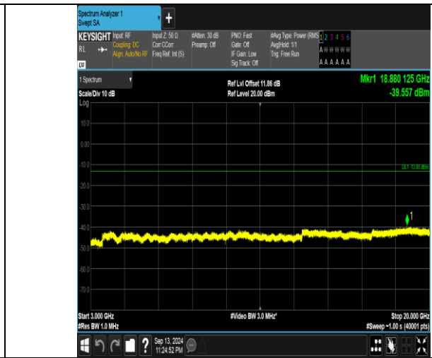
Band66_10MHz_16QAM_132622_1RB#49_3000~20000_3000~20000
