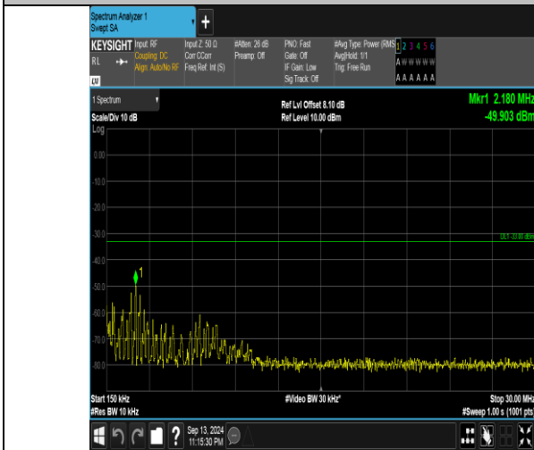
Band66_10MHz_16QAM_132022_50RB#0_0.15~30_0.15~30
