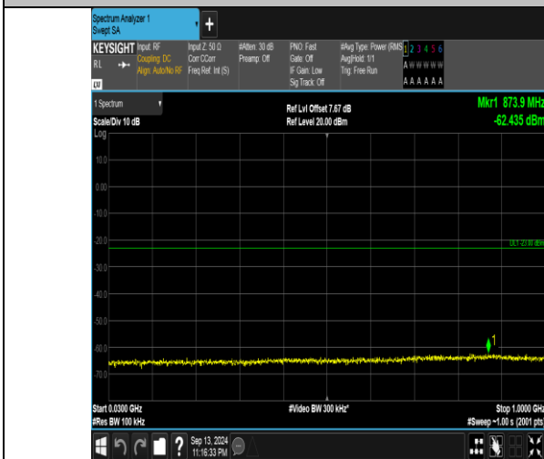
Band66_10MHz_QPSK_132322_1RB#0_30~1000_30~1000
