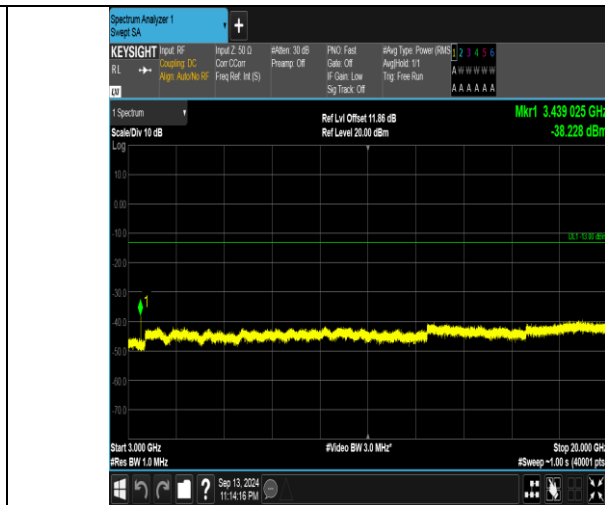
Band66_10MHz_16QAM_132022_1RB#49_3000~20000_3000~20000
