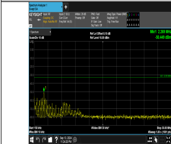
Band66_10MHz_16QAM_132622_1RB#49_0.15~30_0.15~30
