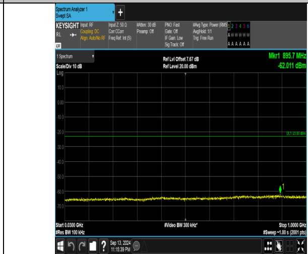
Band66_10MHz_16QAM_132022_50RB#0_30~1000_30~1000
