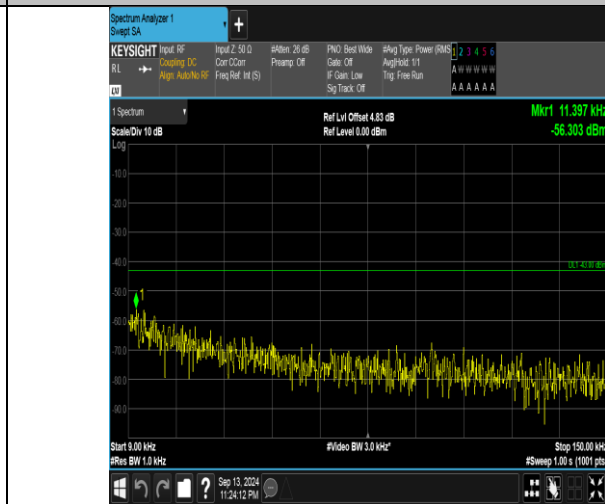
Band66_10MHz_16QAM_132622_1RB#49_0.009~0.15_0.009~0.15
