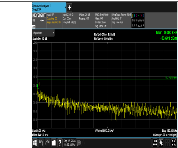
Band66_10MHz_16QAM_132322_50RB#0_0.009~0.15_0.009~0.15
