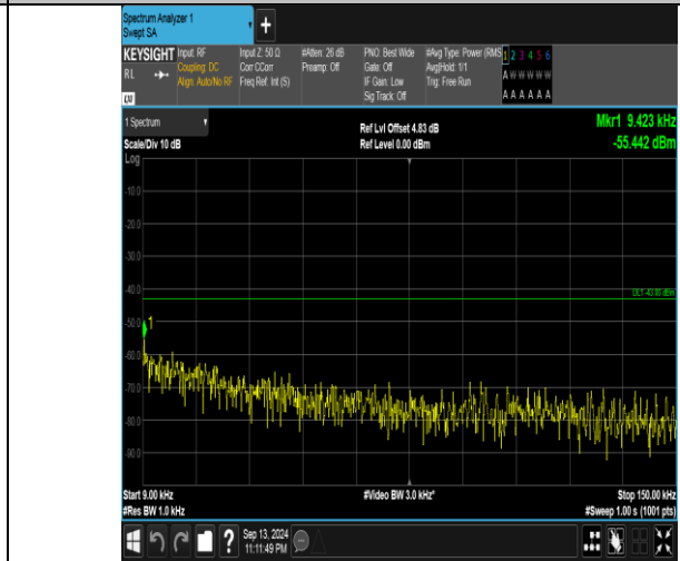
Band66_10MHz_16QAM_132022_1RB#0_0.009~0.15_0.009~0.15
