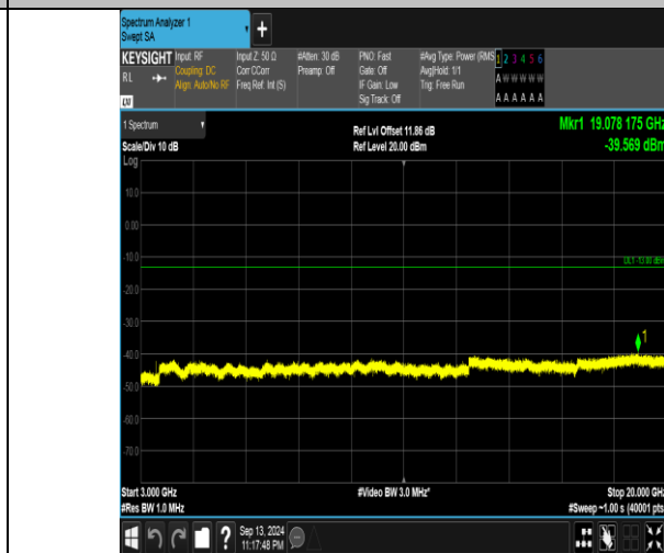
Band66_10MHz_16QAM_132322_1RB#0_3000-20000_3000-20000
