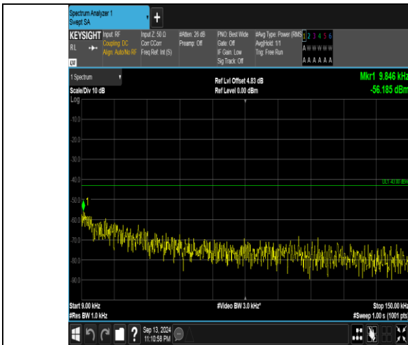
Band66_10MHz_QPSK_132022_1RB#0_0.009~0.15_0.009~0.15
