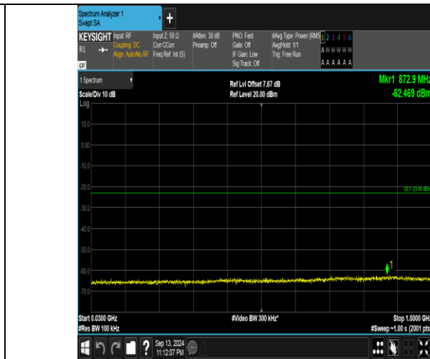
Band66_10MHz_16QAM_132022_1RB#0_30-1000_30-1000
