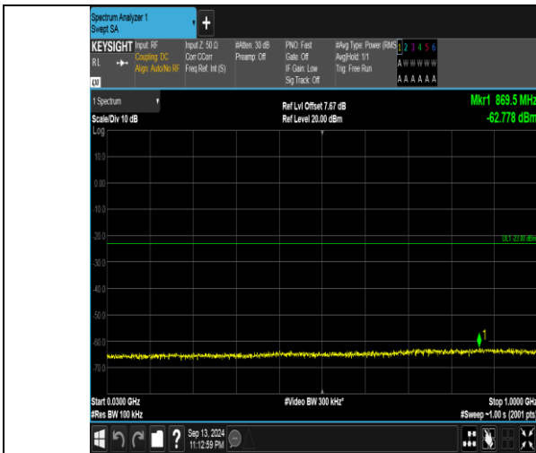
Band66_10MHz_QPSK_132022_1RB#49_30~1000_30~1000
