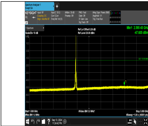
Band66_10MHz_16QAM_132622_1RB#49_1000~3000_1000~3000
