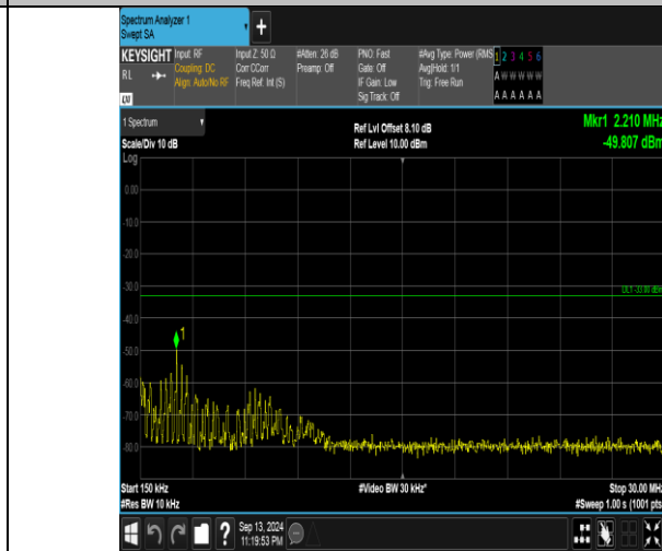
Band66_10MHz_QPSK_132322_50RB#0_0.15~30_0.15~30
