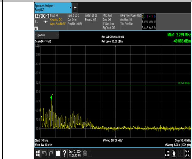
Band66_10MHz_QPSK_132622_50RB#0_0.15~30_0.15~30
