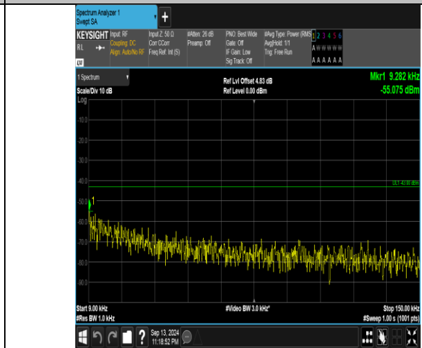
Band66_10MHz_16QAM_132322_1RB#49_0.009~0.15_0.009~0.15
