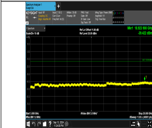
Band66_10MHz_QPSK_132622_1RB#49_3000~20000_3000~20000
