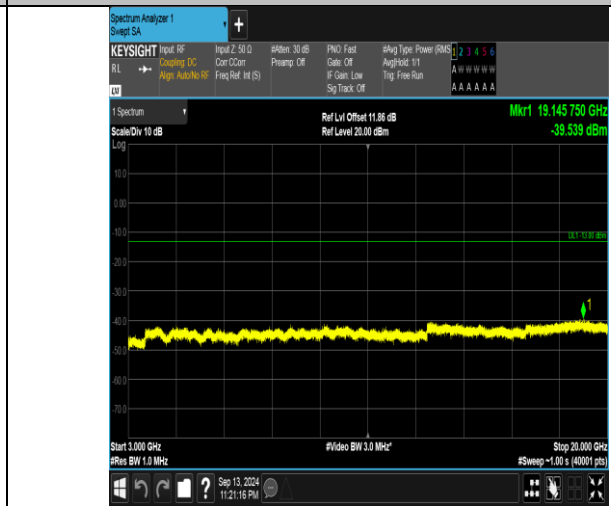
Band66_10MHz_16QAM_132322_50RB#0_3000~20000_3000~20000
