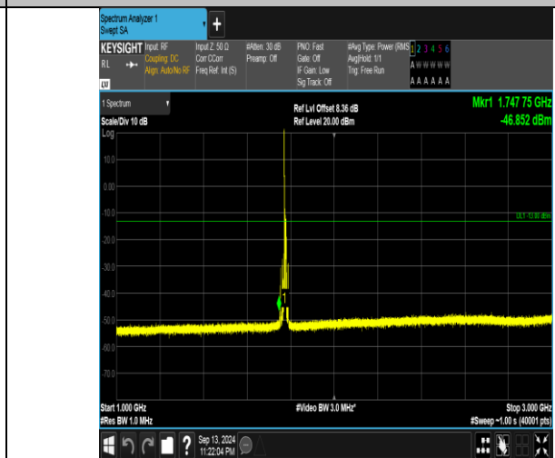
Band66_10MHz_QPSK_132622_1RB#0_1000~3000_1000~3000
