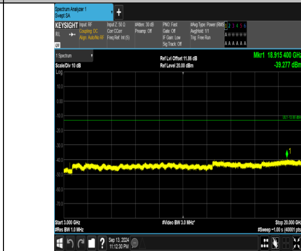
Band66_10MHz_16QAM_132022_1RB#0_3000-20000_3000-20000
