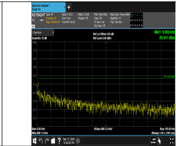
Band66_5MHz_16QAM_132647_25RB#0_0.009~0.15_0.009~0.15
