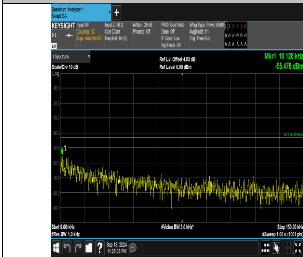
Band66_10MHz_QPSK_132622_50RB#0_0.009~0.15_0.009~0.15
