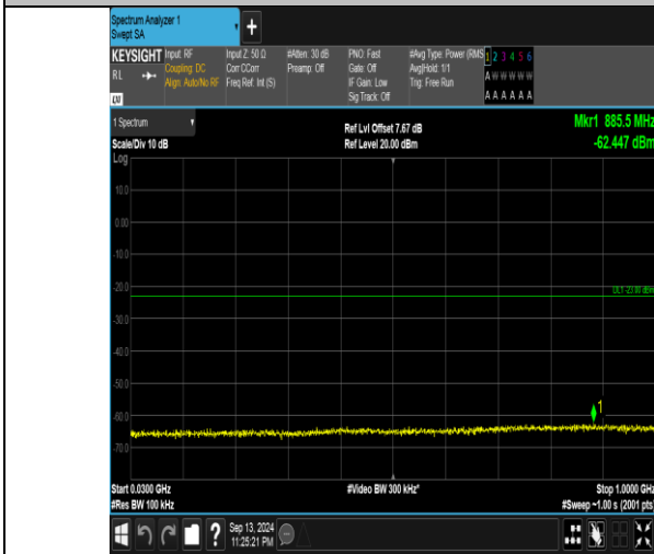
Band66_10MHz_QPSK_132622_50RB#0_30~1000_30~1000
