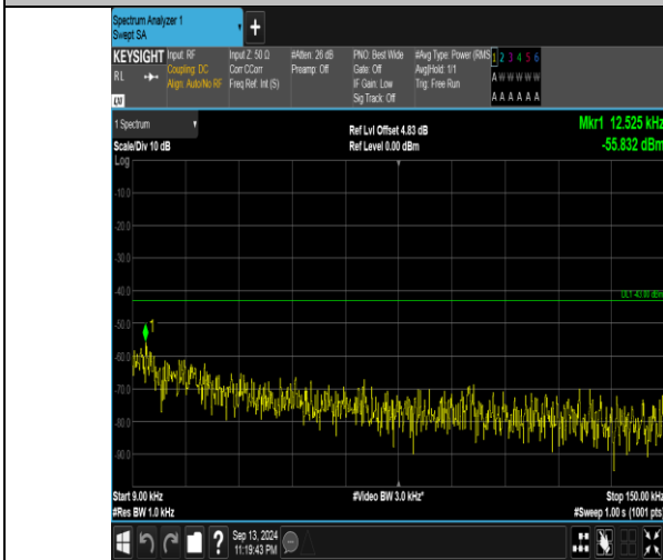
Band66_10MHz_QPSK_132322_50RB#0_0.009~0.15_0.009~0.15
