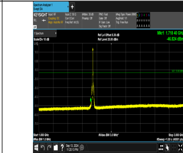
Band66_10MHz_QPSK_132322_50RB#0_1000~3000_1000~3000
