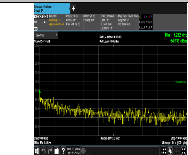
Band66_10MHz_16QAM_132322_1RB#0_0.009~0.15_0.009~0.15
