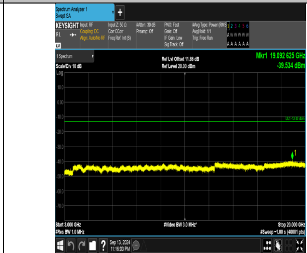
Band66_10MHz_16QAM_132022_50RB#0_3000~20000_3000~20000
