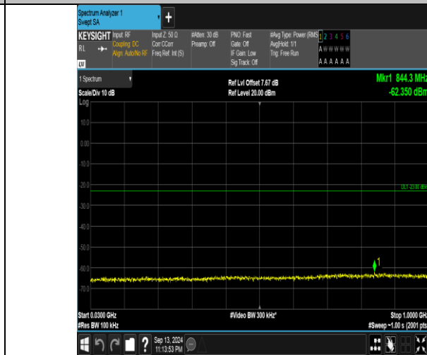
Band66_10MHz_16QAM_132022_1RB#49_30~1000_30~1000
