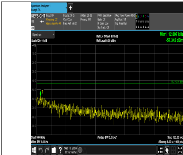
Band66_10MHz_QPSK_132322_1RB#0_0.009~0.15_0.009~0.15
