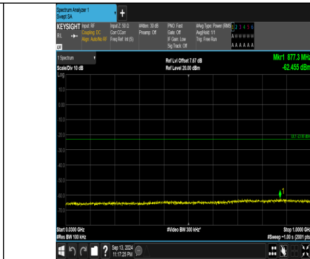
Band66_10MHz_16QAM_132322_1RB#0_30-1000_30-1000
