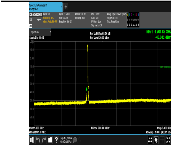
Band66_5MHz_16QAM_132647_25RB#0_1000~3000_1000~3000
