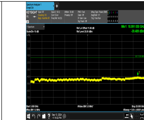
Band66_10MHz_16QAM_132322_1RB#49_3000~20000_3000~20000
