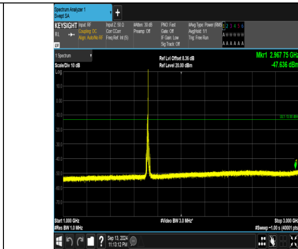
Band66_10MHz_QPSK_132022_1RB#49_1000~3000_1000~3000
