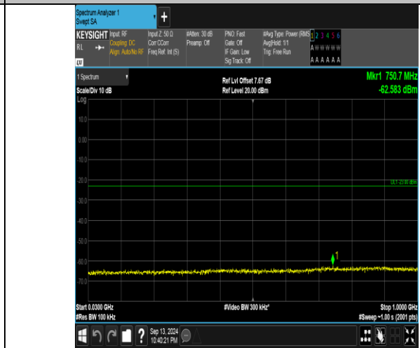
Band66_5MHz_16QAM_132647_25RB#0_30~1000_30~1000
