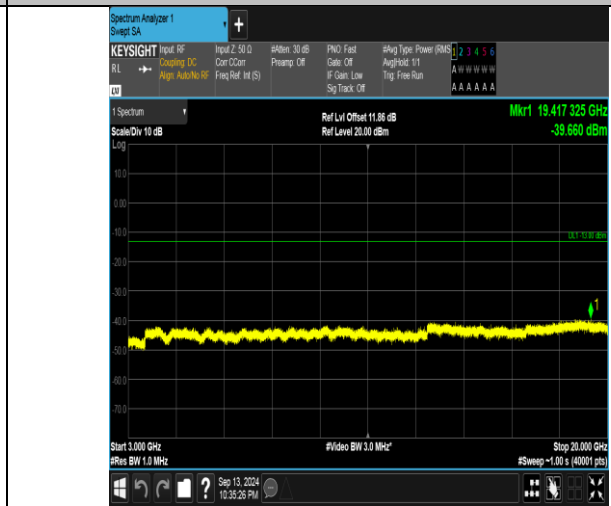
Band66_5MHz_16QAM_132322_25RB#0_3000~20000_3000~20000
