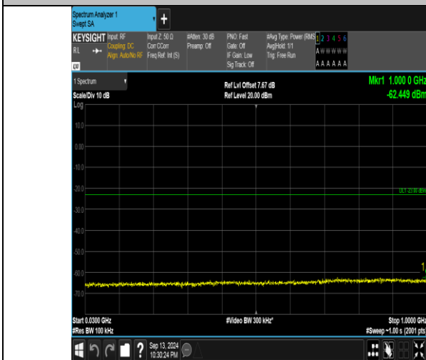
Band66_5MHz_QPSK_132322_1RB#0_30-1000_30-1000
