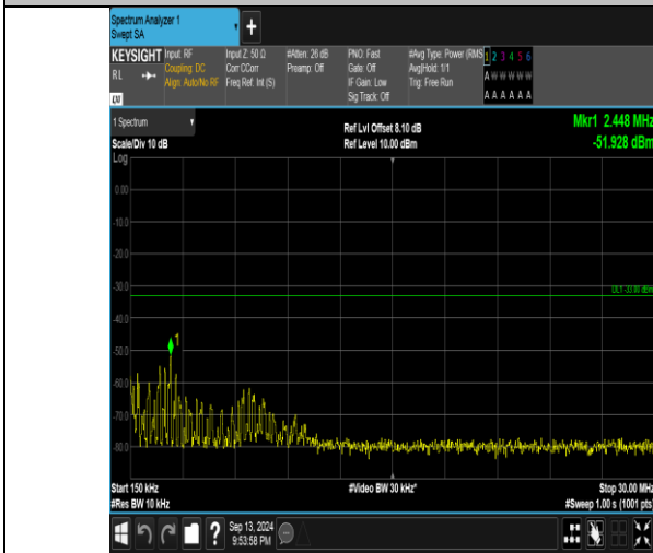
Band66_3MHz_16QAM_132657_15RB#0_0.15~30_0.15~30
