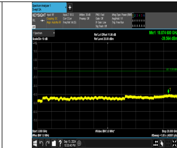
Band66_5MHz_16QAM_132322_1RB#24_3000~20000_3000~20000
