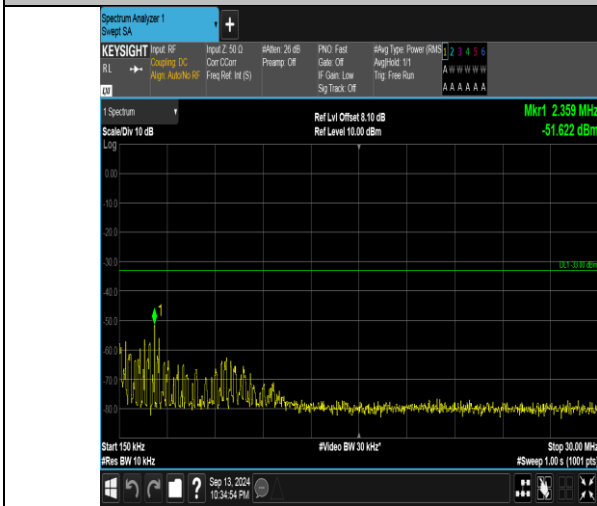
Band66_5MHz_16QAM_132322_25RB#0_0.15~30_0.15~30
