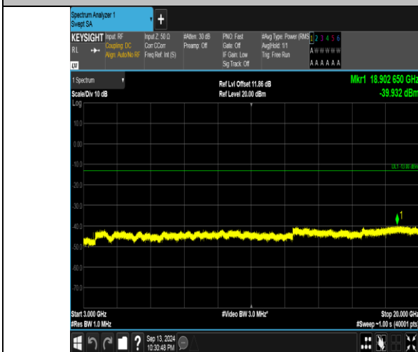
Band66_5MHz_QPSK_132322_1RB#0_3000-20000_3000-20000
