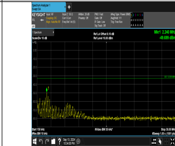
Band66_5MHz_QPSK_132322_25RB#0_0.15~30_0.15~30
