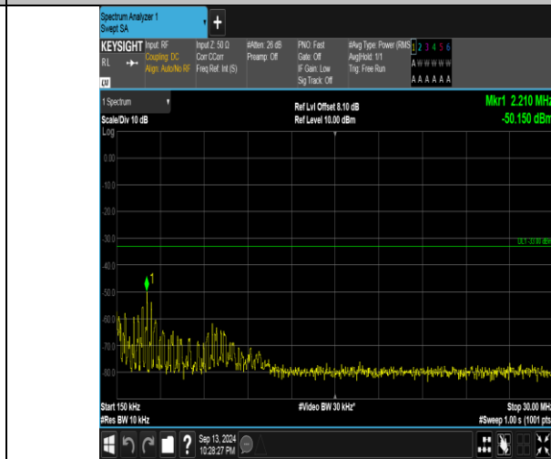
Band66_5MHz_QPSK_131997_25RB#0_0.15~30_0.15~30
