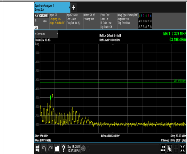
Band66_5MHz_QPSK_132647_1RB#24_0.15~30_0.15~30
