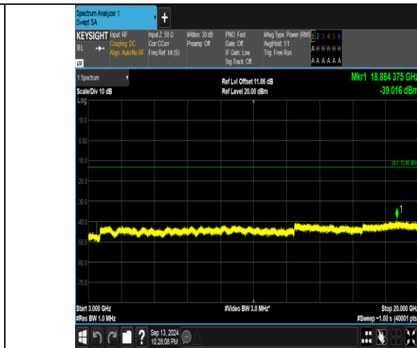
Band66_5MHz_16QAM_131997_1RB#24_3000~20000_3000~20000
