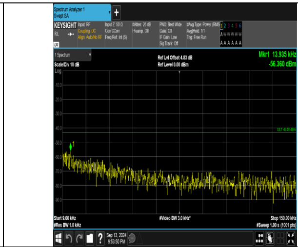
Band66_3MHz_16QAM_132657_15RB#0_0.009~0.15_0.009~0.15
