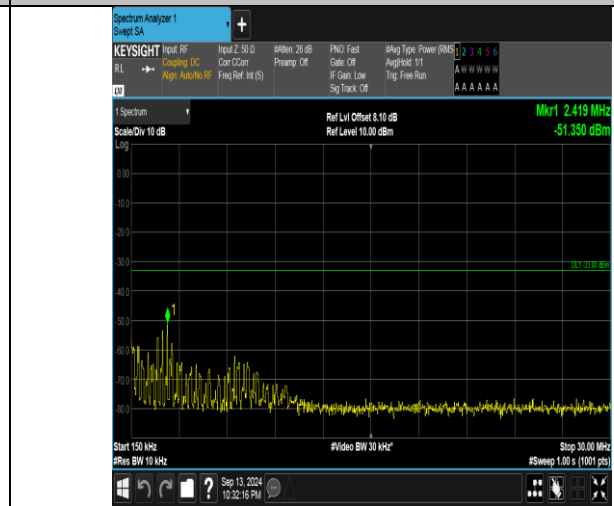
Band66_5MHz_QPSK_132322_1RB#24_0.15~30_0.15~30
