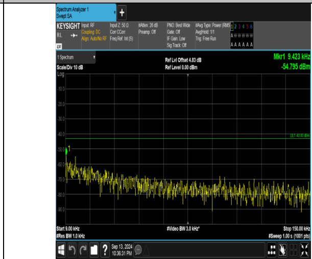
Band66_5MHz_16QAM_132647_1RB#0_0.009-0.15_0.009-0.15
