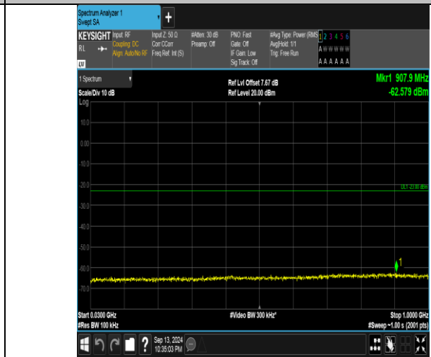
Band66_5MHz_16QAM_132322_25RB#0_30~1000_30~1000
