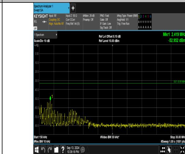
Band66_5MHz_QPSK_132647_25RB#0_0.15~30_0.15~30
