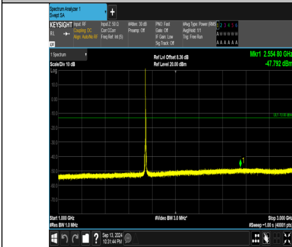
Band66_5MHz_16QAM_132322_1RB#0_1000~3000_1000~3000
