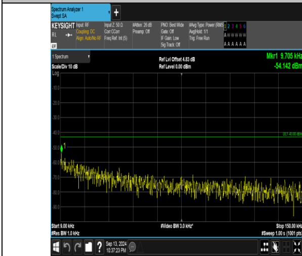
Band66_5MHz_QPSK_132647_1RB#24_0.009~0.15_0.009~0.15
