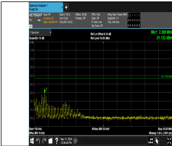
Band66_5MHz_16QAM_132647_1RB#0_0.15~30_0.15~30
