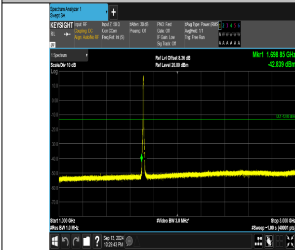
Band66_5MHz_16QAM_131997_25RB#0_1000~3000_1000~3000
