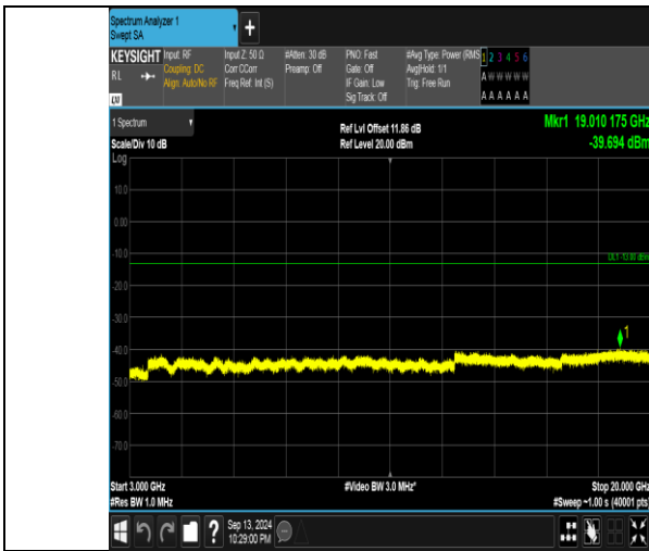
Band66_5MHz_QPSK_131997_25RB#0_3000~20000_3000~20000
