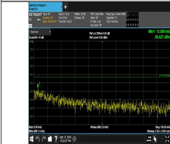
Band66_5MHz_QPSK_132322_1RB#24_0.009~0.15_0.009~0.15
