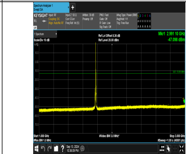
Band66_5MHz_QPSK_132647_1RB#0_1000-3000_1000-3000
