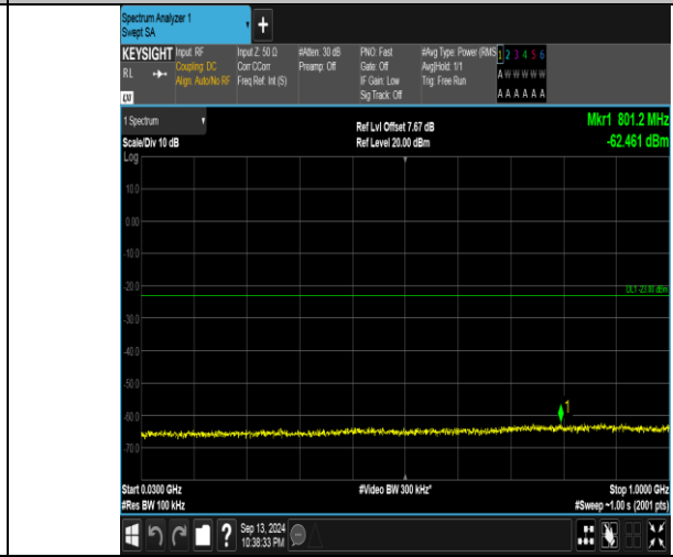
Band66_5MHz_16QAM_132647_1RB#24_30~1000_30~1000
