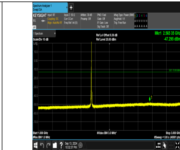
Band66_5MHz_QPSK_132322_1RB#24_1000~3000_1000~3000
