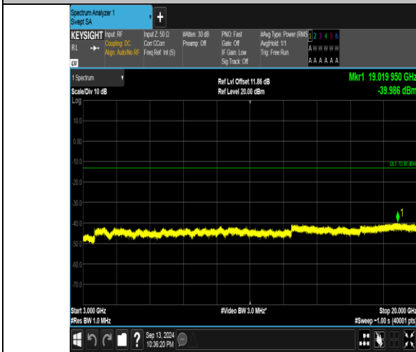
Band66_5MHz_QPSK_132647_1RB#0_3000-20000_3000-20000
