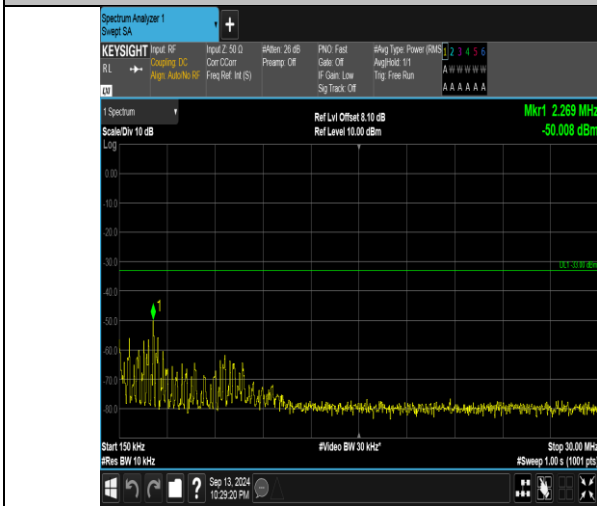
Band66_5MHz_16QAM_131997_25RB#0_0.15~30_0.15~30
