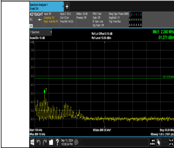
Band66_5MHz_16QAM_132647_1RB#24_0.15~30_0.15~30
