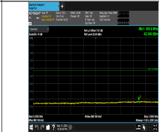
Band66_5MHz_16QAM_131997_25RB#0_30~1000_30~1000
