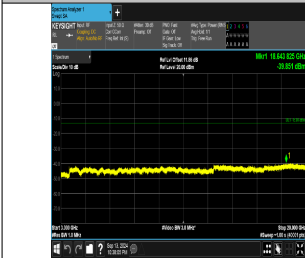
Band66_5MHz_QPSK_132647_1RB#24_3000~20000_3000~20000
