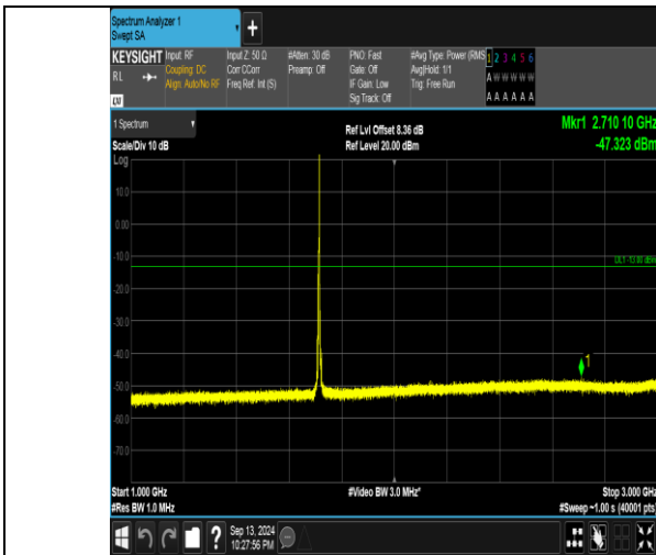
Band66_5MHz_16QAM_131997_1RB#24_1000~3000_1000~3000
