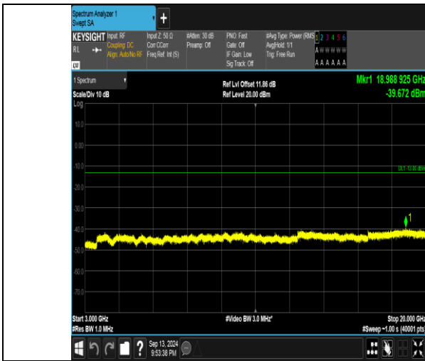
Band66_3MHz_QPSK_132657_15RB#0_3000~20000_3000~20000
