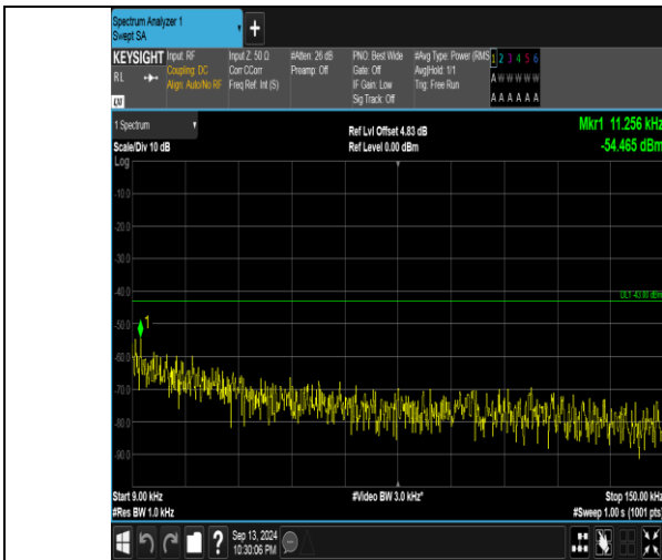
Band66_5MHz_QPSK_132322_1RB#0_0.009-0.15_0.009-0.15
