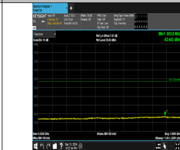
Band66_5MHz_16QAM_131997_1RB#24_30~1000_30~1000
