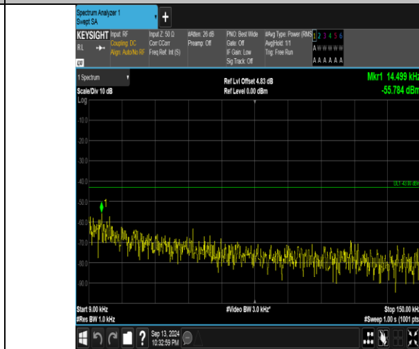
Band66_5MHz_16QAM_132322_1RB#24_0.009~0.15_0.009~0.15
