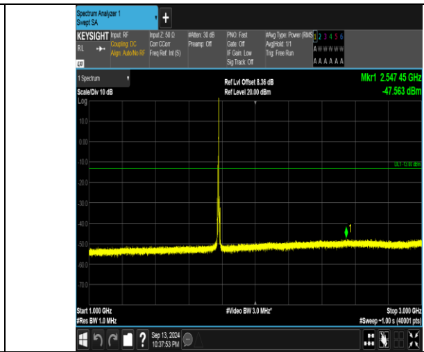
Band66_5MHz_QPSK_132647_1RB#24_1000~3000_1000~3000
