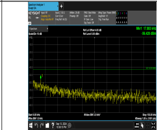
Band66_5MHz_16QAM_132647_1RB#24_0.009~0.15_0.009~0.15
