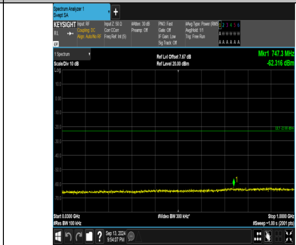
Band66_3MHz_16QAM_132657_15RB#0_30~1000_30~1000
