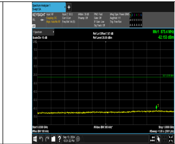
Band66_5MHz_16QAM_132322_1RB#0_30~1000_30~1000
