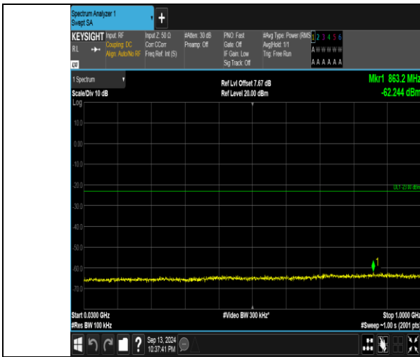
Band66_5MHz_QPSK_132647_1RB#24_30~1000_30~1000
