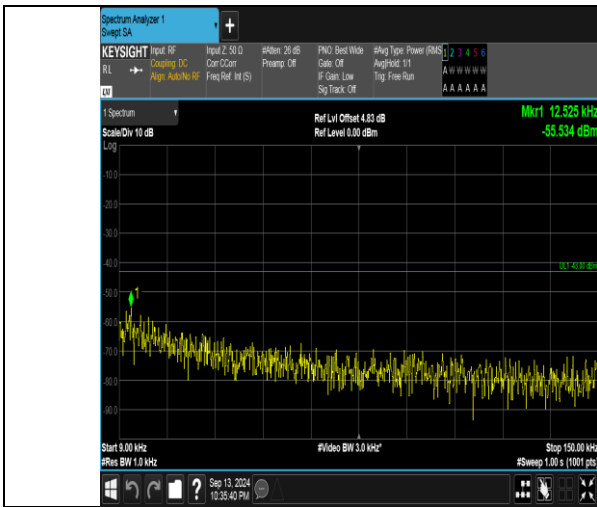
Band66_5MHz_QPSK_132647_1RB#0_0.009-0.15_0.009-0.15
