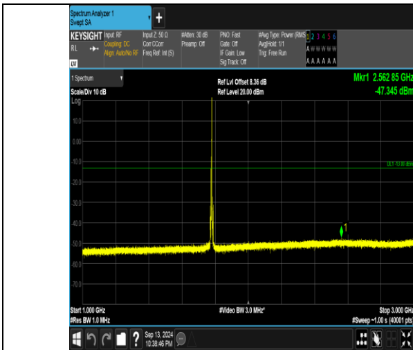
Band66_5MHz_16QAM_132647_1RB#24_1000~3000_1000~3000
