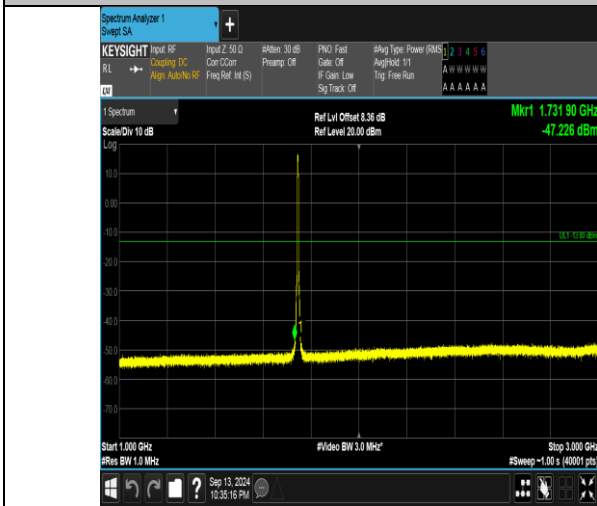
Band66_5MHz_16QAM_132322_25RB#0_1000~3000_1000~3000
