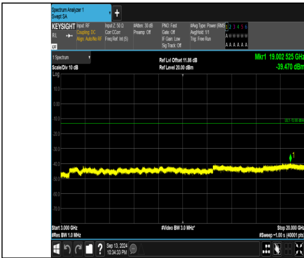
Band66_5MHz_QPSK_132322_25RB#0_3000~20000_3000~20000
