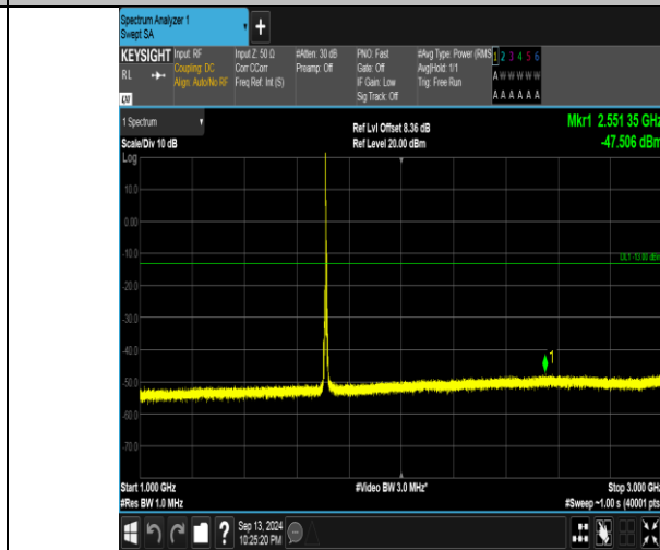
Band66_5MHz_QPSK_131997_1RB#0_1000-3000_1000-3000
