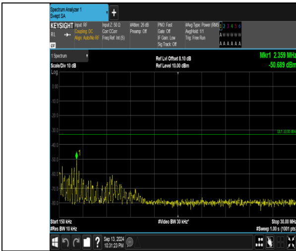
Band66_5MHz_16QAM_132322_1RB#0_0.15~30_0.15~30
