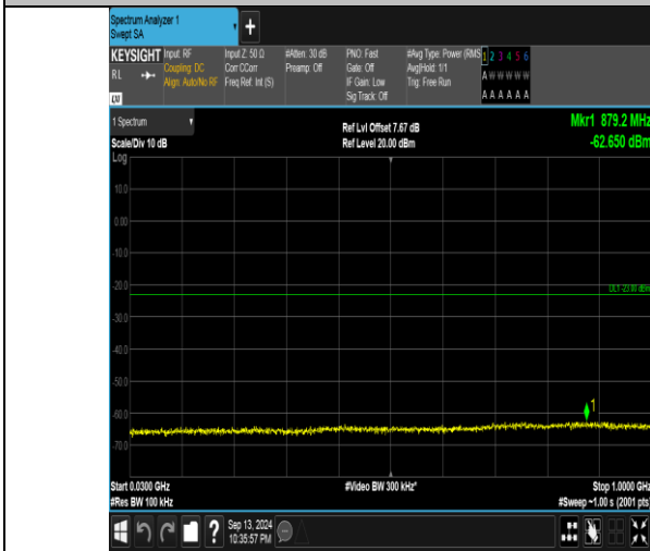
Band66_5MHz_QPSK_132647_1RB#0_30-1000_30-1000
