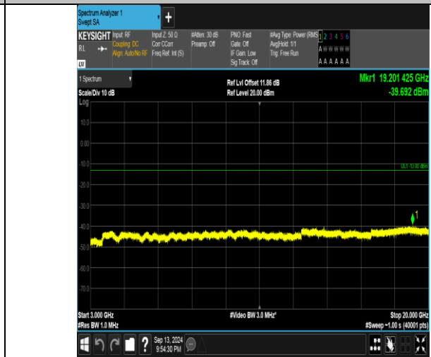
Band66_3MHz_16QAM_132657_15RB#0_3000~20000_3000~20000
