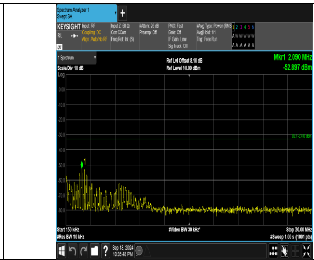
Band66_5MHz_QPSK_132647_1RB#0_0.15-30_0.15-30
