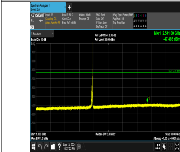
Band66_5MHz_16QAM_132647_1RB#0_1000~3000_1000~3000
