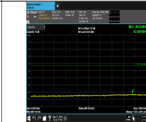
Band66_5MHz_16QAM_132322_1RB#24_30~1000_30~1000
