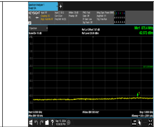
Band66_5MHz_16QAM_132647_1RB#0_30~1000_30~1000
