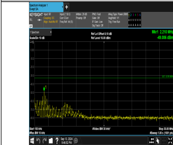
Band66_3MHz_16QAM_132322_1RB#14_0.15~30_0.15~30
