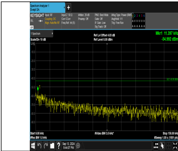
Band66_3MHz_QPSK_132322_1RB#0_0.009-0.15_0.009-0.15
