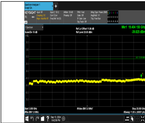
Band66_3MHz_QPSK_131987_15RB#0_3000~20000_3000~20000
