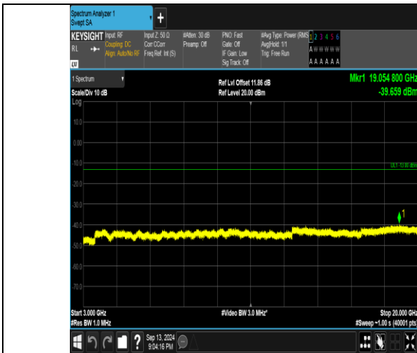
Band66_1.4MHz_QPSK_132665_6RB#0_3000~20000_3000~20000
