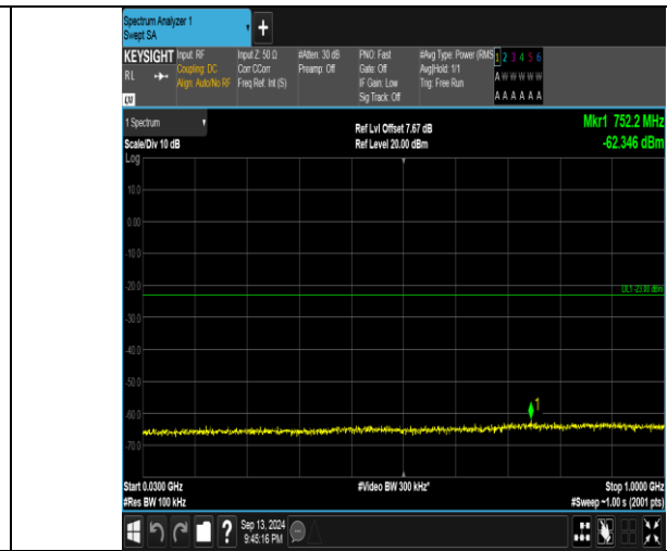
Band66_3MHz_16QAM_132322_1RB#0_30~1000_30~1000
