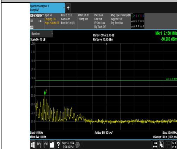
Band66_1.4MHz_16QAM_132665_6RB#0_0.15~30_0.15~30
