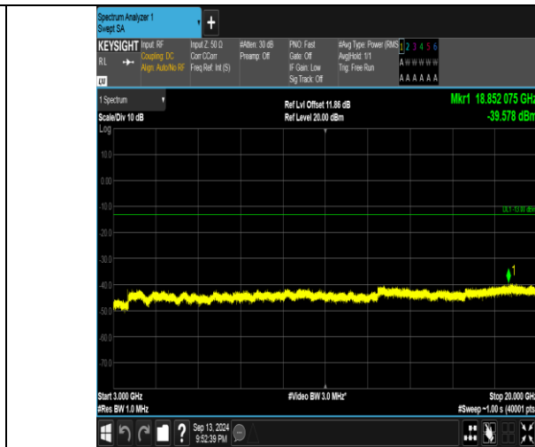
Band66_3MHz_16QAM_132657_1RB#14_3000~20000_3000~20000
