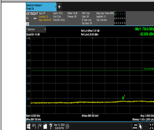
Band66_3MHz_QPSK_132657_1RB#0_30-1000_30-1000
