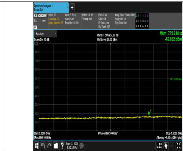
Band66_3MHz_16QAM_132657_1RB#0_30~1000_30~1000
