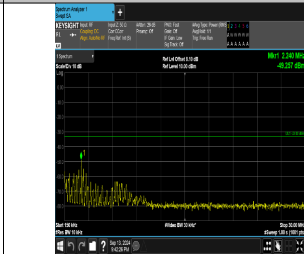
Band66_3MHz_QPSK_131987_15RB#0_0.15~30_0.15~30
