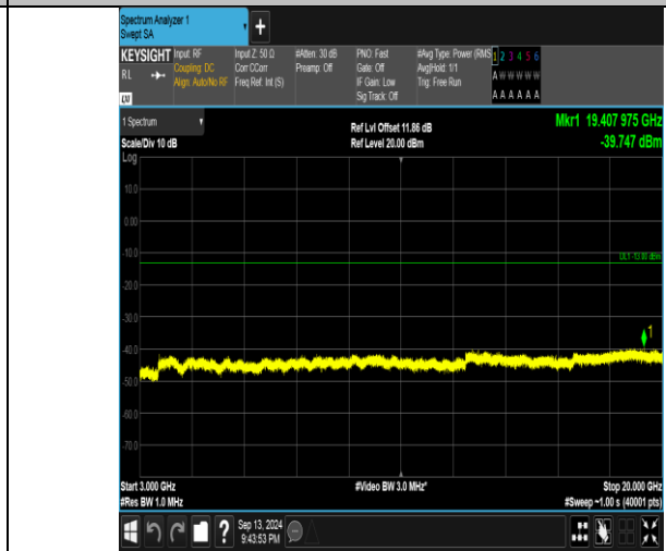
Band66_3MHz_16QAM_131987_15RB#0_3000~20000_3000~20000
