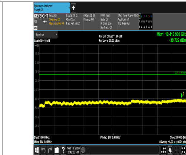
Band66_3MHz_16QAM_131987_1RB#14_3000~20000_3000~20000
