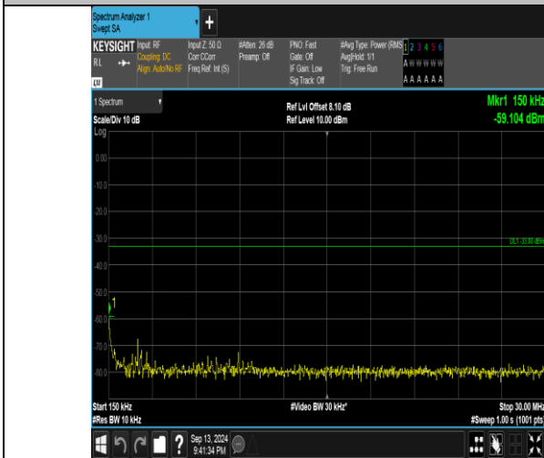
Band66_3MHz_16QAM_131987_1RB#14_0.15~30_0.15~30
