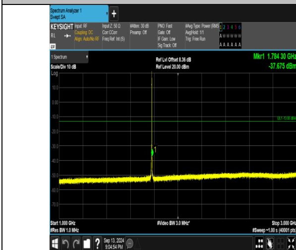
Band66_1.4MHz_16QAM_132665_6RB#0_1000~3000_1000~3000
