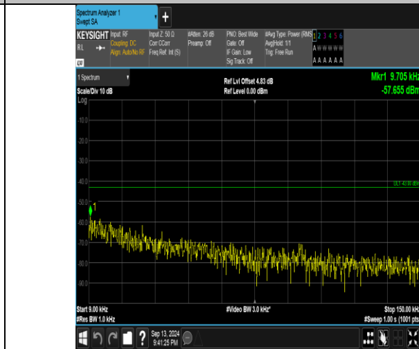
Band66_3MHz_16QAM_131987_1RB#14_0.009~0.15_0.009~0.15
