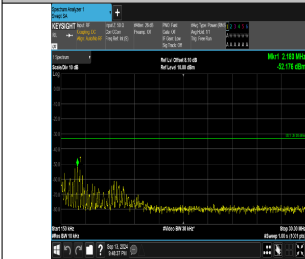
Band66_3MHz_16QAM_132322_15RB#0_0.15~30_0.15~30
