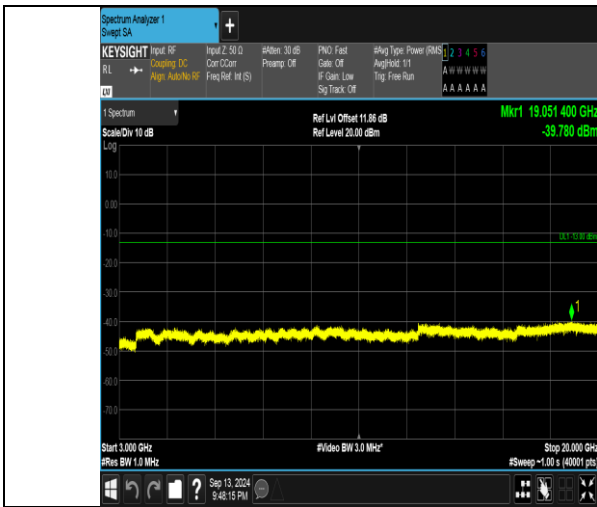
Band66_3MHz_QPSK_132322_15RB#0_3000~20000_3000~20000
