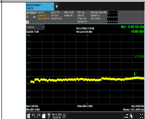
Band66_1.4MHz_16QAM_132665_6RB#0_3000~20000_3000~20000
