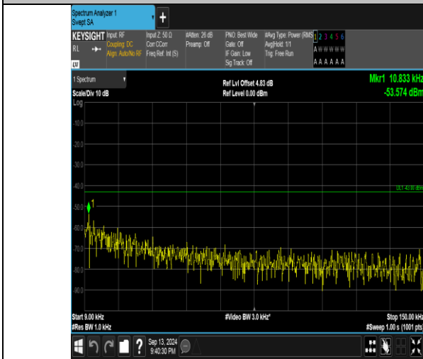
Band66_3MHz_QPSK_131987_1RB#14_0.009~0.15_0.009~0.15
