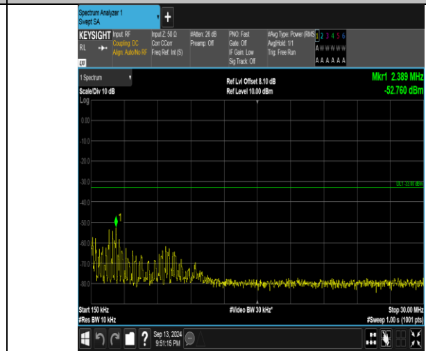
Band66_3MHz_QPSK_132657_1RB#14_0.15~30_0.15~30
