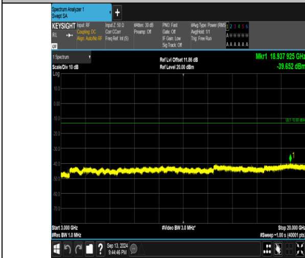
Band66_3MHz_QPSK_132322_1RB#0_3000-20000_3000-20000
