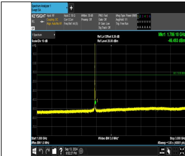
Band66_3MHz_16QAM_132657_1RB#14_1000~3000_1000~3000
