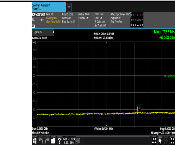
Band66_3MHz_16QAM_132657_1RB#14_30~1000_30~1000
