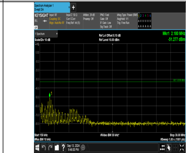
Band66_3MHz_QPSK_132322_1RB#14_0.15~30_0.15~30
