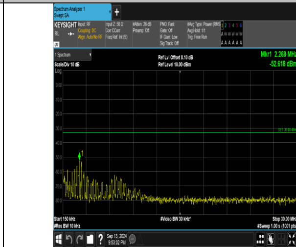
Band66_3MHz_QPSK_132657_15RB#0_0.15~30_0.15~30
