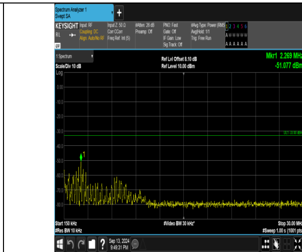
Band66_3MHz_QPSK_132657_1RB#0_0.15-30_0.15-30
