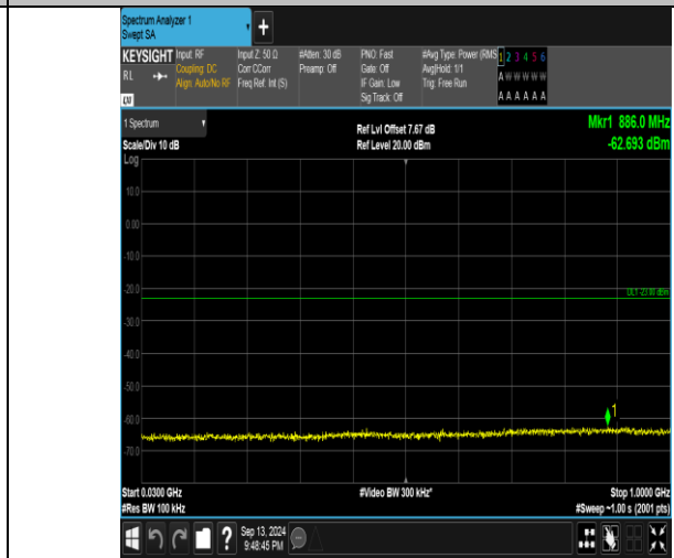
Band66_3MHz_16QAM_132322_15RB#0_30~1000_30~1000
