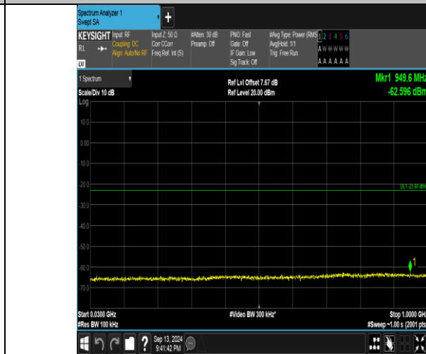
Band66_3MHz_16QAM_131987_1RB#14_30~1000_30~1000
