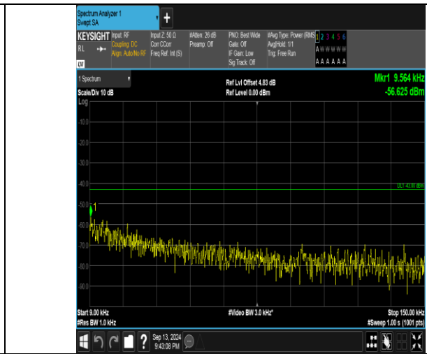
Band66_3MHz_16QAM_131987_15RB#0_0.009~0.15_0.009~0.15
