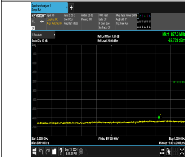
Band66_3MHz_QPSK_132322_1RB#0_30-1000_30-1000
