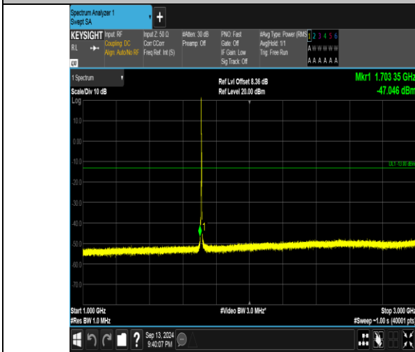
Band66_3MHz_16QAM_131987_1RB#0_1000~3000_1000~3000
