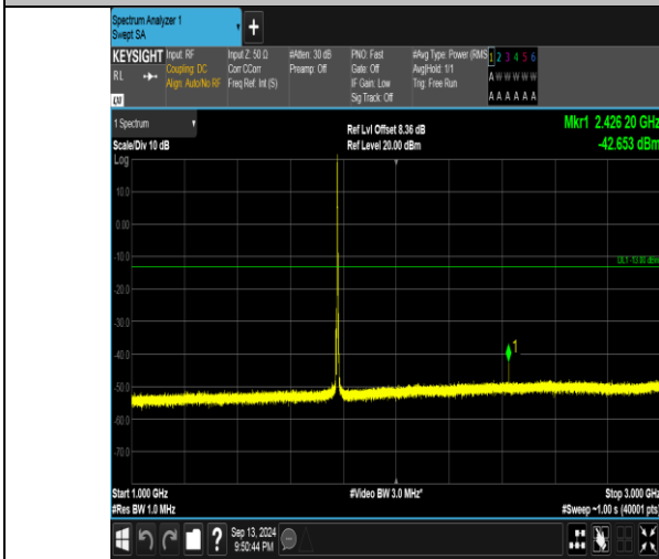
Band66_3MHz_16QAM_132657_1RB#0_1000~3000_1000~3000
