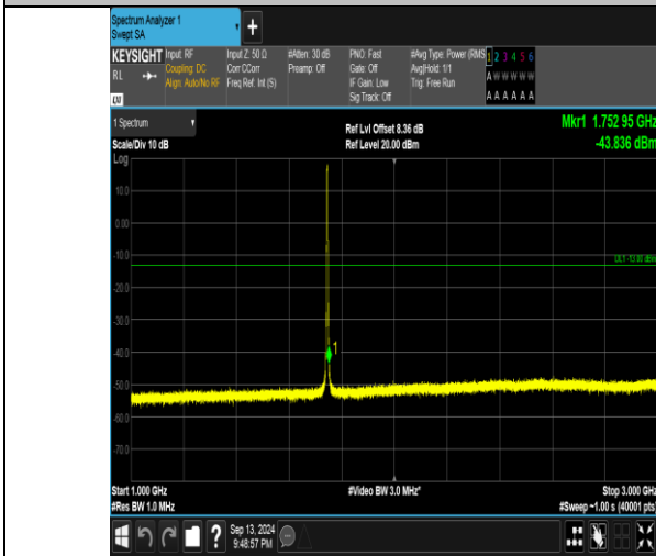
Band66_3MHz_16QAM_132322_15RB#0_1000~3000_1000~3000
