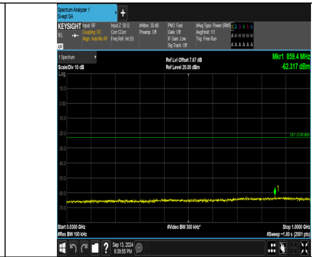
Band66_3MHz_16QAM_131987_1RB#0_30~1000_30~1000
