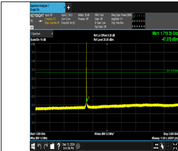
Band66_3MHz_16QAM_131987_1RB#14_1000~3000_1000~3000
