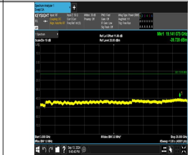
Band66_3MHz_16QAM_132322_1RB#0_3000~20000_3000~20000
