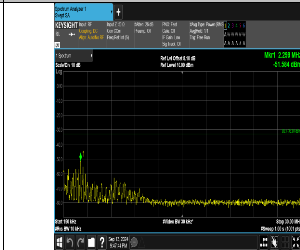
Band66_3MHz_QPSK_132322_15RB#0_0.15~30_0.15~30
