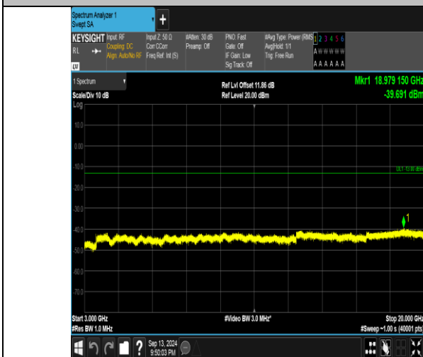
Band66_3MHz_QPSK_132657_1RB#0_3000-20000_3000-20000
