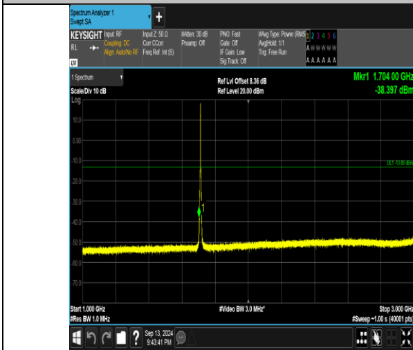
Band66_3MHz_16QAM_131987_15RB#0_1000~3000_1000~3000
