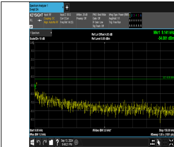
Band66_3MHz_QPSK_132657_1RB#0_0.009-0.15_0.009-0.15
