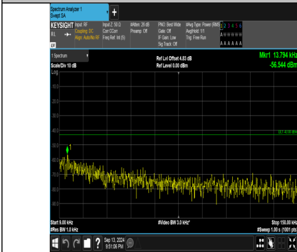
Band66_3MHz_QPSK_132657_1RB#14_0.009~0.15_0.009~0.15
