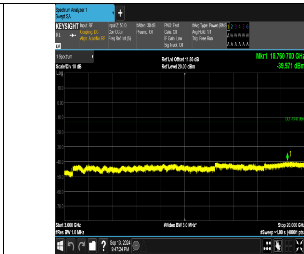
Band66_3MHz_16QAM_132322_1RB#14_3000~20000_3000~20000
