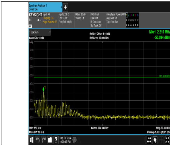
Band66_3MHz_16QAM_131987_1RB#0_0.15~30_0.15~30
