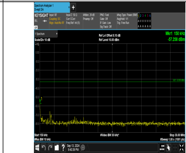
Band66_3MHz_QPSK_131987_1RB#14_0.15~30_0.15~30
