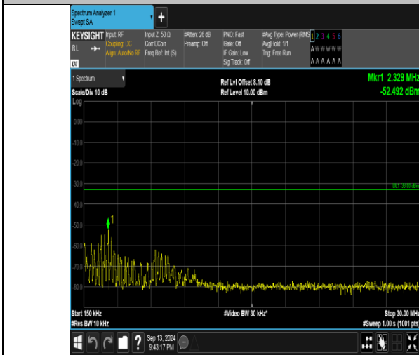
Band66_3MHz_16QAM_131987_15RB#0_0.15~30_0.15~30
