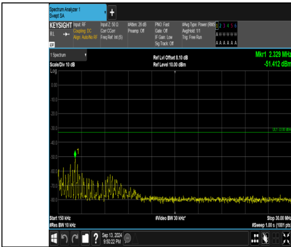
Band66_3MHz_16QAM_132657_1RB#0_0.15~30_0.15~30
