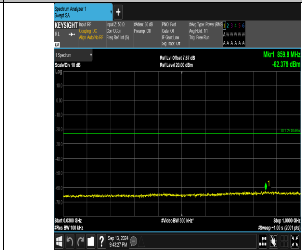
Band66_3MHz_16QAM_131987_15RB#0_30~1000_30~1000
