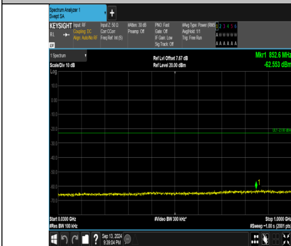
Band66_3MHz_QPSK_131987_1RB#0_30-1000_30-1000
