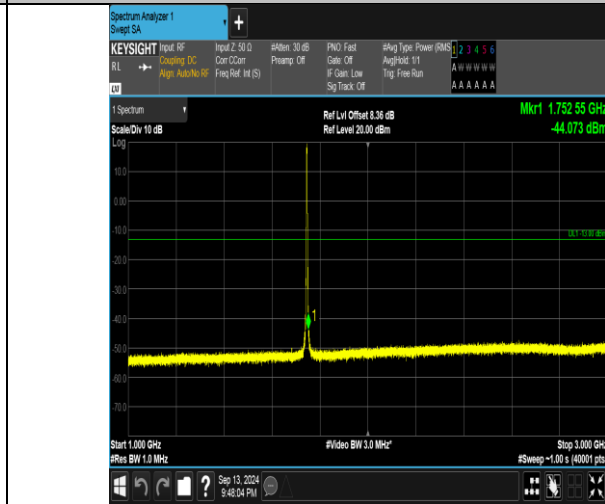
Band66_3MHz_QPSK_132322_15RB#0_1000~3000_1000~3000
