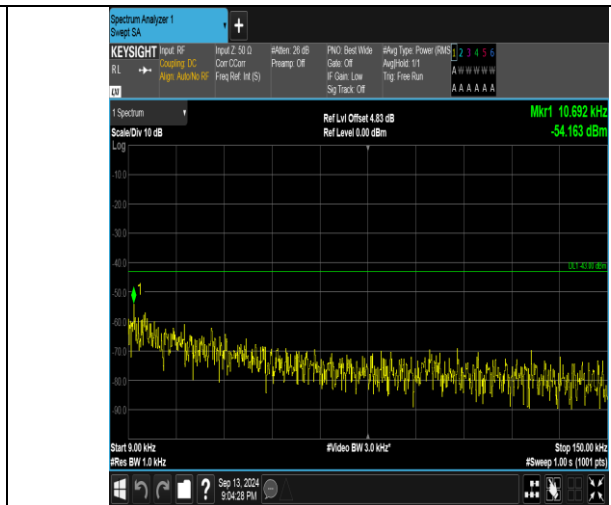
Band66_1.4MHz_16QAM_132665_6RB#0_0.009~0.15_0.009~0.15
