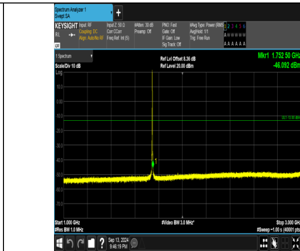
Band66_3MHz_QPSK_132322_1RB#14_1000~3000_1000~3000
