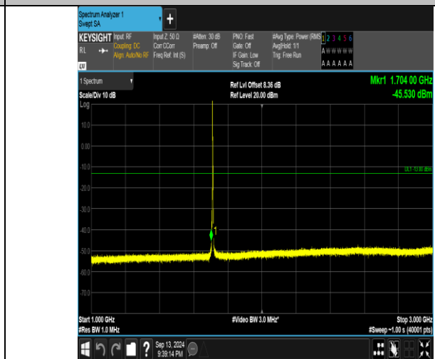
Band66_3MHz_QPSK_131987_1RB#0_1000-3000_1000-3000
