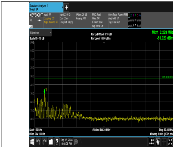
Band66_3MHz_16QAM_132322_1RB#0_0.15~30_0.15~30
