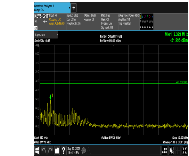
Band66_3MHz_QPSK_132322_1RB#0_0.15-30_0.15-30
