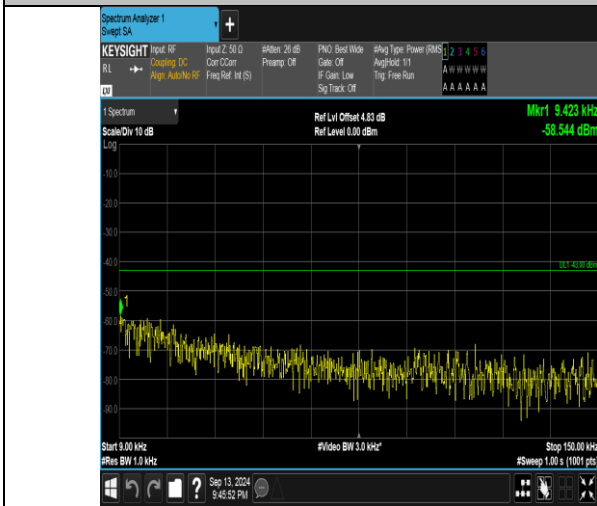
Band66_3MHz_QPSK_132322_1RB#14_0.009~0.15_0.009~0.15
