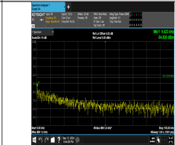
Band66_3MHz_16QAM_132322_1RB#0_0.009-0.15_0.009-0.15
