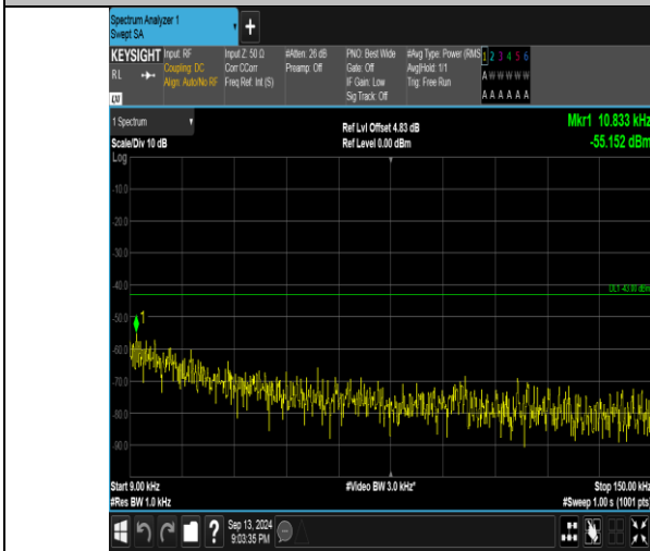
Band66_1.4MHz_QPSK_132665_6RB#0_0.009-0.15_0.009-0.15
