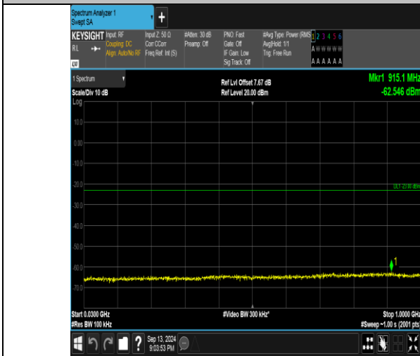
Band66_1.4MHz_QPSK_132665_6RB#0_30-1000_30-1000
