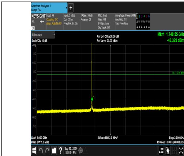
Band66_1.4MHz_16QAM_132322_1RB#5_1000-3000_1000-3000
