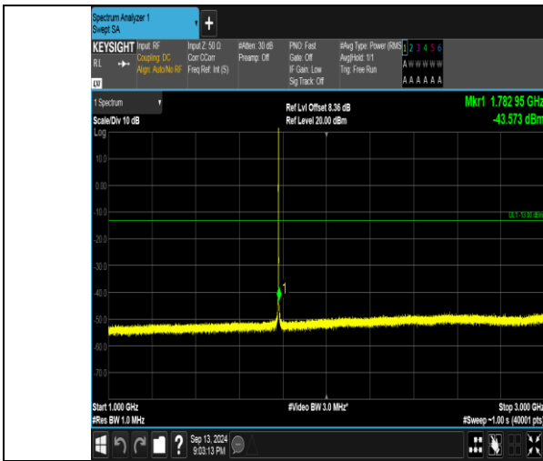
Band66_1.4MHz_16QAM_132665_1RB#5_1000-3000_1000-3000
