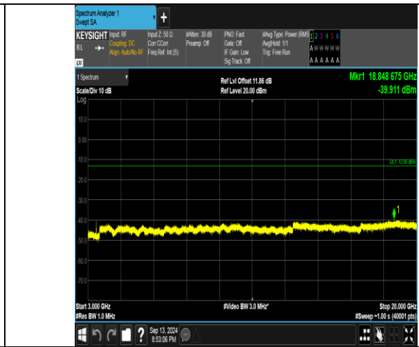
Band66_1.4MHz_16QAM_131979_1RB#5_3000-20000_3000-20000
