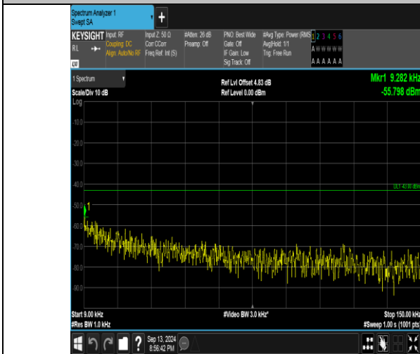
Band66_1.4MHz_QPSK_132322_1RB#5_0.009-0.15_0.009-0.15
