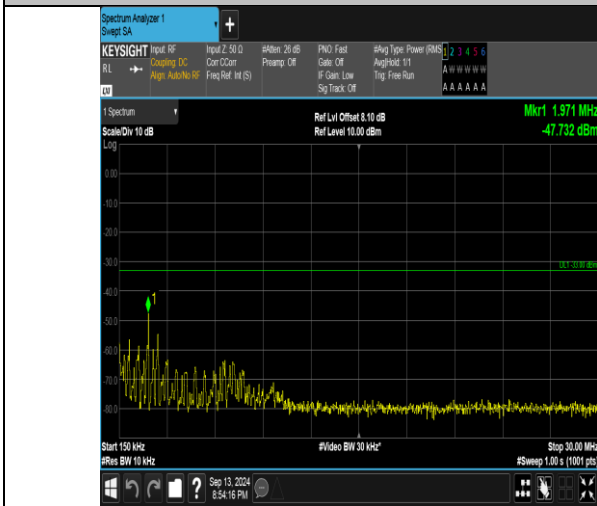
Band66_1.4MHz_16QAM_131979_6RB#0_0.15~30_0.15~30
