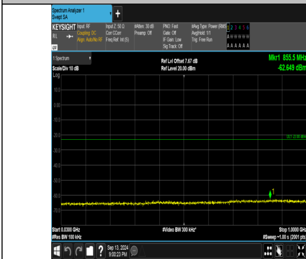
Band66_1.4MHz_QPSK_132665_1RB#0_30~1000_30~1000
