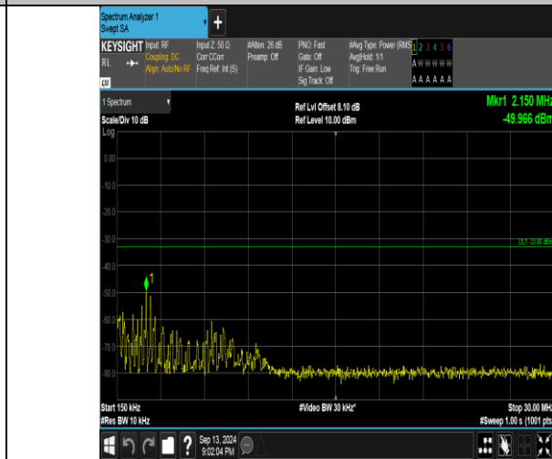
Band66_1.4MHz_QPSK_132665_1RB#5_0.15-30_0.15-30
