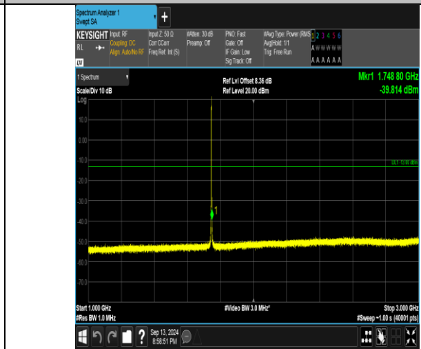
Band66_1.4MHz_QPSK_132322_6RB#0_1000-3000_1000-3000
