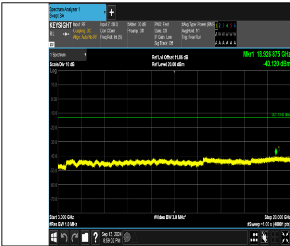
Band66_1.4MHz_QPSK_132322_6RB#0_3000~20000_3000~20000
