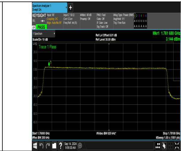
Band66_20MHz_16QAM_132572_100RB#0
