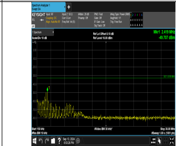
Band66_1.4MHz_QPSK_131979_6RB#0_0.15-30_0.15-30
