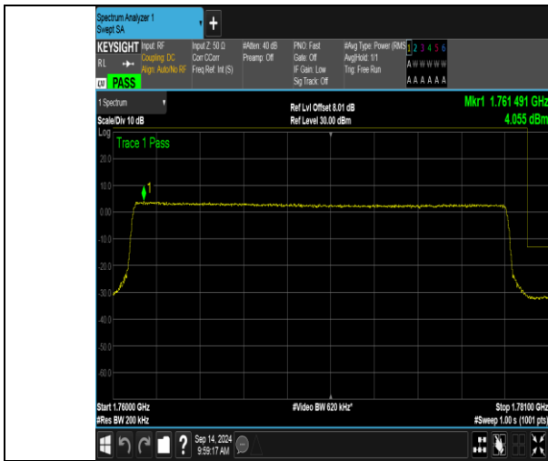
Band66_20MHz_QPSK_132572_100RB#0
