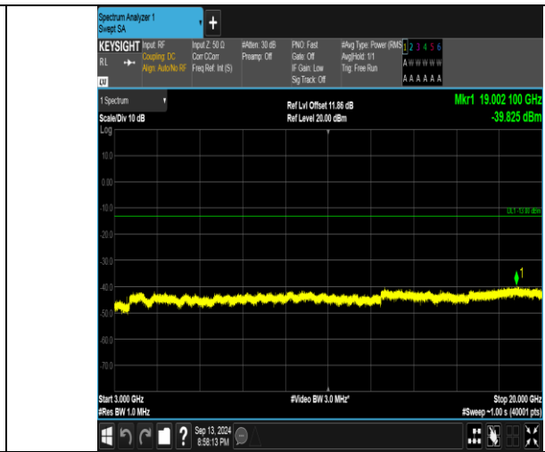
Band66_1.4MHz_16QAM_132322_1RB#5_3000-20000_3000-20000
