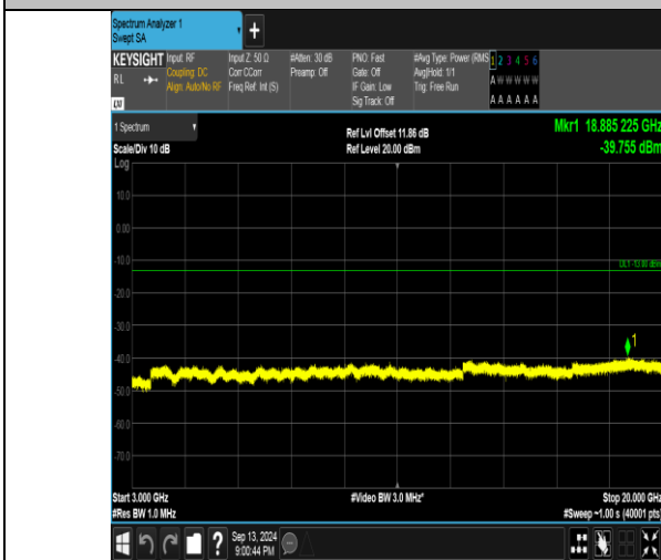
Band66_1.4MHz_QPSK_132665_1RB#0_3000~20000_3000~20000
