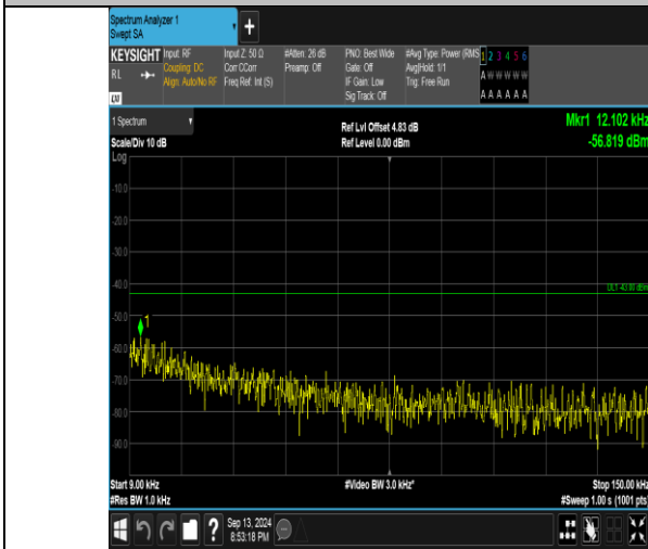
Band66_1.4MHz_QPSK_131979_6RB#0_0.009-0.15_0.009-0.15
