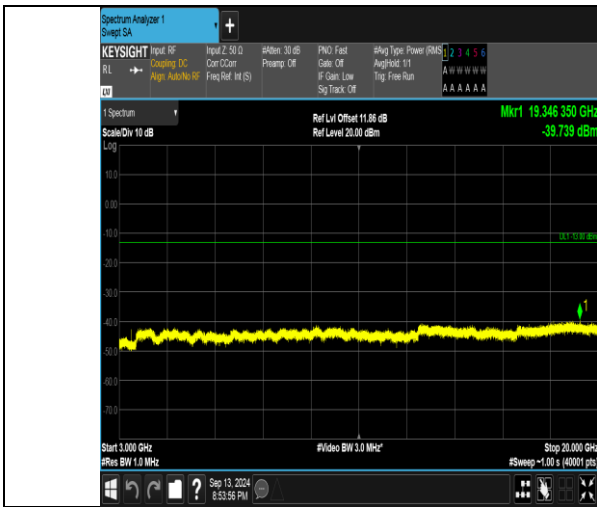
Band66_1.4MHz_QPSK_131979_6RB#0_3000~20000_3000~20000
