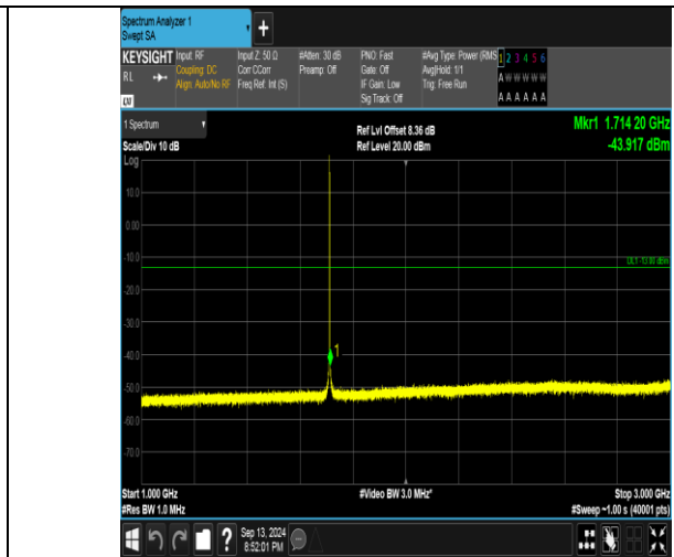
Band66_1.4MHz_QPSK_131979_1RB#5_1000~3000_1000~3000
