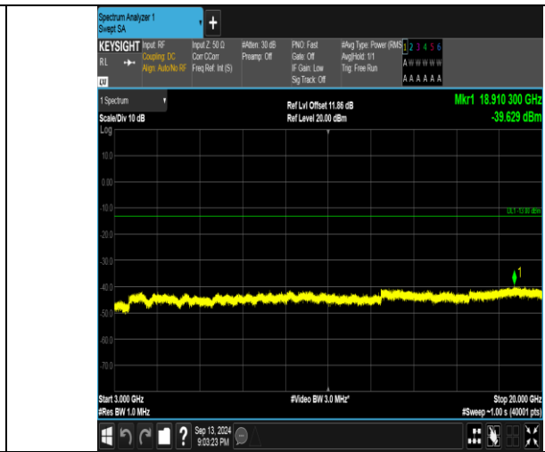
Band66_1.4MHz_16QAM_132665_1RB#5_3000-20000_3000-20000
