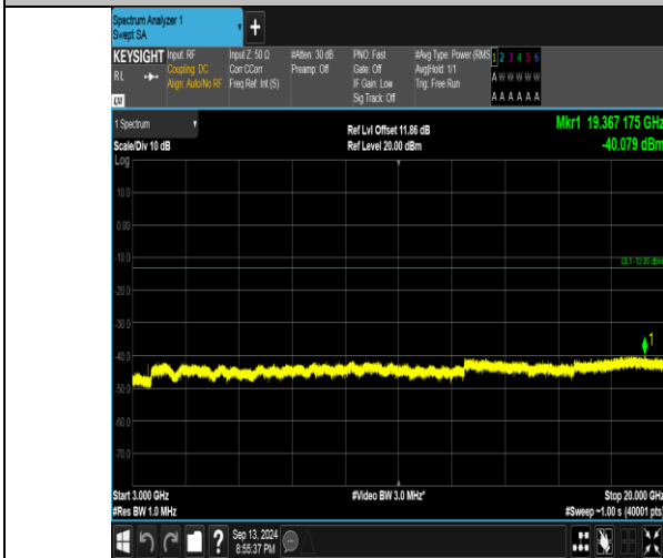
Band66_1.4MHz_QPSK_132322_1RB#0_3000~20000_3000~20000
