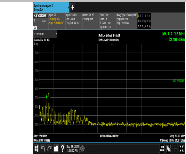
Band66_1.4MHz_QPSK_132322_6RB#0_0.15-30_0.15-30
