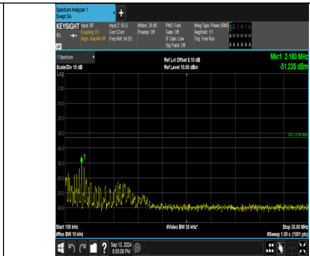
Band66_1.4MHz_QPSK_132322_1RB#0_0.15~30_0.15~30
