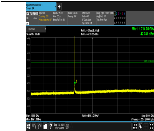
Band66_1.4MHz_16QAM_131979_1RB#5_1000-3000_1000-3000
