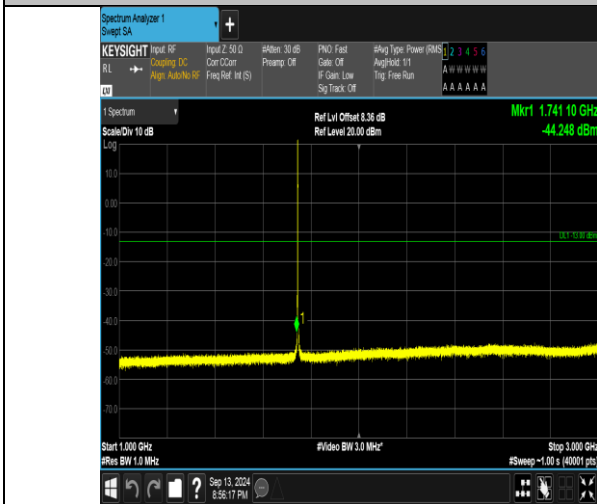
Band66_1.4MHz_16QAM_132322_1RB#0_1000-3000_1000-3000
