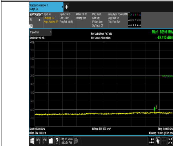
Band66_1.4MHz_QPSK_131979_6RB#0_30-1000_30-1000
