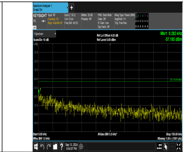
Band66_1.4MHz_16QAM_131979_6RB#0_0.009~0.15_0.009~0.15
