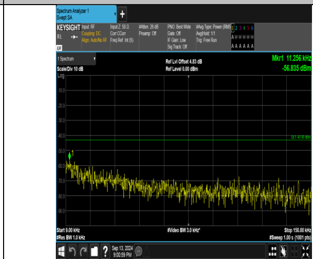
Band66_1.4MHz_16QAM_132665_1RB#0_0.009~0.15_0.009~0.15
