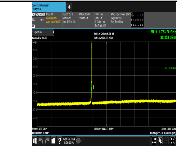
Band66_1.4MHz_QPSK_132665_6RB#0_1000-3000_1000-3000
