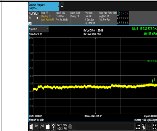
Band66_1.4MHz_16QAM_132665_1RB#0_3000-20000_3000-20000
