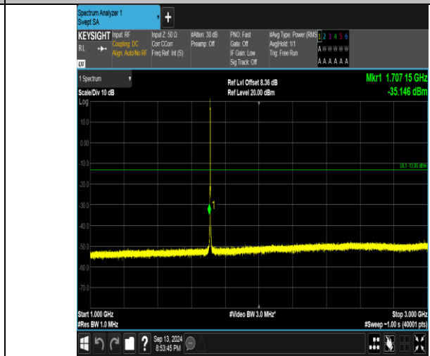
Band66_1.4MHz_QPSK_131979_6RB#0_1000-3000_1000-3000
