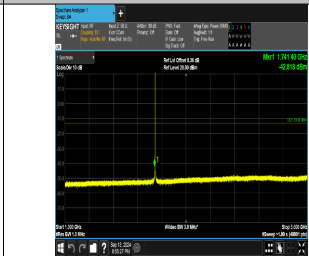
Band66_1.4MHz_QPSK_132322_1RB#0_1000~3000_1000~3000
