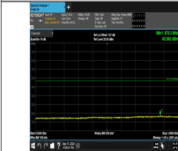
Band66_1.4MHz_QPSK_132322_6RB#0_30-1000_30-1000
