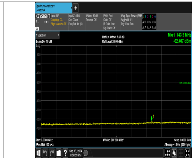
Band66_1.4MHz_16QAM_131979_1RB#0_30-1000_30-1000
