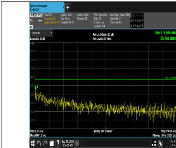
Band66_1.4MHz_QPSK_132322_1RB#0_0.009~0.15_0.009~0.15
