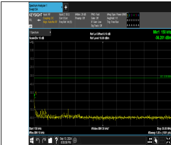
Band66_1.4MHz_16QAM_132322_1RB#0_0.15-30_0.15-30
