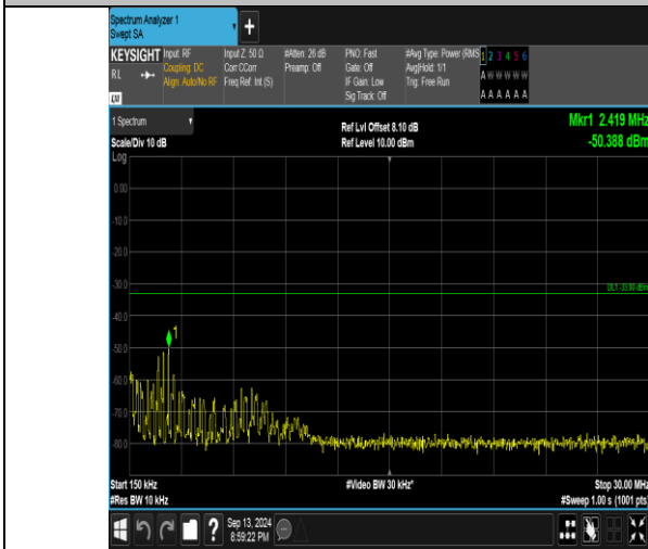
Band66_1.4MHz_16QAM_132322_6RB#0_0.15~30_0.15~30
