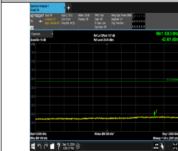
Band66_1.4MHz_QPSK_132322_1RB#0_30~1000_30~1000
