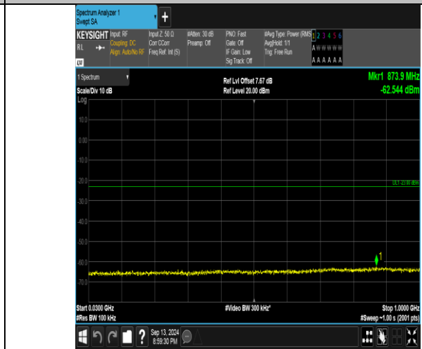
Band66_1.4MHz_16QAM_132322_6RB#0_30~1000_30~1000
