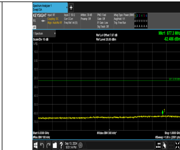
Band66_1.4MHz_16QAM_132665_1RB#0_30-1000_30-1000
