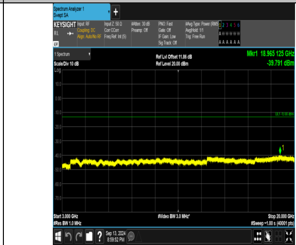
Band66_1.4MHz_16QAM_132322_6RB#0_3000~20000_3000~20000
