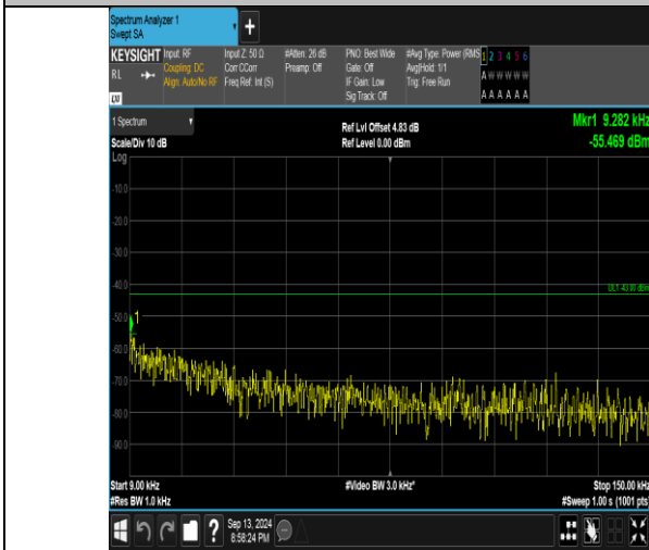
Band66_1.4MHz_QPSK_132322_6RB#0_0.009-0.15_0.009-0.15
