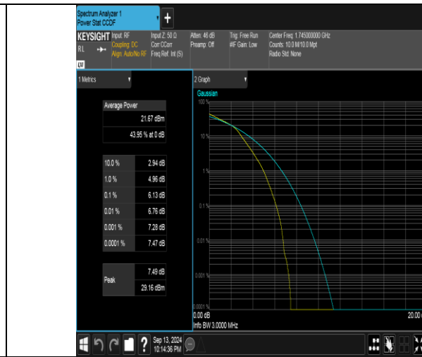
Band66-3MHz-16QAM-132322-15RB#0-PASS
