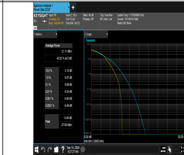
Band66-1.4MHz-16QAM-132665-6RB#0-PASS
