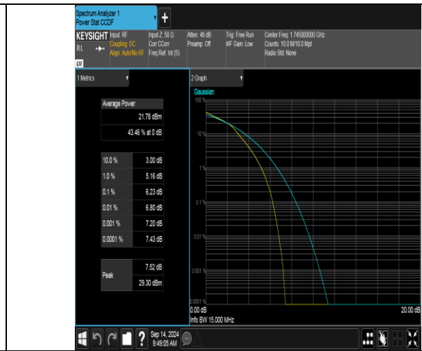
Band66-15MHz-16QAM-132322-75RB#0-PASS
