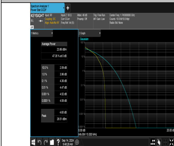
Band66-15MHz-QPSK-132322-1RB#0-PASS
