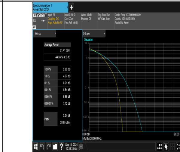
Band66-20MHz-16QAM-132572-100RB#0-PASS
