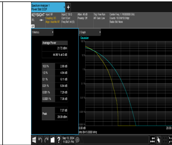
Band66-5MHz-16QAM-132322-25RB#0-PASS
