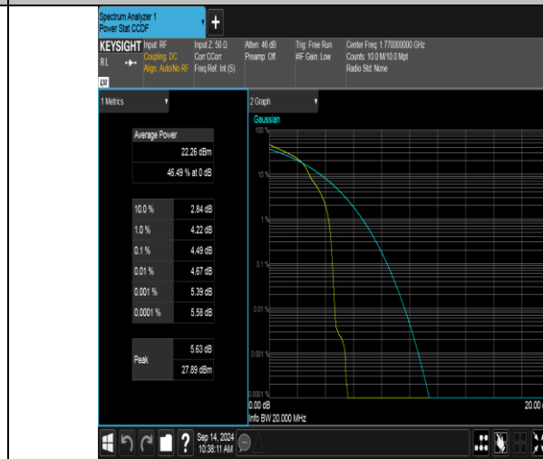
Band66-20MHz-16QAM-132572-1RB#0-PASS
