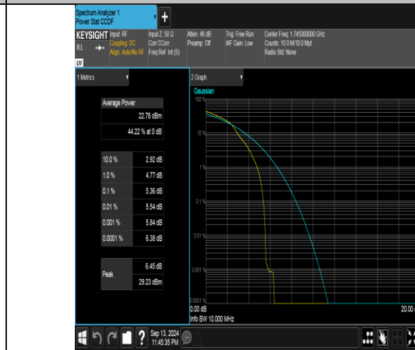
Band66-10MHz-16QAM-132322-1RB#0-PASS
