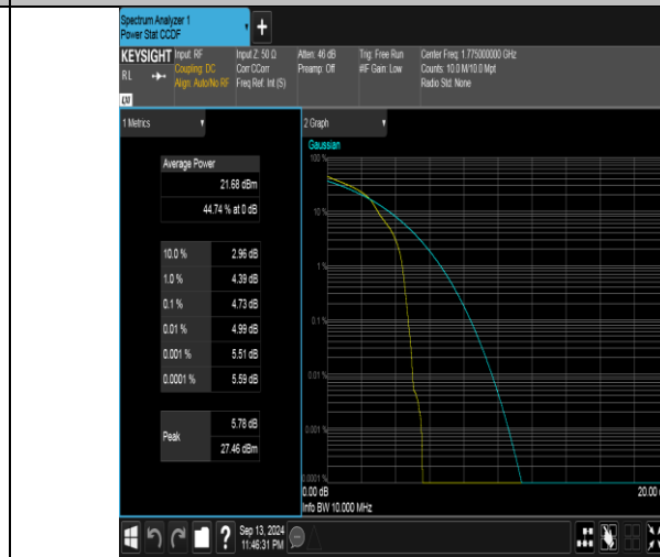
Band66-10MHz-16QAM-132622-1RB#0-PASS
