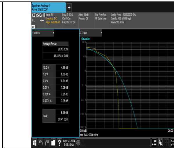
Band66-1.4MHz-16QAM-132665-1RB#0-PASS
