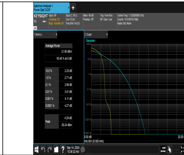
Band66-20MHz-16QAM-132072-1RB#0-PASS
