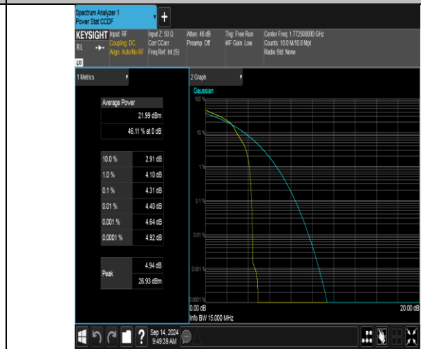
Band66-15MHz-16QAM-132597-1RB#0-PASS
