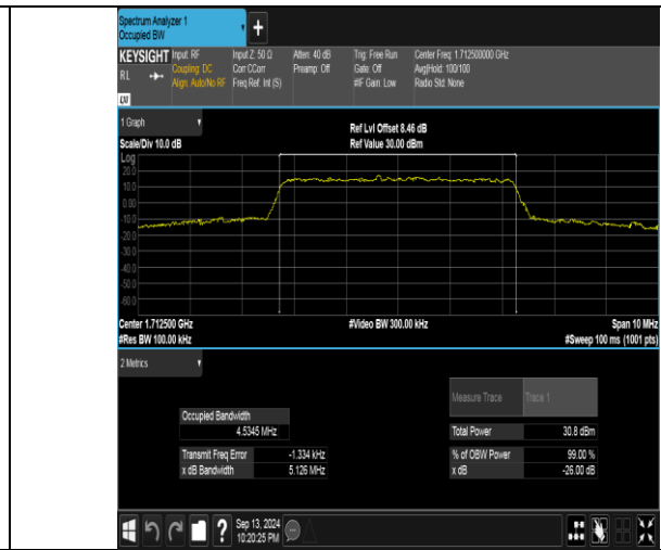
Band66-5MHz-16QAM-131997-25RB#0-PASS
