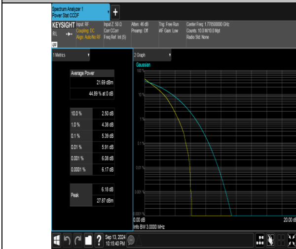
Band66-3MHz-QPSK-132657-15RB#0-PASS
