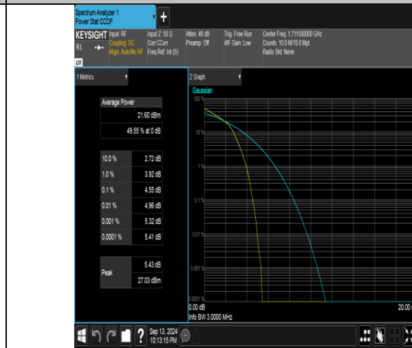
Band66-3MHz-16QAM-131987-15RB#0-PASS
