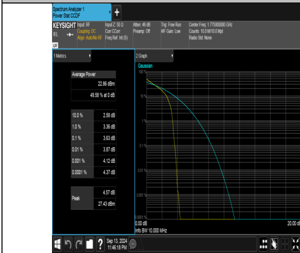
Band66-10MHz-QPSK-132622-1RB#0-PASS
