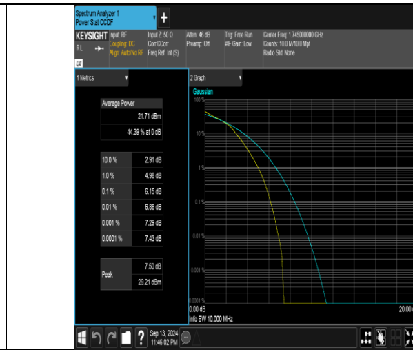
Band66-10MHz-16QAM-132322-50RB#0-PASS
