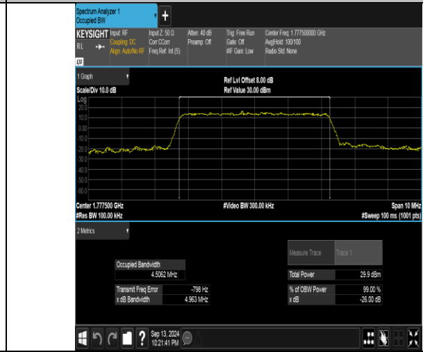
Band66-5MHz-16QAM-132647-25RB#0-PASS
