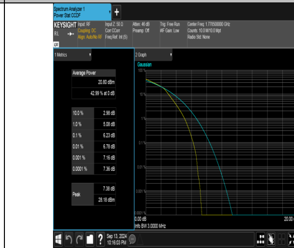
Band66-3MHz-16QAM-132657-15RB#0-PASS
