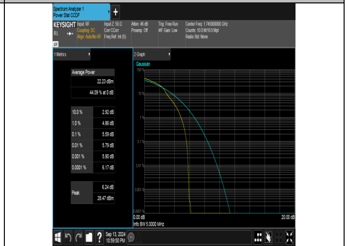
Band66-5MHz-16QAM-132322-1RB#0-PASS
