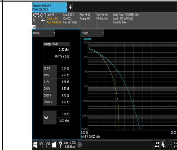
Band66-1.4MHz-16QAM-132322-6RB#0-PASS
