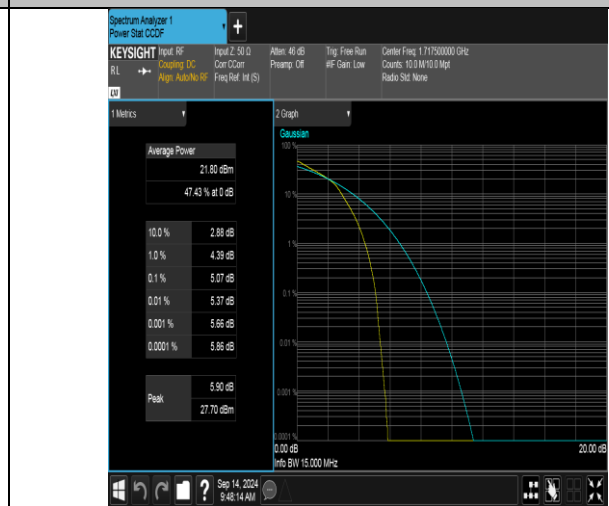
Band66-15MHz-16QAM-132047-75RB#0-PASS
