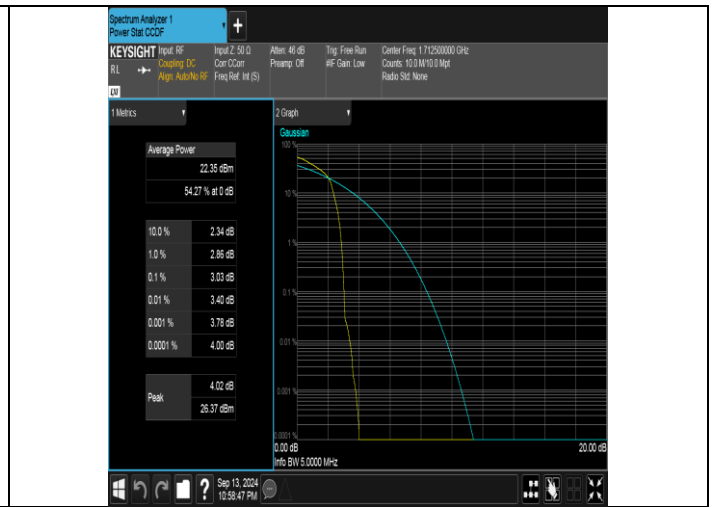
Band66-5MHz-16QAM-131997-1RB#0-PASS
