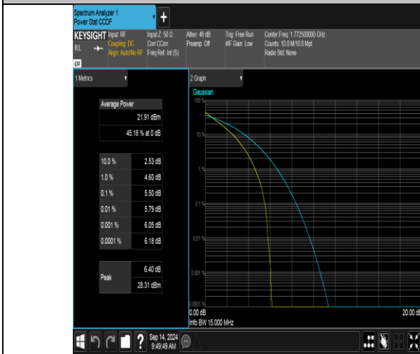
Band66-15MHz-QPSK-132597-75RB#0-PASS
