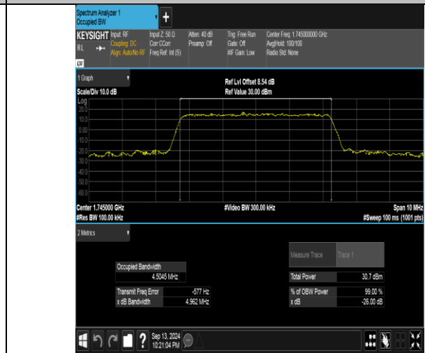
Band66-5MHz-16QAM-132322-25RB#0-PASS
