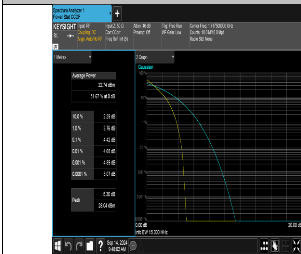
Band66-15MHz-QPSK-132047-75RB#0-PASS
