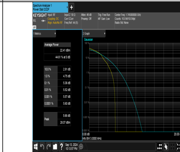
Band66-3MHz-16QAM-132322-1RB#0-PASS
