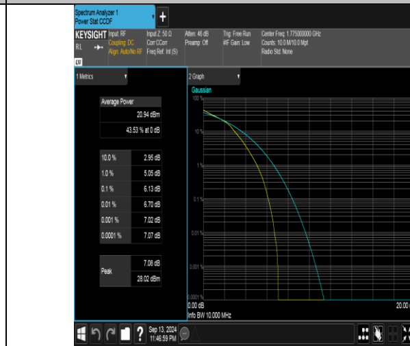
Band66-10MHz-16QAM-132622-50RB#0-PASS
