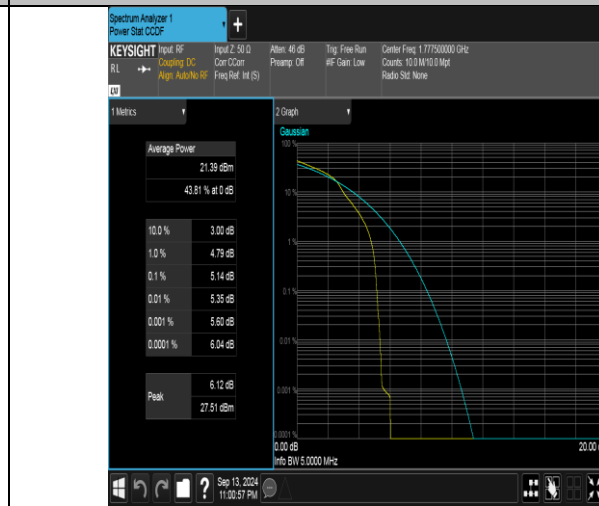
Band66-5MHz-16QAM-132647-1RB#0-PASS
