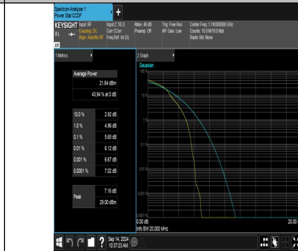
Band66-20MHz-16QAM-132322-1RB#0-PASS
