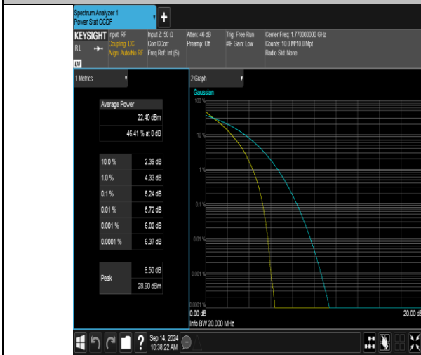
Band66-20MHz-QPSK-132572-100RB#0-PASS
