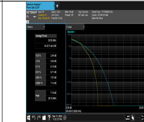
Band66-5MHz-16QAM-132647-25RB#0-PASS
