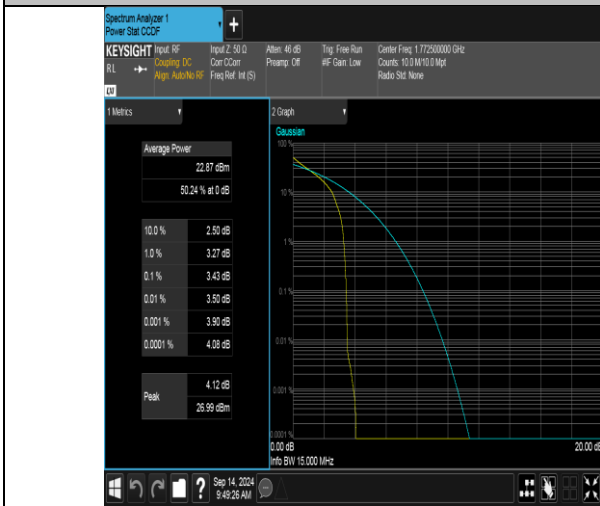
Band66-15MHz-QPSK-132597-1RB#0-PASS
