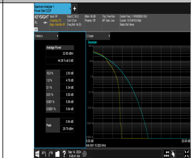
Band66-15MHz-16QAM-132322-1RB#0-PASS
