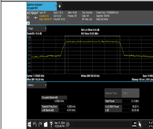
Band66-5MHz-QPSK-132322-25RB#0-PASS
