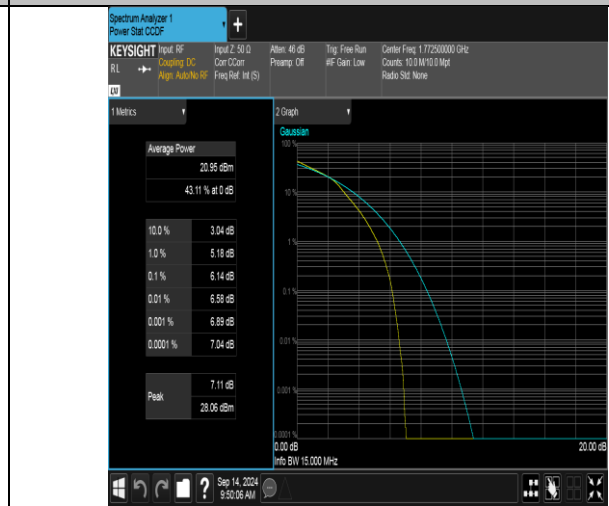
Band66-15MHz-16QAM-132597-75RB#0-PASS
