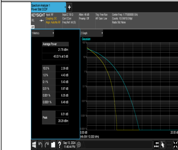
Band66-10MHz-QPSK-132622-50RB#0-PASS
