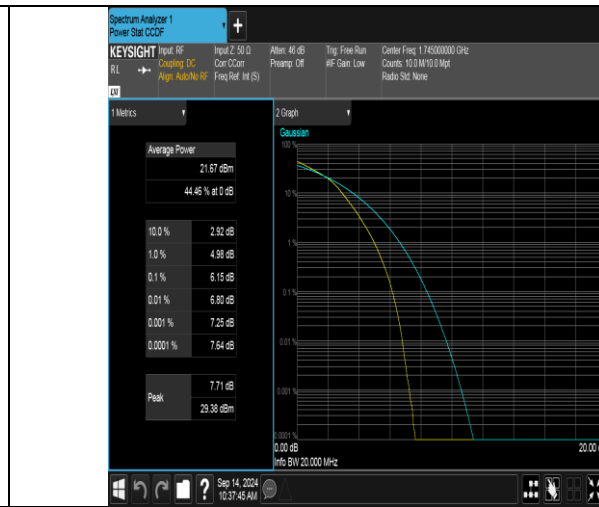
Band66-20MHz-16QAM-132322-100RB#0-PASS
