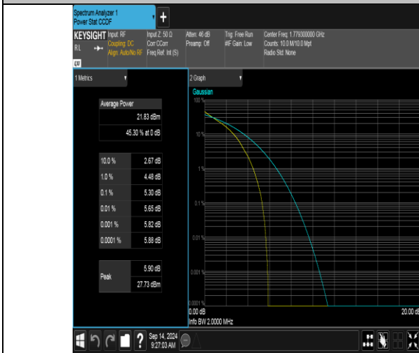
Band66-1.4MHz-QPSK-132665-6RB#0-PASS
