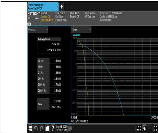
Band66-5MHz-QPSK-131997-1RB#0-PASS
