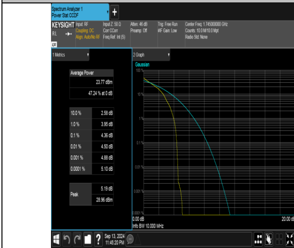
Band66-10MHz-QPSK-132322-1RB#0-PASS
