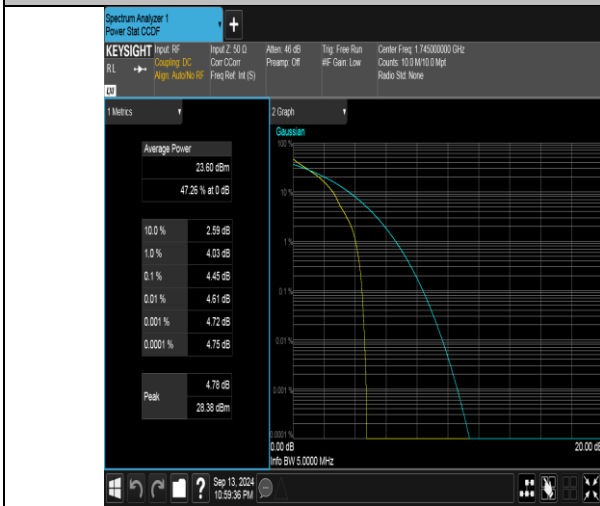
Band66-5MHz-QPSK-132322-1RB#0-PASS
