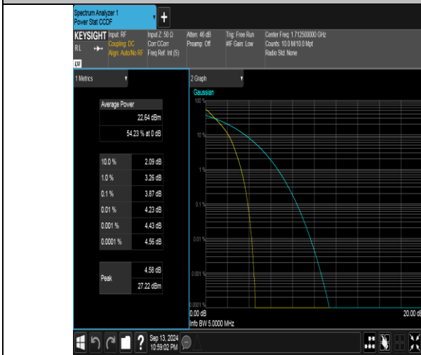
Band66-5MHz-QPSK-131997-25RB#0-PASS
