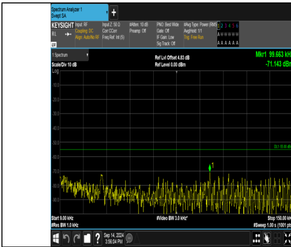
Band41_20MHz_QPSK_41140_100RB#0_0.009-0.15_0.009-0.15
