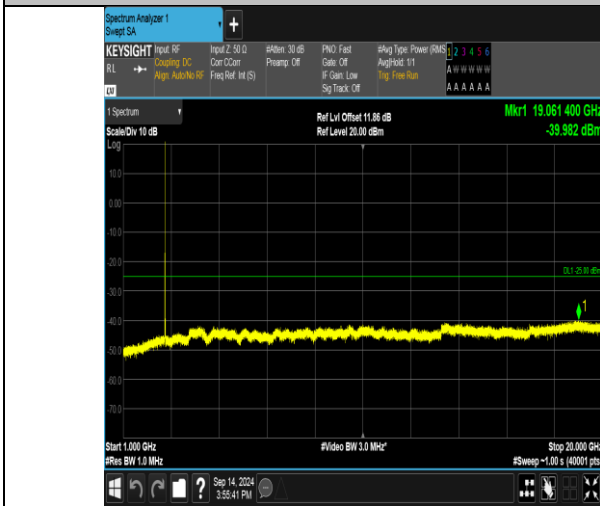
Band41_20MHz_16QAM_41140_1RB#99_1000~20000_1000~20000
