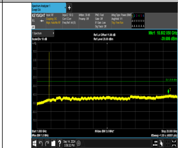
Band41_20MHz_QPSK_41140_100RB#0_1000-20000_1000-20000
