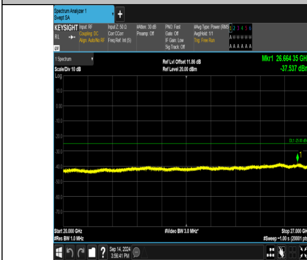
Band41_20MHz_QPSK_41140_100RB#0_20000-27000_20000-27000
