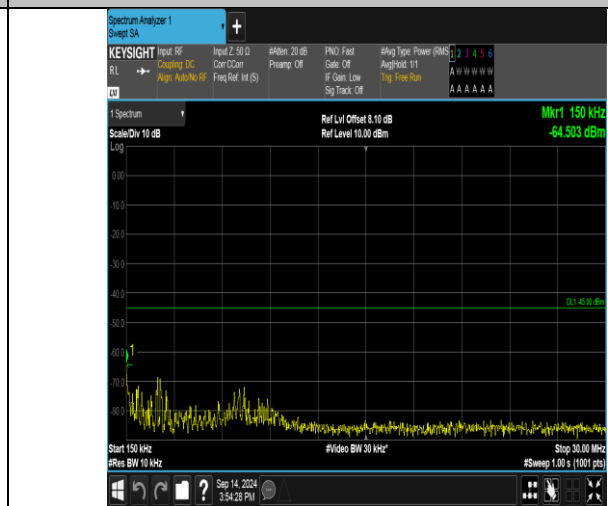
Band41_20MHz_QPSK_41140_1RB#99_0.15~30_0.15~30
