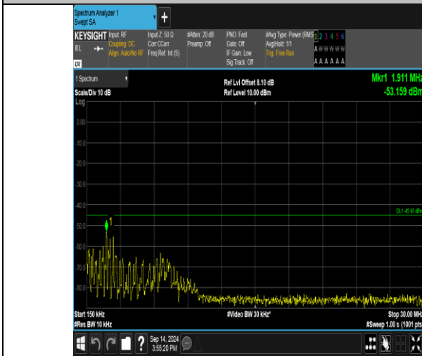
Band41_20MHz_16QAM_41140_1RB#99_0.15~30_0.15~30
