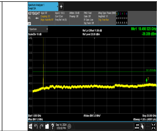
Band41_20MHz_QPSK_41140_1RB#0_1000~20000_1000~20000
