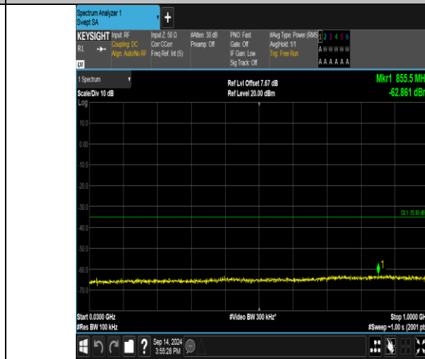
Band41_20MHz_16QAM_41140_1RB#99_30~1000_30~1000
