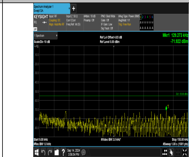
Band41_20MHz_16QAM_41140_100RB#0_0.009-0.15_0.009-0.15
