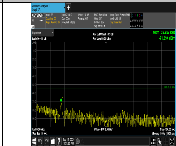
Band41_20MHz_16QAM_41140_1RB#0_0.009~0.15_0.009~0.15
