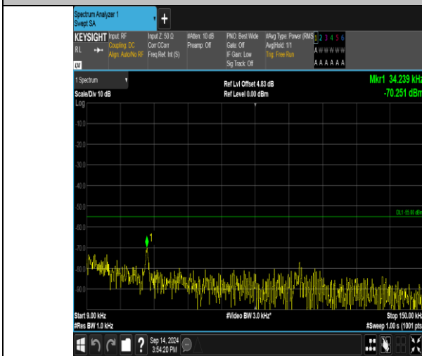
Band41_20MHz_QPSK_41140_1RB#99_0.009~0.15_0.009~0.15
