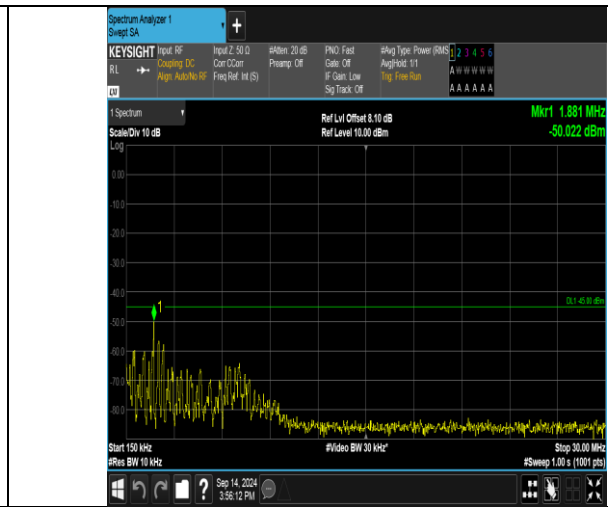
Band41_20MHz_QPSK_41140_100RB#0_0.15-30_0.15-30
