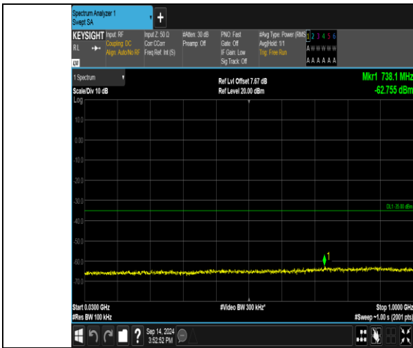
Band41_20MHz_QPSK_41140_1RB#0_30~1000_30~1000
