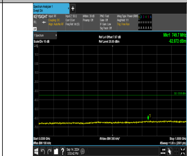
Band41_20MHz_16QAM_41140_1RB#0_30~1000_30~1000
