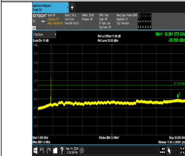
Band41_15MHz_16QAM_41165_1RB#74_1000~20000_1000~20000
