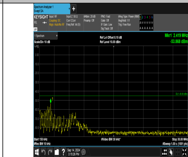
Band41_15MHz_QPSK_41165_1RB#74_0.15~30_0.15~30
