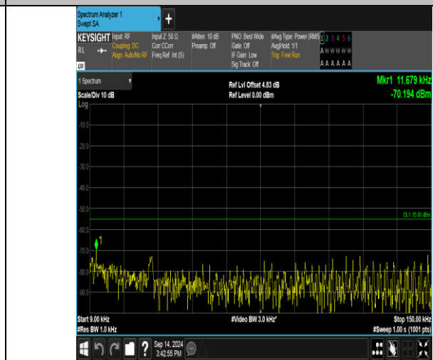
Band41_20MHz_16QAM_40140_1RB#0_0.009~0.15_0.009~0.15
