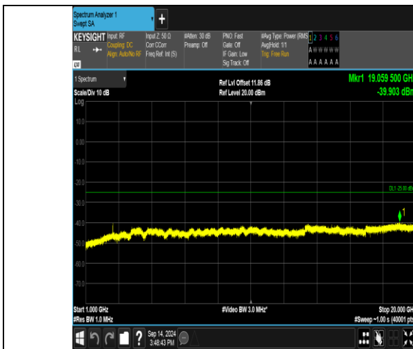
Band41_20MHz_16QAM_40590_1RB#0_1000~20000_1000~20000
