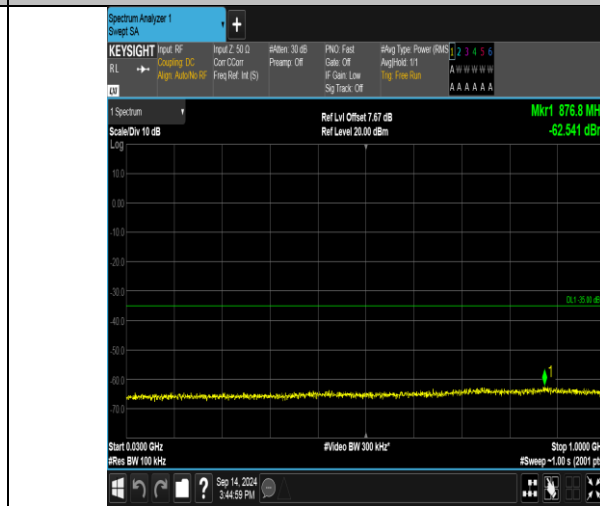
Band41_20MHz_16QAM_40140_1RB#99_30~1000_30~1000
