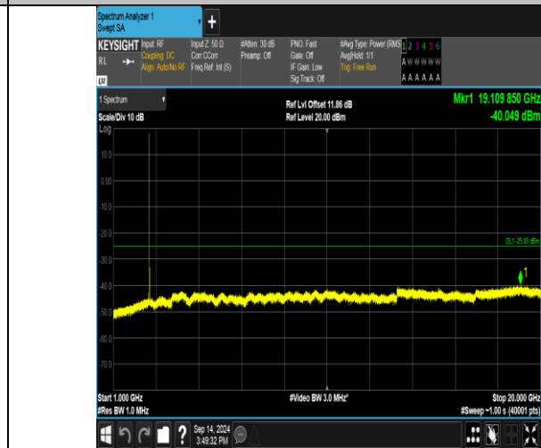
Band41_20MHz_QPSK_40590_1RB#99_1000~20000_1000~20000
