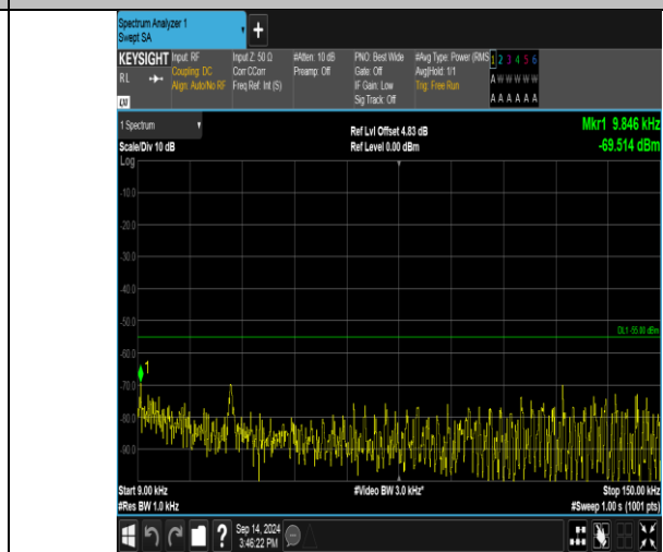
Band41_20MHz_16QAM_40140_100RB#0_0.009-0.15_0.009-0.15
