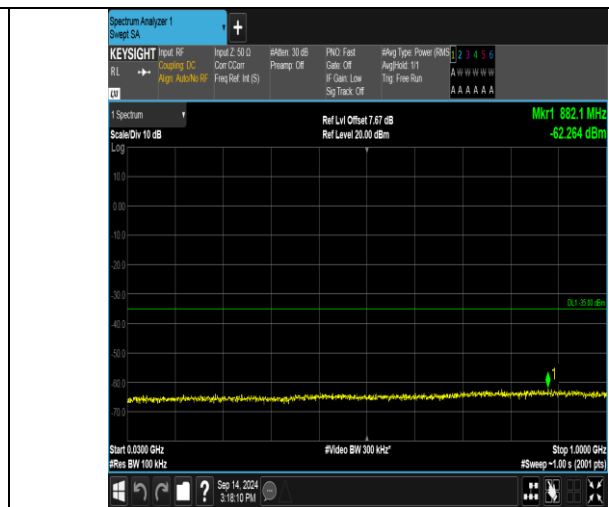
Band41_15MHz_16QAM_41165_75RB#0_30~1000_30~1000
