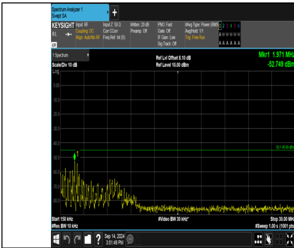
Band41_20MHz_16QAM_40590_100RB#0_0.15~30_0.15~30
