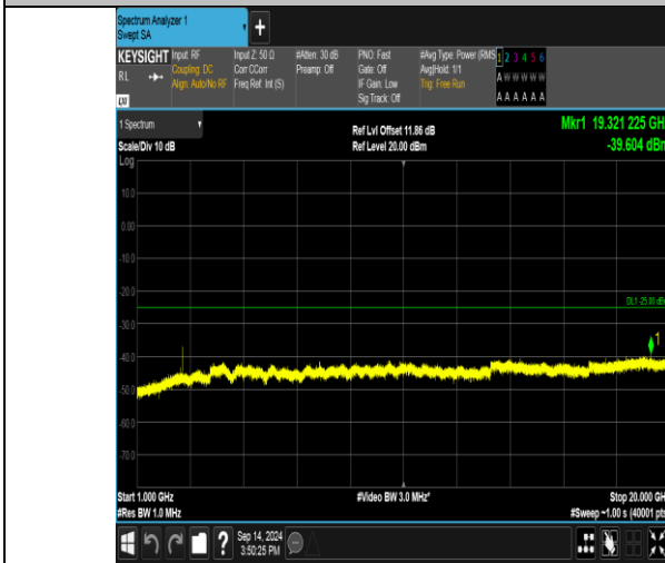
Band41_20MHz_16QAM_40590_1RB#99_1000~20000_1000~20000
