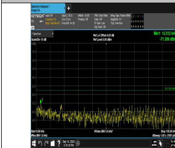
Band41_15MHz_QPSK_41165_1RB#74_0.009~0.15_0.009~0.15
