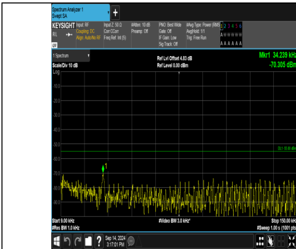
Band41_15MHz_QPSK_41165_75RB#0_0.009-0.15_0.009-0.15
