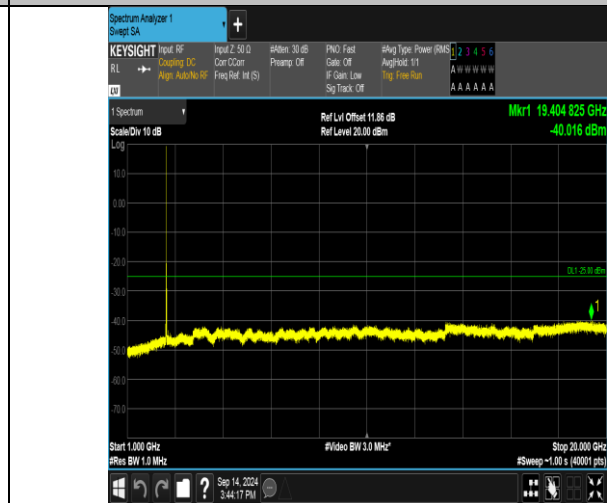
Band41_20MHz_QPSK_40140_1RB#99_1000~20000_1000~20000
