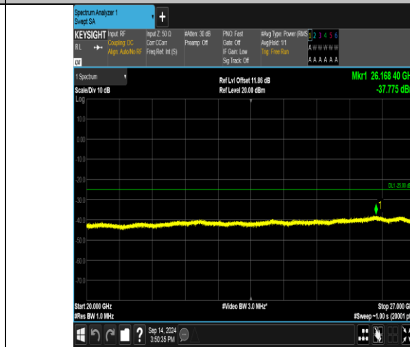
Band41_20MHz_16QAM_40590_1RB#99_20000~27000_20000~27000
