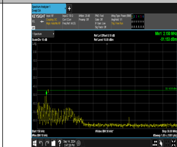
Band41_20MHz_QPSK_40590_1RB#0_0.15~30_0.15~30
