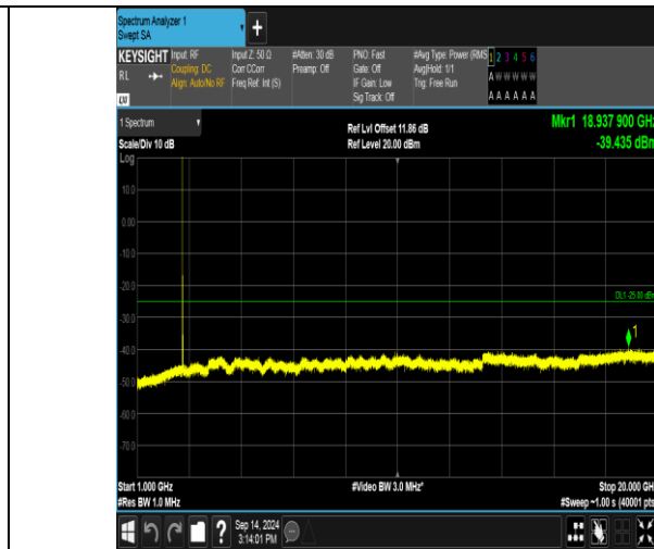
Band41_15MHz_QPSK_41165_1RB#0_1000~20000_1000~20000
