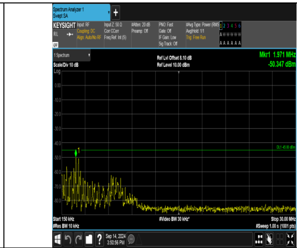
Band41_20MHz_QPSK_40590_100RB#0_0.15-30_0.15-30
