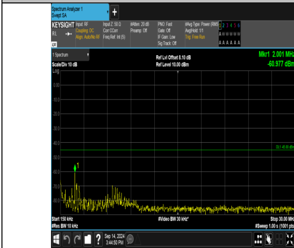
Band41_20MHz_16QAM_40140_1RB#99_0.15~30_0.15~30
