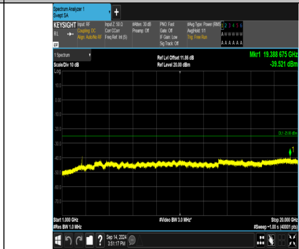
Band41_20MHz_QPSK_40590_100RB#0_1000-20000_1000-20000
