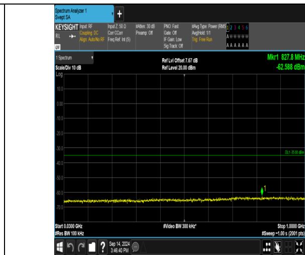
Band41_20MHz_16QAM_40140_100RB#0_30~1000_30~1000
