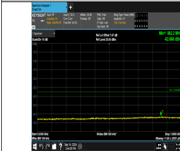
Band41_20MHz_QPSK_40140_1RB#99_30~1000_30~1000
