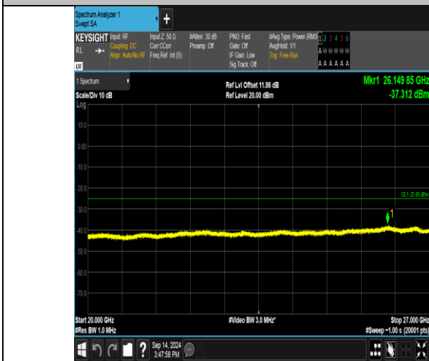
Band41_20MHz_QPSK_40590_1RB#0_20000~27000_20000~27000
