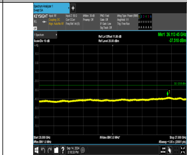
Band41_15MHz_16QAM_41165_75RB#0_20000~27000_20000~27000
