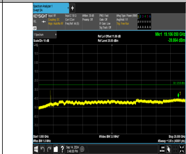
Band41_20MHz_QPSK_40140_100RB#0_1000-20000_1000-20000
