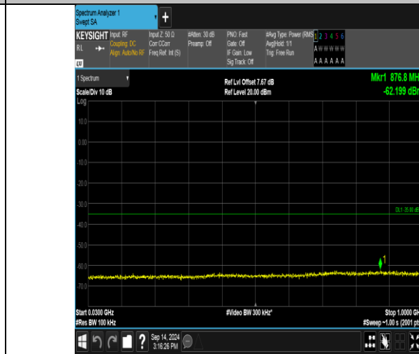
Band41_15MHz_16QAM_41165_1RB#74_30~1000_30~1000
