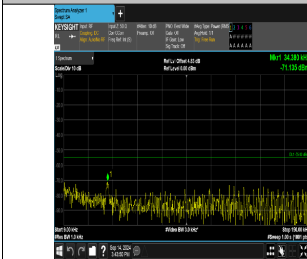
Band41_20MHz_QPSK_40140_1RB#99_0.009~0.15_0.009~0.15
