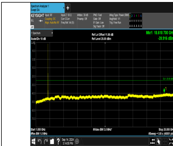
Band41_15MHz_16QAM_41165_1RB#0_1000~20000_1000~20000
