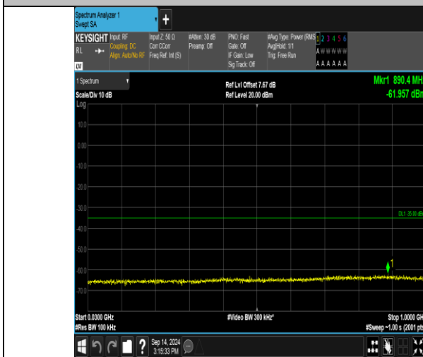
Band41_15MHz_QPSK_41165_1RB#74_30~1000_30~1000
