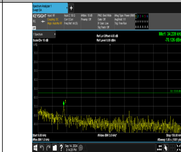
Band41_15MHz_16QAM_41165_1RB#0_0.009~0.15_0.009~0.15
