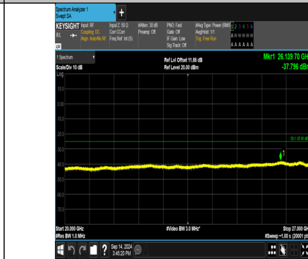
Band41_20MHz_16QAM_40140_1RB#99_20000~27000_20000~27000
