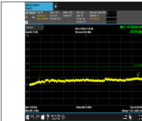
Band41_20MHz_16QAM_40140_1RB#0_1000~20000_1000~20000
