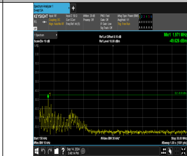
Band41_20MHz_QPSK_40590_1RB#99_0.15~30_0.15~30
