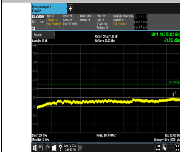
Band41_20MHz_16QAM_40140_100RB#0_1000~20000_1000~20000
