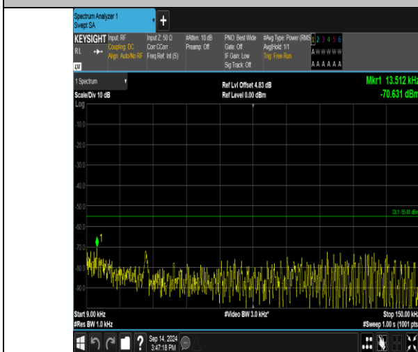
Band41_20MHz_QPSK_40590_1RB#0_0.009~0.15_0.009~0.15
