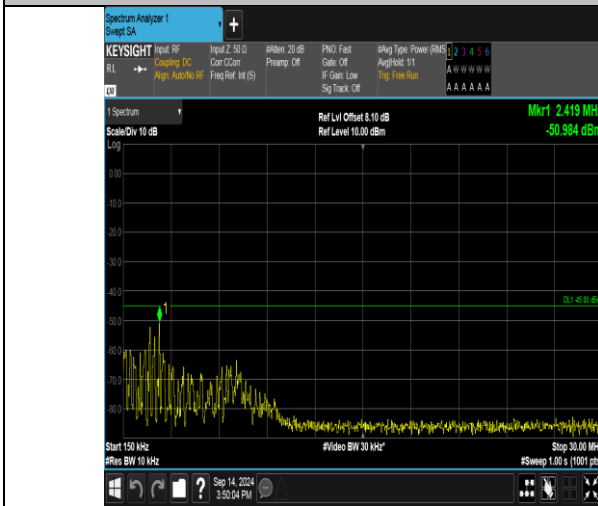
Band41_20MHz_16QAM_40590_1RB#99_0.15~30_0.15~30
