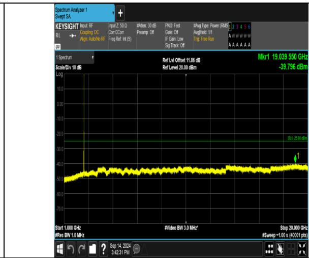
Band41_20MHz_QPSK_40140_1RB#0_1000~20000_1000~20000
