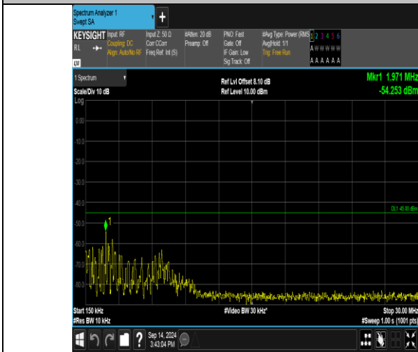
Band41_20MHz_16QAM_40140_1RB#0_0.15~30_0.15~30
