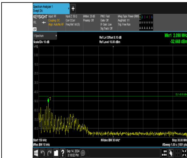
Band41_15MHz_16QAM_41165_75RB#0_0.15~30_0.15~30
