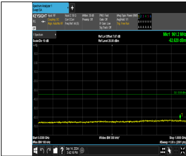
Band41_20MHz_QPSK_40140_1RB#0_30~1000_30~1000
