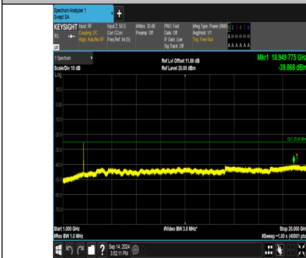
Band41_20MHz_16QAM_40590_100RB#0_1000~20000_1000~20000
