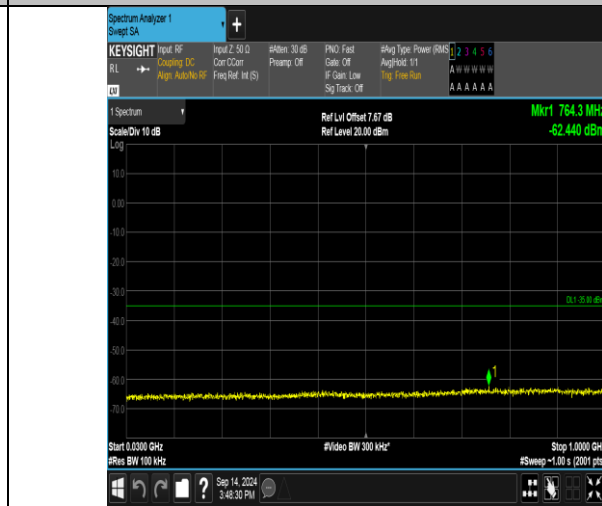
Band41_20MHz_16QAM_40590_1RB#0_30~1000_30~1000
