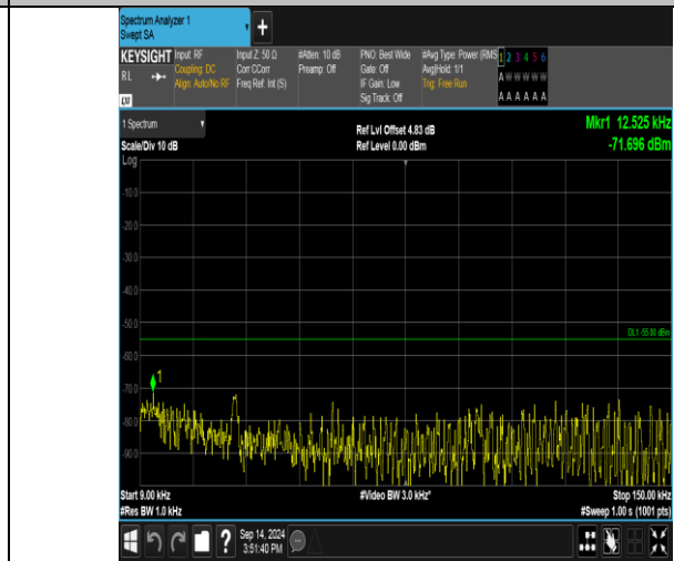
Band41_20MHz_16QAM_40590_100RB#0_0.009-0.15_0.009-0.15
