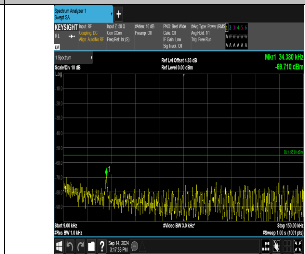
Band41_15MHz_16QAM_41165_75RB#0_0.009-0.15_0.009-0.15
