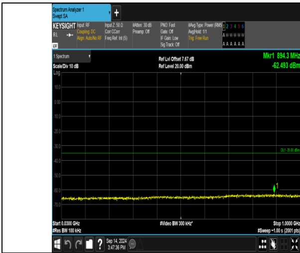
Band41_20MHz_QPSK_40590_1RB#0_30~1000_30~1000
