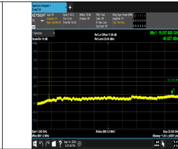
Band41_20MHz_QPSK_40590_1RB#0_1000~20000_1000~20000
