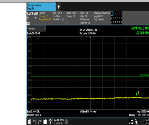
Band41_15MHz_16QAM_41165_1RB#0_30~1000_30~1000
