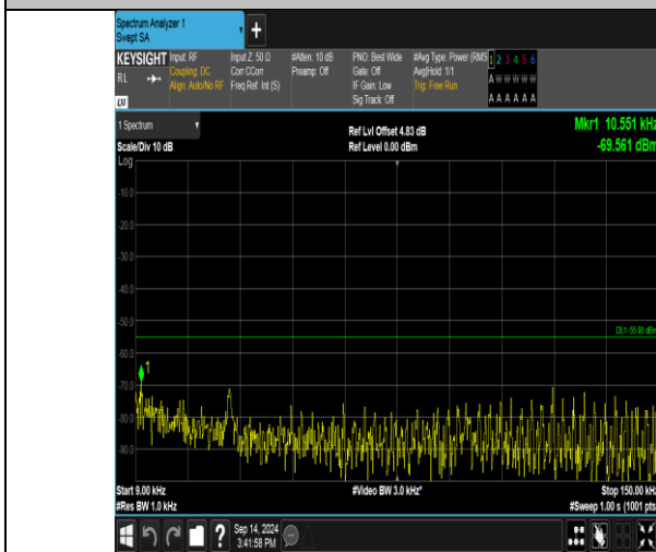
Band41_20MHz_QPSK_40140_1RB#0_0.009~0.15_0.009~0.15
