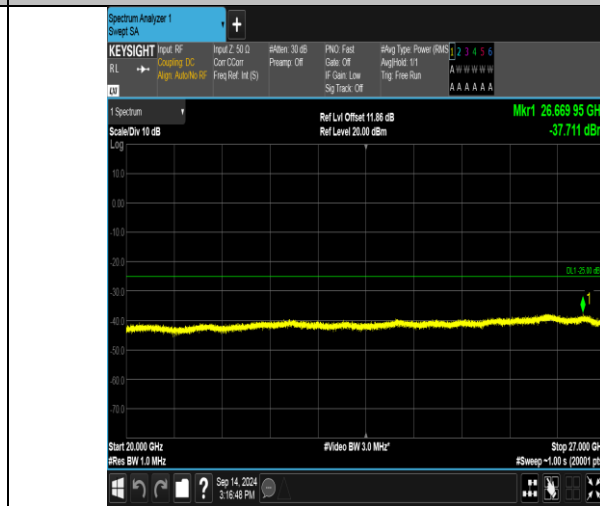
Band41_15MHz_16QAM_41165_1RB#74_20000~27000_20000~27000
