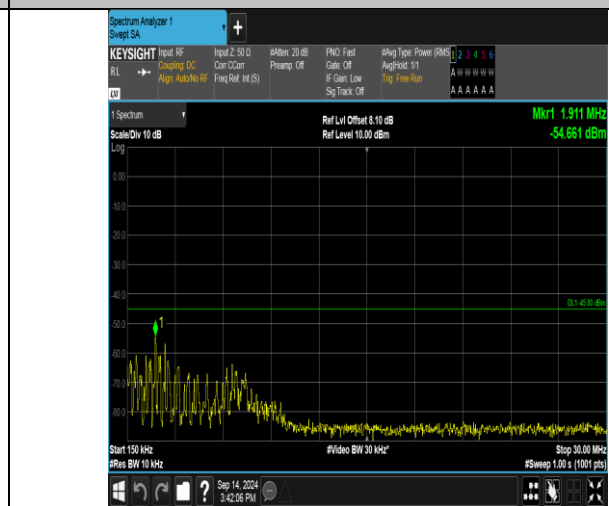
Band41_20MHz_QPSK_40140_1RB#0_0.15~30_0.15~30
