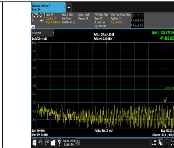
Band41_20MHz_16QAM_40590_1RB#99_0.009~0.15_0.009~0.15
