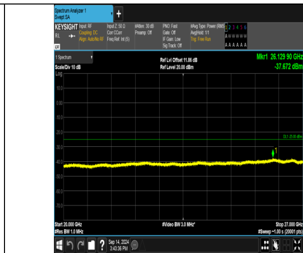
Band41_20MHz_16QAM_40140_1RB#0_20000~27000_20000~27000
