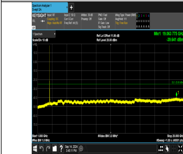
Band41_20MHz_16QAM_40140_1RB#99_1000~20000_1000~20000
