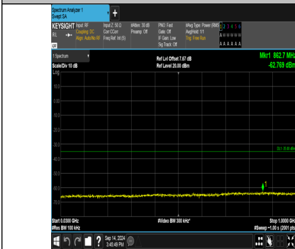
Band41_20MHz_QPSK_40140_100RB#0_30-1000_30-1000
