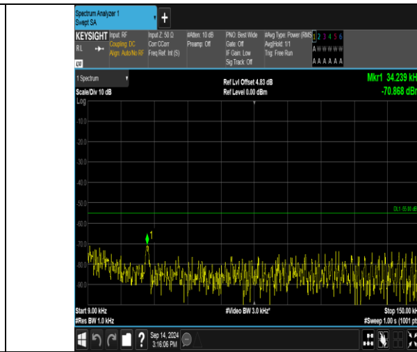
Band41_15MHz_16QAM_41165_1RB#74_0.009~0.15_0.009~0.15
