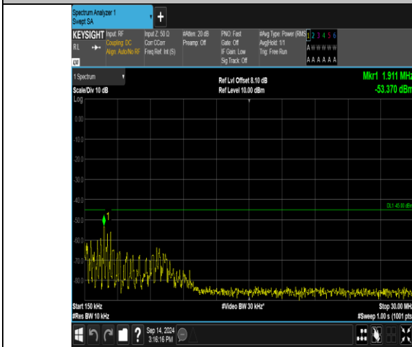
Band41_15MHz_16QAM_41165_1RB#74_0.15~30_0.15~30
