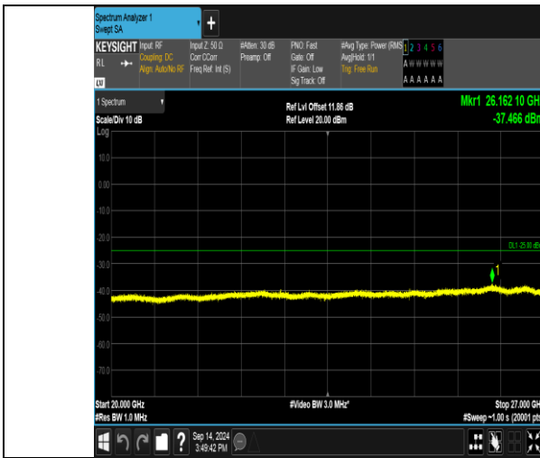
Band41_20MHz_QPSK_40590_1RB#99_20000~27000_20000~27000
