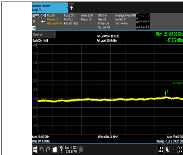
Band41_15MHz_QPSK_41165_1RB#74_20000~27000_20000~27000
