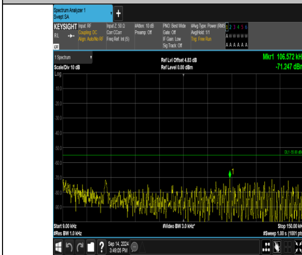
Band41_20MHz_QPSK_40590_1RB#99_0.009~0.15_0.009~0.15
