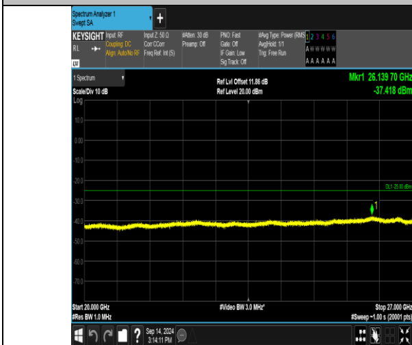
Band41_15MHz_QPSK_41165_1RB#0_20000~27000_20000~27000
