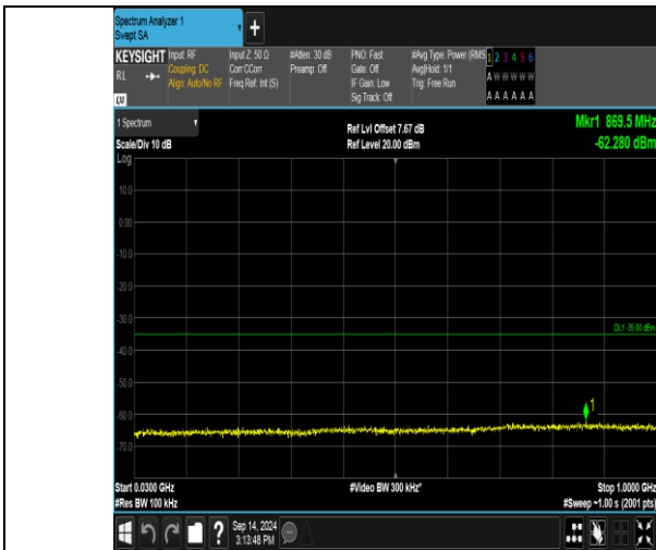
Band41_15MHz_QPSK_41165_1RB#0_30~1000_30~1000
