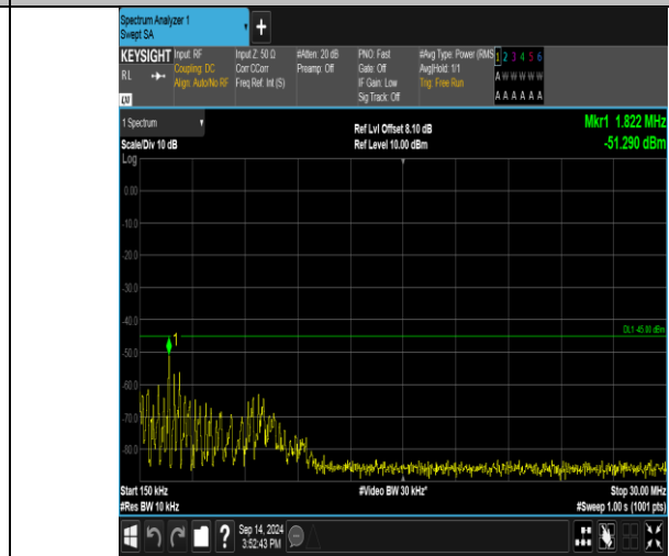
Band41_20MHz_QPSK_41140_1RB#0_0.15~30_0.15~30
