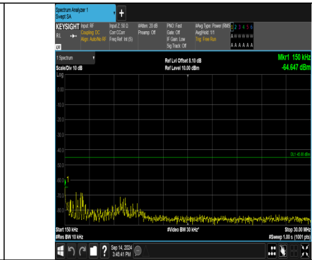
Band41_20MHz_QPSK_40140_100RB#0_0.15-30_0.15-30
