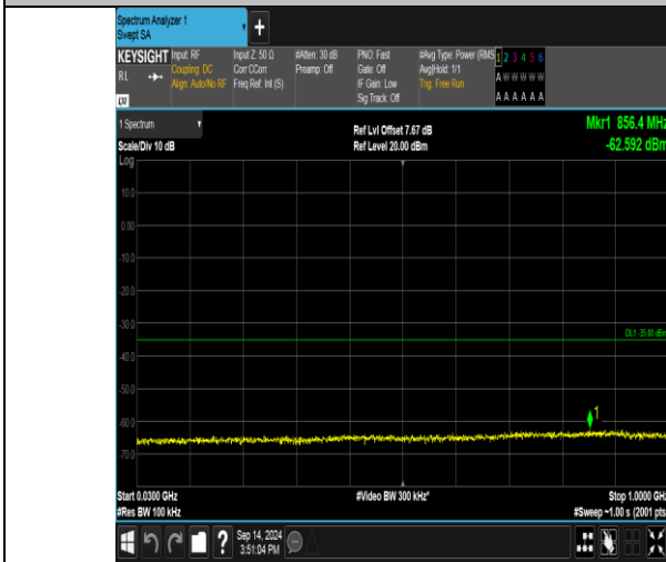
Band41_20MHz_QPSK_40590_100RB#0_30-1000_30-1000
