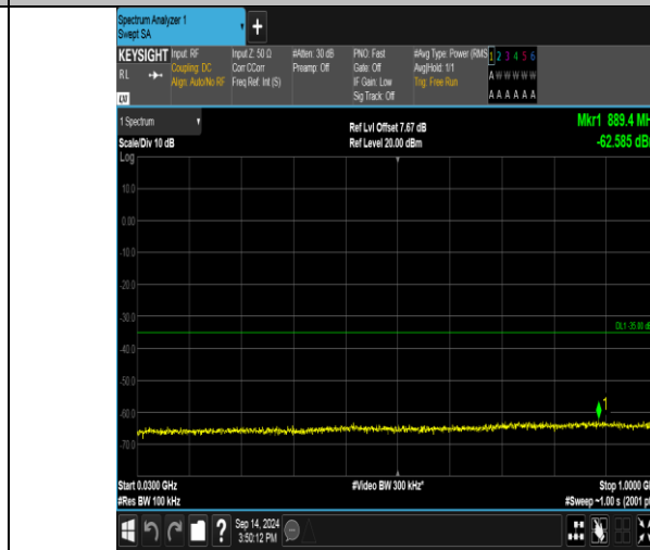
Band41_20MHz_16QAM_40590_1RB#99_30~1000_30~1000
