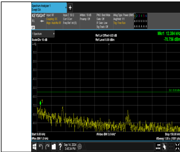
Band41_20MHz_QPSK_40140_100RB#0_0.009-0.15_0.009-0.15
