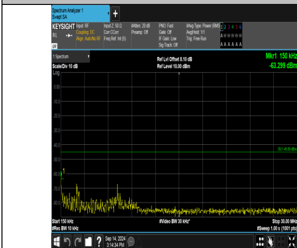
Band41_15MHz_16QAM_41165_1RB#0_0.15~30_0.15~30
