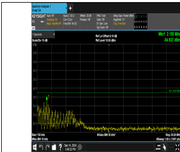
Band41_20MHz_16QAM_40140_100RB#0_0.15~30_0.15~30
