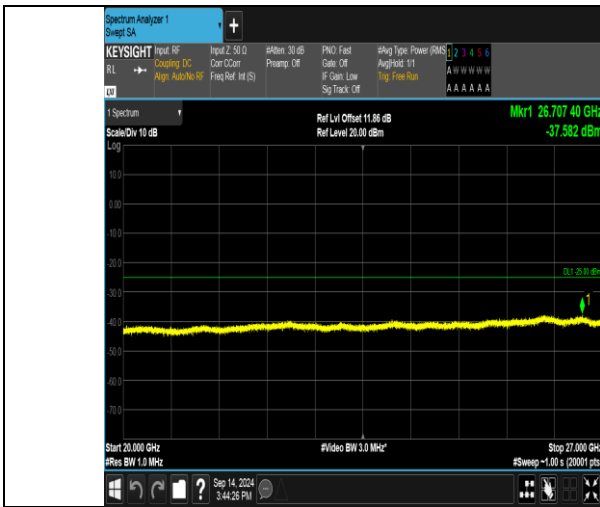
Band41_20MHz_QPSK_40140_1RB#99_20000~27000_20000~27000
