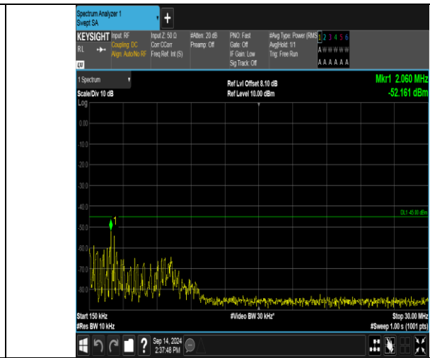
Band41_10MHz_QPSK_41190_50RB#0_0.15~30_0.15~30
