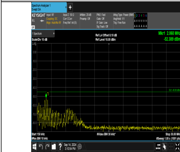
Band41_15MHz_16QAM_40590_1RB#74_0.15~30_0.15~30
