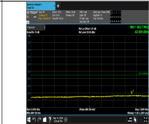
Band41_15MHz_16QAM_40115_1RB#74_30~1000_30~1000
