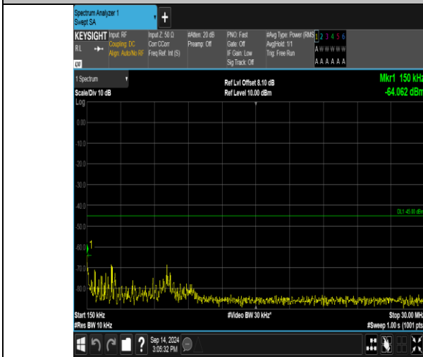
Band41_15MHz_16QAM_40115_1RB#74_0.15~30_0.15~30
