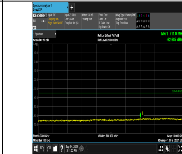
Band41_15MHz_16QAM_40590_1RB#74_30~1000_30~1000
