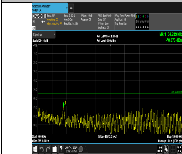
Band41_15MHz_QPSK_40590_1RB#74_0.009~0.15_0.009~0.15
