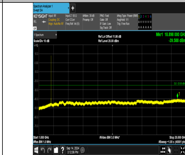
Band41_15MHz_QPSK_40590_75RB#0_1000~20000_1000~20000
