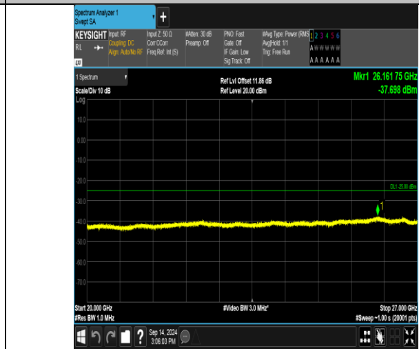
Band41_15MHz_16QAM_40115_1RB#74_20000~27000_20000~27000
