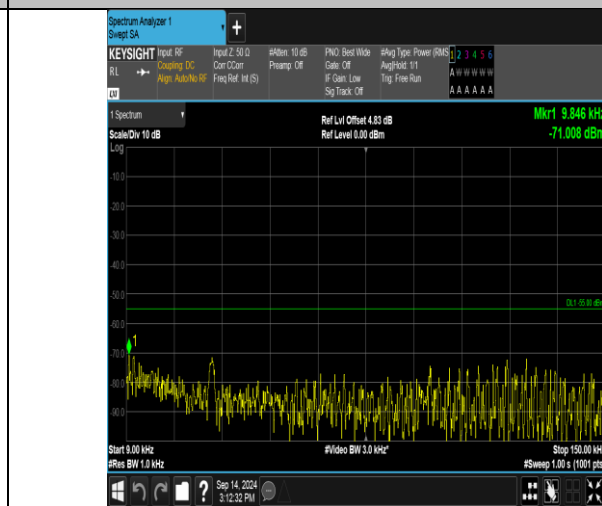
Band41_15MHz_16QAM_40590_75RB#0_0.009~0.15_0.009~0.15
