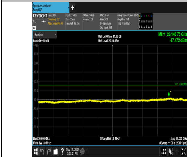
Band41_15MHz_QPSK_40115_1RB#0_20000~27000_20000~27000
