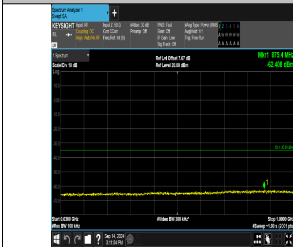
Band41_15MHz_QPSK_40590_75RB#0_30~1000_30~1000
