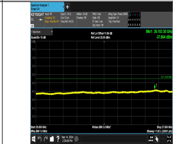
Band41_10MHz_16QAM_41190_50RB#0_20000~27000_20000~27000
