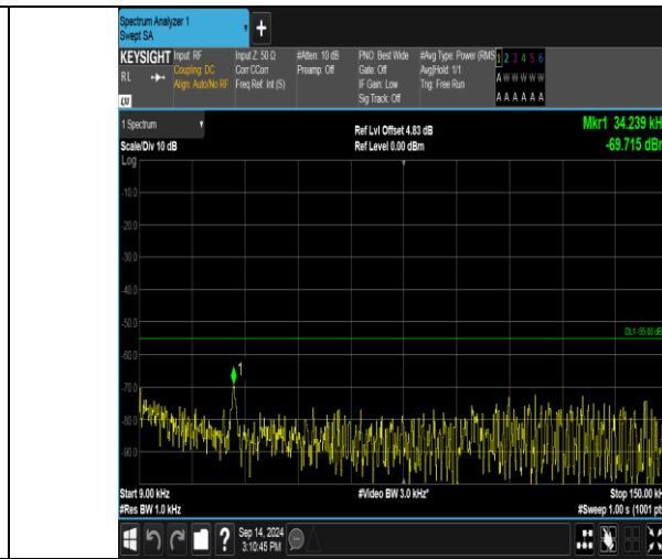
Band41_15MHz_16QAM_40590_1RB#74_0.009~0.15_0.009~0.15
