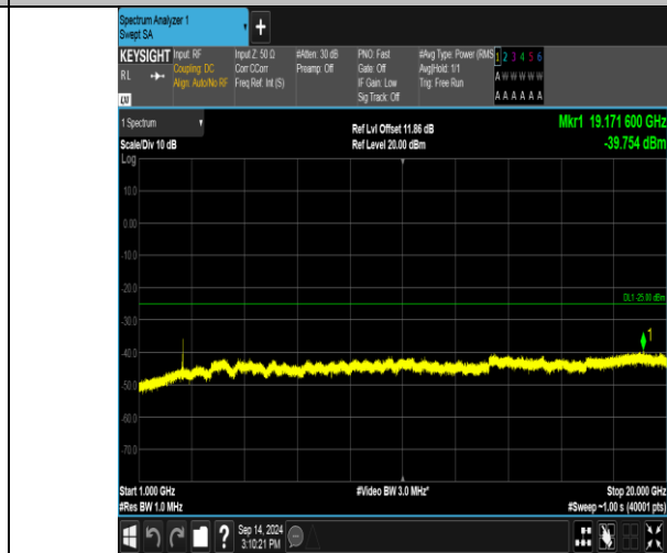
Band41_15MHz_QPSK_40590_1RB#74_1000~20000_1000~20000
