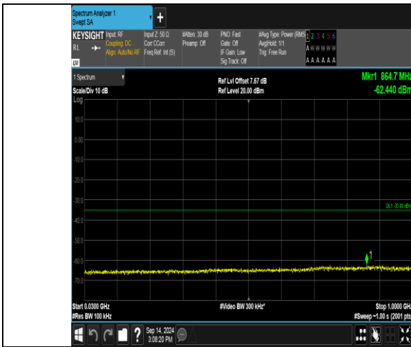
Band41_15MHz_QPSK_40590_1RB#0_30~1000_30~1000
