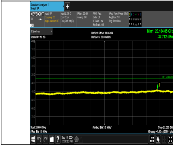
Band41_10MHz_QPSK_41190_50RB#0_20000~27000_20000~27000
