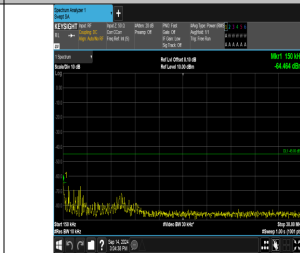
Band41_15MHz_QPSK_40115_1RB#74_0.15~30_0.15~30
