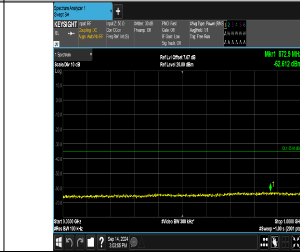
Band41_15MHz_16QAM_40115_1RB#0_30~1000_30~1000
