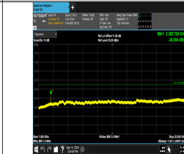
Band41_15MHz_QPSK_40115_1RB#74_1000~20000_1000~20000
