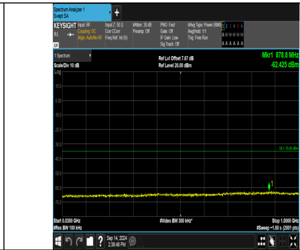
Band41_10MHz_16QAM_41190_50RB#0_30~1000_30~1000
