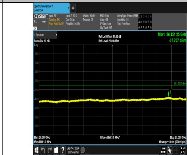
Band41_15MHz_16QAM_40115_75RB#0_20000-27000_20000-27000
