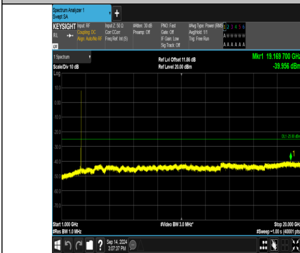
Band41_15MHz_16QAM_40115_75RB#0_1000-20000_1000-20000
