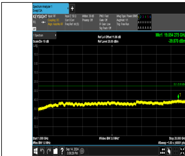
Band41_15MHz_16QAM_40590_1RB#0_1000~20000_1000~20000
