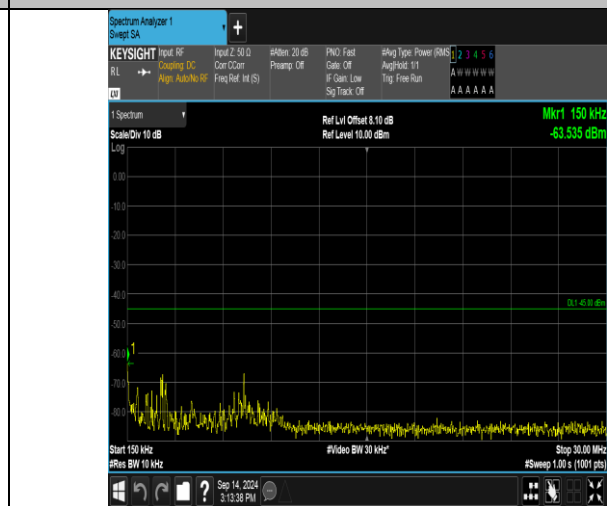
Band41_15MHz_QPSK_41165_1RB#0_0.15~30_0.15~30
