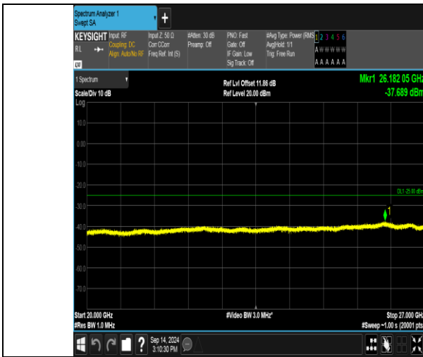
Band41_15MHz_QPSK_40590_1RB#74_2000~27000_20000~27000
