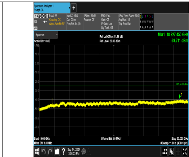
Band41_15MHz_QPSK_40590_1RB#0_1000~20000_1000~20000
