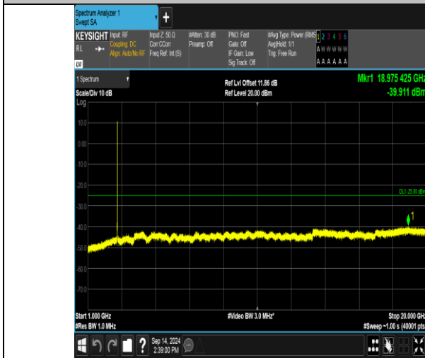
Band41_10MHz_16QAM_41190_50RB#0_1000~20000_1000~20000
