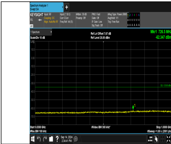
Band41_10MHz_QPSK_41190_1RB#0_30~1000_30~1000
