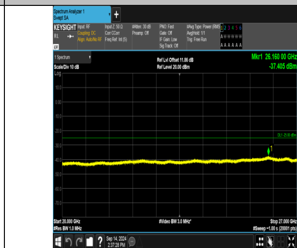
Band41_10MHz_16QAM_41190_1RB#49_20000~27000_20000~27000
