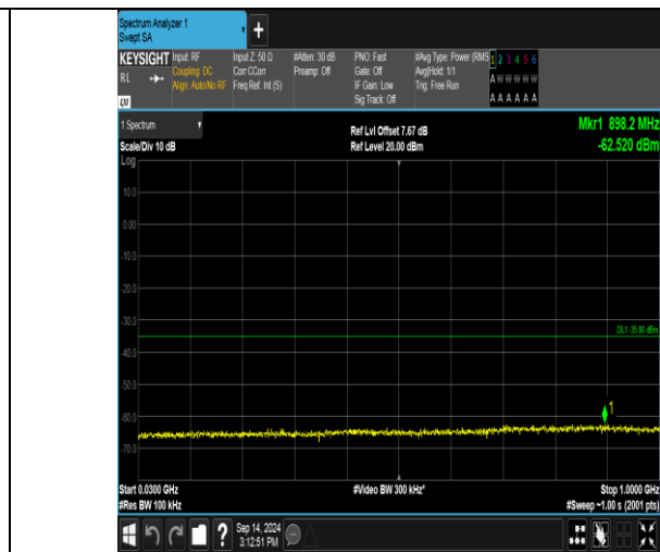
Band41_15MHz_16QAM_40590_75RB#0_30~1000_30~1000
