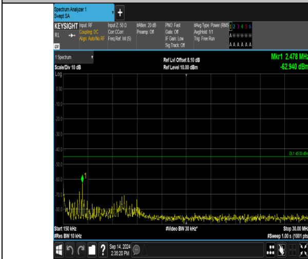
Band41_10MHz_16QAM_41190_1RB#0_0.15~30_0.15~30
