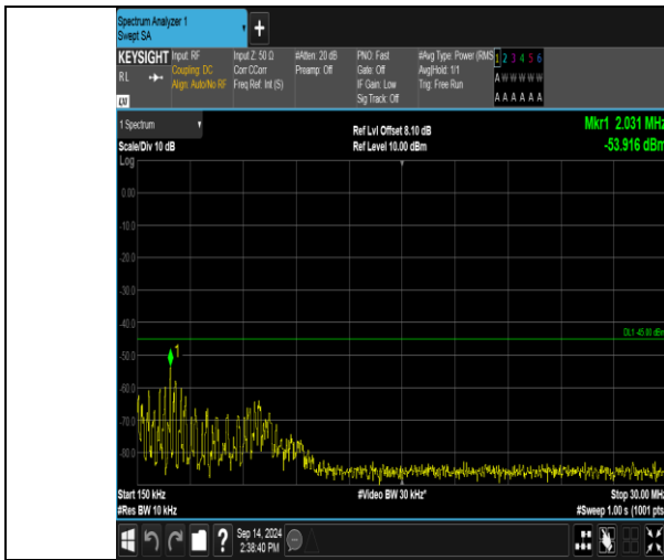
Band41_10MHz_16QAM_41190_50RB#0_0.15~30_0.15~30
