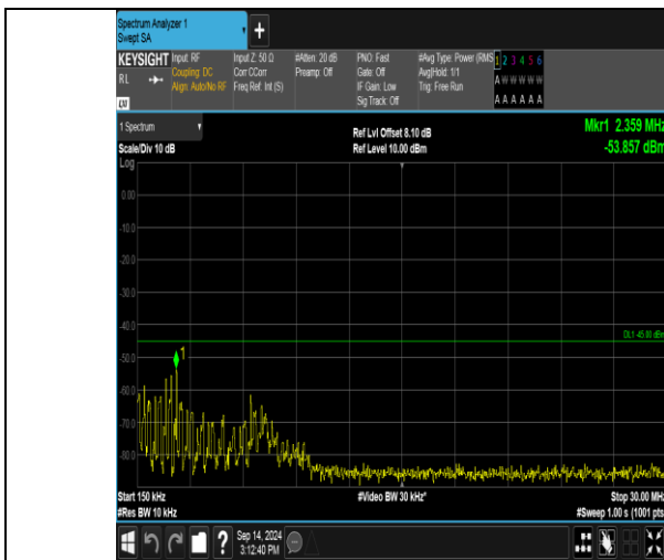
Band41_15MHz_16QAM_40590_75RB#0_0.15~30_0.15~30
