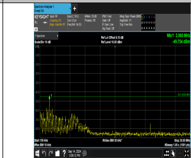
Band41_15MHz_QPSK_40590_1RB#0_0.15-30_0.15-30
