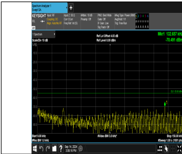
Band41_15MHz_QPSK_40115_75RB#0_0.009~0.15_0.009~0.15
