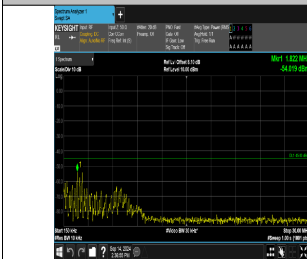
Band41_10MHz_16QAM_41190_1RB#49_0.15~30_0.15~30
