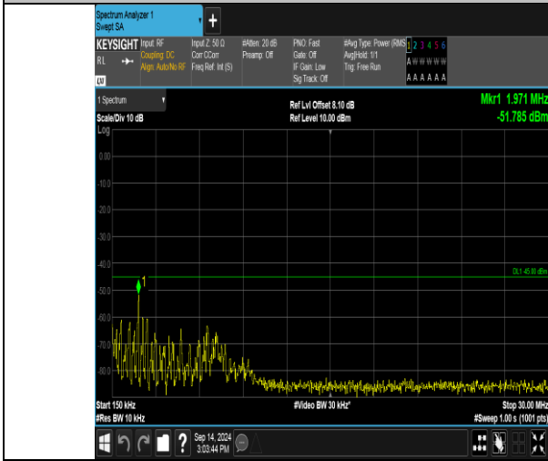
Band41_15MHz_16QAM_40115_1RB#0_0.15~30_0.15~30
