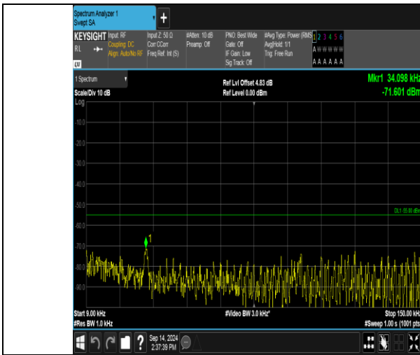
Band41_10MHz_QPSK_41190_50RB#0_0.009~0.15_0.009~0.15
