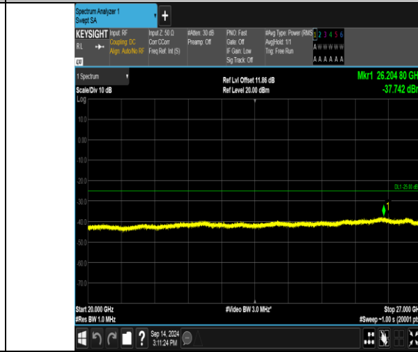
Band41_15MHz_16QAM_40590_1RB#74_20000~27000_20000~27000
