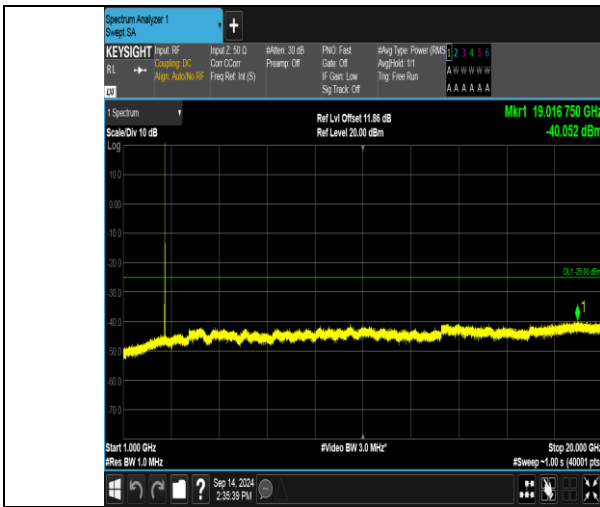
Band41_10MHz_16QAM_41190_1RB#0_1000~20000_1000~20000
