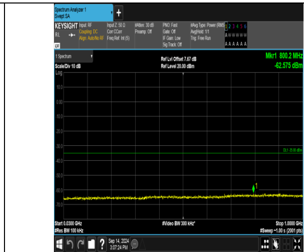
Band41_15MHz_16QAM_40115_75RB#0_30-1000_30-1000
