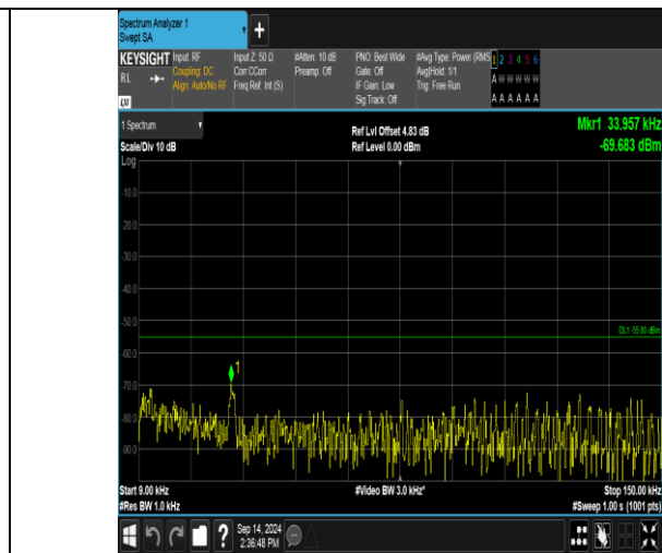
Band41_10MHz_16QAM_41190_1RB#49_0.009~0.15_0.009~0.15
