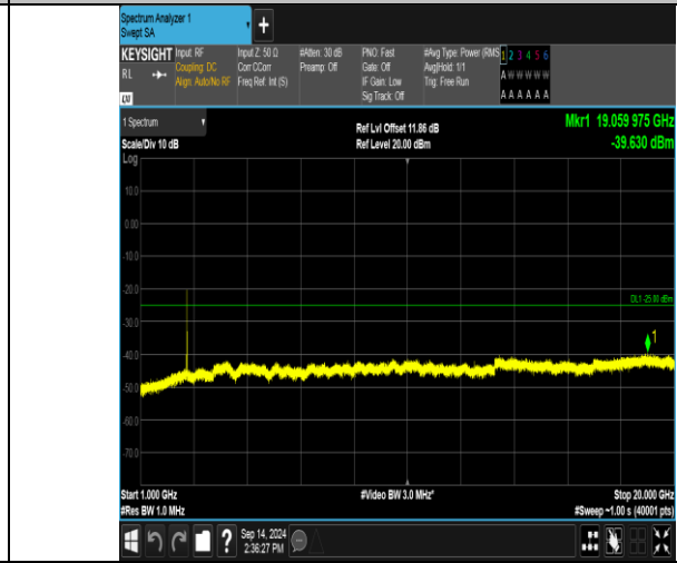
Band41_10MHz_QPSK_41190_1RB#49_1000~20000_1000~20000
