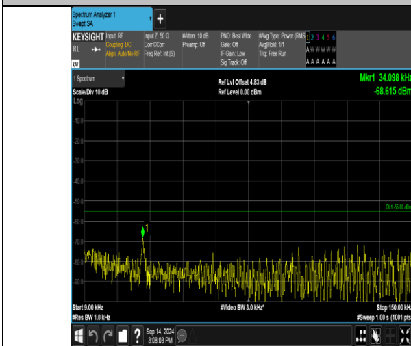
Band41_15MHz_QPSK_40590_1RB#0_0.009-0.15_0.009-0.15
