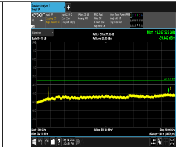
Band41_10MHz_QPSK_41190_1RB#0_1000~20000_1000~20000
