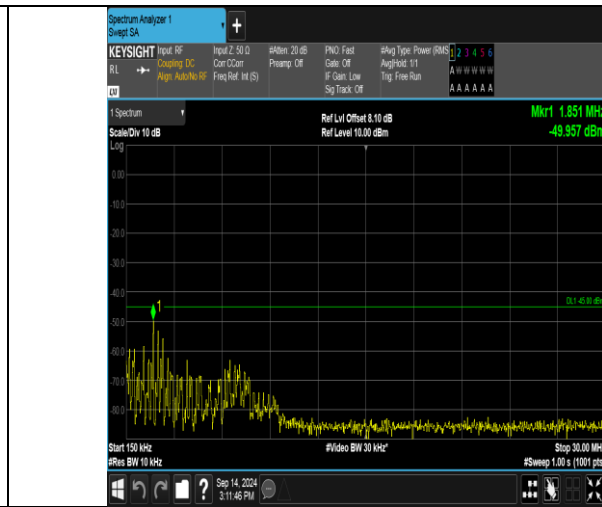
Band41_15MHz_QPSK_40590_75RB#0_0.15~30_0.15~30
