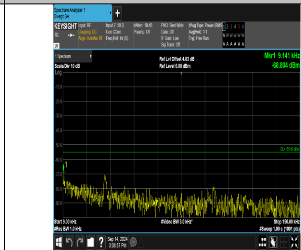
Band41_15MHz_16QAM_40590_1RB#0_0.009~0.15_0.009~0.15
