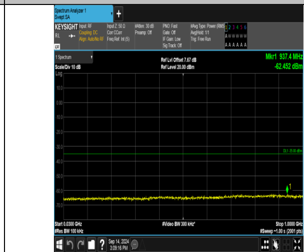
Band41_15MHz_16QAM_40590_1RB#0_30~1000_30~1000
