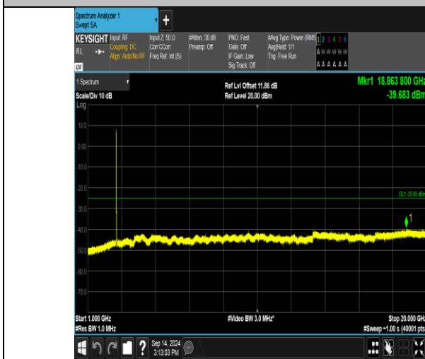
Band41_15MHz_16QAM_40590_75RB#0_1000~20000_1000~20000
