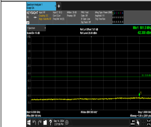
Band41_10MHz_QPSK_41190_50RB#0_30~1000_30~1000
