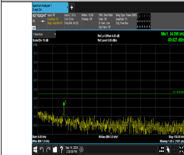
Band41_10MHz_QPSK_41190_1RB#49_0.009~0.15_0.009~0.15
