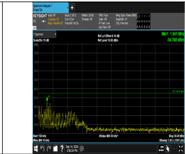
Band41_15MHz_QPSK_40115_75RB#0_0.15~30_0.15~30
