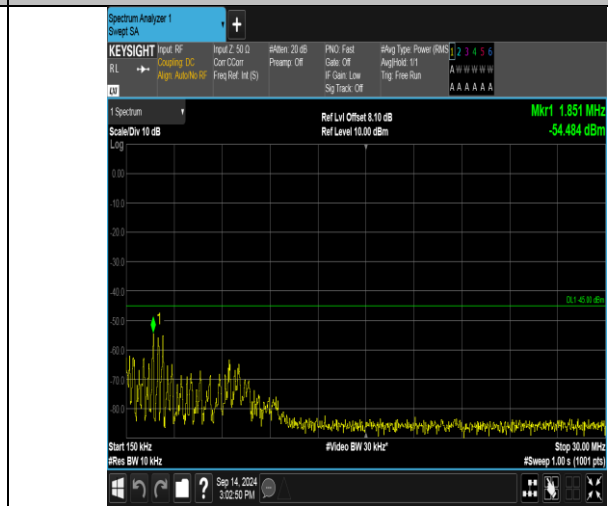
Band41_15MHz_QPSK_40115_1RB#0_0.15~30_0.15~30
