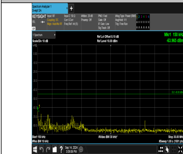
Band41_15MHz_16QAM_40590_1RB#0_0.15~30_0.15~30
