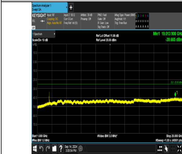
Band41_15MHz_16QAM_40115_1RB#74_1000~20000_1000~20000
