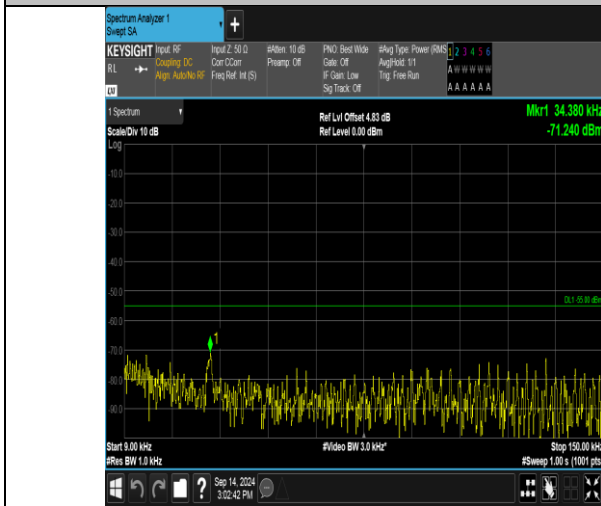
Band41_15MHz_QPSK_40115_1RB#0_0.009~0.15_0.009~0.15
