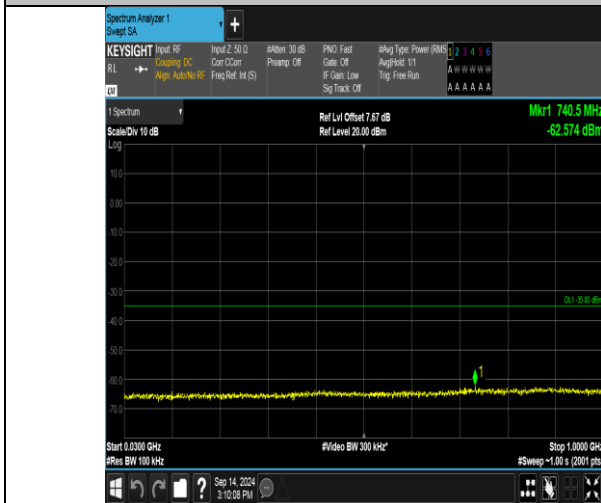
Band41_15MHz_QPSK_40590_1RB#74_30~1000_30~1000
