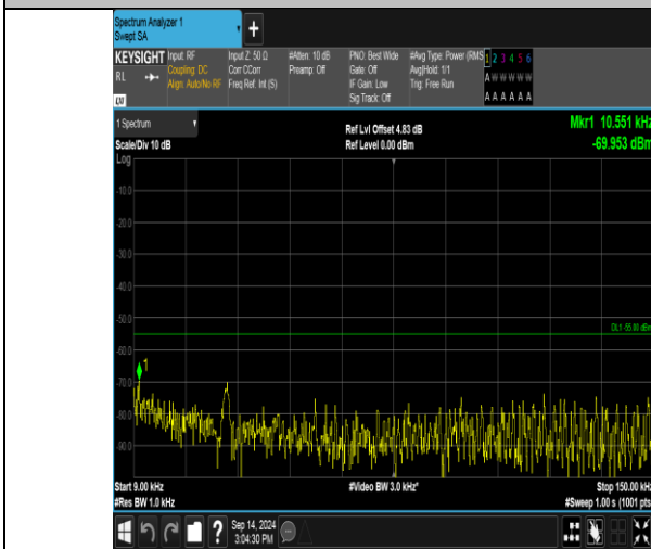
Band41_15MHz_QPSK_40115_1RB#74_0.009~0.15_0.009~0.15
