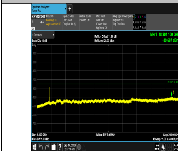
Band41_10MHz_16QAM_41190_1RB#49_1000~20000_1000~20000
