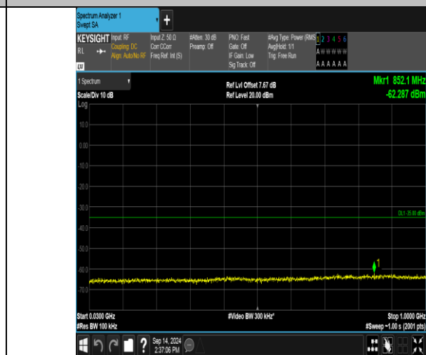
Band41_10MHz_16QAM_41190_1RB#49_30~1000_30~1000
