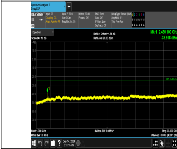
Band41_15MHz_16QAM_40590_1RB#74_1000~20000_1000~20000
