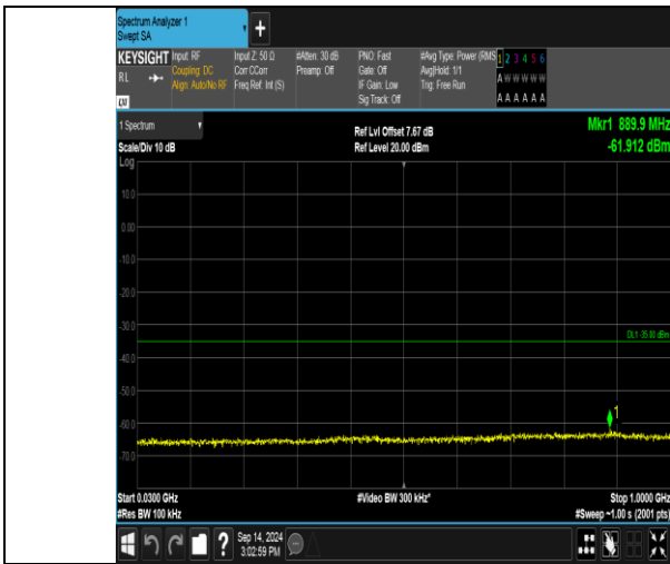
Band41_15MHz_QPSK_40115_1RB#0_30~1000_30~1000
