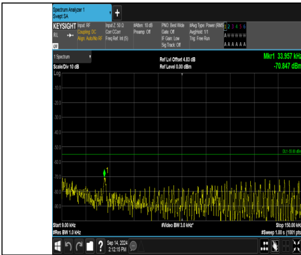
Band41_10MHz_QPSK_40090_50RB#0_0.009~0.15_0.009~0.15
