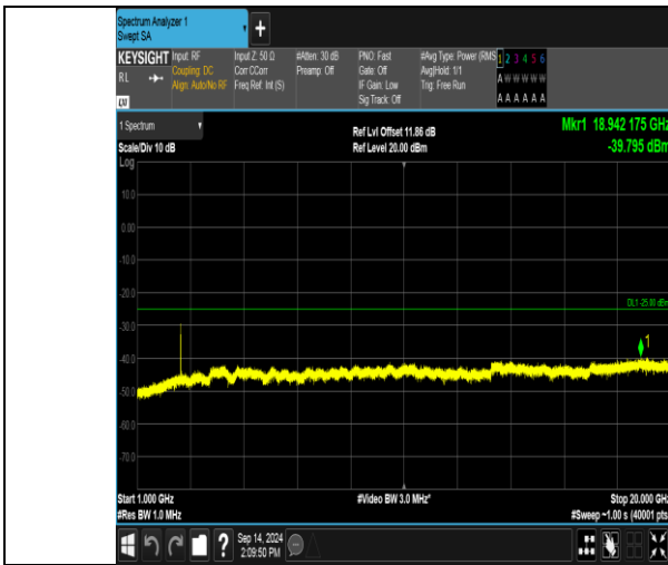
Band41_10MHz_16QAM_40090_1RB#0_1000~20000_1000~20000
