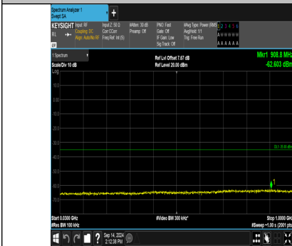
Band41_10MHz_QPSK_40090_50RB#0_30~1000_30~1000
