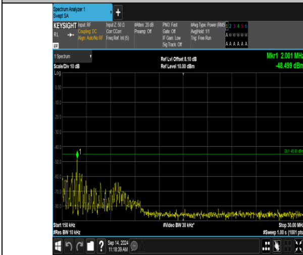
Band41_5MHz_16QAM_41215_1RB#0_0.15~30_0.15~30
