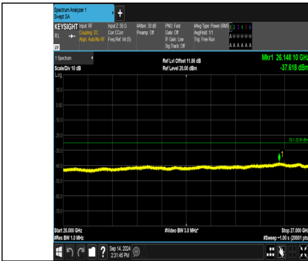
Band41_10MHz_QPSK_40590_1RB#49_20000~27000_20000~27000
