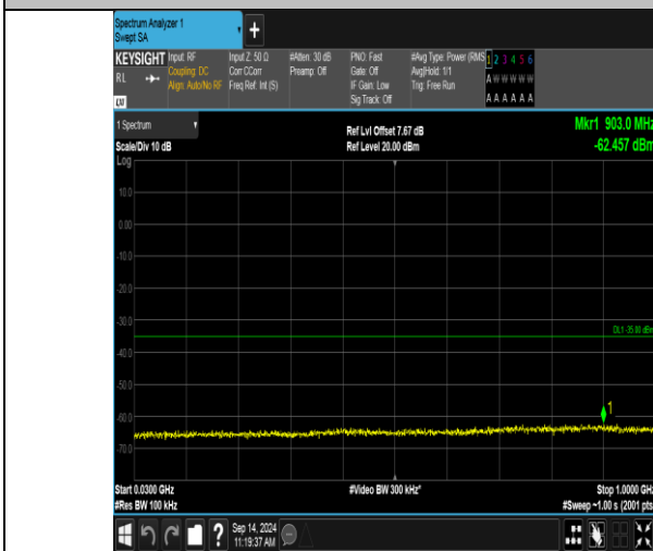
Band41_5MHz_QPSK_41215_1RB#24_30-1000_30-1000
