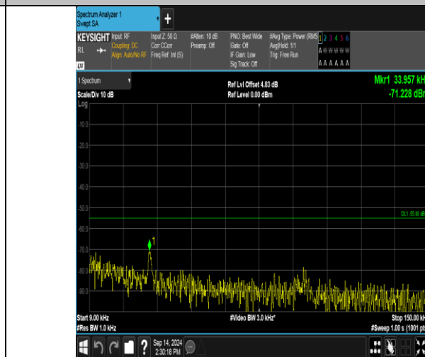
Band41_10MHz_16QAM_40590_1RB#0_0.009~0.15_0.009~0.15
