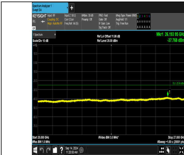
Band41_5MHz_QPSK_41215_1RB#24_20000-27000_20000-27000
