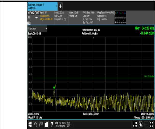
Band41_10MHz_16QAM_40590_50RB#0_0.009~0.15_0.009~0.15
