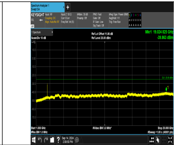
Band41_10MHz_QPSK_40090_1RB#0_1000~20000_1000~20000
