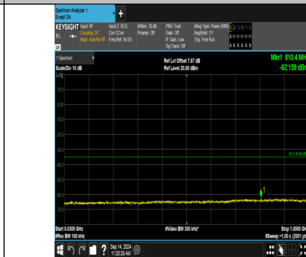
Band41_5MHz_16QAM_41215_1RB#24_30-1000_30-1000
