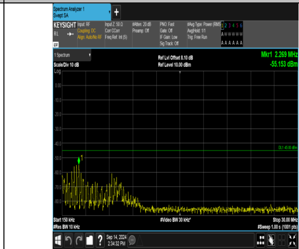
Band41_10MHz_QPSK_41190_1RB#0_0.15~30_0.15~30
