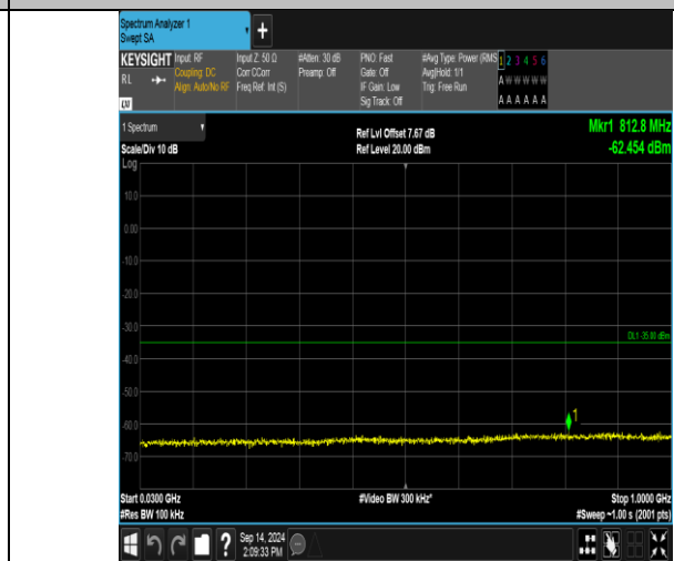
Band41_10MHz_16QAM_40090_1RB#0_30~1000_30~1000
