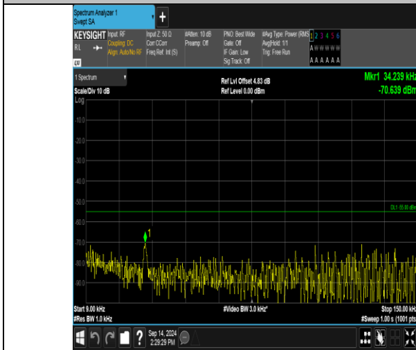
Band41_10MHz_QPSK_40590_1RB#0_0.009~0.15_0.009~0.15
