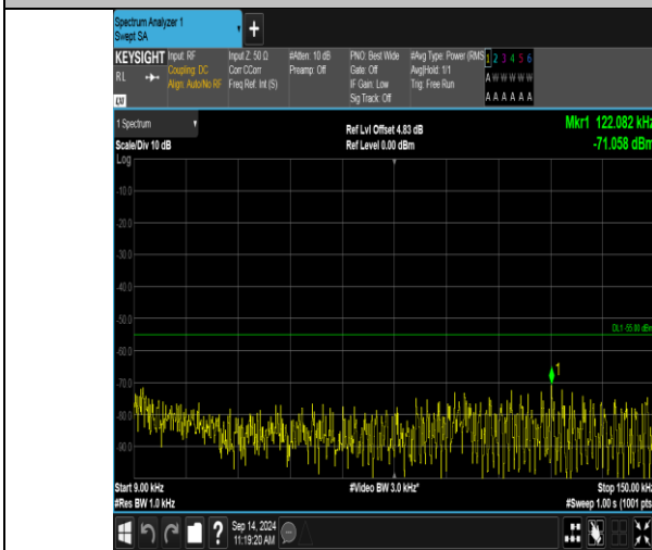
Band41_5MHz_QPSK_41215_1RB#24_0.009-0.15_0.009-0.15
