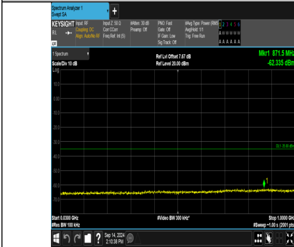
Band41_10MHz_QPSK_40090_1RB#49_30~1000_30~1000
