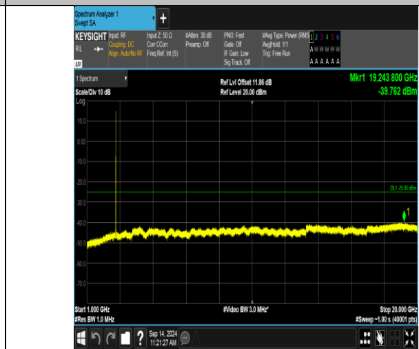
Band41_5MHz_QPSK_41215_25RB#0_1000~20000_1000~20000
