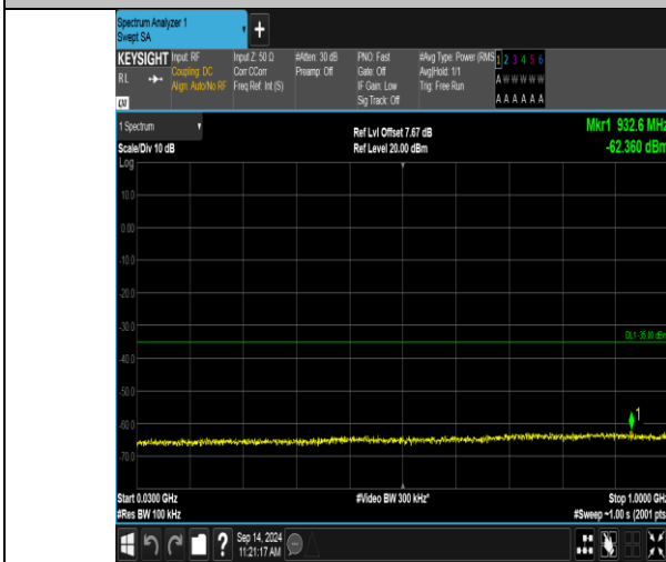
Band41_5MHz_QPSK_41215_25RB#0_30~1000_30~1000
