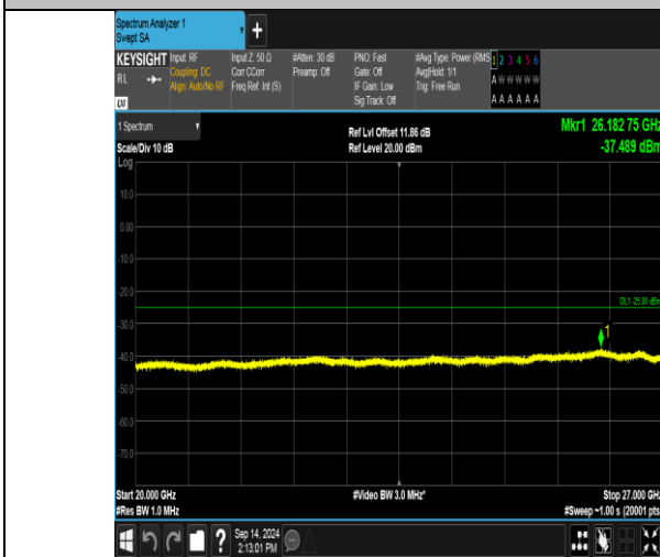
Band41_10MHz_QPSK_40090_50RB#0_20000~27000_20000~27000
