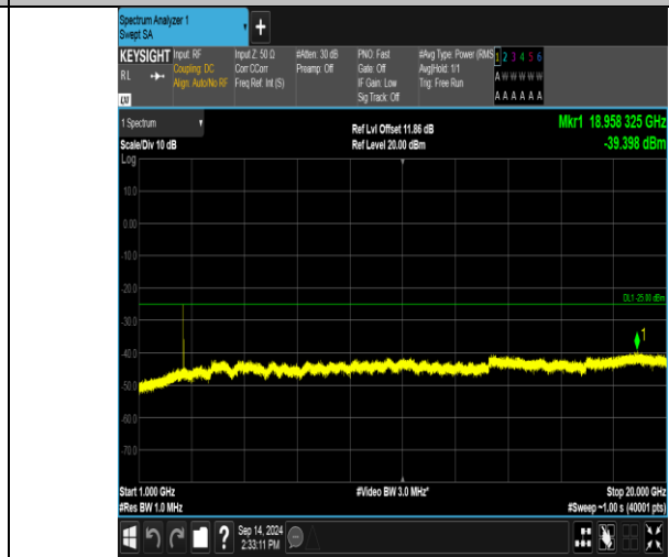
Band41_10MHz_QPSK_40590_50RB#0_1000~20000_1000~20000
