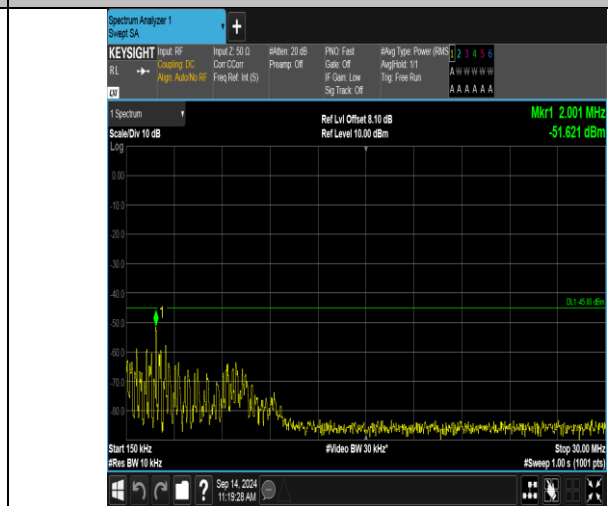
Band41_5MHz_QPSK_41215_1RB#24_0.15-30_0.15-30
