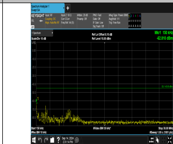
Band41_10MHz_QPSK_40590_1RB#49_0.15~30_0.15~30
