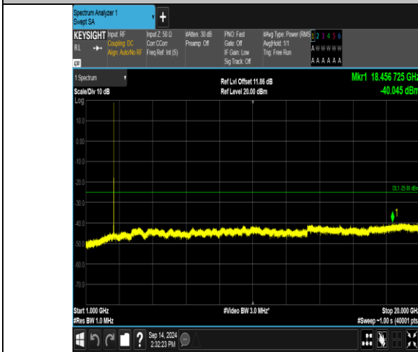
Band41_10MHz_16QAM_40590_1RB#49_1000~20000_1000~20000
