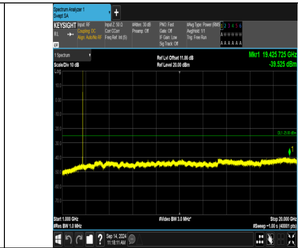
Band41_5MHz_QPSK_41215_1RB#0_1000~20000_1000~20000
