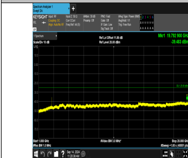
Band41_5MHz_16QAM_41215_1RB#24_1000-20000_1000-20000
