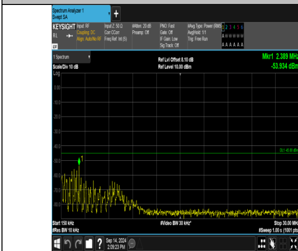
Band41_10MHz_16QAM_40090_1RB#0_0.15~30_0.15~30
