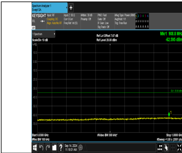
Band41_5MHz_QPSK_41215_1RB#0_30~1000_30~1000
