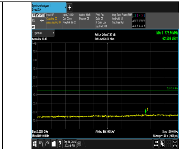
Band41_10MHz_16QAM_40590_50RB#0_30~1000_30~1000
