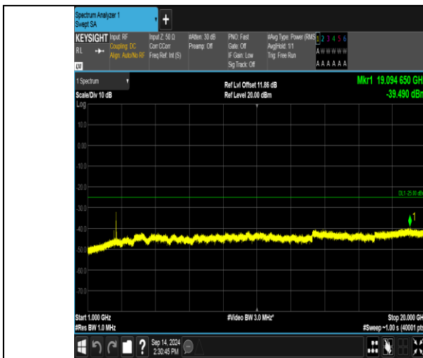
Band41_10MHz_16QAM_40590_1RB#0_1000~20000_1000~20000
