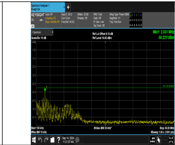
Band41_5MHz_QPSK_41215_25RB#0_0.15~30_0.15~30
