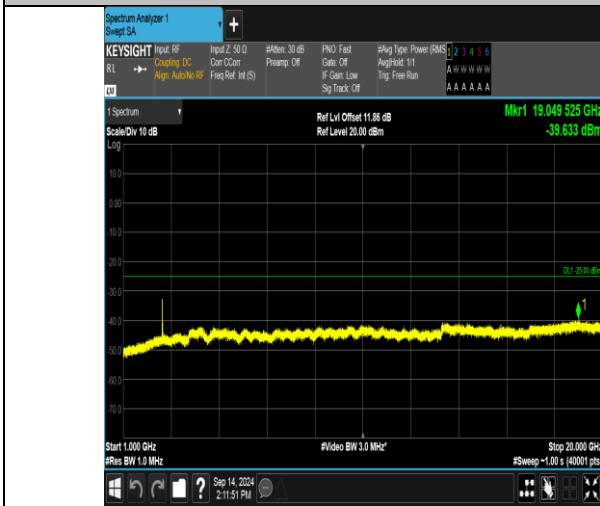
Band41_10MHz_16QAM_40090_1RB#49_1000~20000_1000~20000
