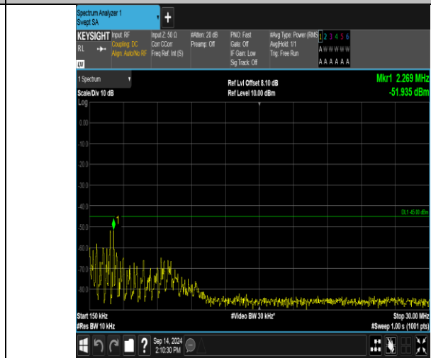
Band41_10MHz_QPSK_40090_1RB#49_0.15~30_0.15~30
