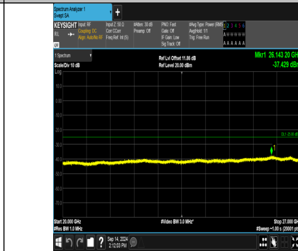
Band41_10MHz_16QAM_40090_1RB#49_20000~27000_20000~27000
