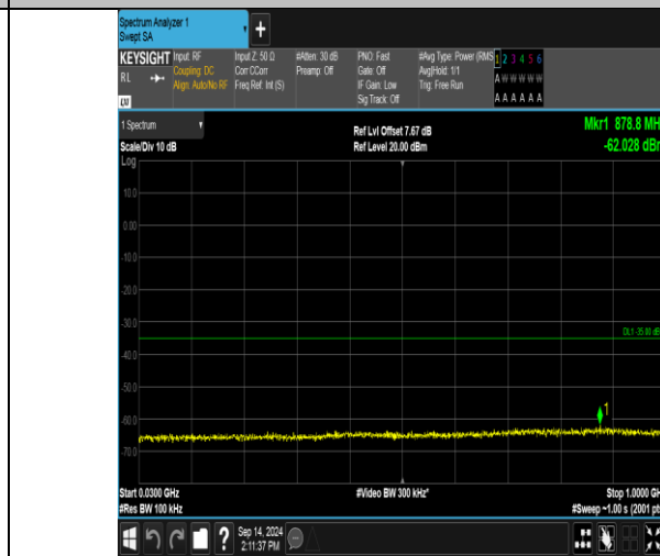
Band41_10MHz_16QAM_40090_1RB#49_30~1000_30~1000
