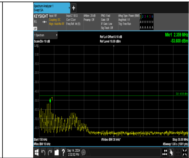
Band41_10MHz_QPSK_40590_50RB#0_0.15~30_0.15~30
