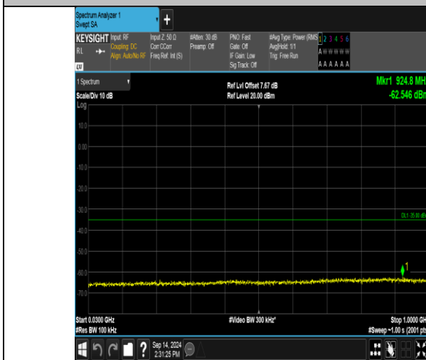
Band41_10MHz_QPSK_40590_1RB#49_30~1000_30~1000
