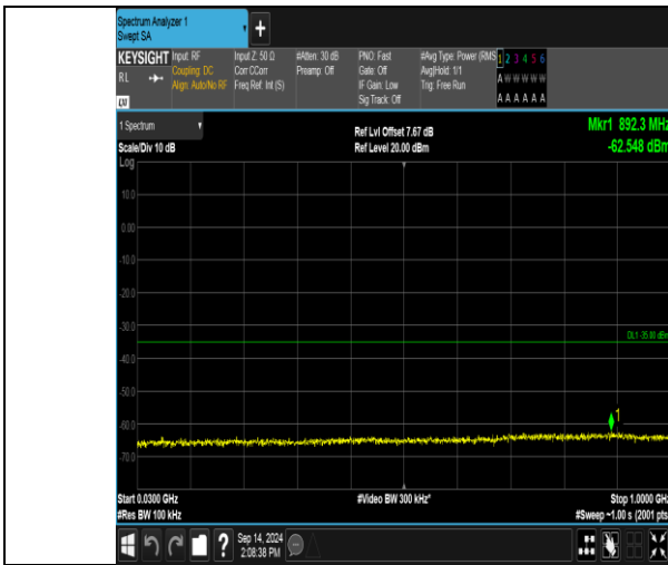
Band41_10MHz_QPSK_40090_1RB#0_30~1000_30~1000
