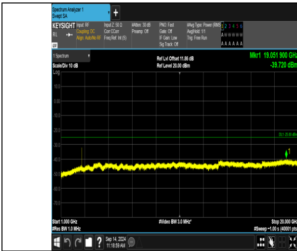
Band41_5MHz_16QAM_41215_1RB#0_1000-20000_1000-20000
