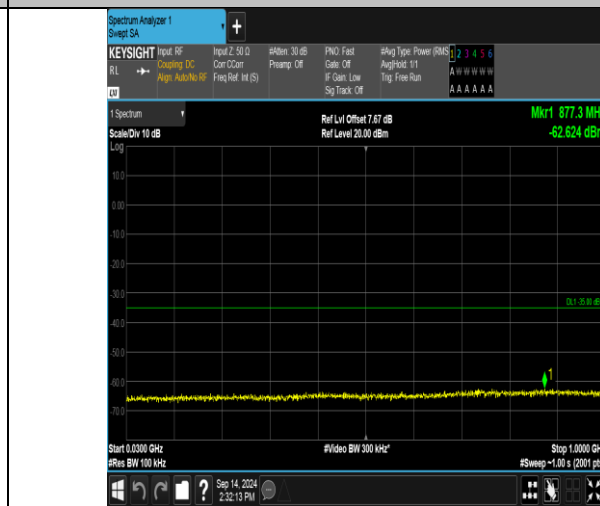
Band41_10MHz_16QAM_40590_1RB#49_30~1000_30~1000
