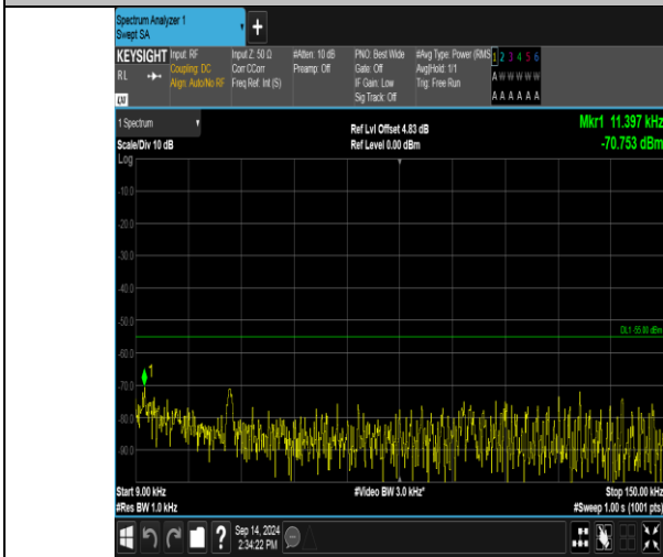
Band41_10MHz_QPSK_41190_1RB#0_0.009~0.15_0.009~0.15
