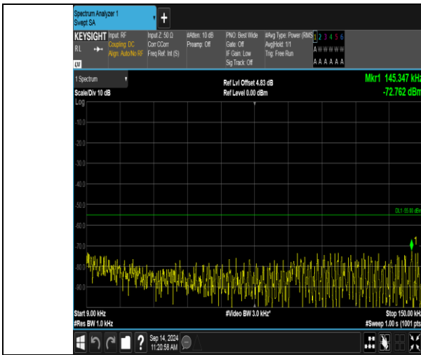
Band41_5MHz_QPSK_41215_25RB#0_0.009~0.15_0.009~0.15
