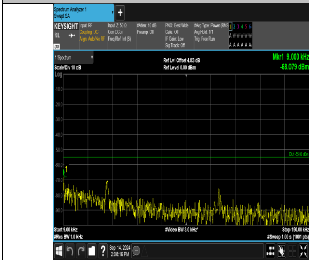
Band41_10MHz_QPSK_40090_1RB#0_0.009~0.15_0.009~0.15
