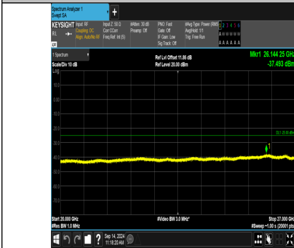
Band41_5MHz_QPSK_41215_1RB#0_20000~27000_20000~27000
