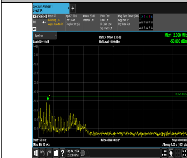
Band41_10MHz_16QAM_40590_1RB#49_0.15~30_0.15~30
