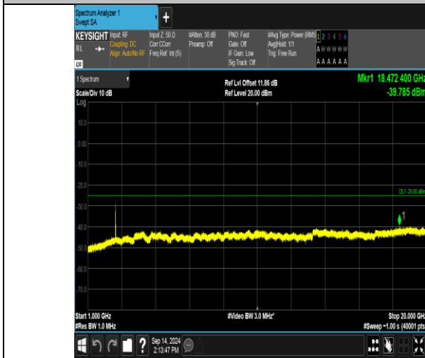
Band41_10MHz_16QAM_40090_50RB#0_1000~20000_1000~20000
