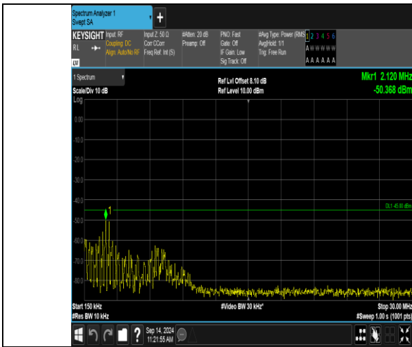
Band41_5MHz_16QAM_41215_25RB#0_0.15~30_0.15~30
