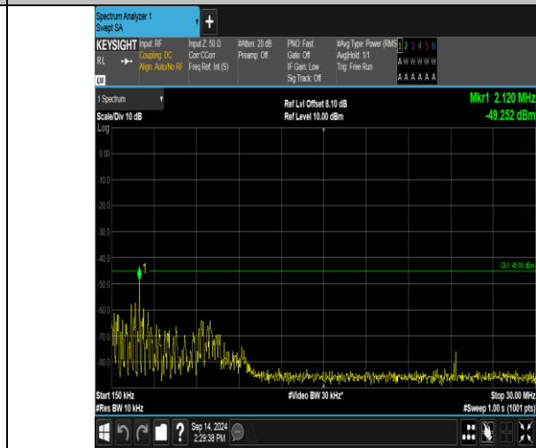
Band41_10MHz_QPSK_40590_1RB#0_0.15~30_0.15~30
