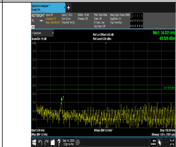
Band41_10MHz_16QAM_40090_1RB#0_0.009~0.15_0.009~0.15
