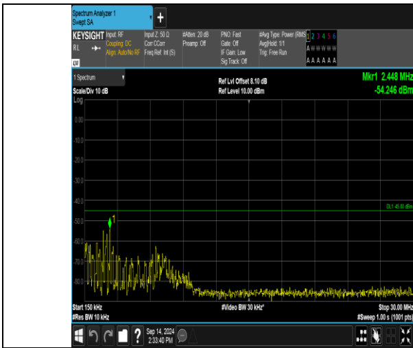
Band41_10MHz_16QAM_40590_50RB#0_0.15~30_0.15~30
