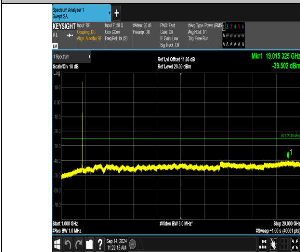
Band41_5MHz_16QAM_41215_25RB#0_1000~20000_1000~20000
