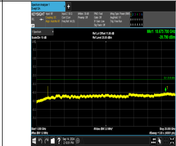
Band41_10MHz_QPSK_40090_1RB#49_1000~20000_1000~20000
