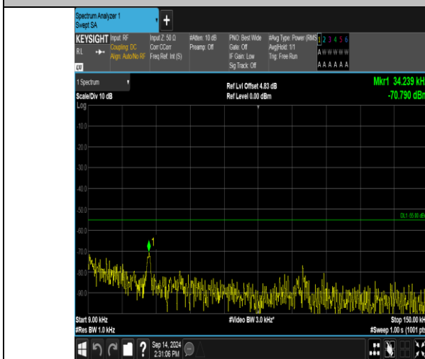
Band41_10MHz_QPSK_40590_1RB#49_0.009~0.15_0.009~0.15
