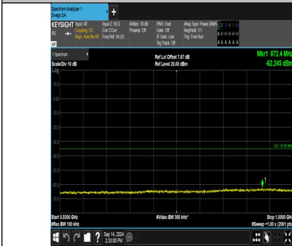
Band41_10MHz_QPSK_40590_50RB#0_30~1000_30~1000
