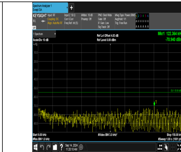
Band41_5MHz_16QAM_41215_1RB#24_0.009-0.15_0.009-0.15
