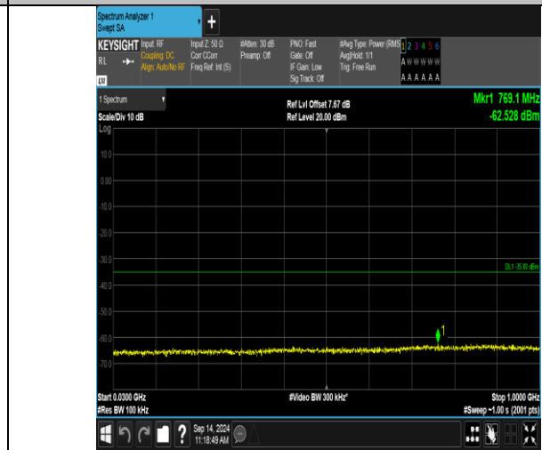
Band41_5MHz_16QAM_41215_1RB#0_30~1000_30~1000
