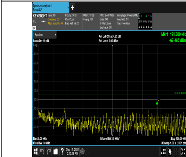
Band41_10MHz_QPSK_40090_1RB#49_0.009~0.15_0.009~0.15
