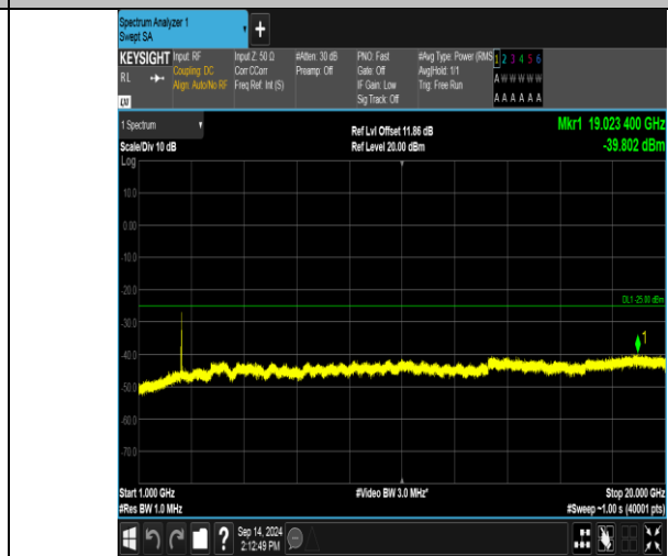
Band41_10MHz_QPSK_40090_50RB#0_1000~20000_1000~20000
