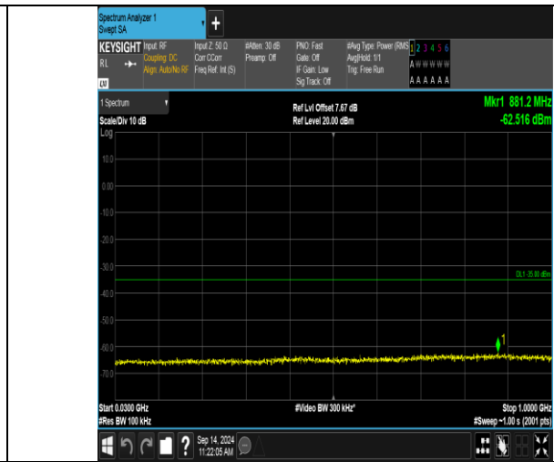
Band41_5MHz_16QAM_41215_25RB#0_30~1000_30~1000
