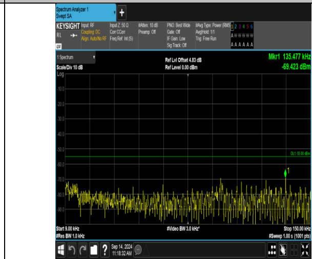
Band41_5MHz_16QAM_41215_1RB#0_0.009~0.15_0.009~0.15
