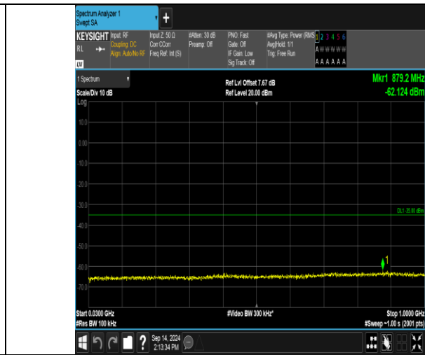
Band41_10MHz_16QAM_40090_50RB#0_30~1000_30~1000
