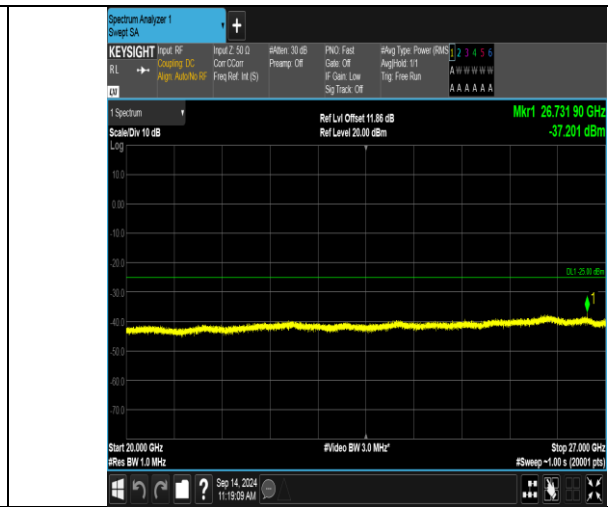
Band41_5MHz_16QAM_41215_1RB#0_20000-27000_20000-27000
