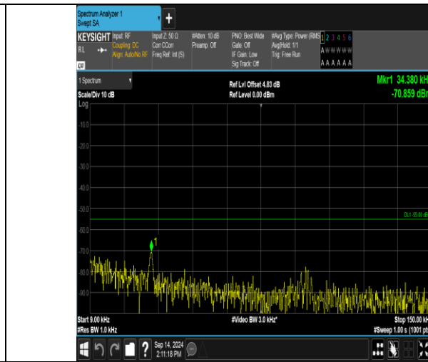
Band41_10MHz_16QAM_40090_1RB#49_0.009~0.15_0.009~0.15
