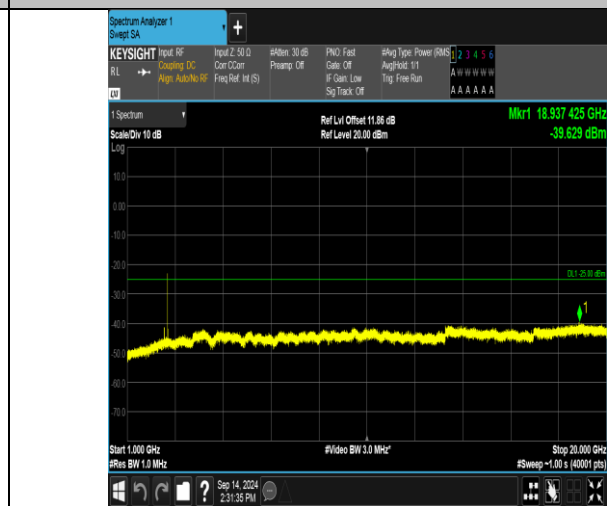
Band41_10MHz_QPSK_40590_1RB#49_1000~20000_1000~20000
