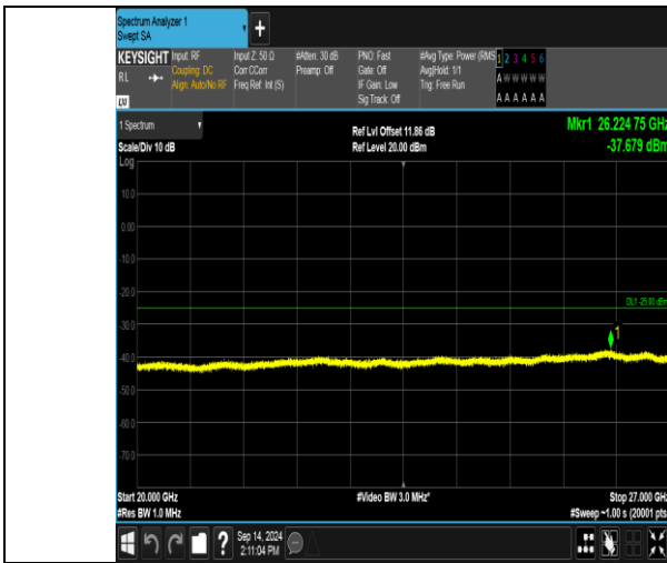
Band41_10MHz_QPSK_40090_1RB#49_20000~27000_20000~27000
