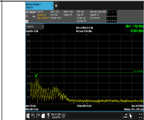
Band41_10MHz_QPSK_40090_1RB#0_0.15~30_0.15~30
