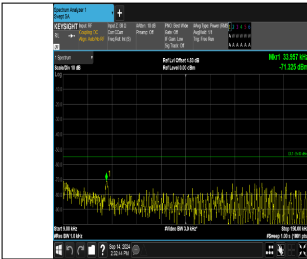
Band41_10MHz_QPSK_40590_50RB#0_0.009~0.15_0.009~0.15
