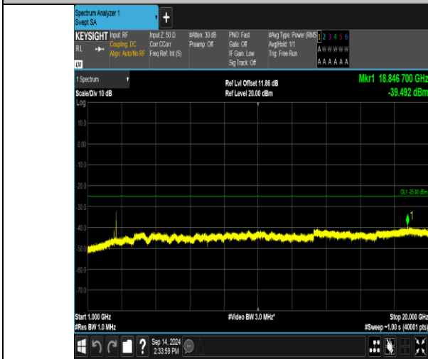
Band41_10MHz_16QAM_40590_50RB#0_1000~20000_1000~20000
