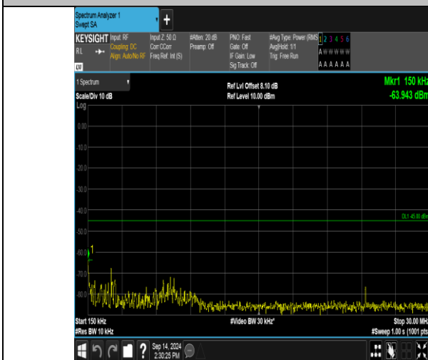
Band41_10MHz_16QAM_40590_1RB#0_0.15~30_0.15~30
