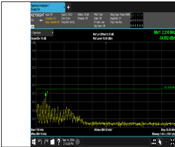
Band41_10MHz_16QAM_40090_50RB#0_0.15~30_0.15~30
