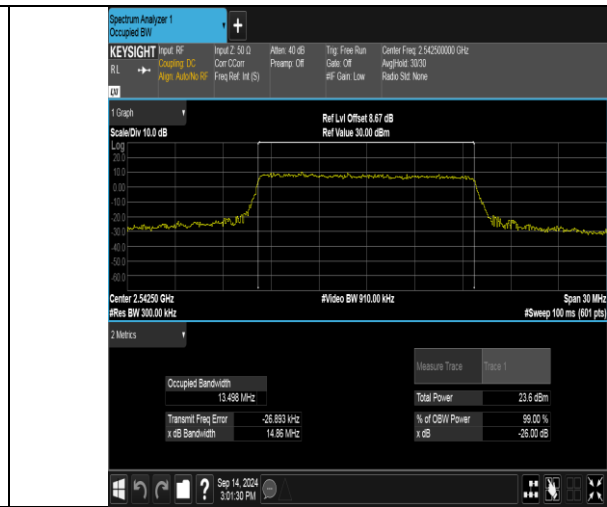
Band41(2535-2655)-15MHz-16QAM-40115-75RB#0-PASS
