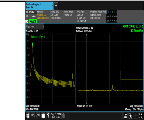
Band41_10MHz_16QAM_41190_1RB#0
