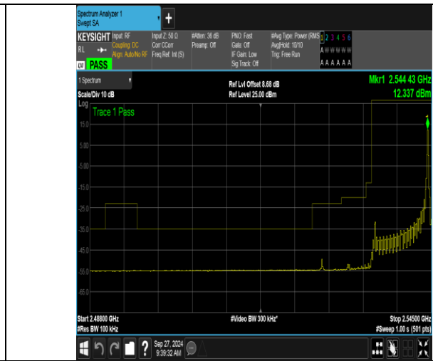
Band41_10MHz_16QAM_40090_1RB#49
