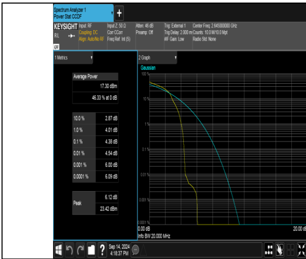
Band41(2535-2655)-20MHz-16QAM-41140-1RB#0-PASS
