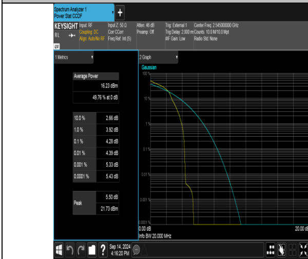
Band41(2535-2655)-20MHz-16QAM-40140-1RB#0-PASS
