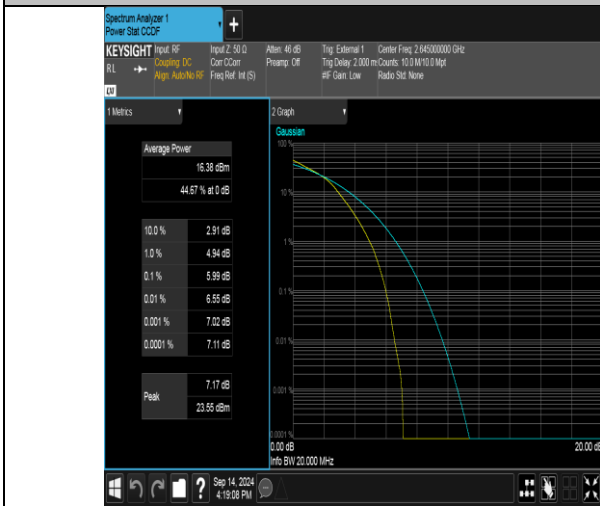
Band41(2535-2655)-20MHz-16QAM-41140-100RB#0-PASS
