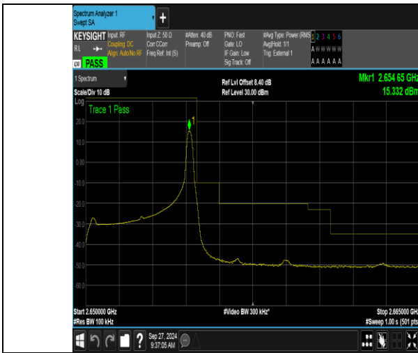
Band41_5MHz_QPSK_41215_1RB#24
