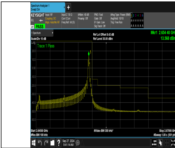
Band41_10MHz_QPSK_41190_1RB#49
