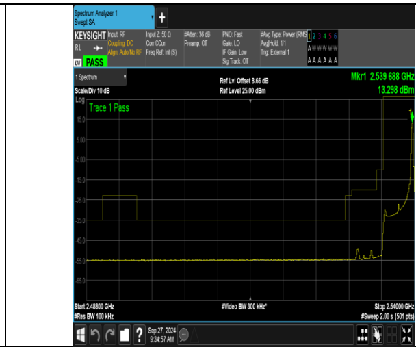
Band41_5MHz_16QAM_40065_1RB#24
