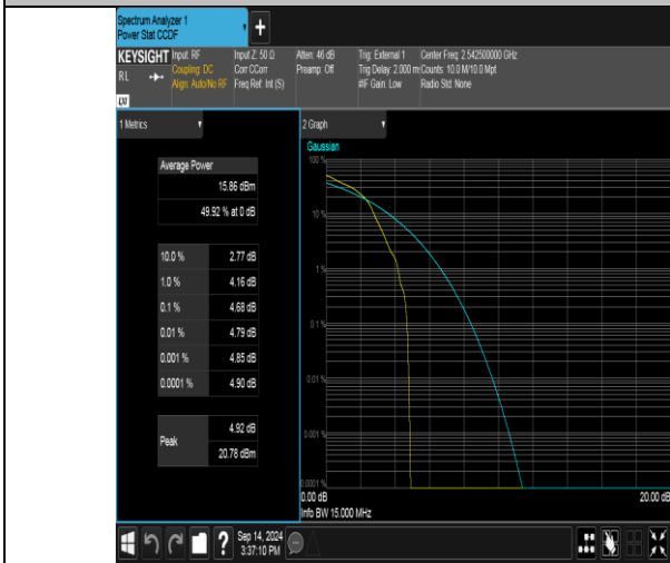
Band41(2535-2655)-15MHz-16QAM-40115-1RB#0-PASS
