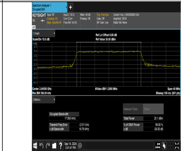
Band41(2535-2655)-20MHz-16QAM-41140-100RB#0-PASS
