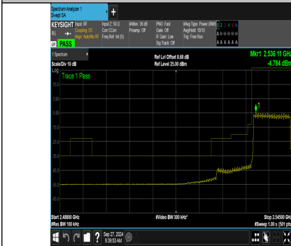
Band41_10MHz_QPSK_40090_50RB#0
