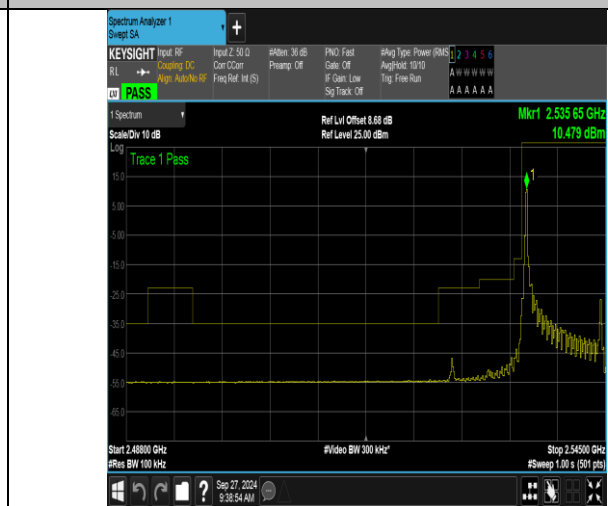
Band41_10MHz_16QAM_40090_1RB#0
