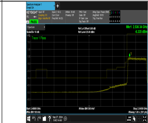
Band41_10MHz_16QAM_40090_50RB#0
