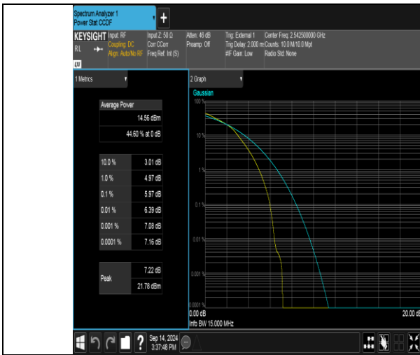
Band41(2535-2655)-15MHz-16QAM-40115-75RB#0-PASS
