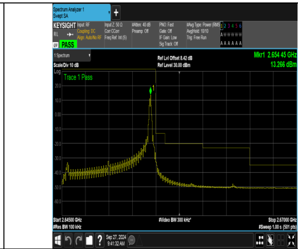
Band41_10MHz_16QAM_41190_1RB#49
