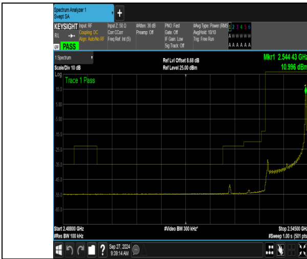
Band41_10MHz_QPSK_40090_1RB#49
