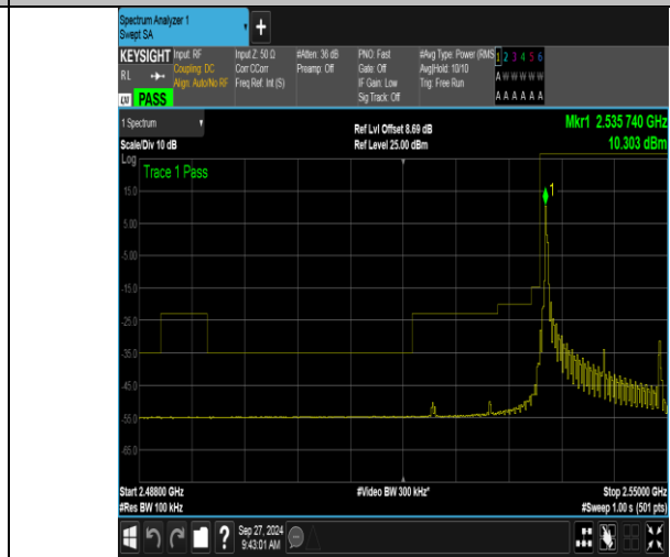
Band41_15MHz_16QAM_40115_1RB#0
