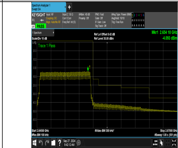
Band41_10MHz_16QAM_41190_50RB#0
