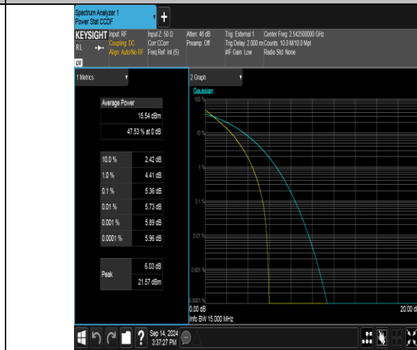
Band41(2535-2655)-15MHz-QPSK-40115-75RB#0-PASS
