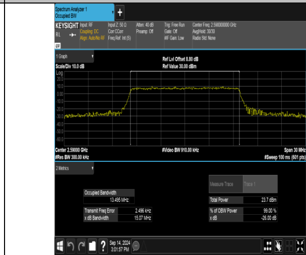
Band41(2535-2655)-15MHz-16QAM-40590-75RB#0-PASS
