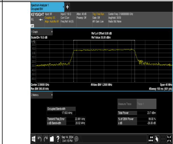
Band41(2535-2655)-20MHz-16QAM-40590-100RB#0-PASS
