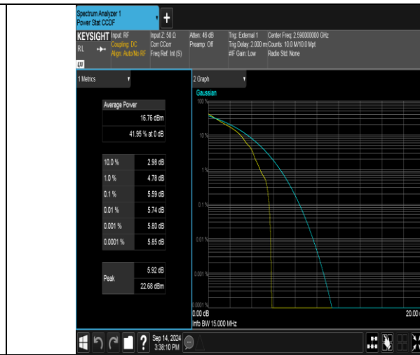
Band41(2535-2655)-15MHz-QPSK-40590-1RB#0-PASS
