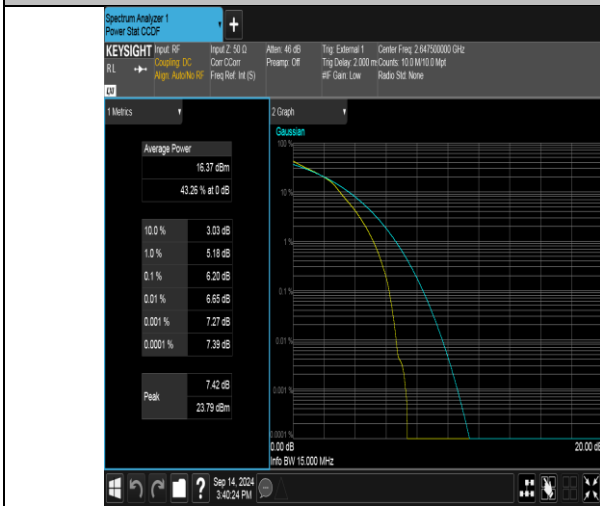
Band41(2535-2655)-15MHz-16QAM-41165-75RB#0-PASS
