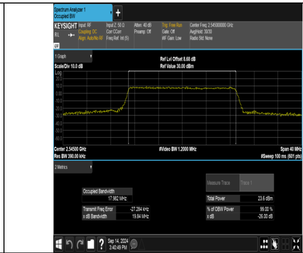
Band41(2535-2655)-20MHz-16QAM-40140-100RB#0-PASS
