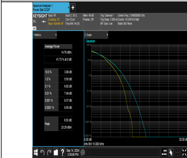
Band41(2535-2655)-15MHz-16QAM-40590-75RB#0-PASS
