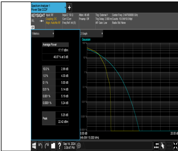
Band41(2535-2655)-15MHz-16QAM-41165-1RB#0-PASS
