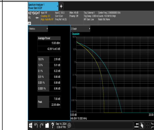
Band41(2535-2655)-15MHz-QPSK-40590-75RB#0-PASS
