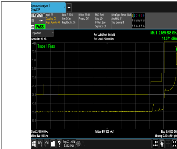
Band41_5MHz_QPSK_40065_1RB#24
