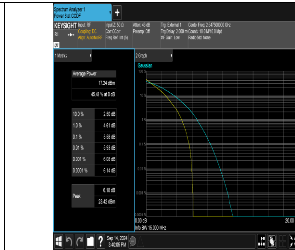
Band41(2535-2655)-15MHz-QPSK-41165-75RB#0-PASS
