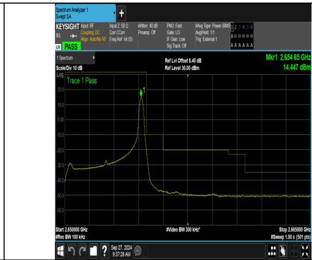
Band41_5MHz_16QAM_41215_1RB#24
