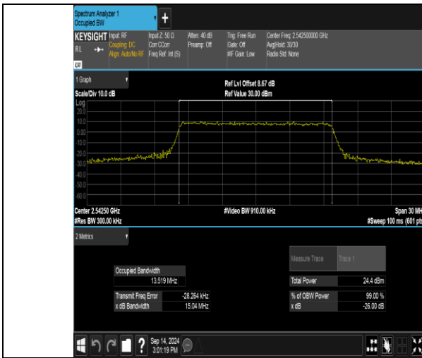
Band41(2535-2655)-15MHz-QPSK-40115-75RB#0-PASS
