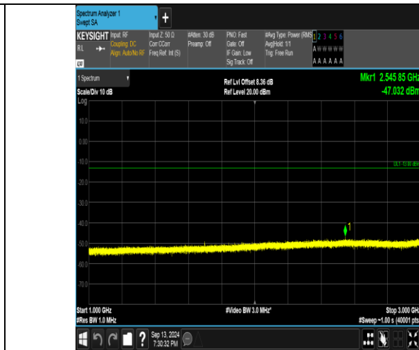
Band26_5MHz_QPSK_27015_1RB#24_1000~3000_1000~3000
