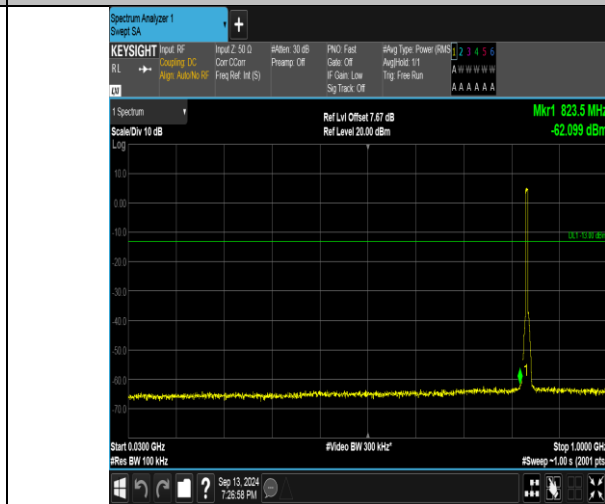
Band26_5MHz_16QAM_26915_25RB#0_30~1000_30~1000
