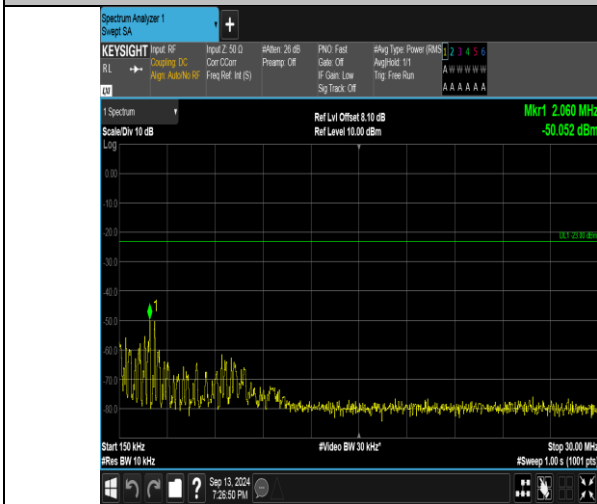
Band26_5MHz_16QAM_26915_25RB#0_0.15~30_0.15~30
