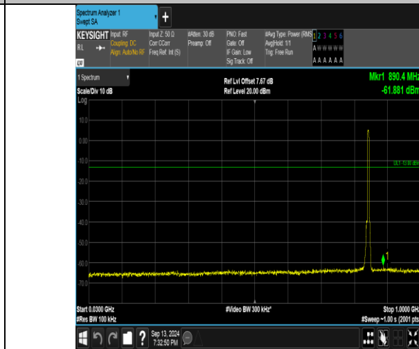
Band26_5MHz_16QAM_27015_25RB#0_30~1000_30~1000
