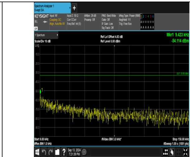
Band26_5MHz_16QAM_26815_25RB#0_0.009~0.15_0.009~0.15
