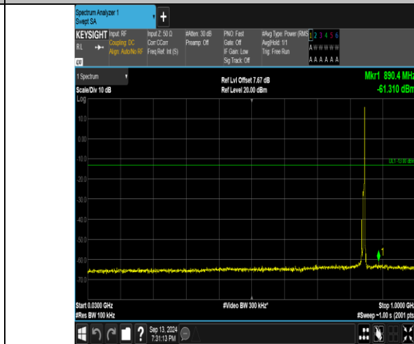
Band26_5MHz_16QAM_27015_1RB#24_30~1000_30~1000
