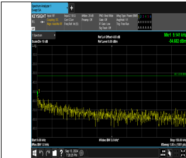
Band26_5MHz_QPSK_27015_1RB#0_0.009~0.15_0.009~0.15
