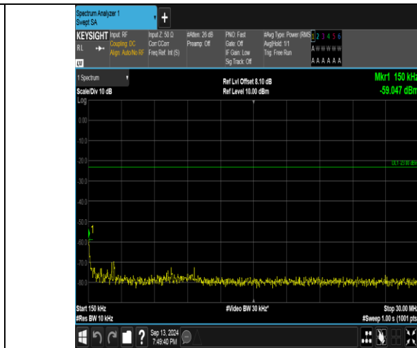
Band26_10MHz_QPSK_26840_1RB#0_0.15-30_0.15-30
