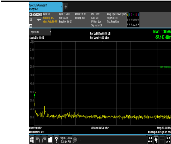
Band26_5MHz_16QAM_27015_1RB#24_0.15~30_0.15~30
