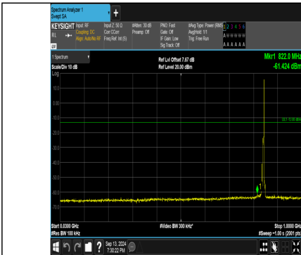
Band26_5MHz_QPSK_27015_1RB#24_30~1000_30~1000
