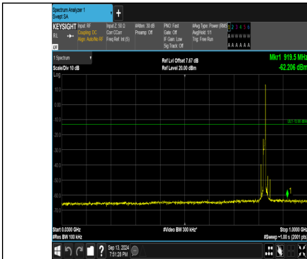
Band26_10MHz_QPSK_26840_1RB#49_30~1000_30~1000
