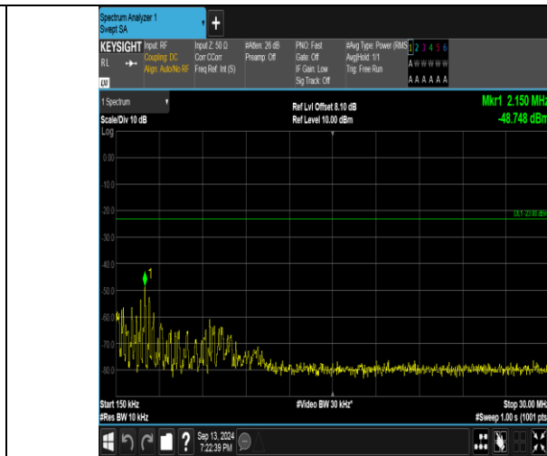
Band26_5MHz_QPSK_26915_1RB#0_0.15~30_0.15~30
