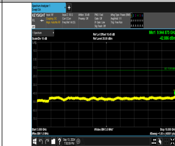
Band26_10MHz_16QAM_26840_1RB#0_3000~10000_3000~10000
