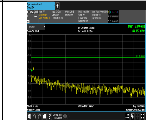
Band26_10MHz_16QAM_26840_1RB#49_0.009~0.15_0.009~0.15
