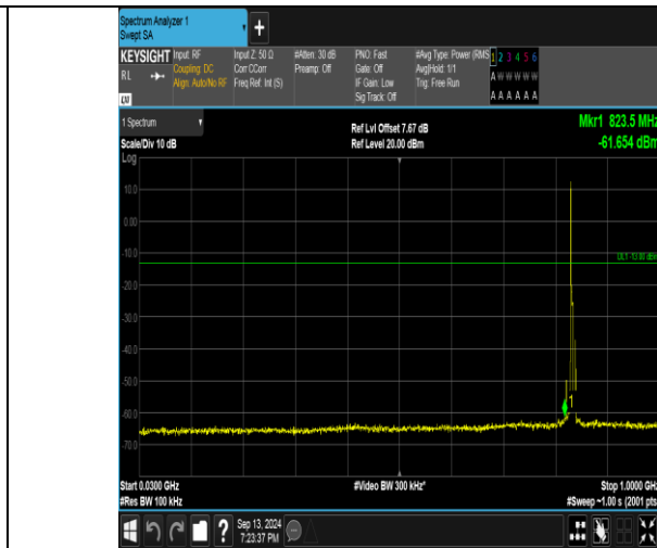
Band26_5MHz_16QAM_26915_1RB#0_30~1000_30~1000
