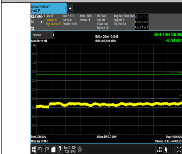
Band26_5MHz_QPSK_26915_1RB#0_3000~10000_3000~10000
