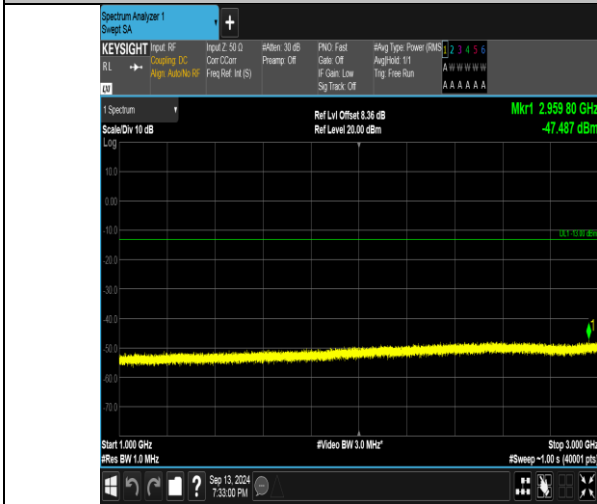
Band26_5MHz_16QAM_27015_25RB#0_1000~3000_1000~3000
