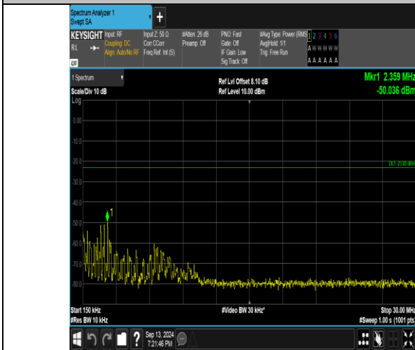
Band26_5MHz_16QAM_26815_25RB#0_0.15~30_0.15~30
