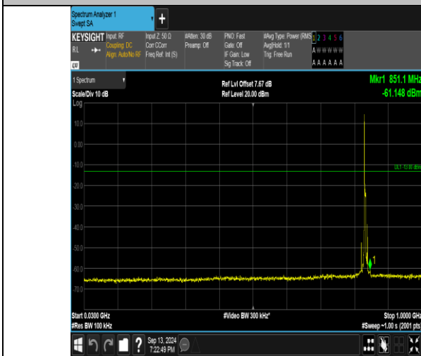
Band26_5MHz_QPSK_26915_1RB#0_30~1000_30~1000
