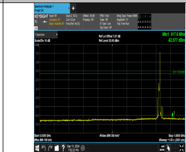
Band26_10MHz_16QAM_26840_1RB#49_30~1000_30~1000
