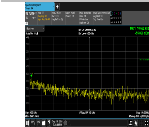
Band26_5MHz_QPSK_26915_25RB#0_0.009~0.15_0.009~0.15
