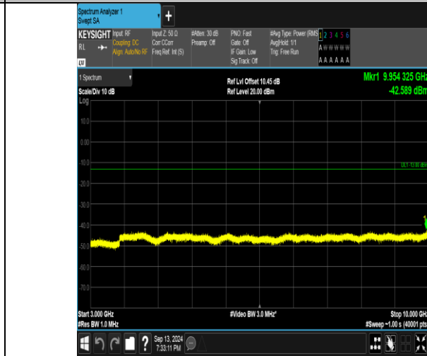
Band26_5MHz_16QAM_27015_25RB#0_3000~10000_3000~10000
