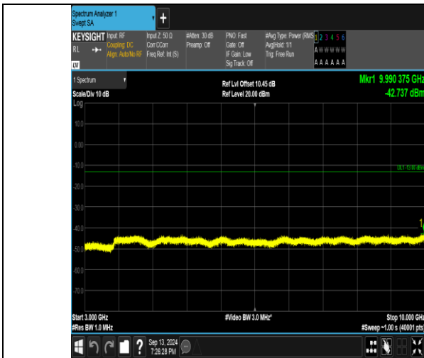
Band26_5MHz_QPSK_26915_25RB#0_3000~10000_3000~10000
