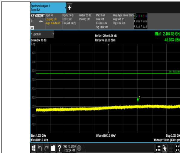
Band26_10MHz_16QAM_26840_1RB#49_1000~3000_1000~3000
