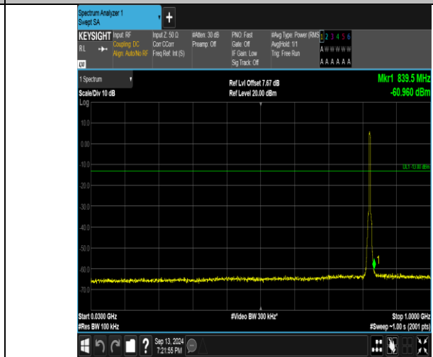
Band26_5MHz_16QAM_26815_25RB#0_30~1000_30~1000
