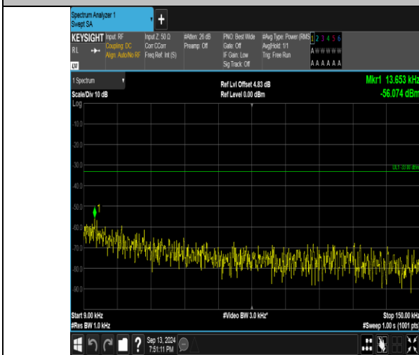
Band26_10MHz_QPSK_26840_1RB#49_0.009~0.15_0.009~0.15
