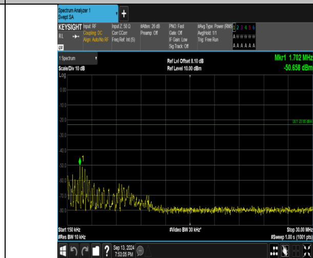
Band26_10MHz_QPSK_26840_50RB#0_0.15~30_0.15~30
