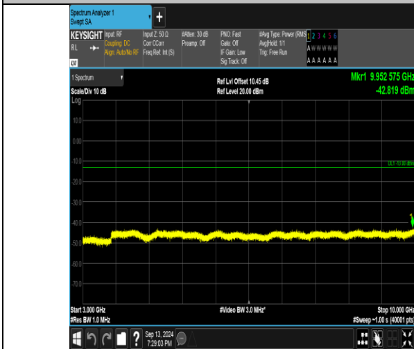
Band26_5MHz_QPSK_27015_1RB#0_3000~10000_3000~10000
