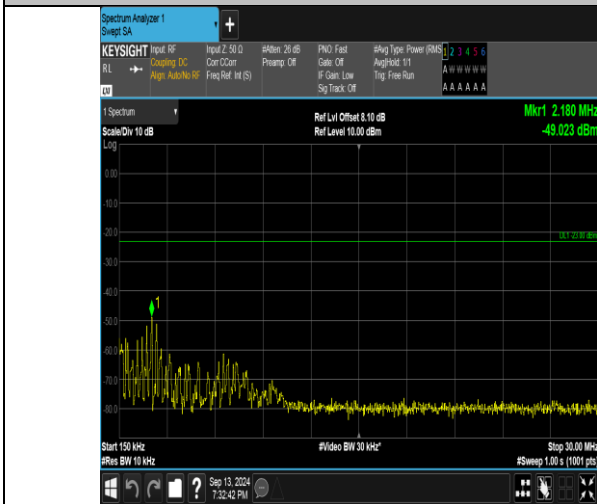
Band26_5MHz_16QAM_27015_25RB#0_0.15~30_0.15~30
