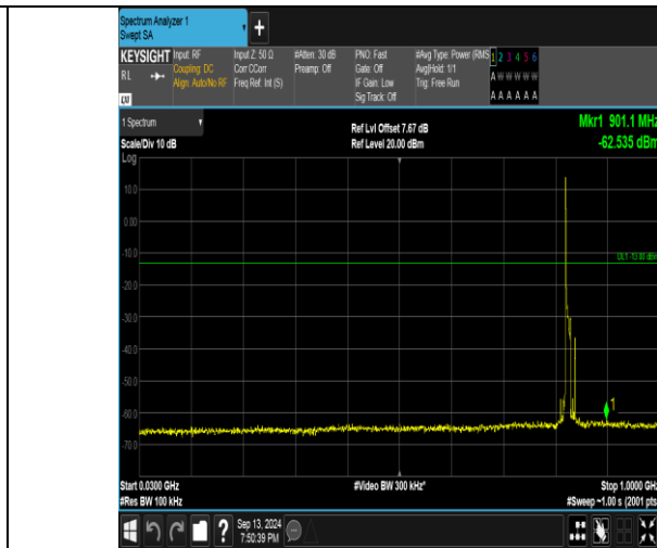
Band26_10MHz_16QAM_26840_1RB#0_30~1000_30~1000
