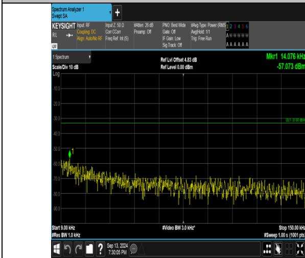
Band26_5MHz_QPSK_27015_1RB#24_0.009~0.15_0.009~0.15
