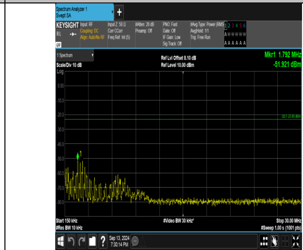
Band26_5MHz_QPSK_27015_1RB#24_0.15~30_0.15~30
