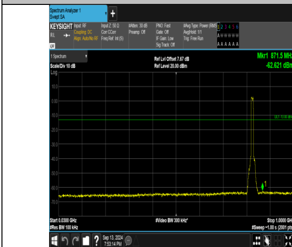
Band26_10MHz_QPSK_26840_50RB#0_30~1000_30~1000
