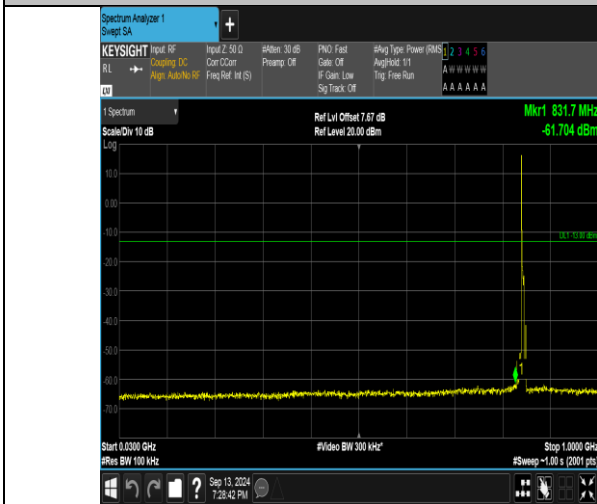
Band26_5MHz_QPSK_27015_1RB#0_30~1000_30~1000
