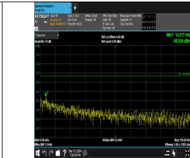
Band26_5MHz_16QAM_26915_25RB#0_0.009~0.15_0.009~0.15
