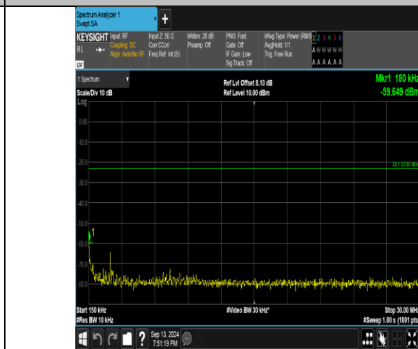
Band26_10MHz_QPSK_26840_1RB#49_0.15~30_0.15~30
