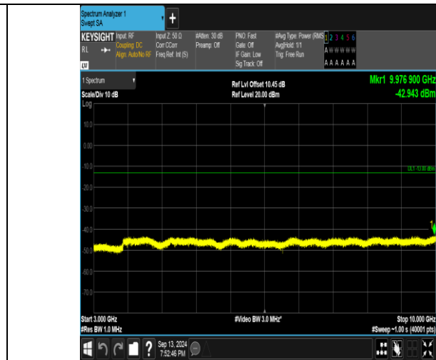
Band26_10MHz_16QAM_26840_1RB#49_3000~10000_3000~10000
