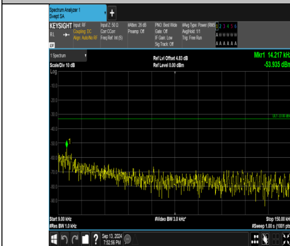
Band26_10MHz_QPSK_26840_50RB#0_0.009~0.15_0.009~0.15
