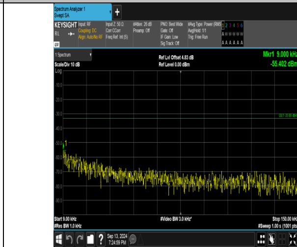
Band26_5MHz_16QAM_26915_1RB#24_0.009~0.15_0.009~0.15
