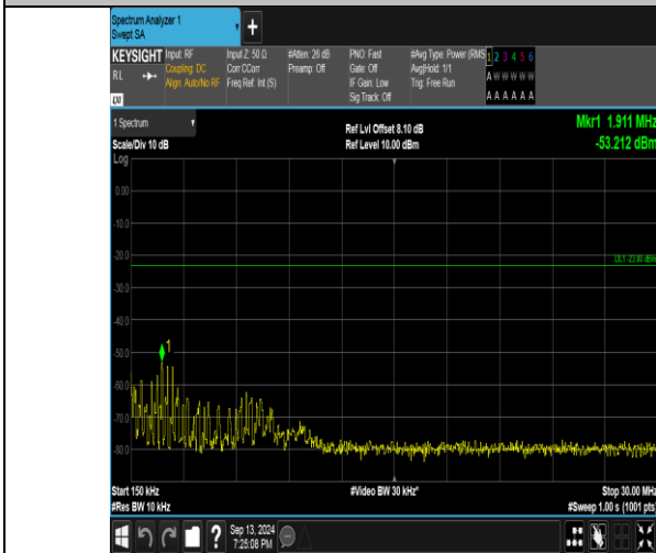
Band26_5MHz_16QAM_26915_1RB#24_0.15~30_0.15~30
