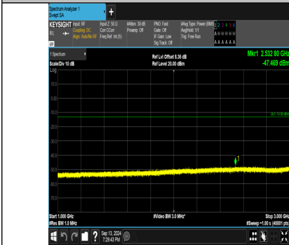
Band26_5MHz_16QAM_27015_1RB#0_1000~3000_1000~3000
