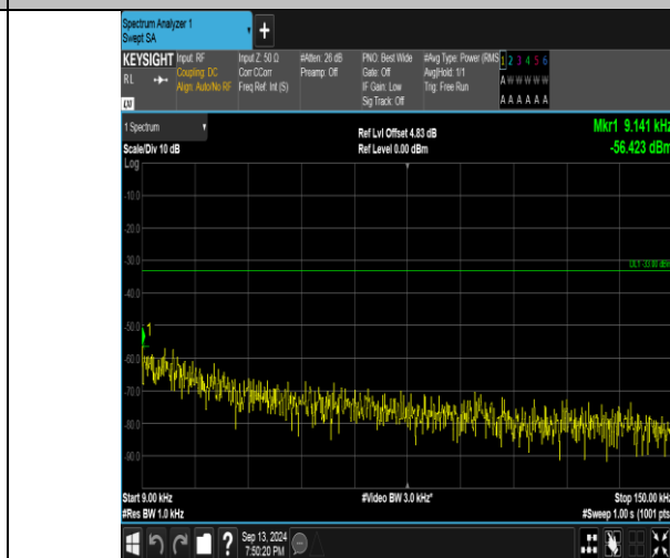
Band26_10MHz_16QAM_26840_1RB#0_0.009-0.15_0.009-0.15
