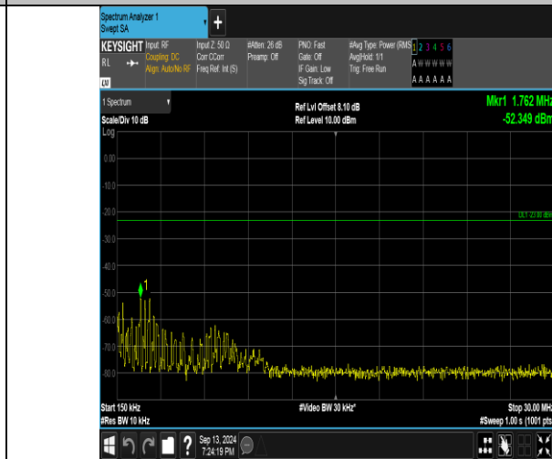
Band26_5MHz_QPSK_26915_1RB#24_0.15~30_0.15~30
