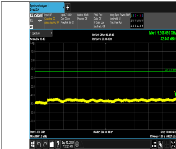
Band26_5MHz_QPSK_27015_25RB#0_3000~10000_3000~10000
