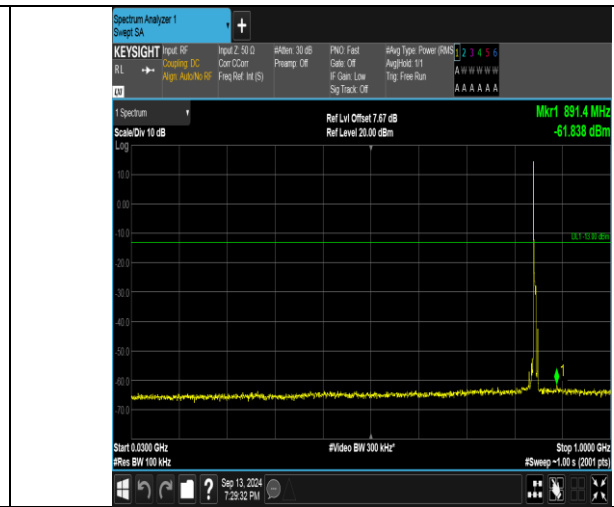
Band26_5MHz_16QAM_27015_1RB#0_30~1000_30~1000
