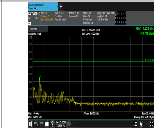
Band26_5MHz_QPSK_26915_25RB#0_0.15~30_0.15~30
