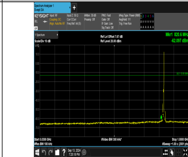
Band26_5MHz_16QAM_26915_1RB#24_30~1000_30~1000
