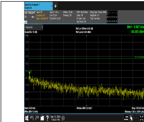
Band26_10MHz_QPSK_26840_1RB#0_0.009-0.15_0.009-0.15
