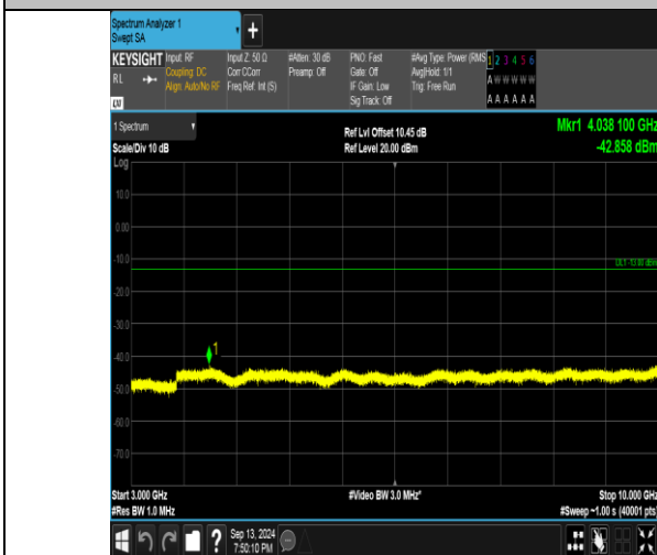
Band26_10MHz_QPSK_26840_1RB#0_3000-10000_3000-10000
