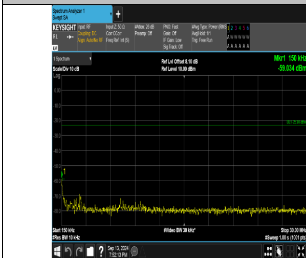
Band26_10MHz_16QAM_26840_1RB#49_0.15~30_0.15~30
