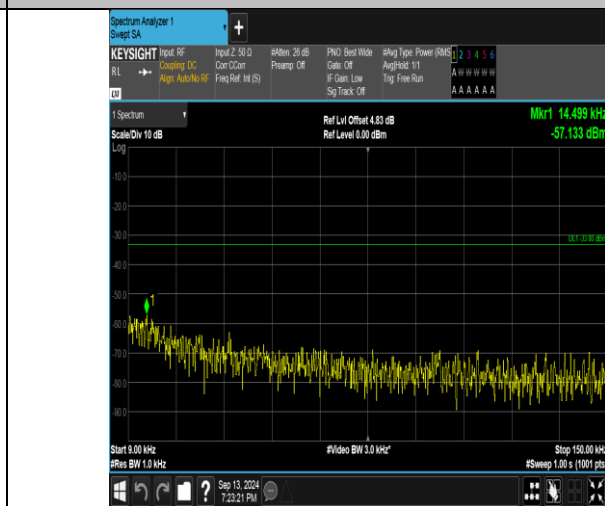
Band26_5MHz_16QAM_26915_1RB#0_0.009~0.15_0.009~0.15
