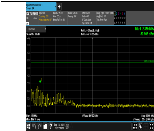
Band26_5MHz_16QAM_27015_1RB#0_0.15~30_0.15~30
