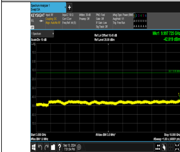
Band26_10MHz_QPSK_26840_1RB#49_3000~10000_3000~10000
