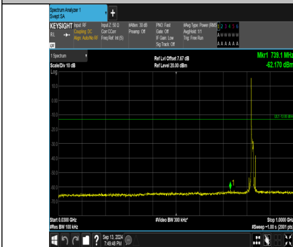
Band26_10MHz_QPSK_26840_1RB#0_30-1000_30-1000
