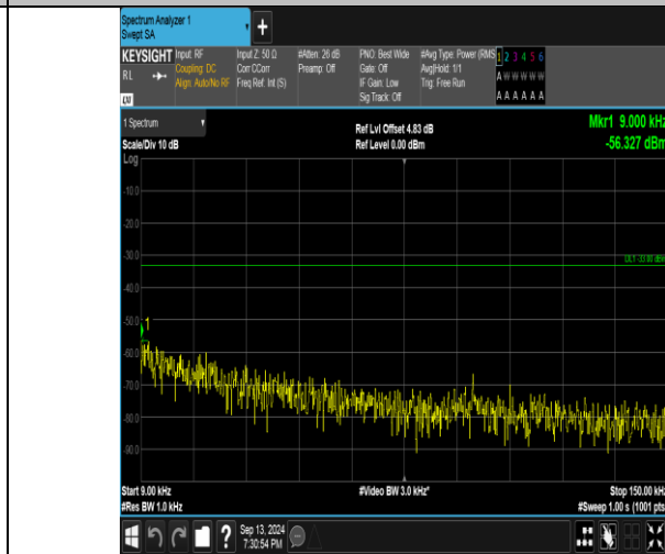
Band26_5MHz_16QAM_27015_1RB#24_0.009~0.15_0.009~0.15
