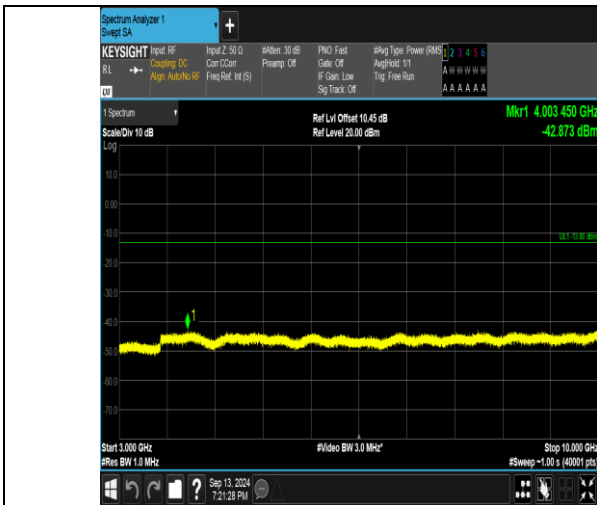
Band26_5MHz_QPSK_26815_25RB#0_3000~10000_3000~10000
