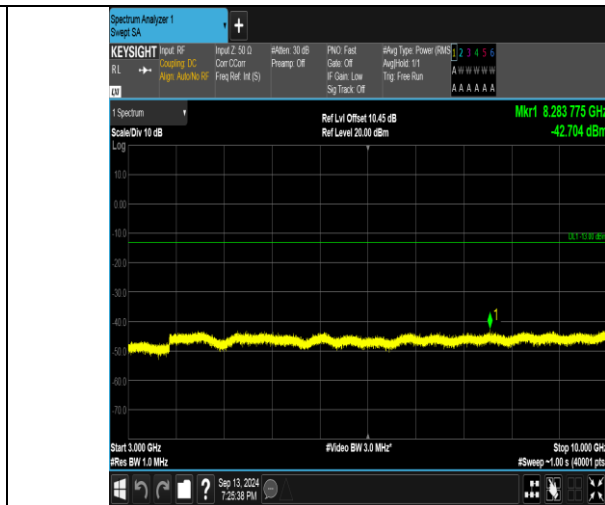
Band26_5MHz_16QAM_26915_1RB#24_3000~10000_3000~10000
