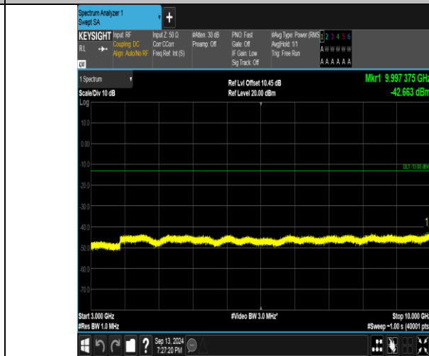
Band26_5MHz_16QAM_26915_25RB#0_3000~10000_3000~10000
