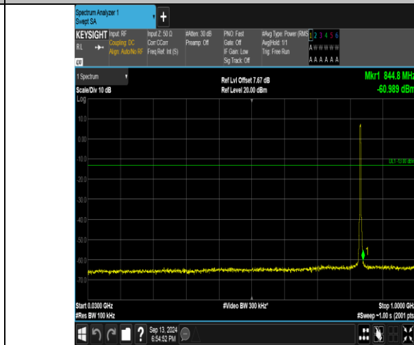
Band26_3MHz_16QAM_26915_15RB#0_30~1000_30~1000
