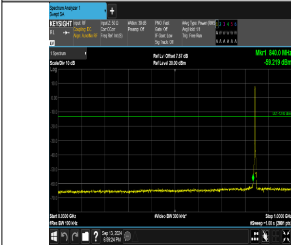
Band26_3MHz_QPSK_27025_15RB#0_30~1000_30~1000
