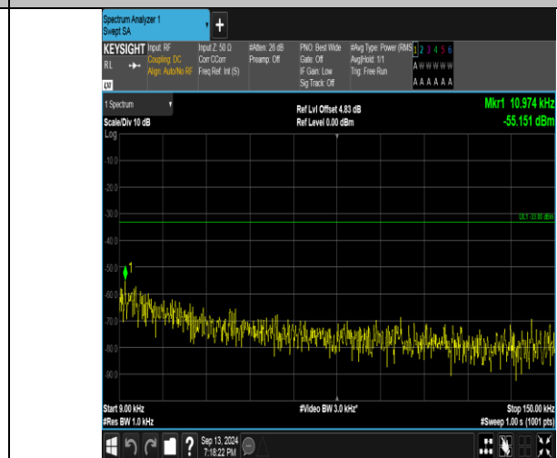
Band26_5MHz_16QAM_26815_1RB#0_0.009~0.15_0.009~0.15
