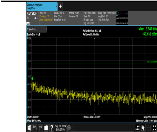
Band26_3MHz_QPSK_27025_15RB#0_0.009~0.15_0.009~0.15
