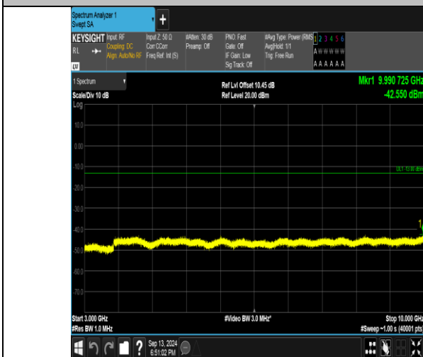
Band26_3MHz_QPSK_26915_1RB#0_3000~10000_3000~10000
