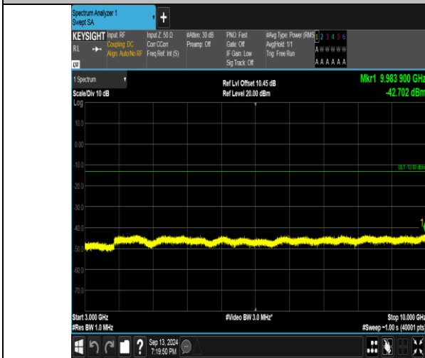
Band26_5MHz_QPSK_26815_1RB#24_3000~10000_3000~10000
