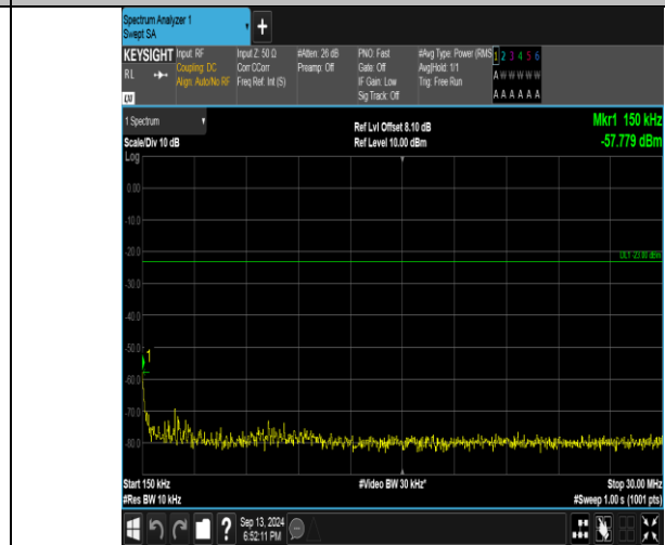
Band26_3MHz_QPSK_26915_1RB#14_0.15~30_0.15~30
