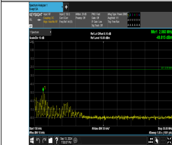
Band26_3MHz_16QAM_27025_15RB#0_0.15~30_0.15~30
