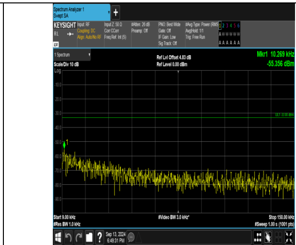
Band26_3MHz_16QAM_26805_15RB#0_0.009~0.15_0.009~0.15
