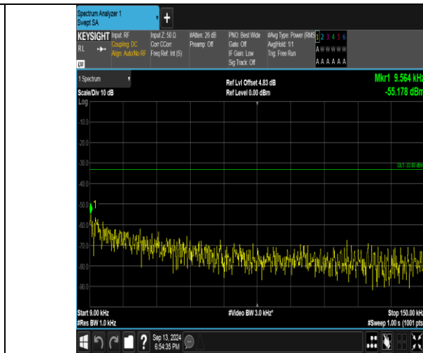
Band26_3MHz_16QAM_26915_15RB#0_0.009~0.15_0.009~0.15
