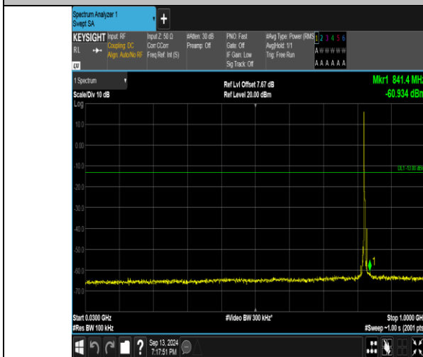
Band26_5MHz_QPSK_26815_1RB#0_30~1000_30~1000
