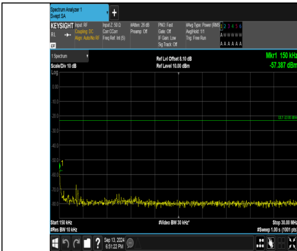
Band26_3MHz_16QAM_26915_1RB#0_0.15~30_0.15~30
