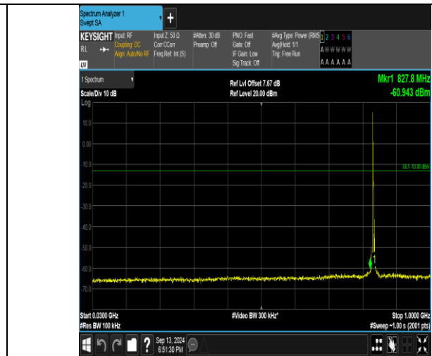
Band26_3MHz_16QAM_26915_1RB#0_30~1000_30~1000
