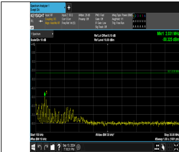
Band26_5MHz_16QAM_26815_1RB#0_0.15~30_0.15~30
