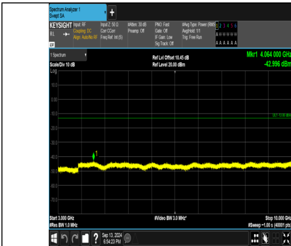
Band26_3MHz_QPSK_26915_15RB#0_3000~10000_3000~10000
