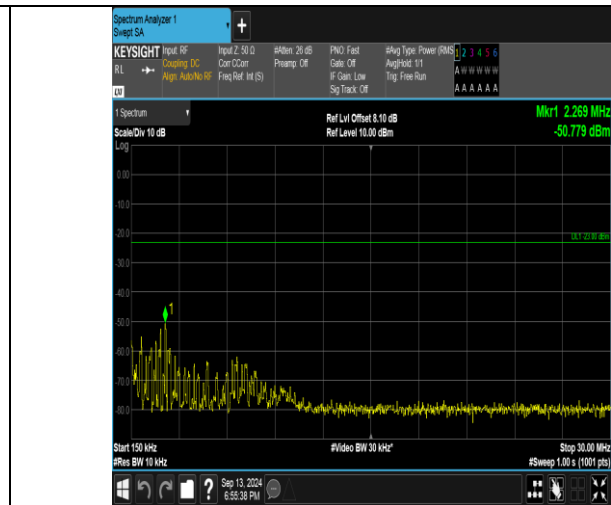
Band26_3MHz_QPSK_27025_1RB#0_0.15~30_0.15~30
