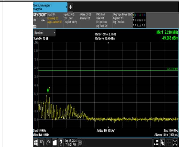
Band26_5MHz_QPSK_26815_1RB#24_0.15~30_0.15~30
