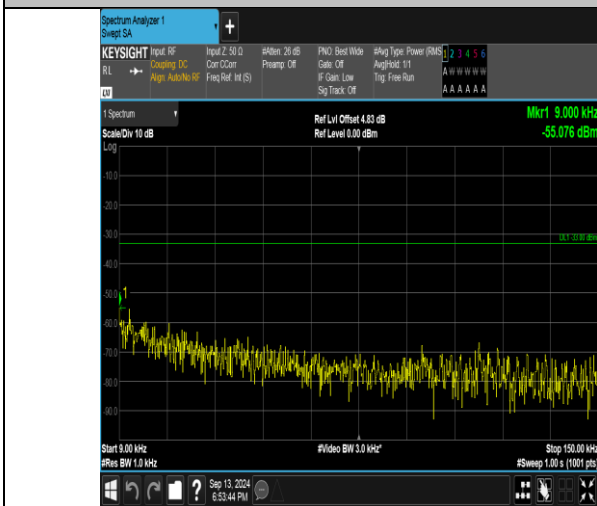
Band26_3MHz_QPSK_26915_15RB#0_0.009~0.15_0.009~0.15
