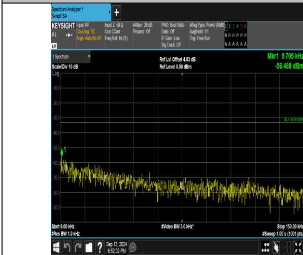
Band26_3MHz_QPSK_26915_1RB#14_0.009~0.15_0.009~0.15
