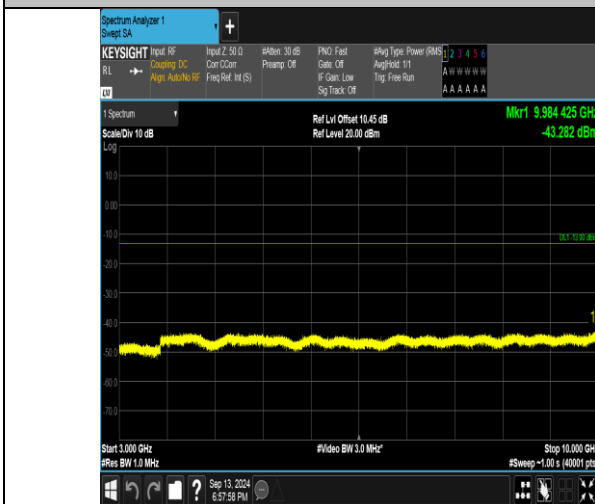
Band26_3MHz_QPSK_27025_1RB#14_3000~10000_3000~10000
