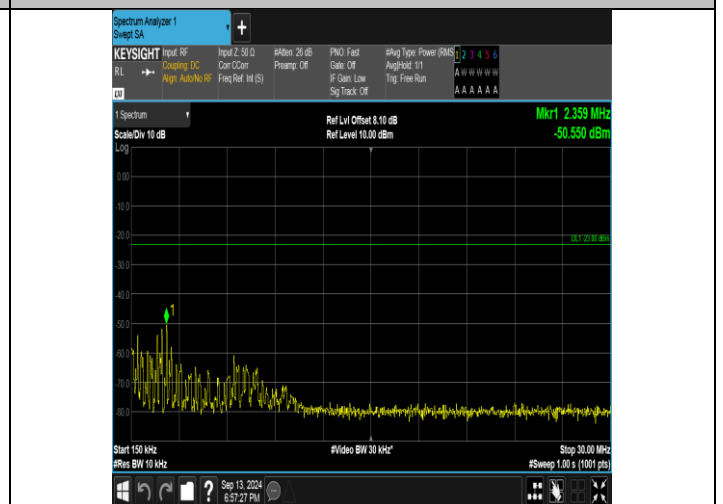
Band26_3MHz_QPSK_27025_1RB#14_0.15~30_0.15~30
