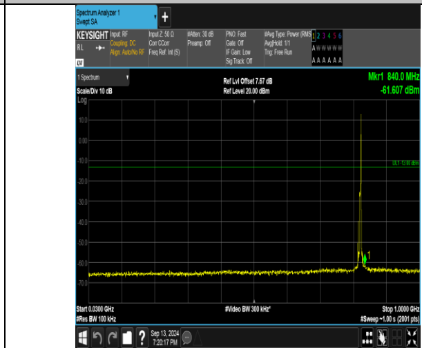
Band26_5MHz_16QAM_26815_1RB#24_30~1000_30~1000
