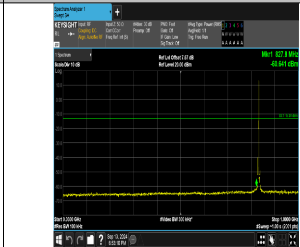
Band26_3MHz_16QAM_26915_1RB#14_30~1000_30~1000
