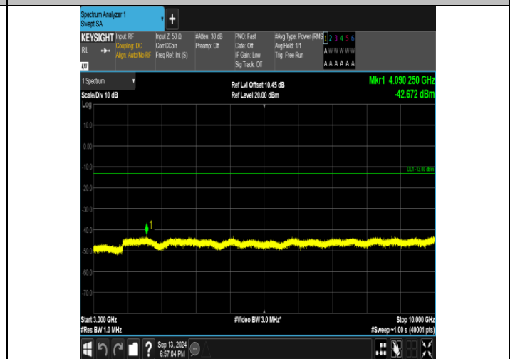
Band26_3MHz_16QAM_27025_1RB#0_3000~10000_3000~10000
