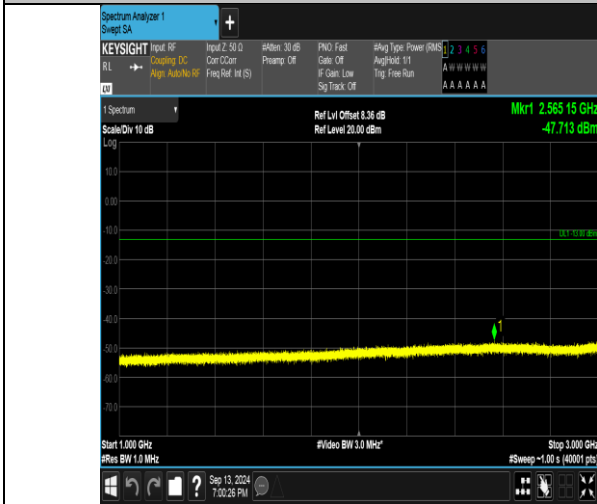
Band26_3MHz_16QAM_27025_15RB#0_1000~3000_1000~3000
