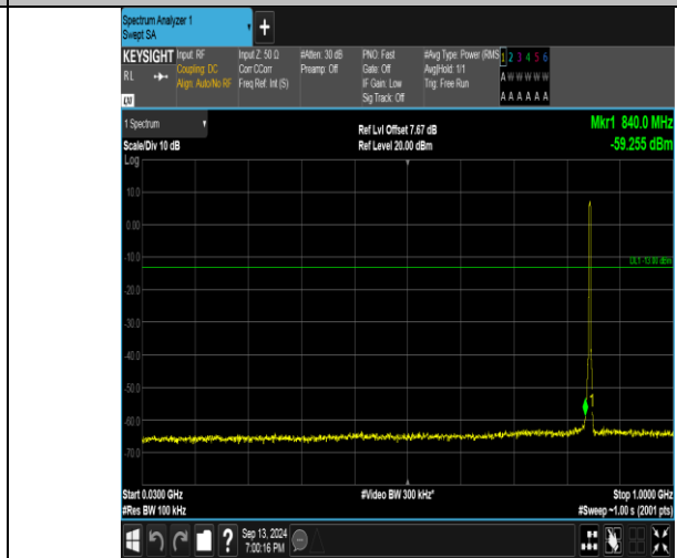
Band26_3MHz_16QAM_27025_15RB#0_30~1000_30~1000
