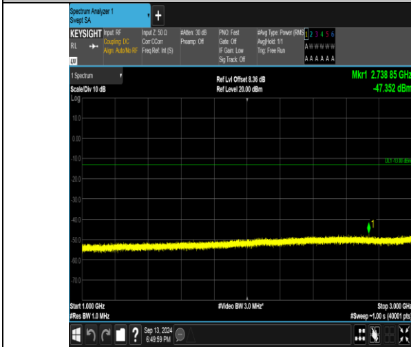
Band26_3MHz_16QAM_26805_15RB#0_1000~3000_1000~3000
