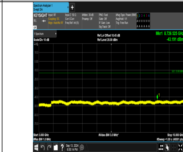
Band26_3MHz_16QAM_26915_15RB#0_3000~10000_3000~10000
