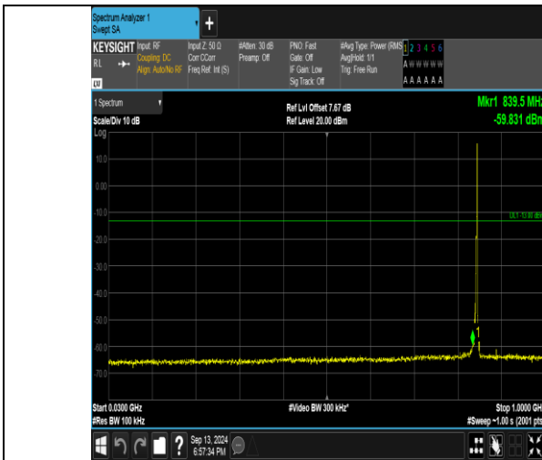
Band26_3MHz_QPSK_27025_1RB#14_30~1000_30~1000
