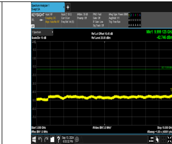
Band26_3MHz_16QAM_26915_1RB#14_3000~10000_3000~10000
