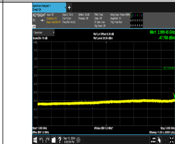
Band26_3MHz_QPSK_27025_1RB#0_1000~3000_1000~3000
