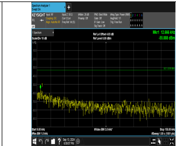
Band26_3MHz_16QAM_27025_15RB#0_0.009~0.15_0.009~0.15
