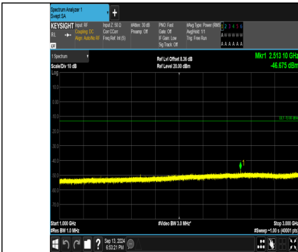
Band26_3MHz_16QAM_26915_1RB#14_1000~3000_1000~3000
