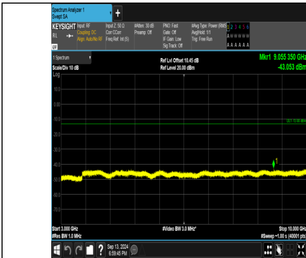
Band26_3MHz_QPSK_27025_15RB#0_3000~10000_3000~10000
