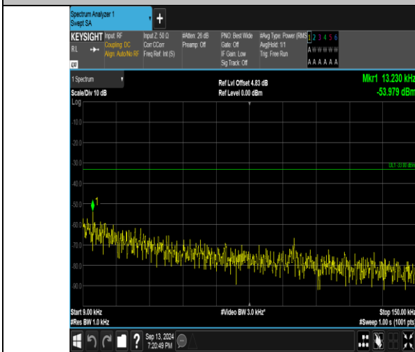
Band26_5MHz_QPSK_26815_25RB#0_0.009~0.15_0.009~0.15
