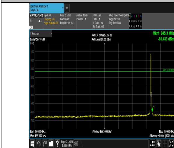
Band26_3MHz_QPSK_26915_15RB#0_30~1000_30~1000
