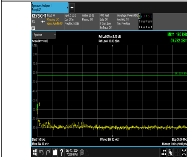
Band26_5MHz_16QAM_26815_1RB#24_0.15~30_0.15~30
