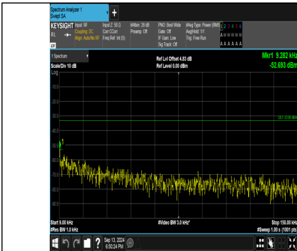
Band26_3MHz_QPSK_26915_1RB#0_0.009~0.15_0.009~0.15
