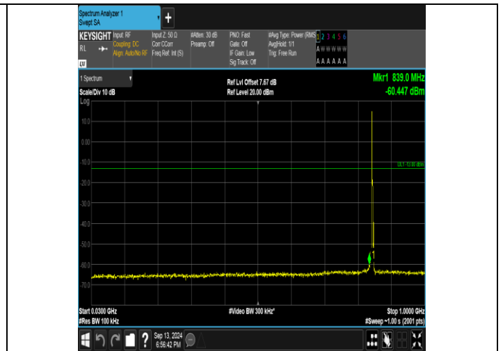
Band26_3MHz_16QAM_27025_1RB#0_30~1000_30~1000
