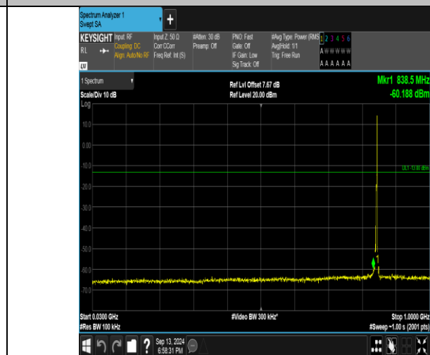
Band26_3MHz_16QAM_27025_1RB#14_30~1000_30~1000
