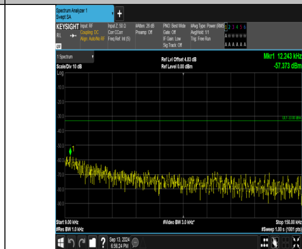
Band26_3MHz_16QAM_27025_1RB#0_0.009~0.15_0.009~0.15
