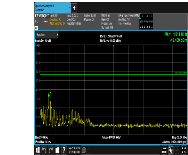
Band26_5MHz_QPSK_26815_1RB#0_0.15~30_0.15~30
