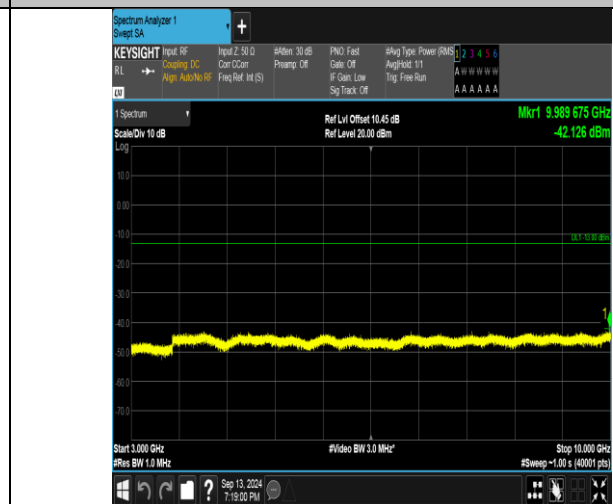
Band26_5MHz_16QAM_26815_1RB#0_3000~10000_3000~10000
