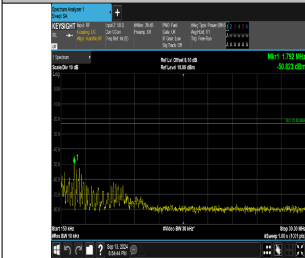
Band26_3MHz_16QAM_26915_15RB#0_0.15~30_0.15~30
