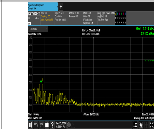
Band26_3MHz_QPSK_26915_15RB#0_0.15~30_0.15~30
