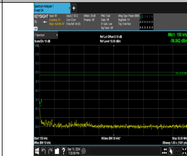
Band26_5MHz_QPSK_26815_25RB#0_0.15~30_0.15~30
