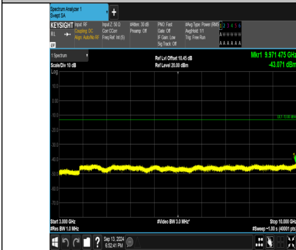
Band26_3MHz_QPSK_26915_1RB#14_3000~10000_3000~10000
