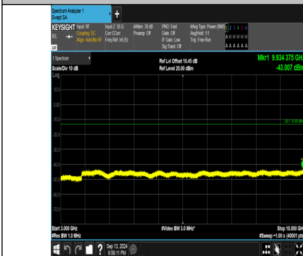
Band26_3MHz_QPSK_27025_1RB#0_3000~10000_3000~10000
