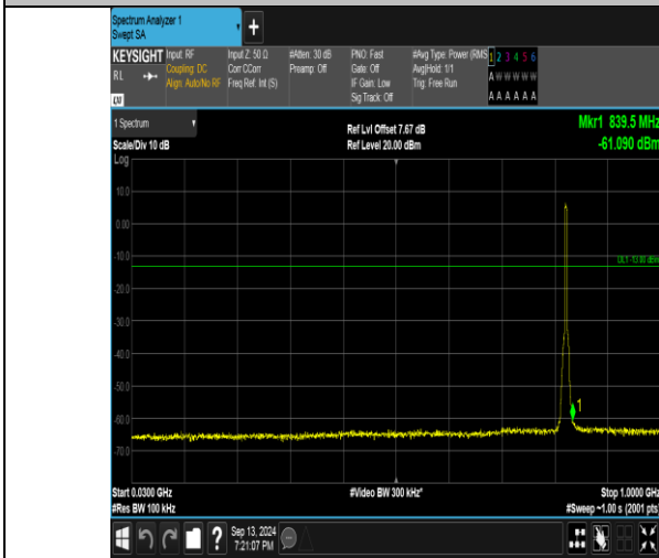
Band26_5MHz_QPSK_26815_25RB#0_30~1000_30~1000
