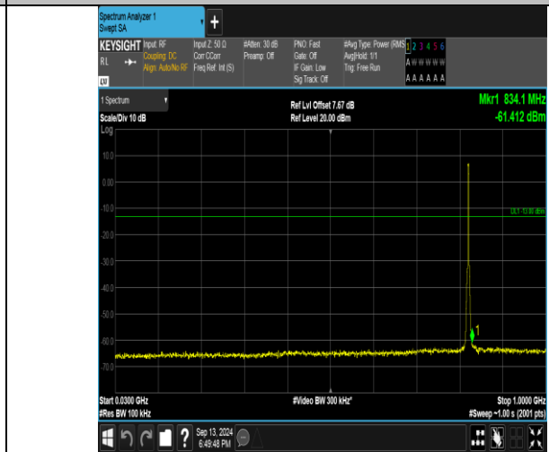
Band26_3MHz_16QAM_26805_15RB#0_30~1000_30~1000
