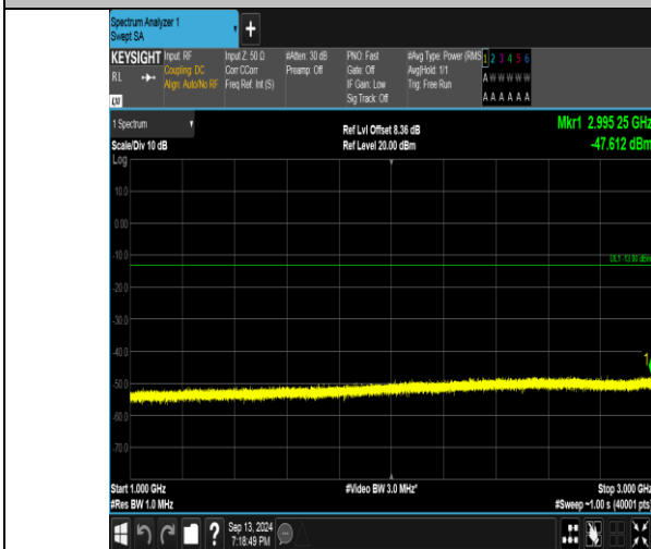
Band26_5MHz_16QAM_26815_1RB#0_1000~3000_1000~3000
