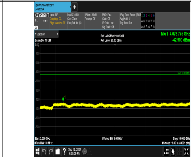
Band26_3MHz_16QAM_26805_15RB#0_3000~10000_3000~10000
