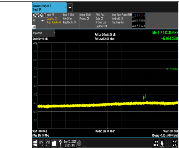
Band26_3MHz_QPSK_26915_1RB#14_1000~3000_1000~3000
