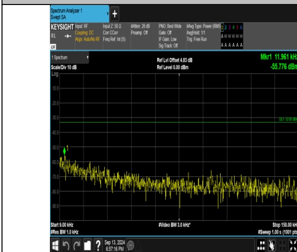
Band26_3MHz_QPSK_27025_1RB#14_0.009~0.15_0.009~0.15
