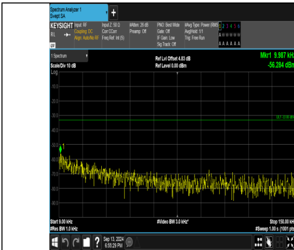
Band26_3MHz_QPSK_27025_1RB#0_0.009~0.15_0.009~0.15
