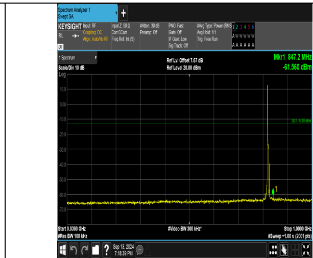
Band26_5MHz_16QAM_26815_1RB#0_30~1000_30~1000
