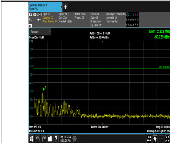
Band26_3MHz_16QAM_26915_1RB#14_0.15~30_0.15~30
