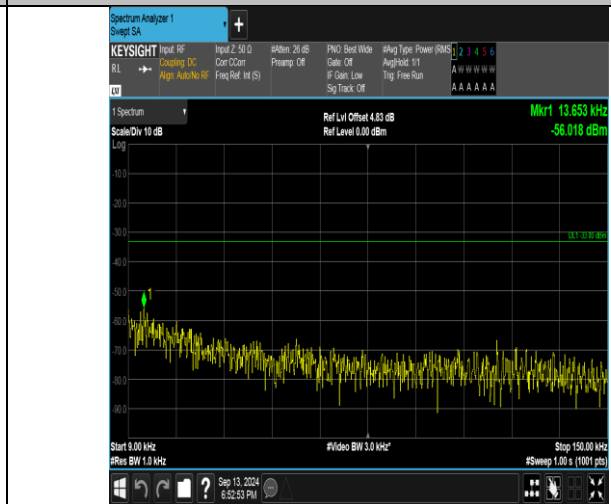
Band26_3MHz_16QAM_26915_1RB#14_0.009~0.15_0.009~0.15
