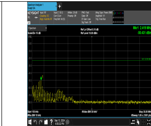
Band26_3MHz_QPSK_26915_1RB#0_0.15~30_0.15~30
