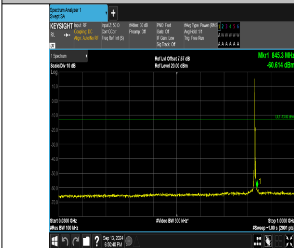
Band26_3MHz_QPSK_26915_1RB#0_30~1000_30~1000
