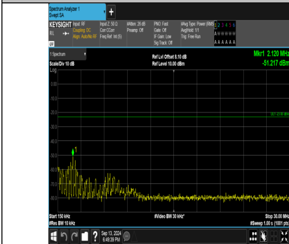
Band26_3MHz_16QAM_26805_15RB#0_0.15~30_0.15~30
