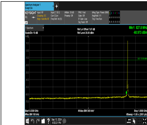
Band26_3MHz_QPSK_26915_1RB#14_30~1000_30~1000
