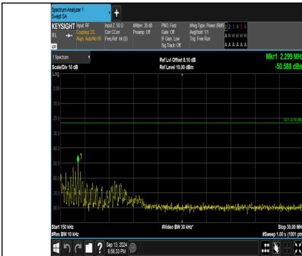
Band26_3MHz_16QAM_27025_1RB#0_0.15~30_0.15~30
