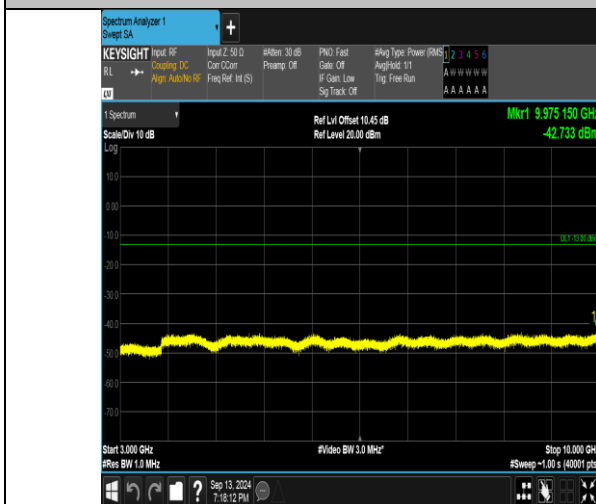
Band26_5MHz_QPSK_26815_1RB#0_3000~10000_3000~10000
