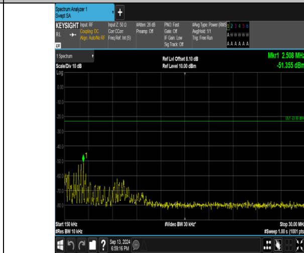
Band26_3MHz_QPSK_27025_15RB#0_0.15~30_0.15~30
