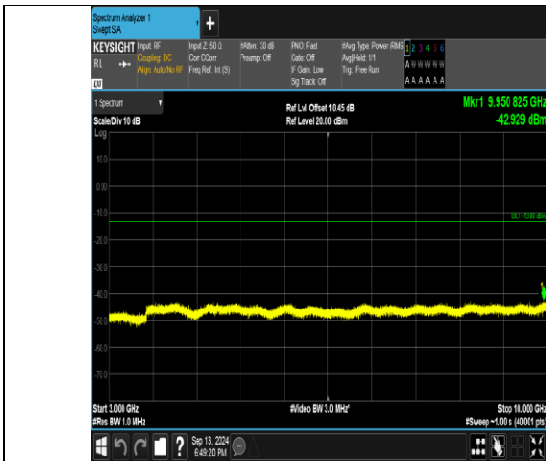
Band26_3MHz_QPSK_26805_15RB#0_3000~10000_3000~10000
