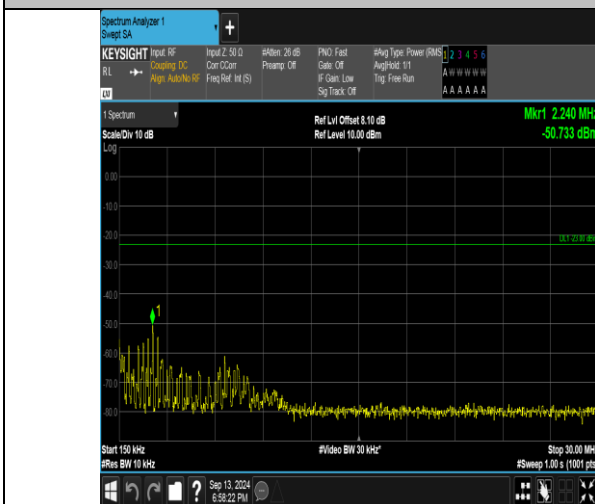
Band26_3MHz_16QAM_27025_1RB#14_0.15~30_0.15~30
