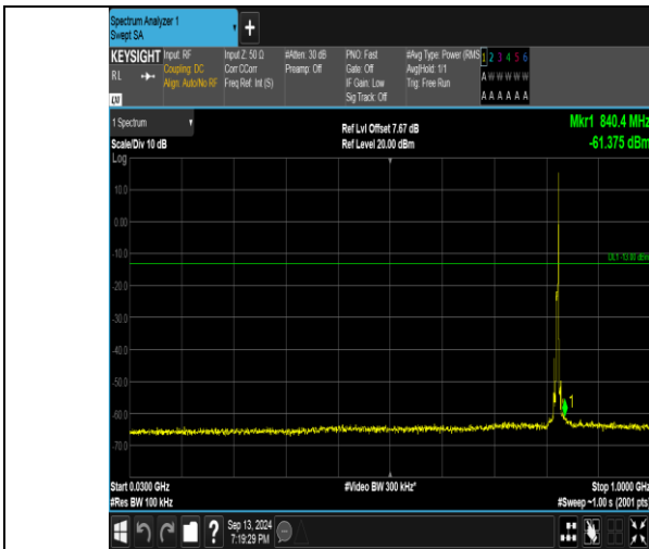
Band26_5MHz_QPSK_26815_1RB#24_30~1000_30~1000
