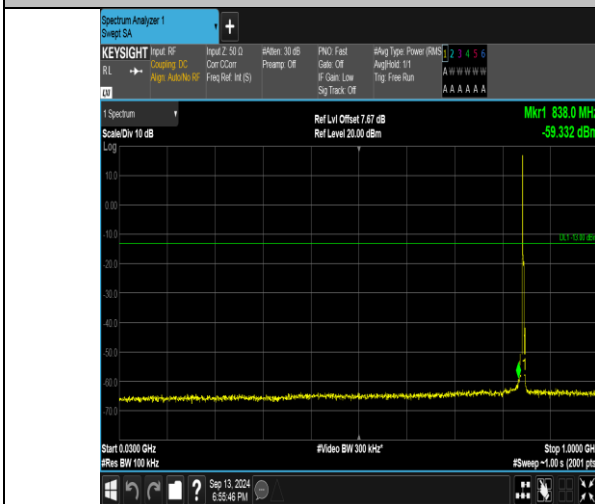
Band26_3MHz_QPSK_27025_1RB#0_30~1000_30~1000
