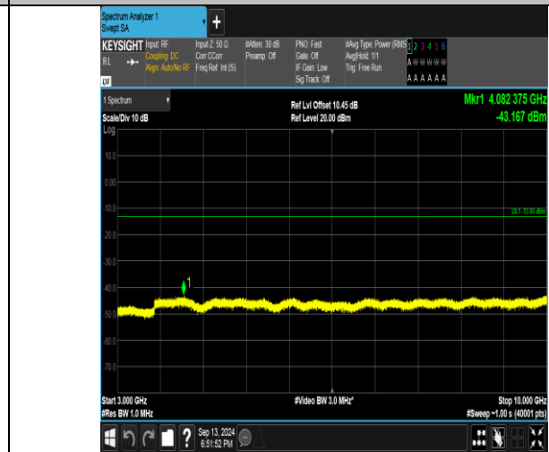
Band26_3MHz_16QAM_26915_1RB#0_3000~10000_3000~10000
