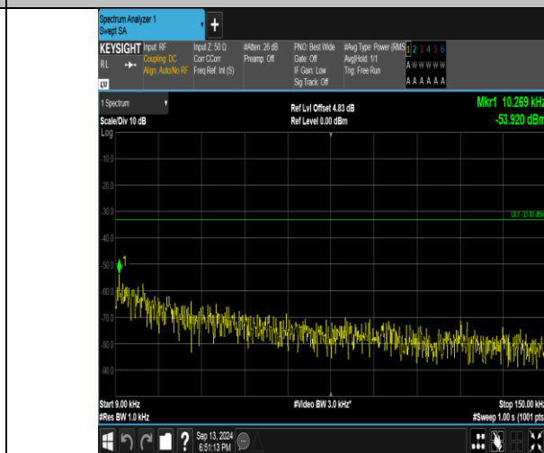
Band26_3MHz_16QAM_26915_1RB#0_0.009~0.15_0.009~0.15
